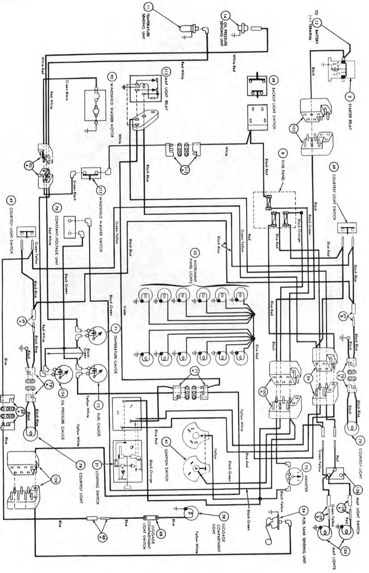
1964 THUNDERBIRD INTERIOR LIGHTING, WINDSHIELD WIPER AND GAUGE SCHEMATIC
