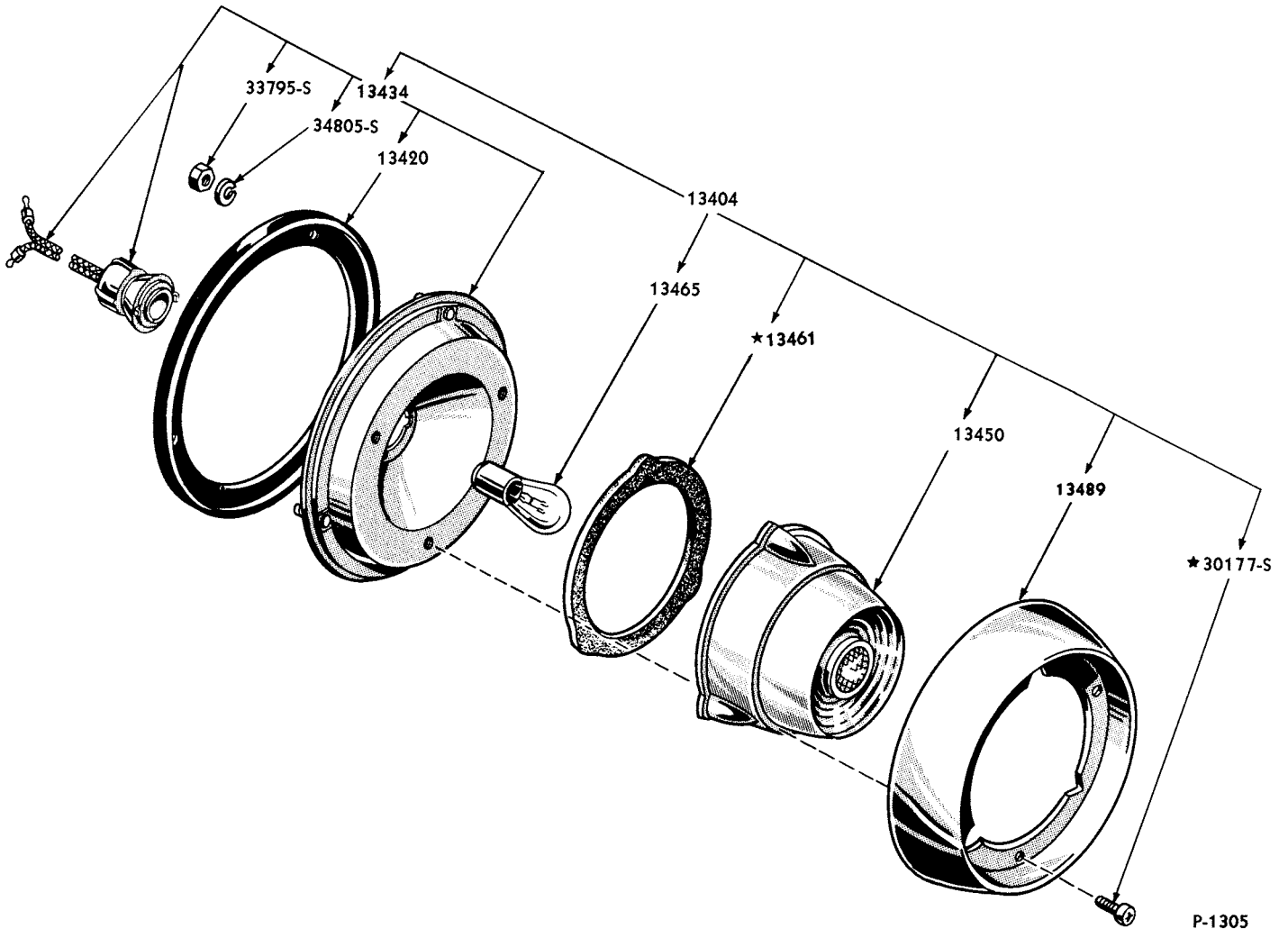
1952 REAR LAMP
