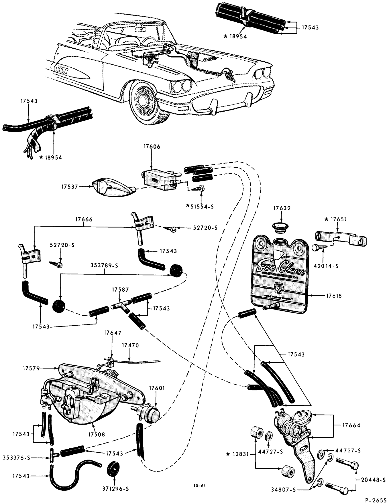
1958/59 WINDSHIELD WASHER (THUNDERBIRD)
