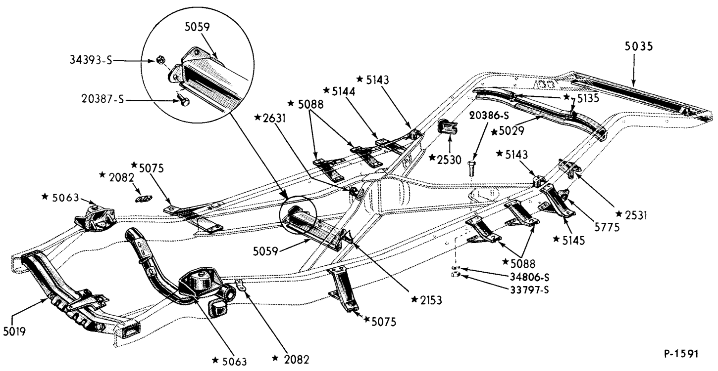
"X" TYPE" 1954 FRAME
