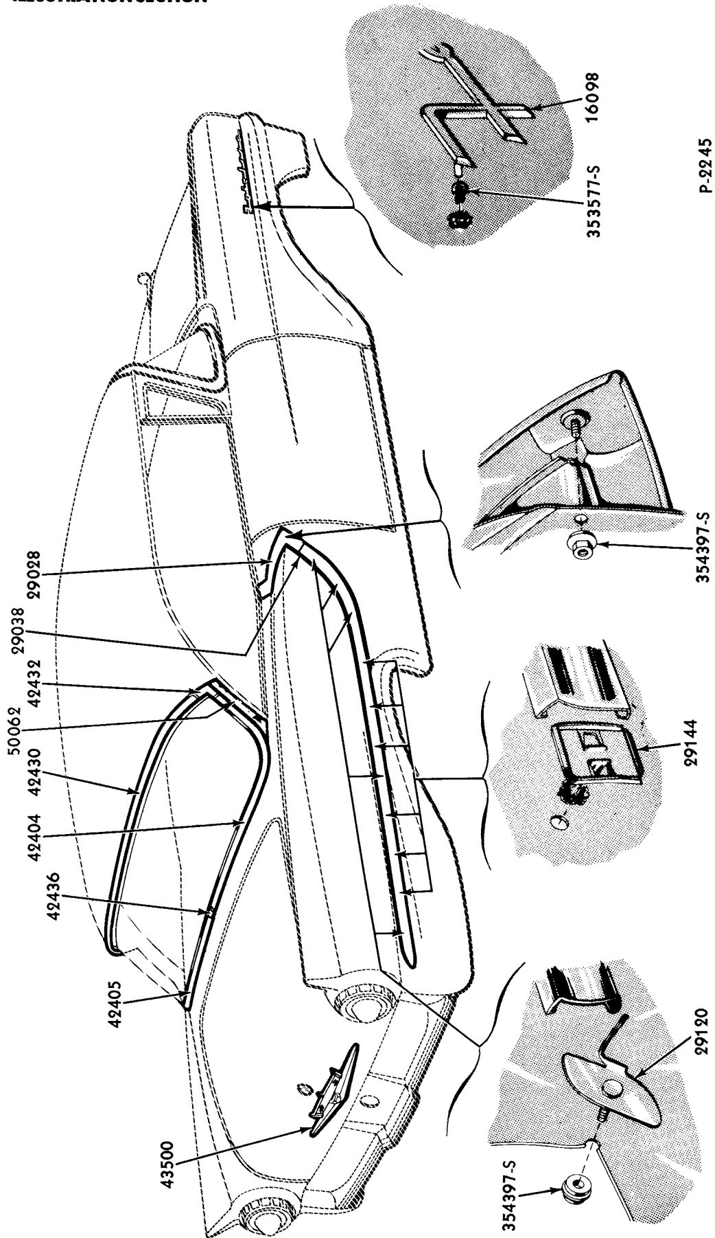
1957 FAIRLANE CLUB VICTORIA (BODY TYPES 63B, 64A)-TYPICAL
