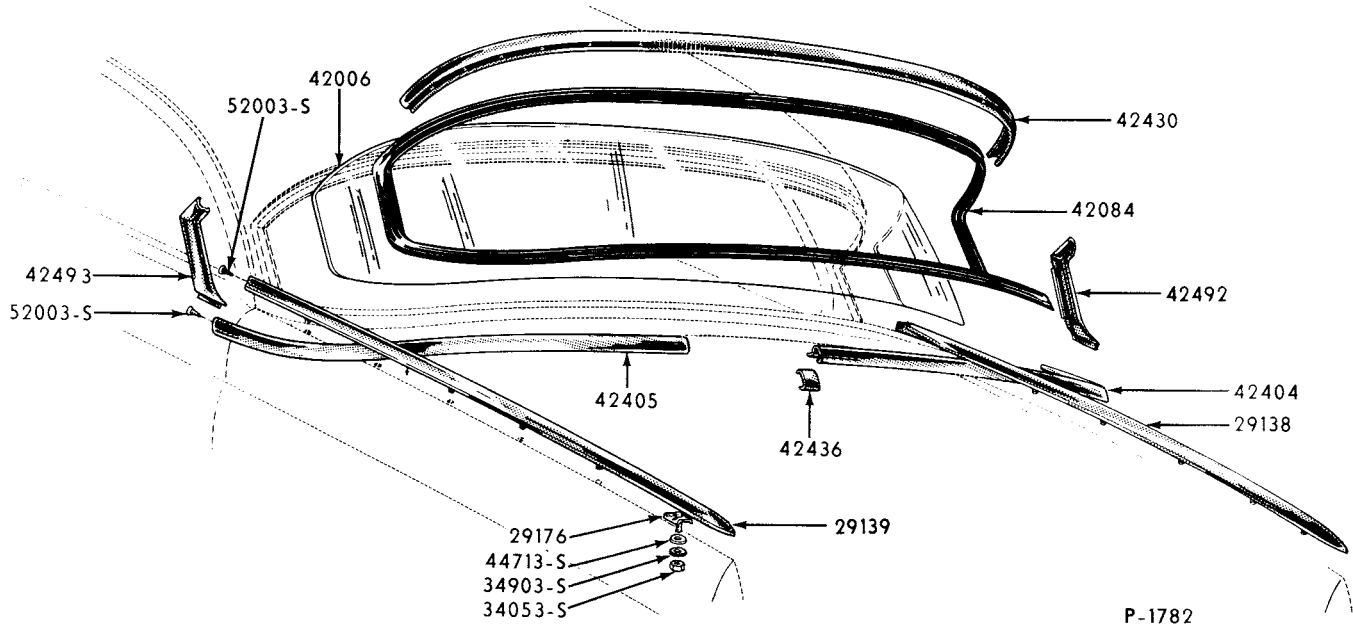
1955 BODY TYPES 70C, 73C BACK WINDOW & RELATED PARTS
