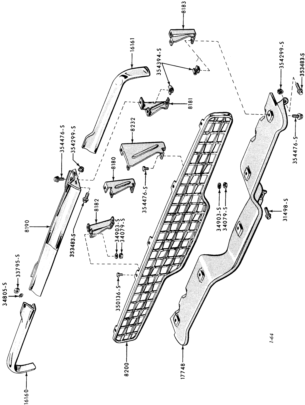
1959 RADIATOR GRILLE & RELATED PARTS (FORD)
