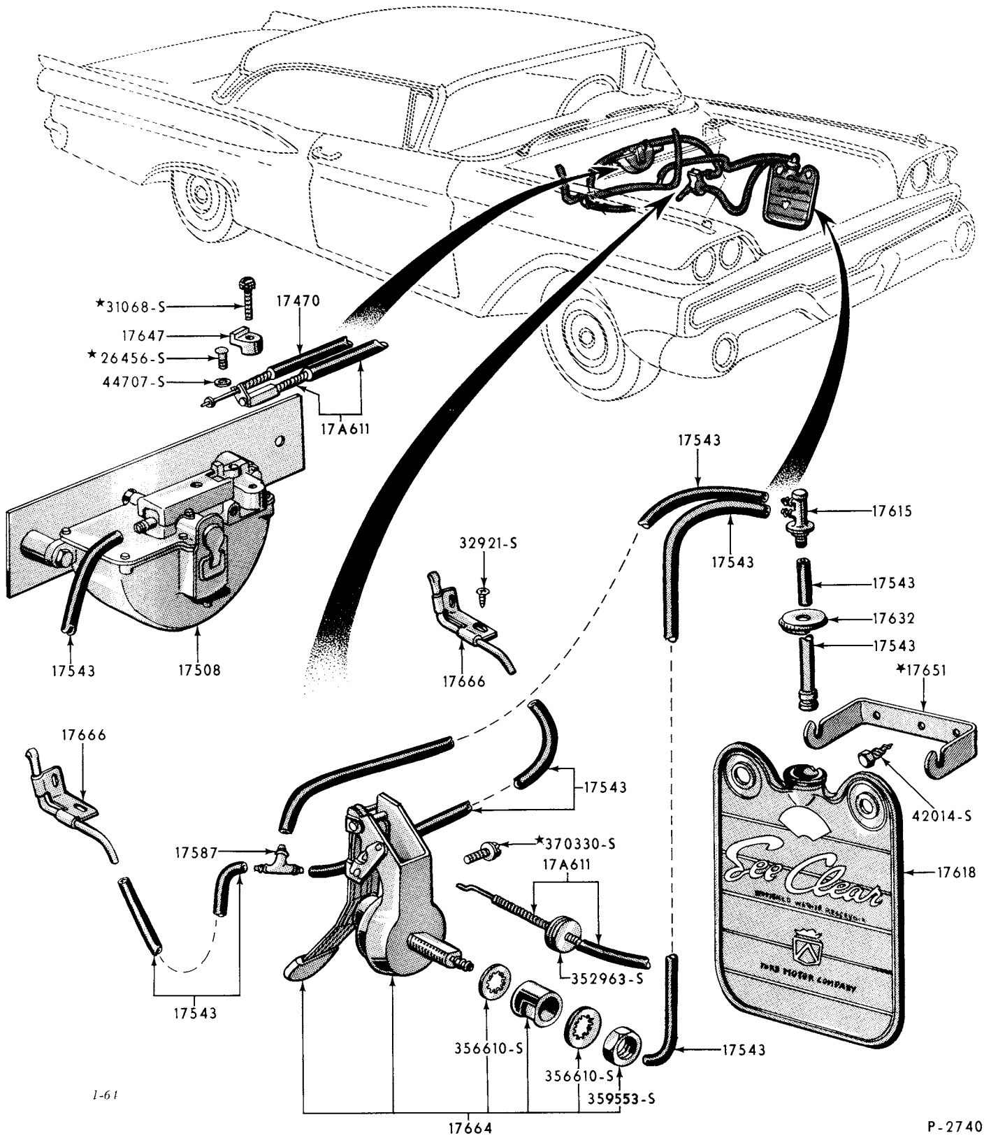
1959 WINDSHIELD WASHER (FORD)
