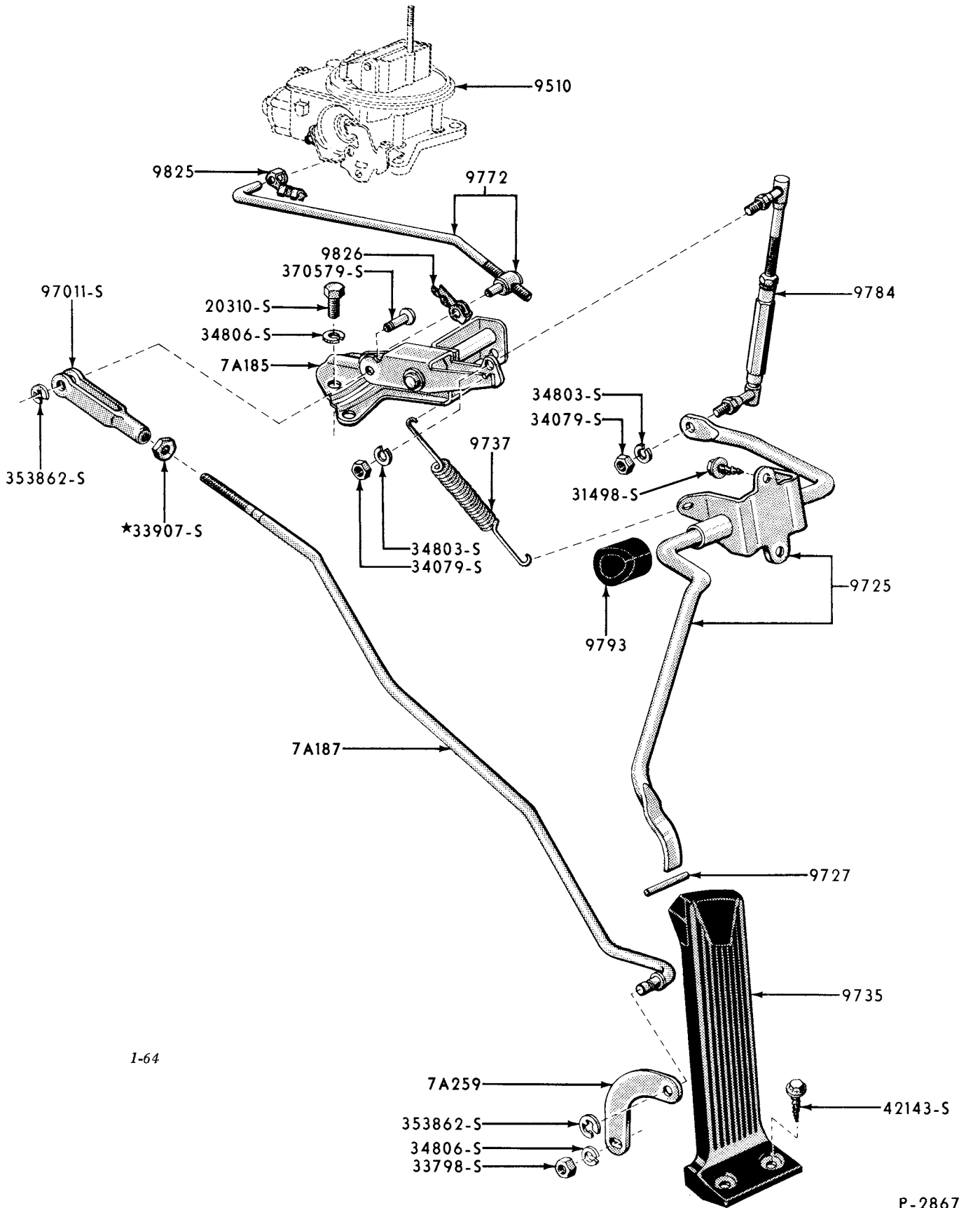
1959 ACCELERATOR LINKAGE - FORD (8 CYLINDER)-WITH FORDOMATIC
