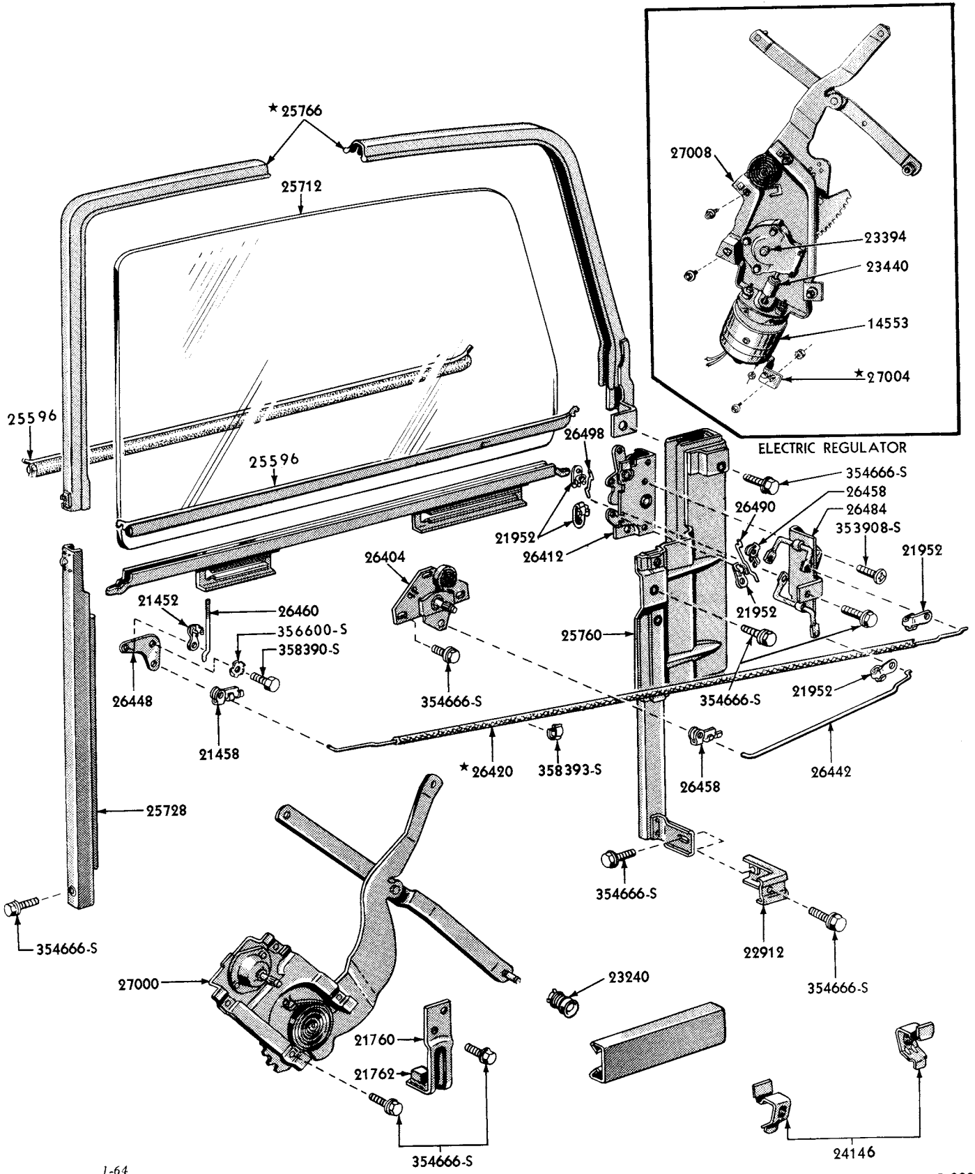
1957/58 REAR DOOR PARTS (BODY TYPE 79)-TYPICAL
