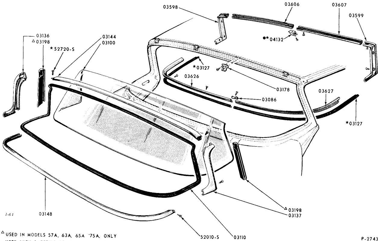
1959 WINDSHIELD PARTS (BODY TYPES 54A, 57A, 58, 59, 63A, 64, 65A, 66C, 71, 75A)
