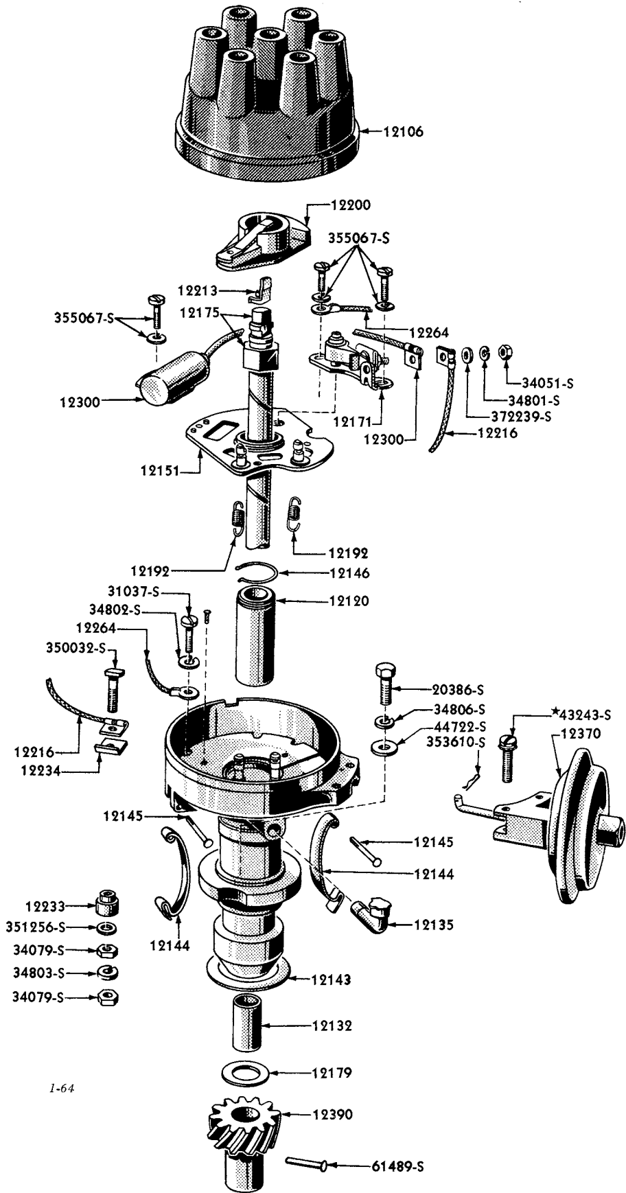
1952/57 "TYPICAL" DISTRIBUTOR (6 CYLINDER 215 & 223 ENGINES)
