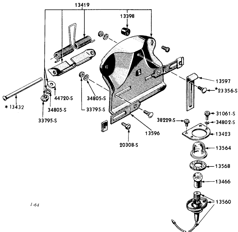
1955/56 "TYPICAL" LICENSE PLATE LAMP (FORD)
