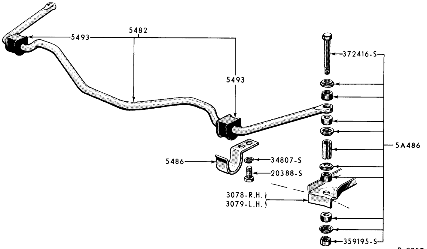
1959 PASSENGER STABILIZER
