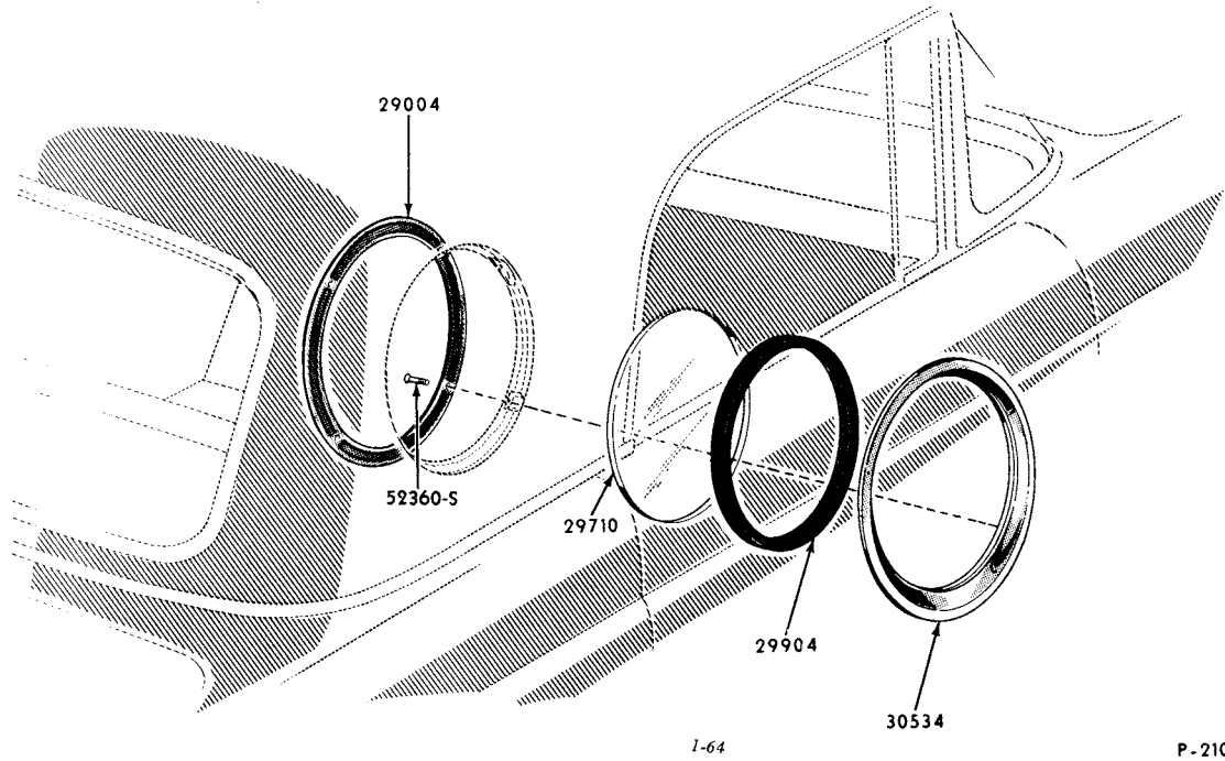
1956/57 HARD TOP QUARTER WINDOW PARTS (THUNDERBIRD)
