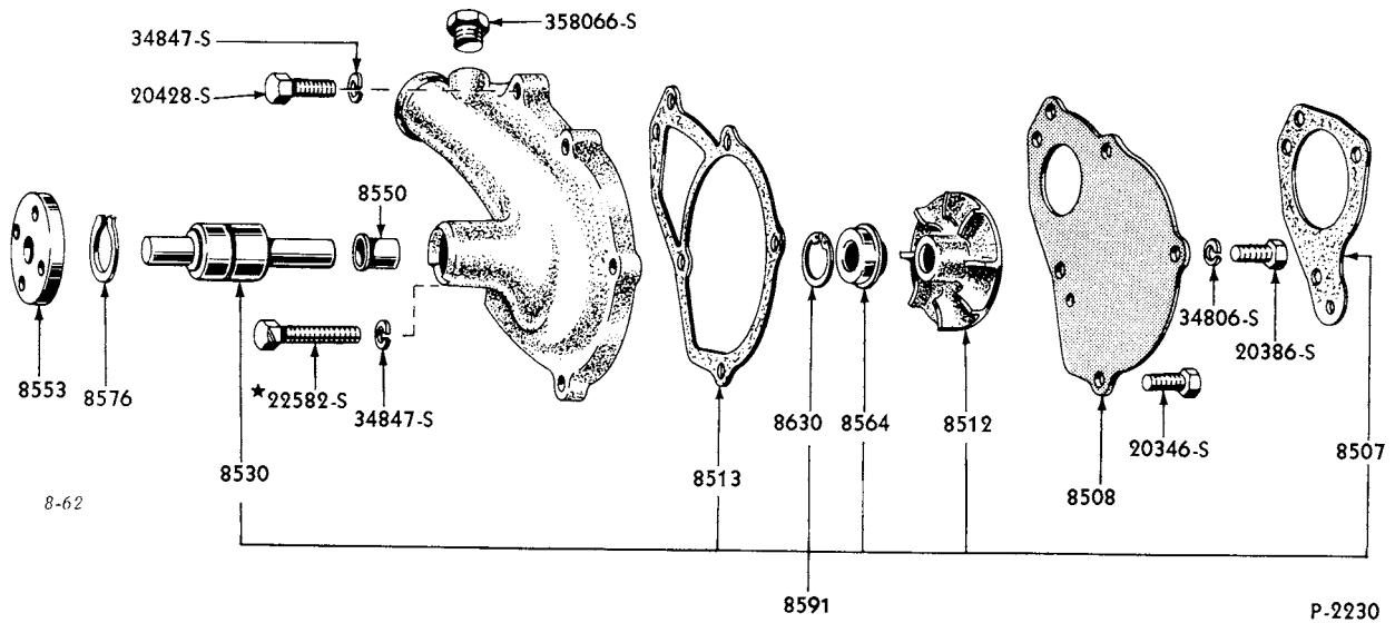
1957/ WATER PUMP (6 CYLINDER 223 ENGINE)-TYPICAL
