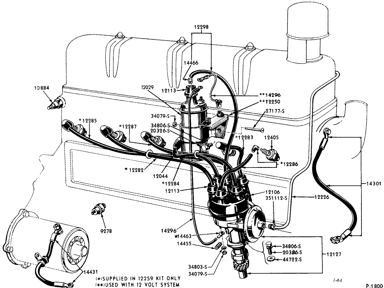
"TYPICAL" IGNITION WIRING (6 CYLINDER 223 ENGINE)
