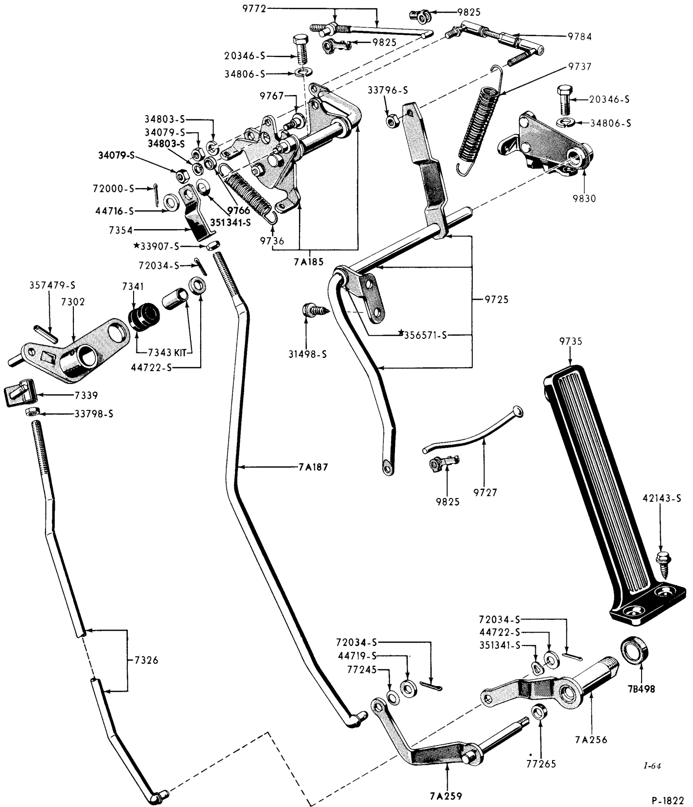
1955/56 "TYPICAL" ACCELERATOR LINKAGE (8 CYLINDER 272 ENGINE)-FORDOMATIC
