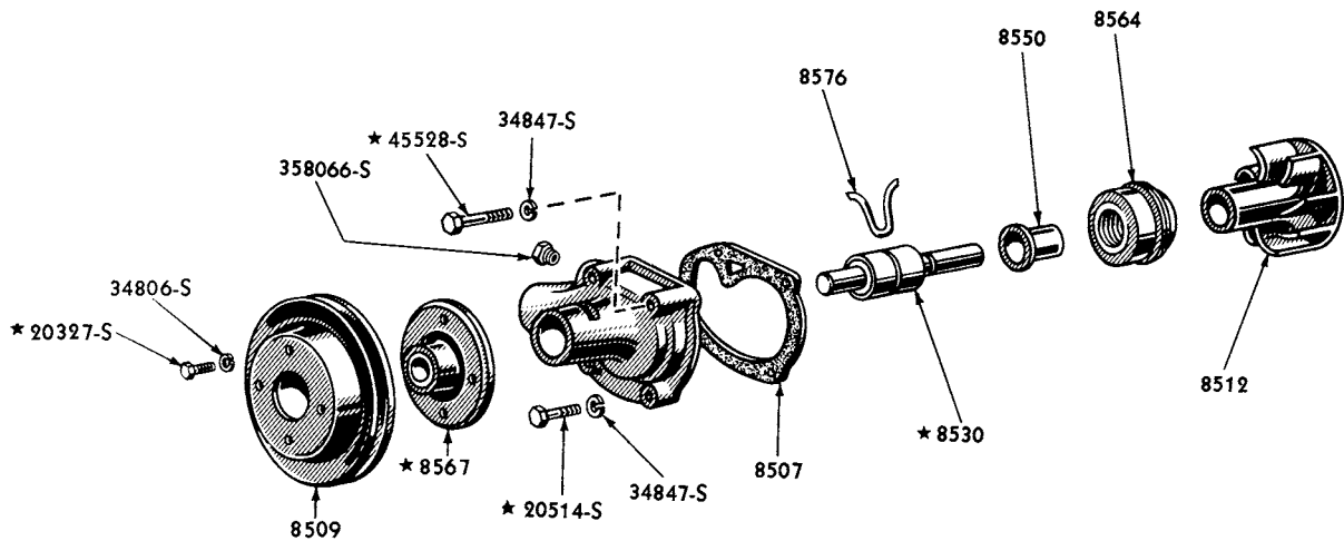
1949/51 WATER PUMP (6 CYLINDER 226 ENGINE)
