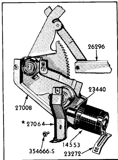
ELECTRIC REGULATOR
