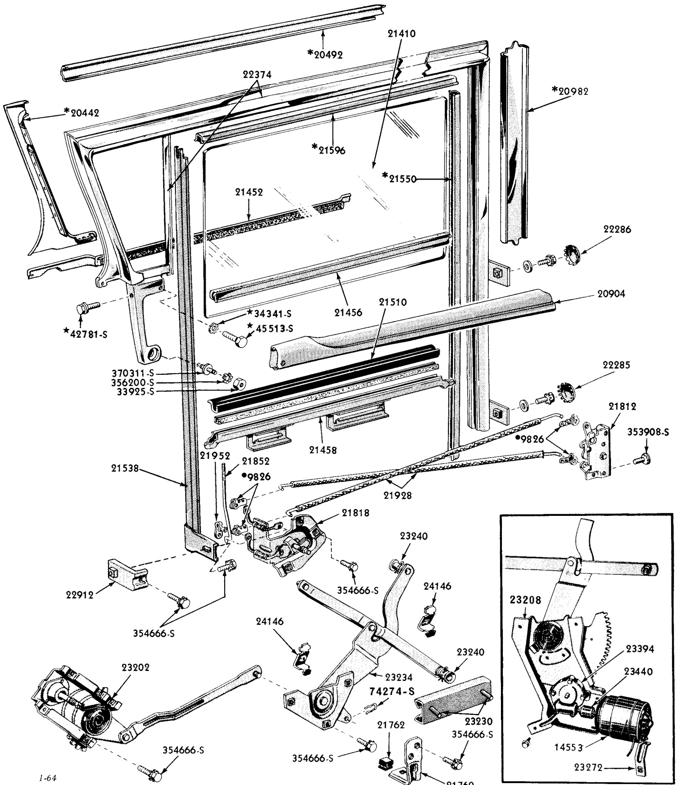
ELECTRIC REGULATOR
