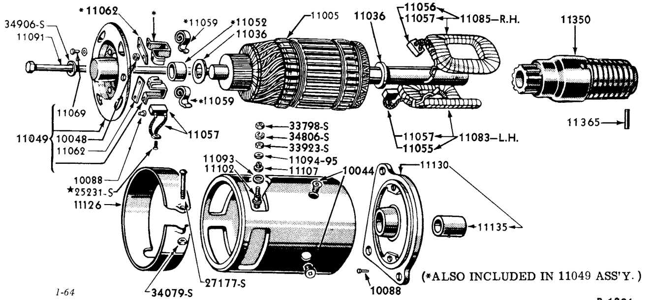
"TYPICAL" STARTER AND STARTER DRIVE (6 VOLT)
