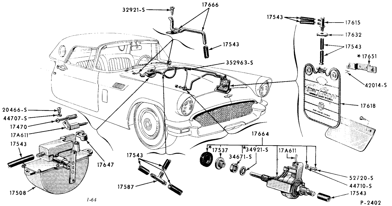
1957 WINDSHIELD WASHER (THUNDERBIRD)
