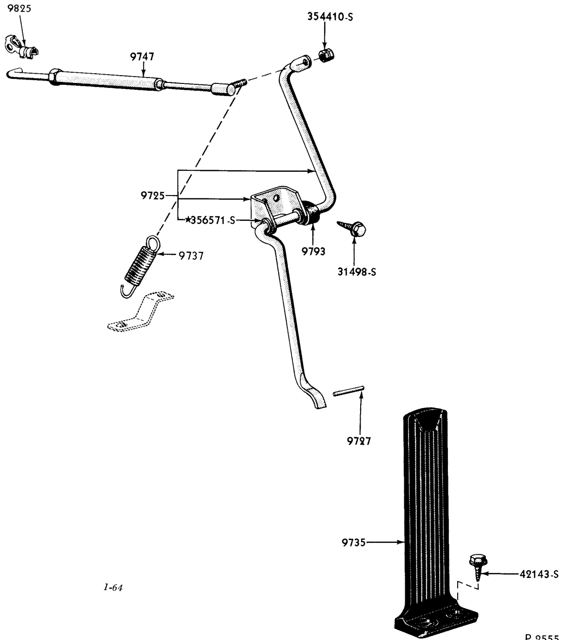
1958/59 ACCELERATOR LINKAGE (8 CYLINDER 332 & 352 ENGINES)-STANDARD & OVERDRIVE TRANSMISSION - (FORD)
