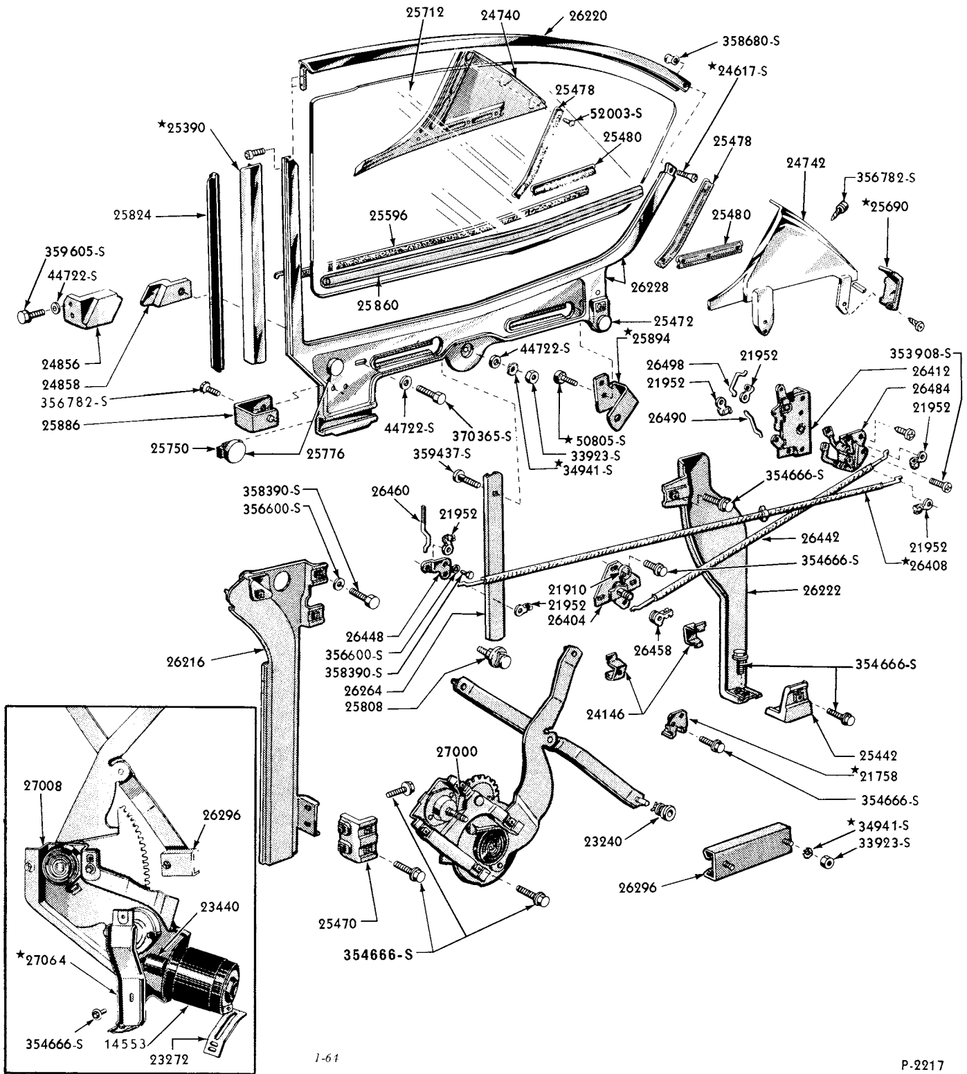
ELECTRIC REGULATOR
