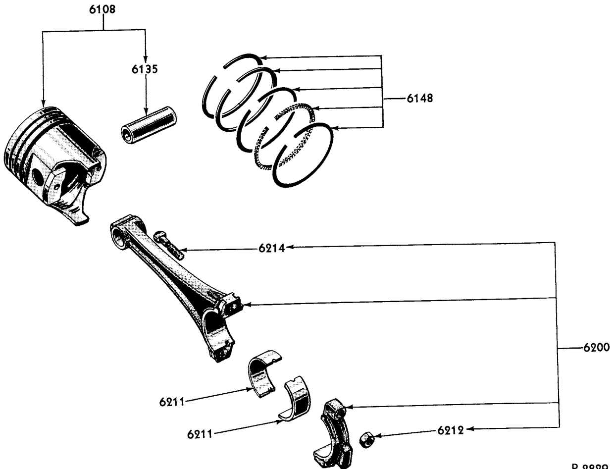
1959/ PISTON AND CONNECTING ROD (THUNDERBIRD-8 CYLINDER 430 ENGINE)-TYPICAL
