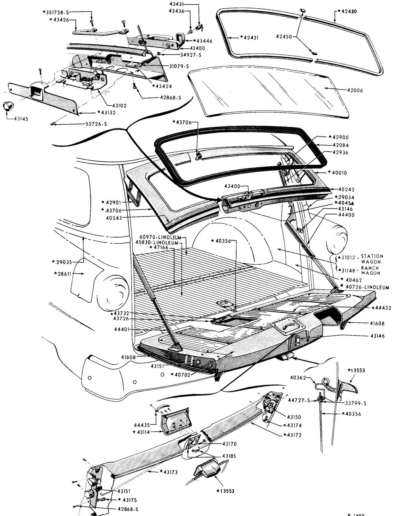
1953/54 STATION WAGON TAIL GATE & LIFT GATE WITH RELATED PARTS
