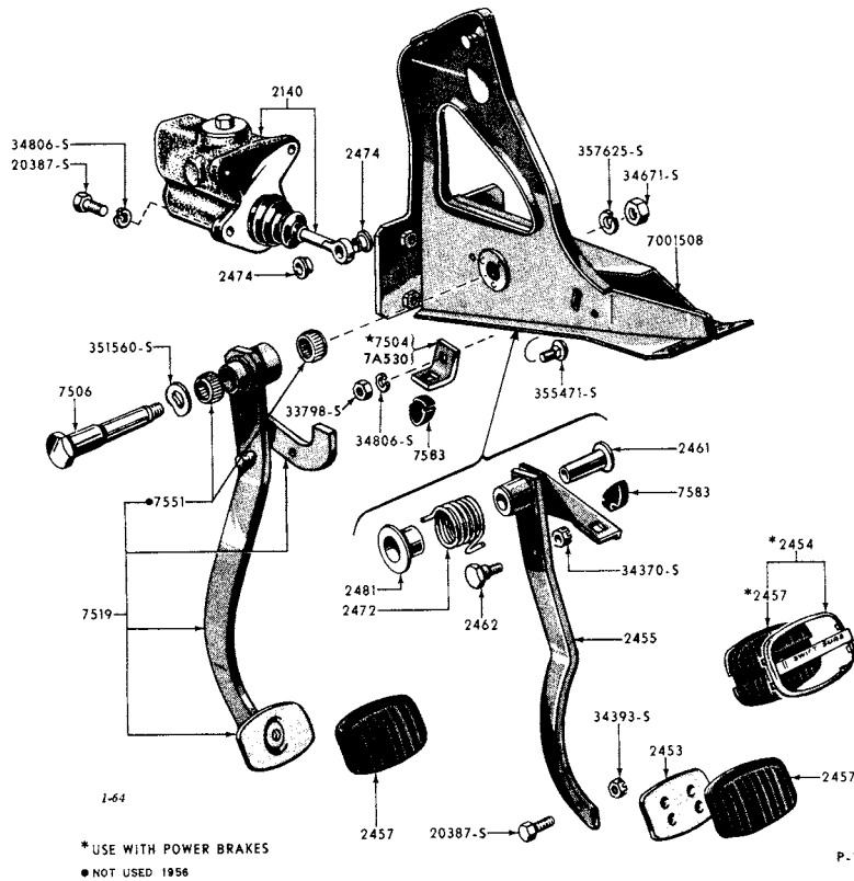
1955/56 BRAKE PEDAL AND RELATED PARTS(MANUAL GEAR SHIFT)(FORD)
