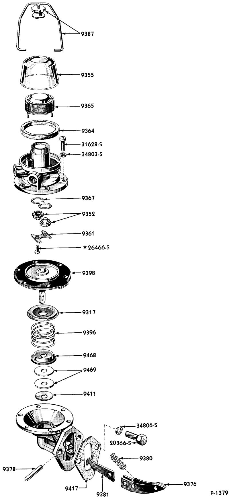
1952/54 FUEL PUMP (6 CYLINDER 215 AND 223 ENGINES) 1954 FUEL PUMP (8 CYLINDER 239 ENGINE)
