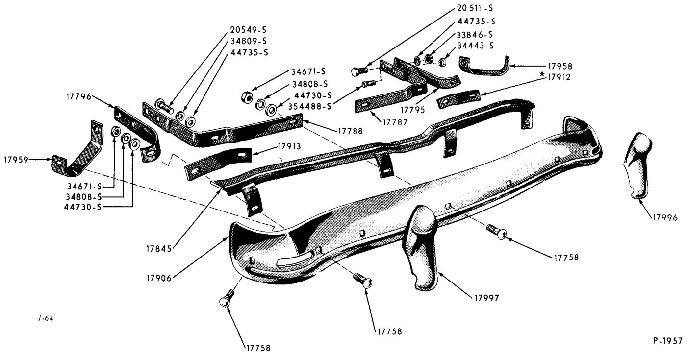
1955/56 REAR BUMPER (FORD)-TYPICAL
