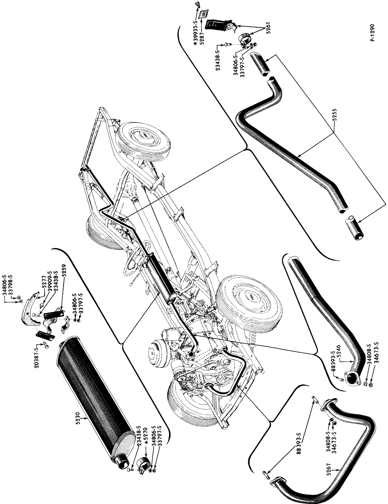
1952/53 EXHAUST SYSTEM (8 CYLINDER)
