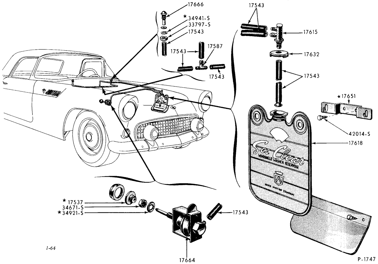
1955/56 WINDSHIELD WASHER (THUNDERBIRD)
