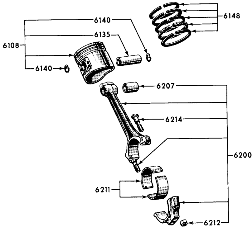
9-60 1958/ PISTON & CONNECTING ROD (8 CYLINDER 332, 352 ENGINES)-TYPICAL
