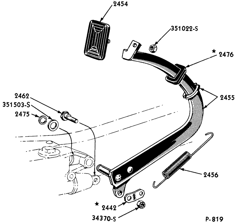
1949/51 BRAKE PEDAL AND RELATED PARTS
