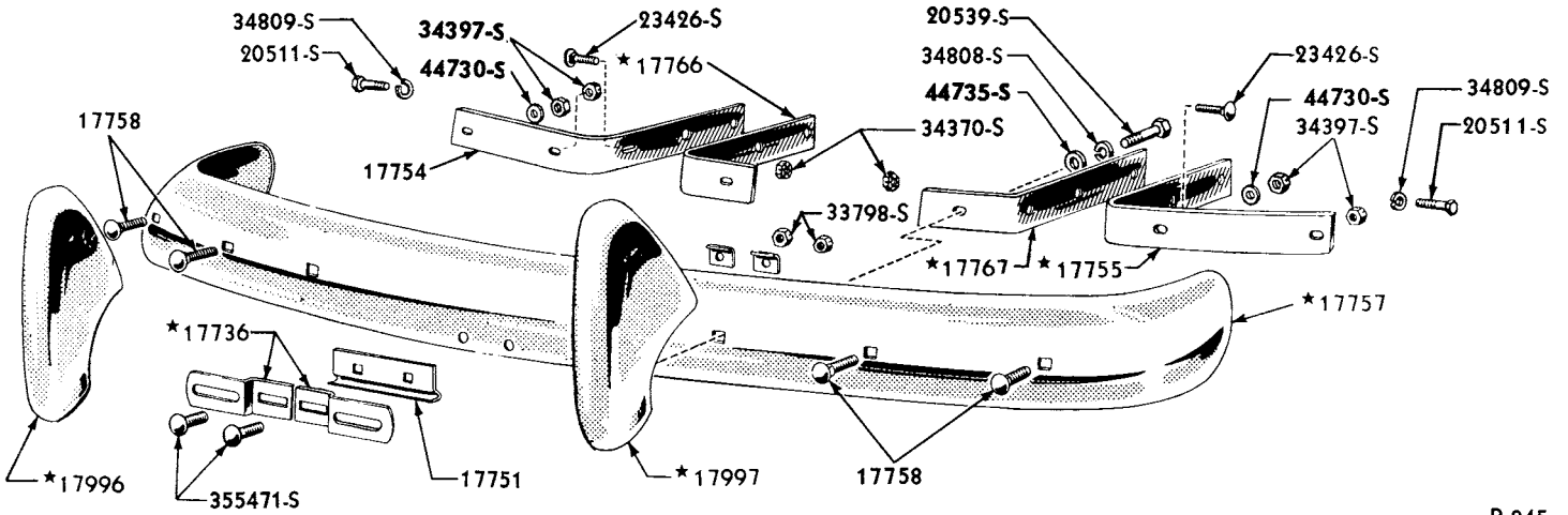
1949 FRONT BUMPER
