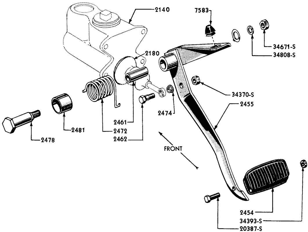
1952/54 BRAKE PEDAL AND RELATED PARTS (FORDOMATIC)
