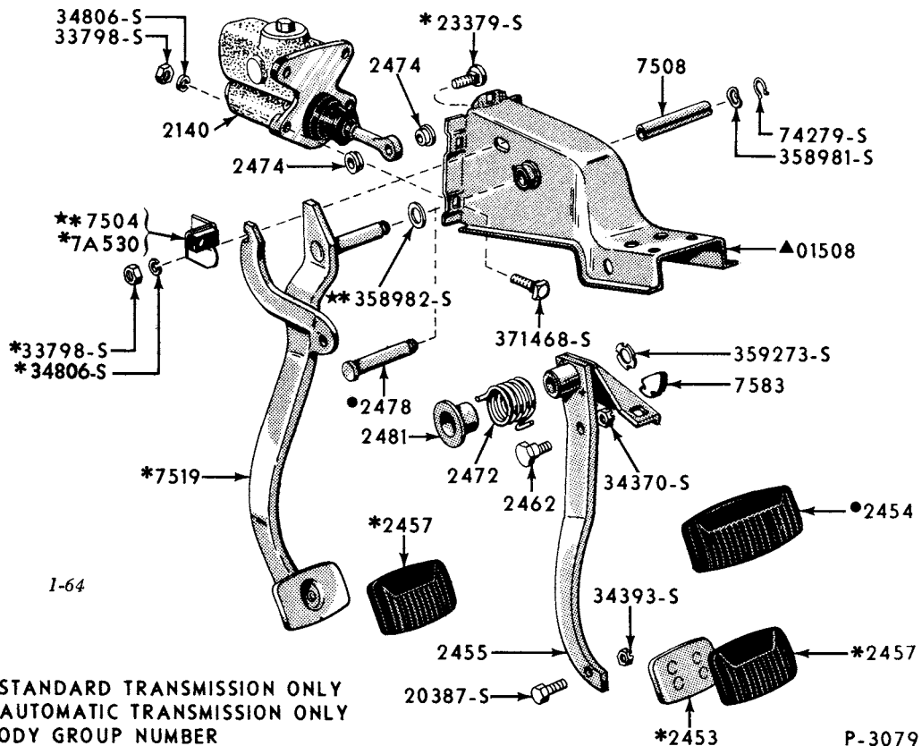
1958/ BRAKE & CLUTCH PEDALS (ALL TRANSMISSIONS)(THUNDERBIRD)
