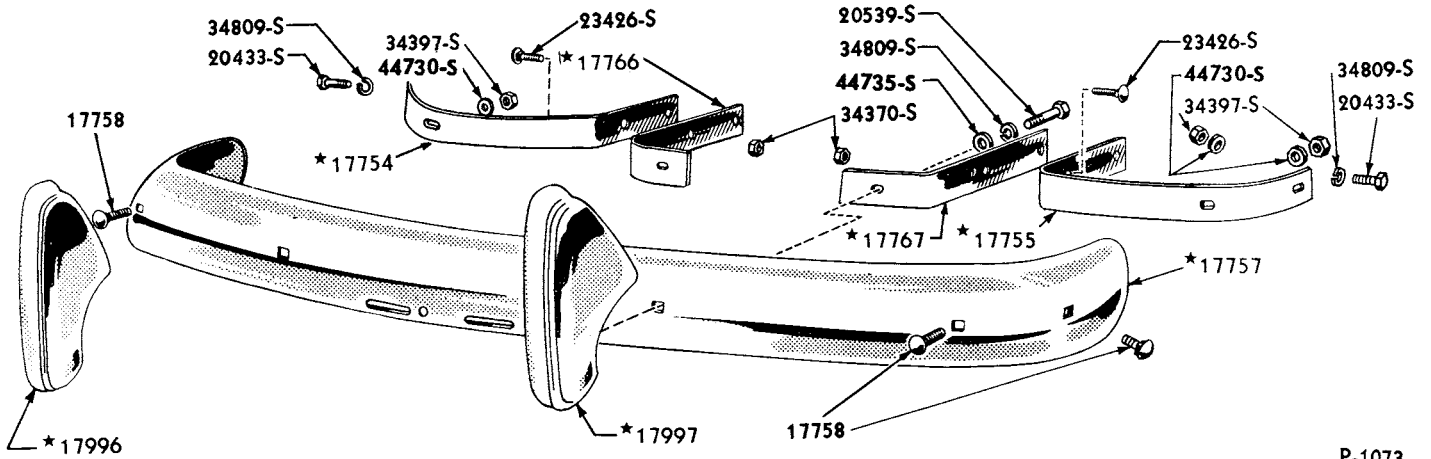
1950 FRONT BUMPER
