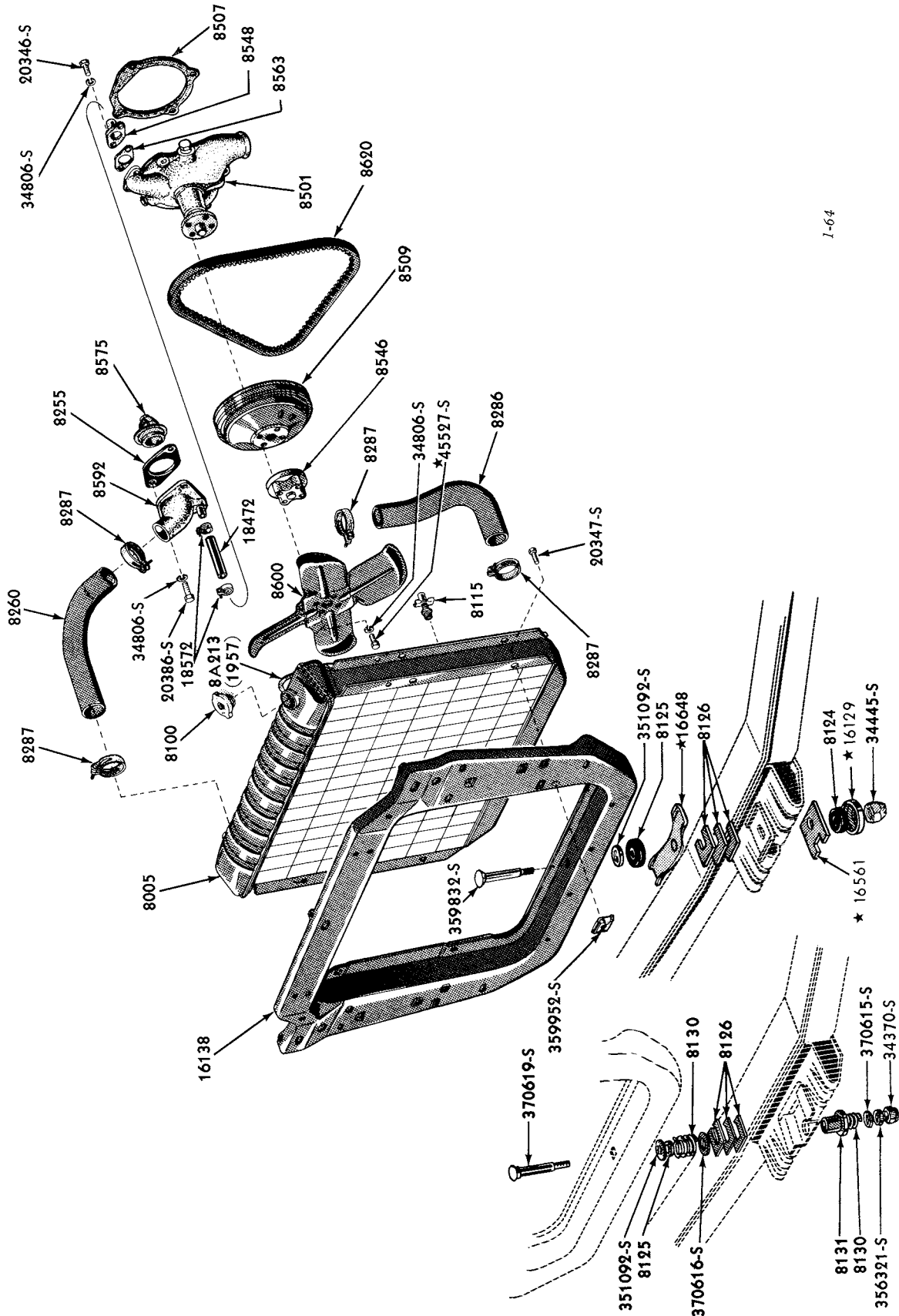
1954/57 "TYPICAL" COOLING SYSTEM (FORD)
