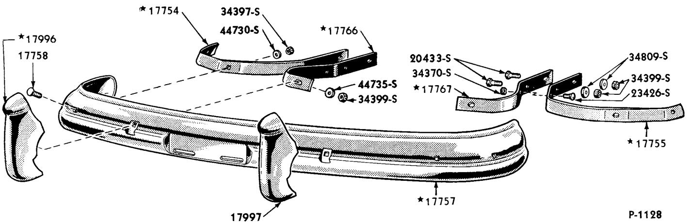
1951 FRONT BUMPER
