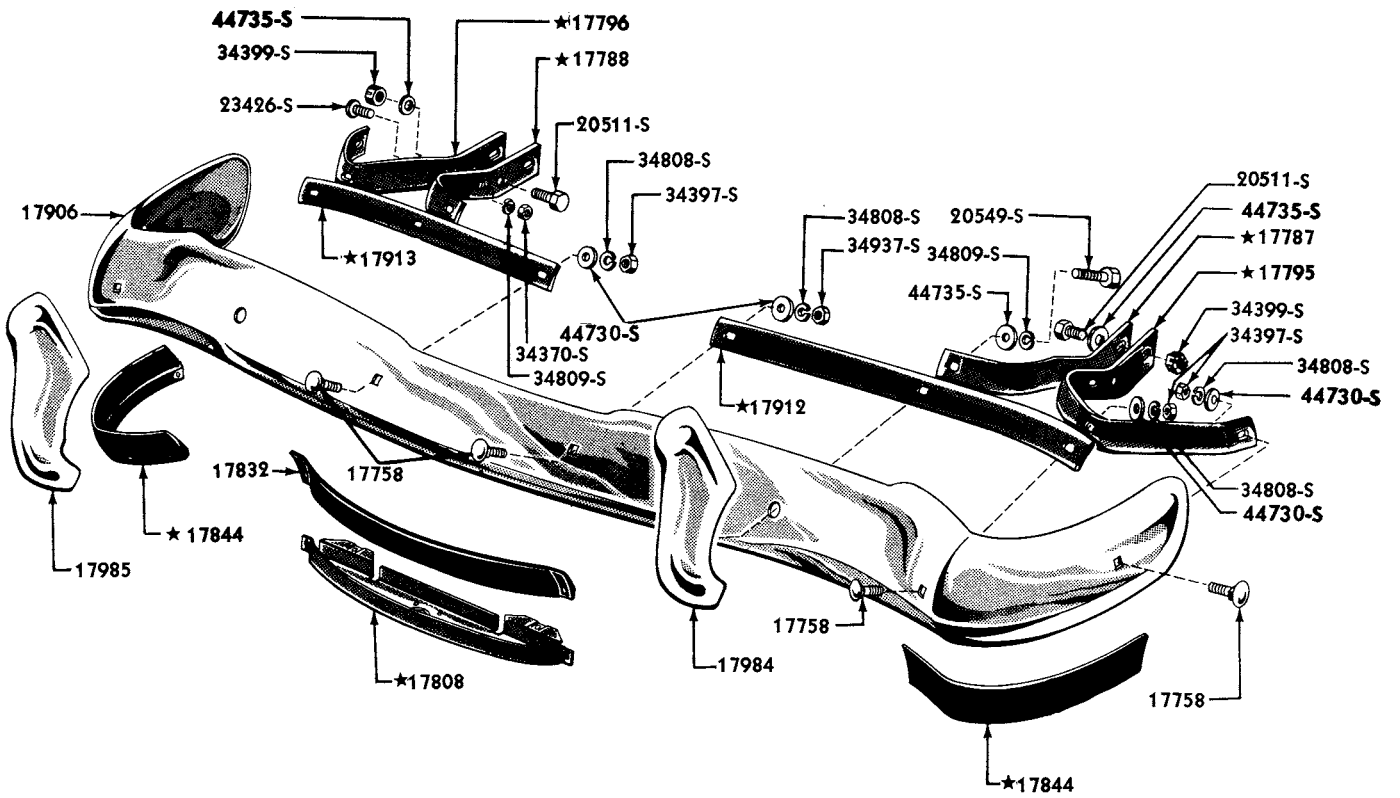
1952/54 REAR BUMPER
