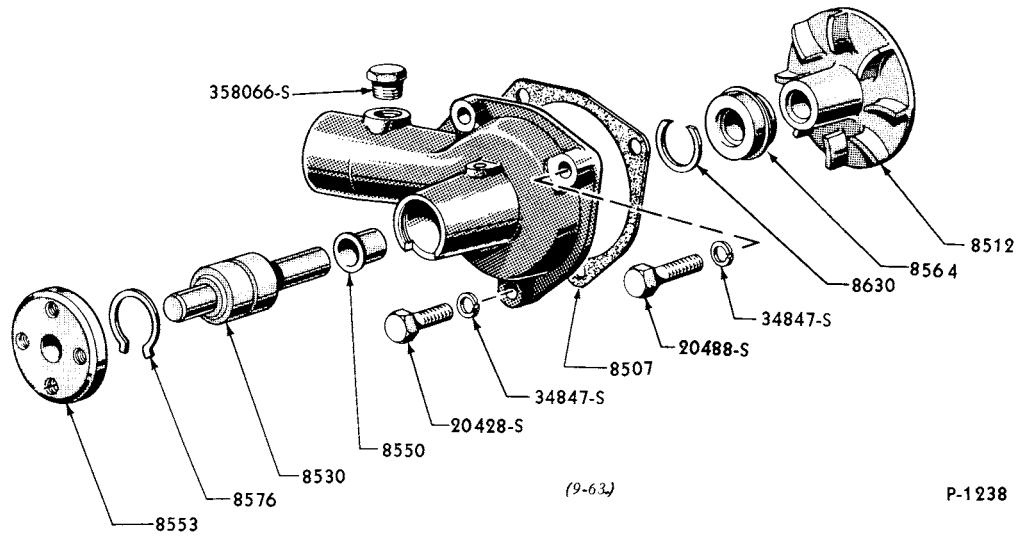
1952/56 WATER PUMP (6 CYLINDER 215 & 223 ENGINES)
