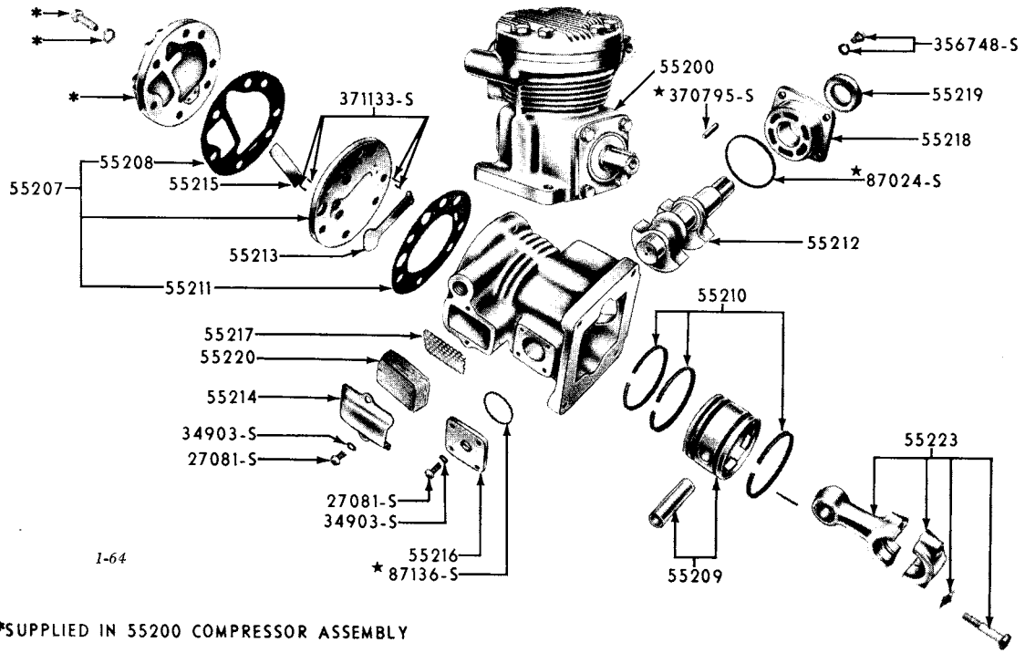
1958 AIR SUSPENSION COMPRESSOR
