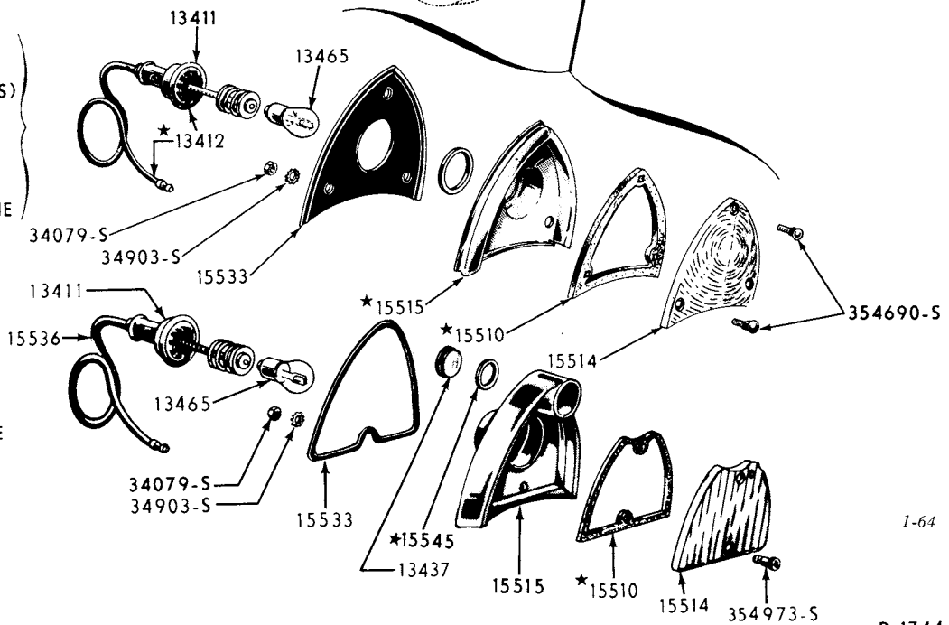
1955/56 BACK UP LAMP (FORD)
