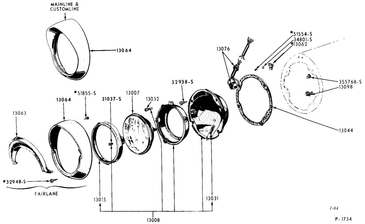
1955 HEADLAMP (FORD)
