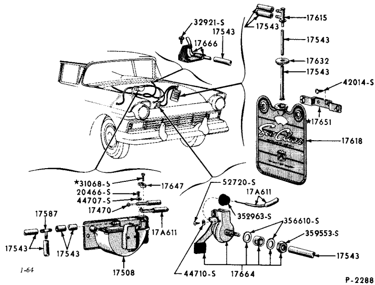
1957 WINDSHIELD WASHER (FORD)
