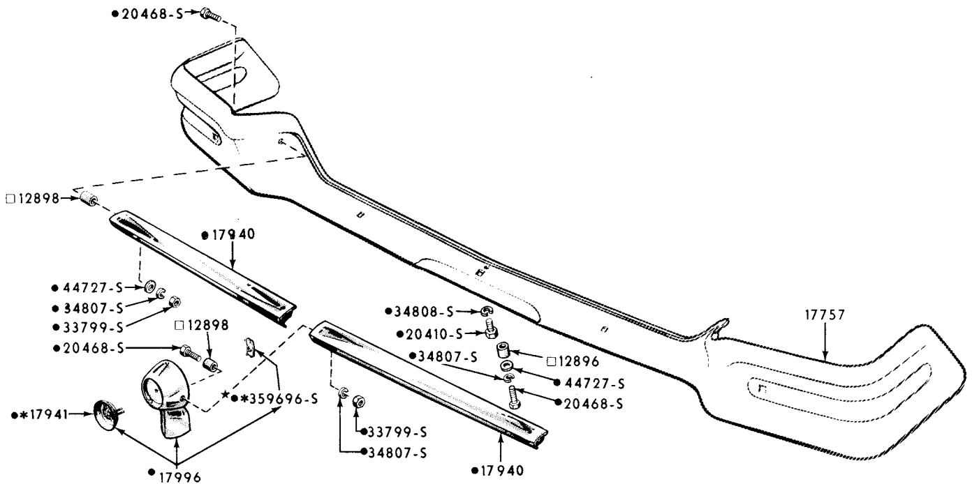
1958 FRONT BUMPER (FORD)
