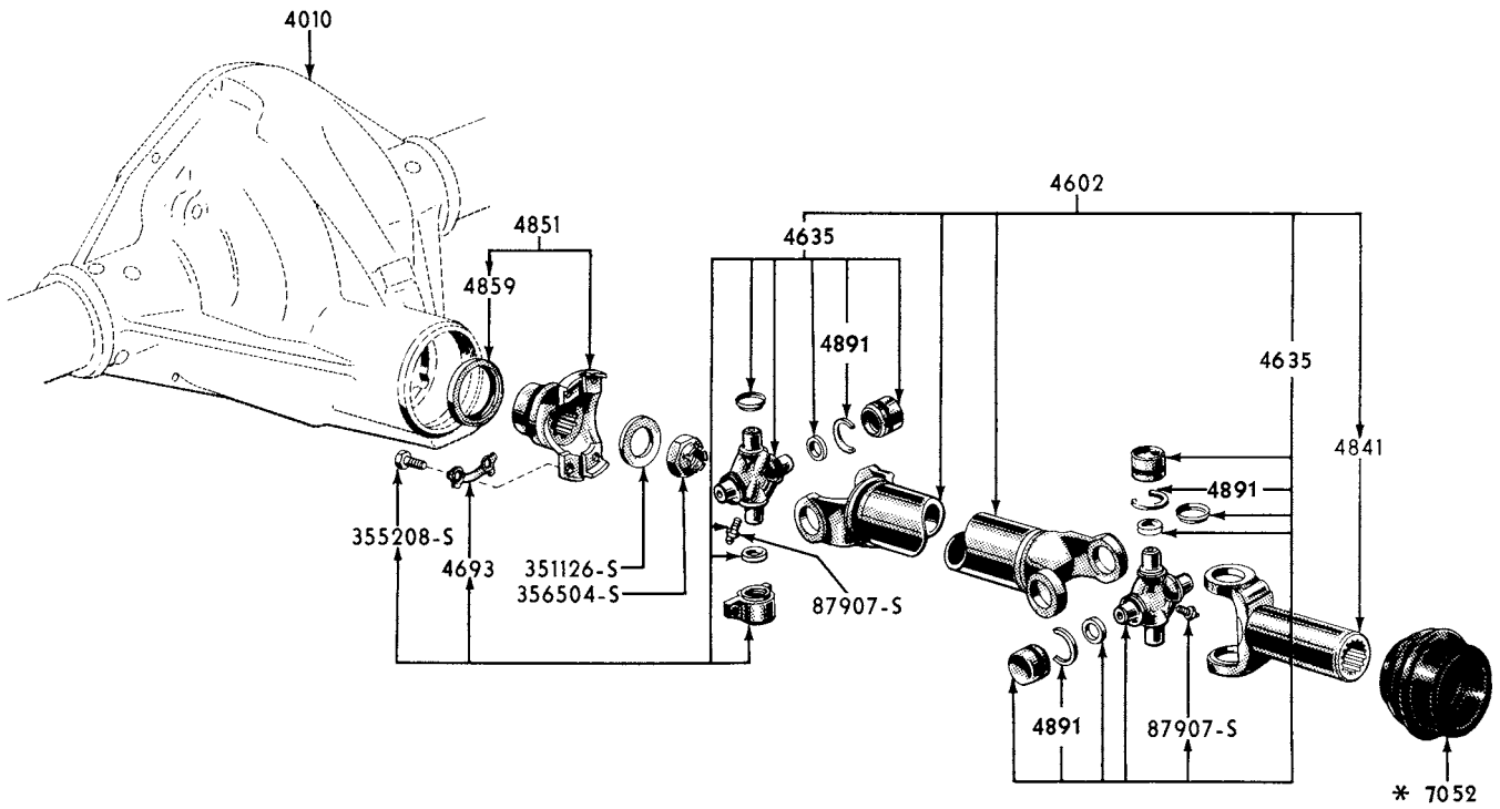
1951 DRIVE SHAFT
