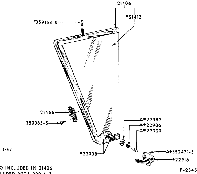
1957/58 DOOR VENT. WINDOW PARTS (BODY TYPES 58, 64)
