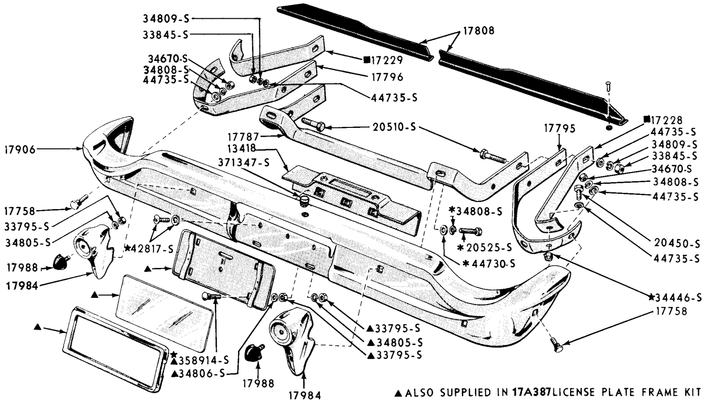
1959 REAR BUMPER (FORD)
