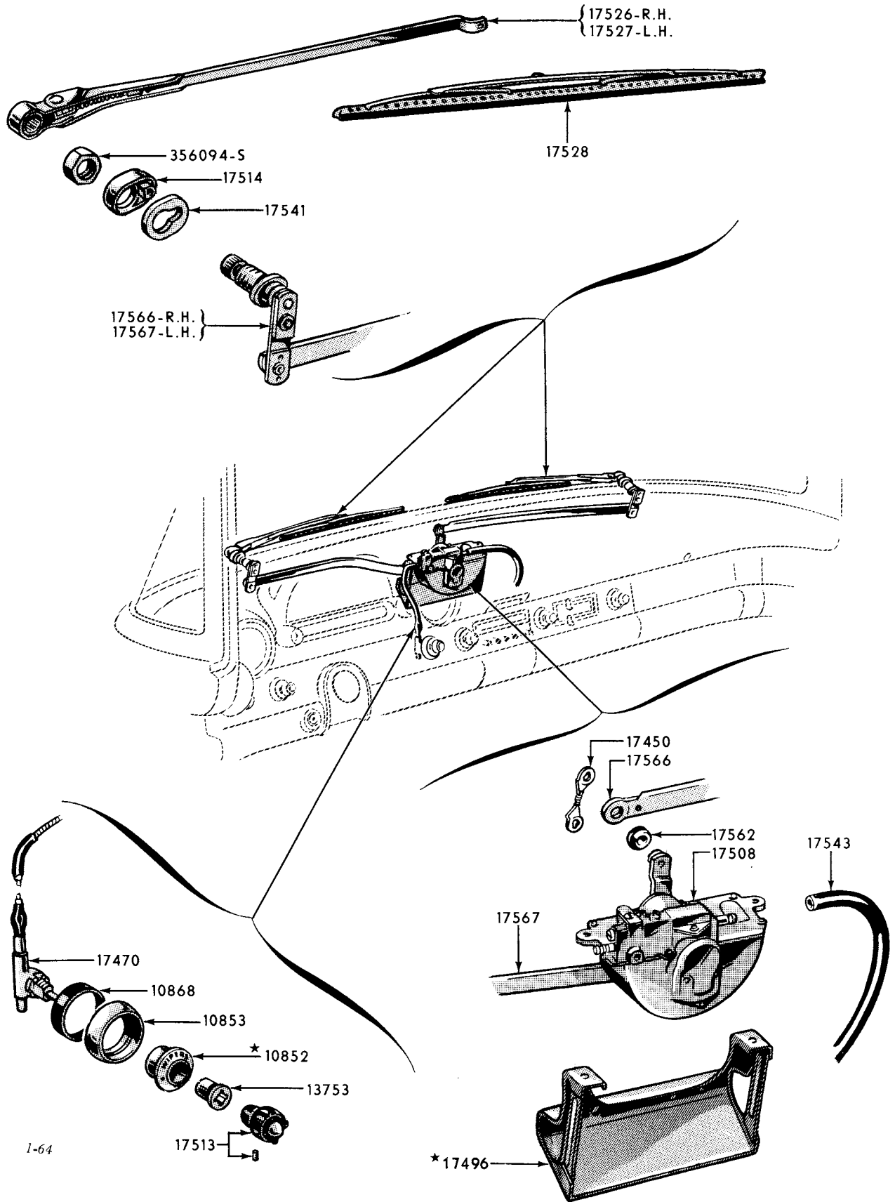
1955/57 "TYPICAL" WINDSHIELD WIPER (THUNDERBIRD)
