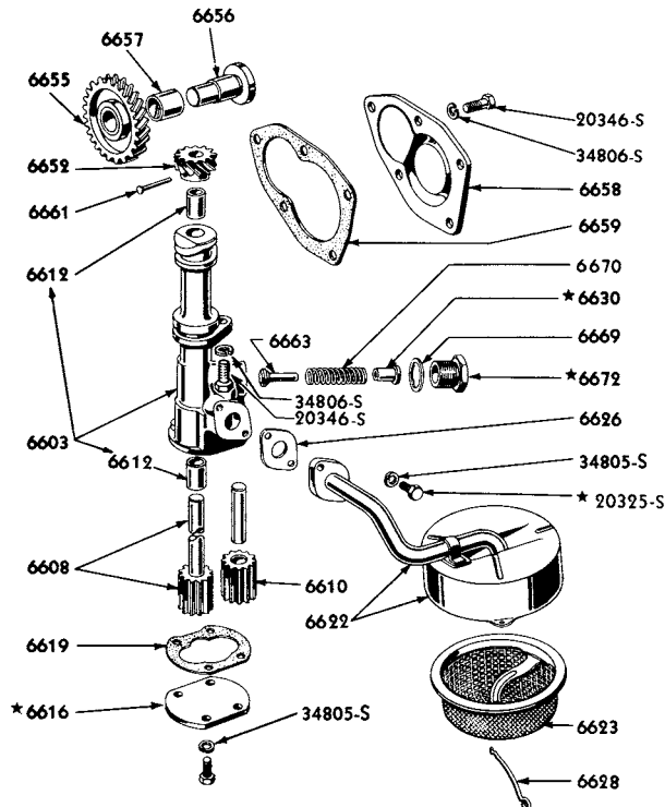
1949/51 OIL PUMP (6 CYLINDER 226 ENGINE)
