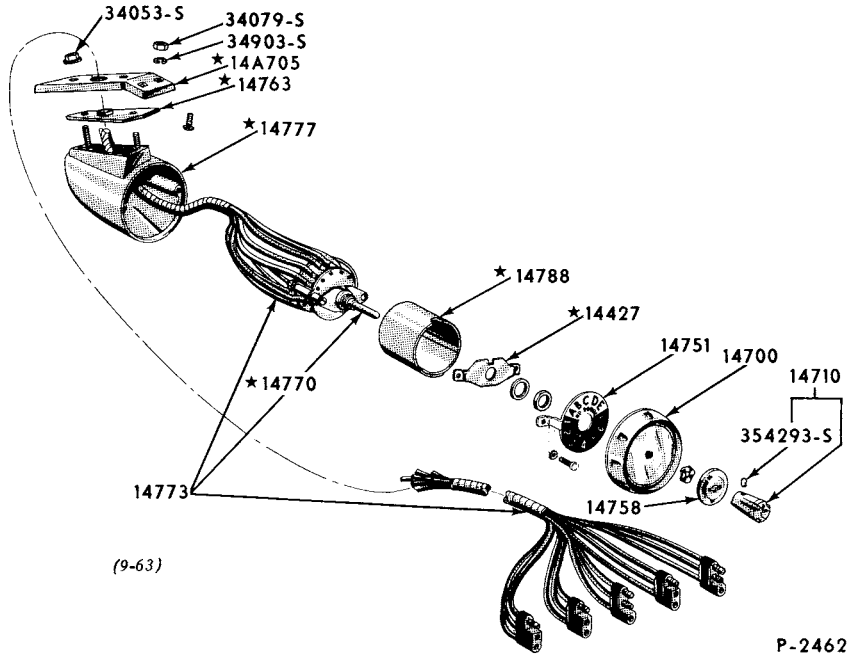
1957 THUNDERBIRD DIAL-O-MATIC SEAT REGULATOR CONTROL
