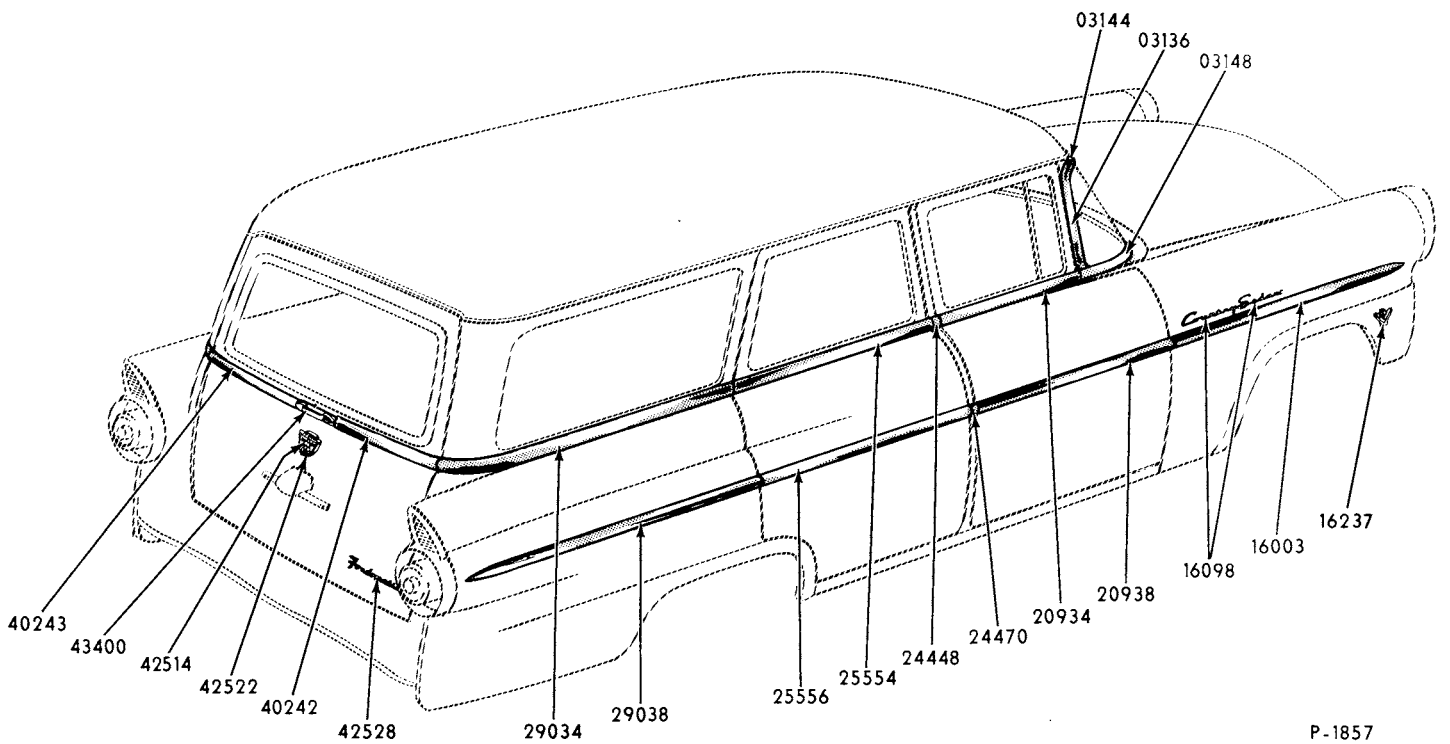
1955 CUSTOMLINE STATION WAGON "COUNTRY SEDAN"-(BODY TYPE 79B)
