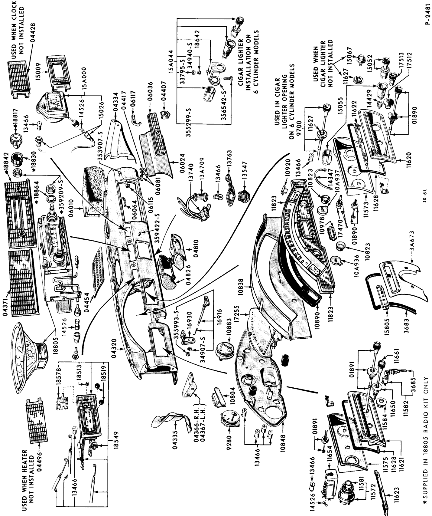
1958 INSTRUMENT PANEL AND RELATED PARTS (FORD)
