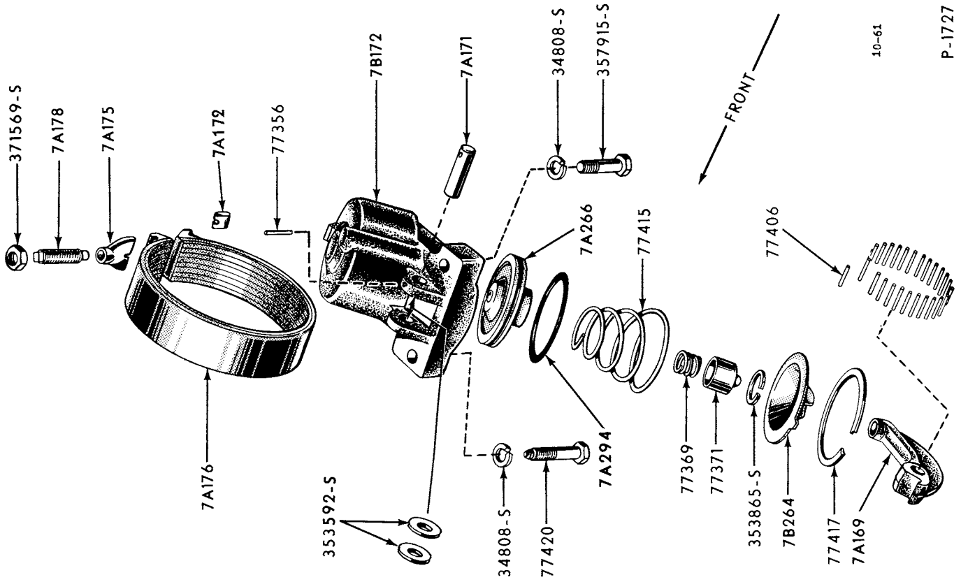
1955/57 "TYPICAL" REAR SERVO & BAND (FORDOMATIC TRANSMISSION)
