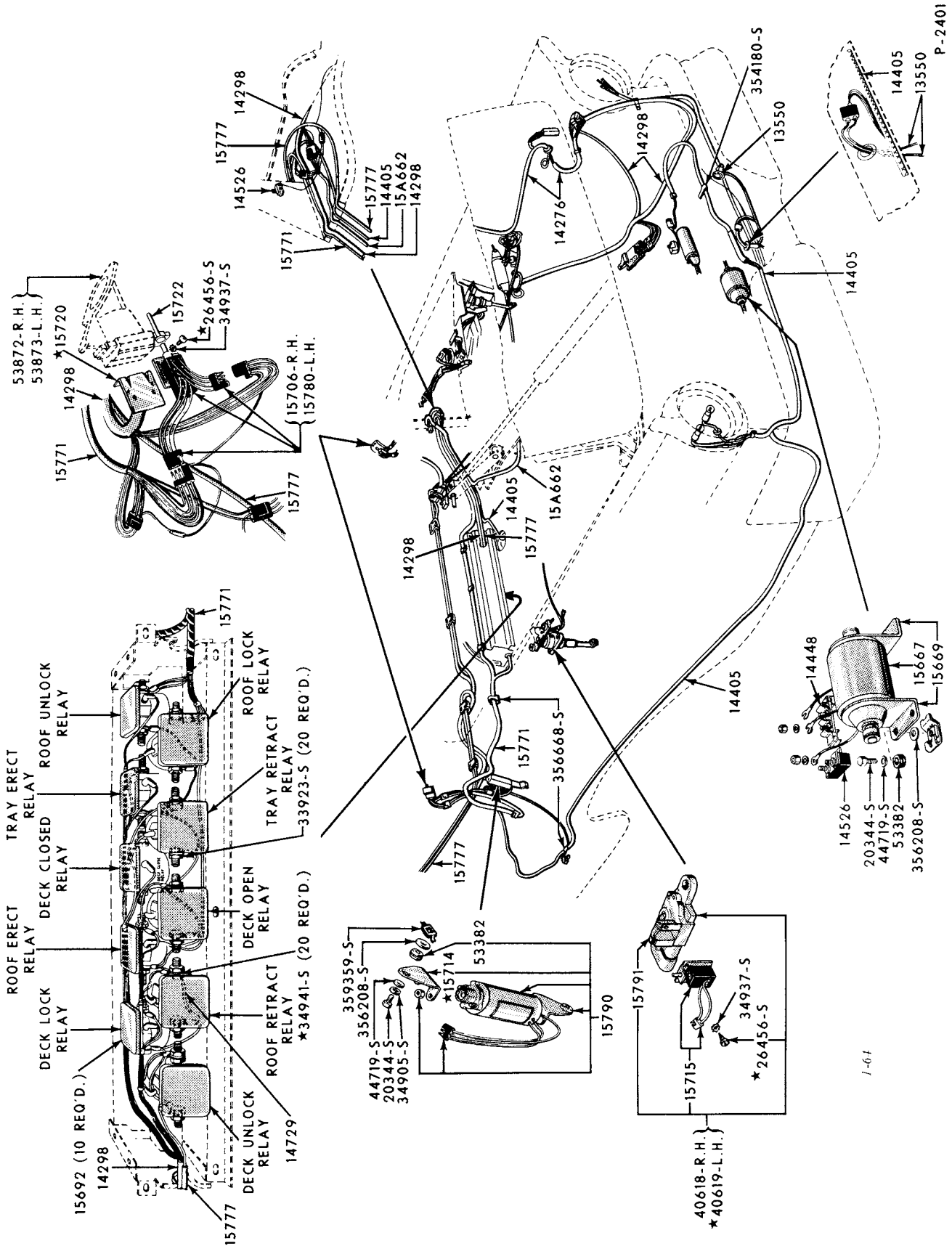
1957/59 ELECTRICAL SYSTEM (RETRACTABLE HARDTOP LUGGAGE COMPARTMENT WIRING, RELAYS, SWITCHES, MOTORS, ETC.)
