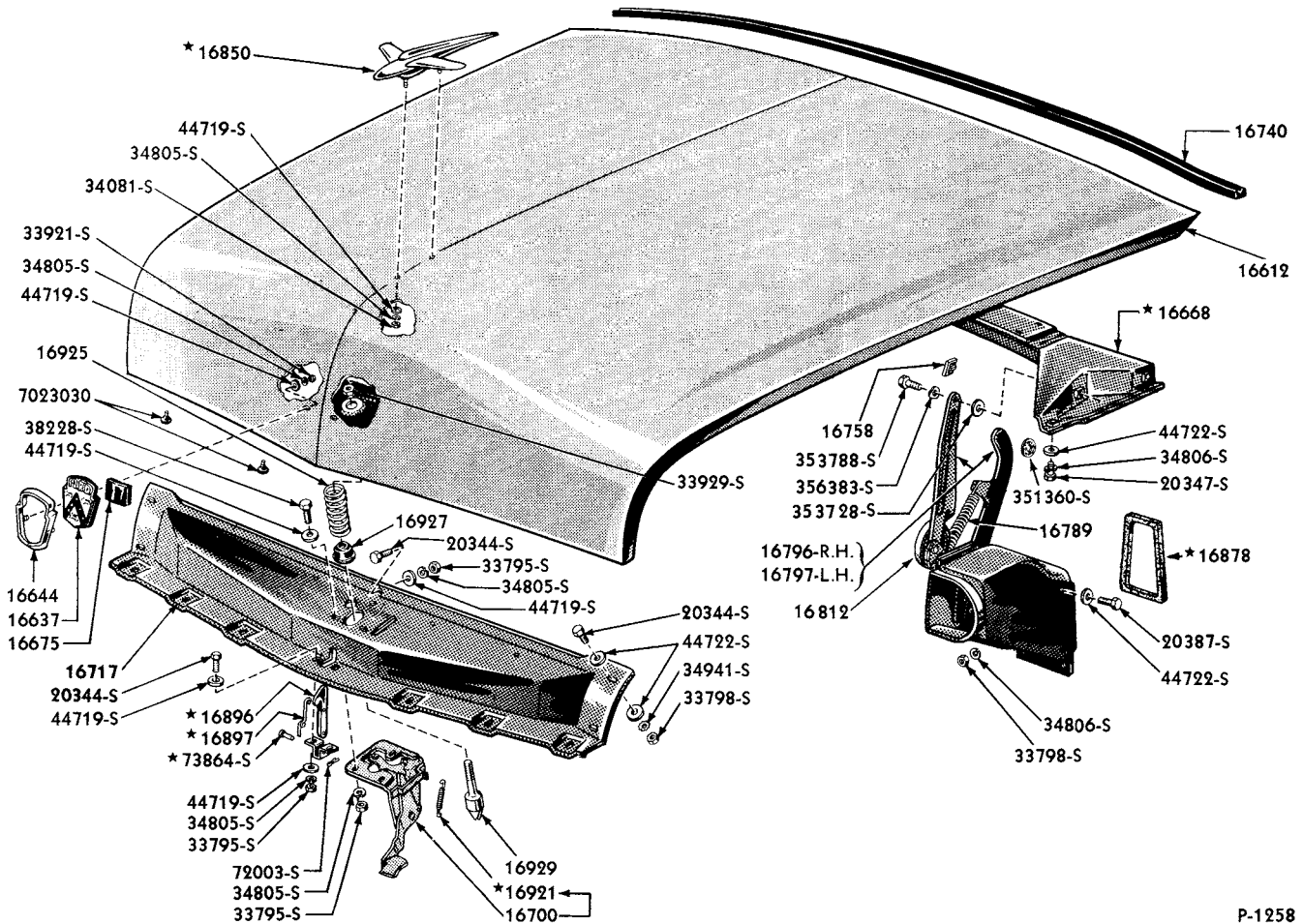
1952 HOOD AND RELATED PARTS
