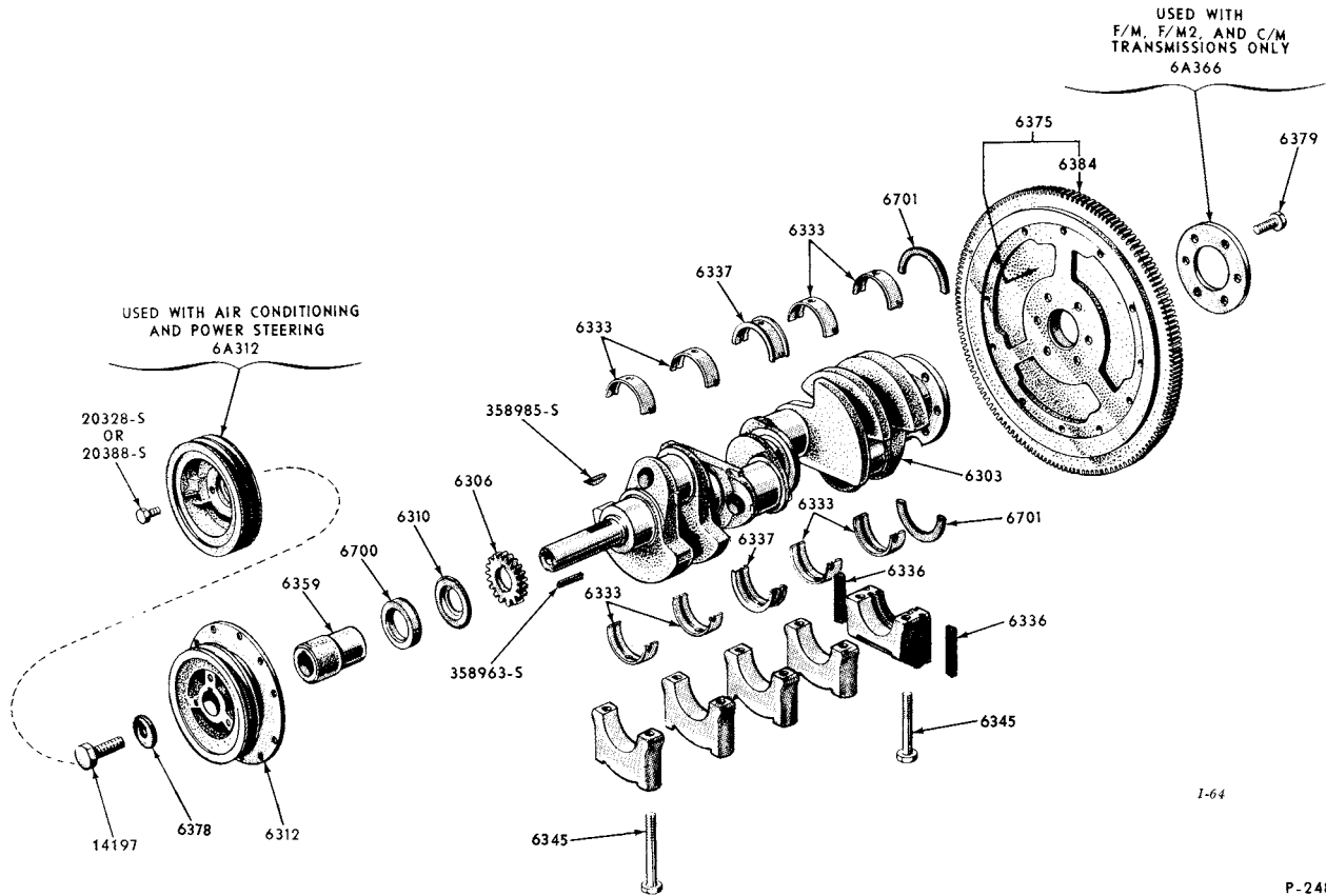
1958/ CRANKSHAFT, FLYWHEEL & RELATED PARTS (8 CYLINDER 332, 352 ENGINES)-TYPICAL
