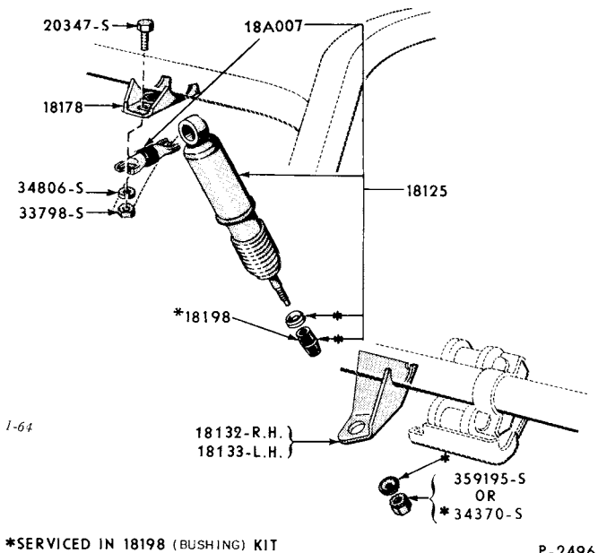
REAR (MODELS 51, 59, 79)
