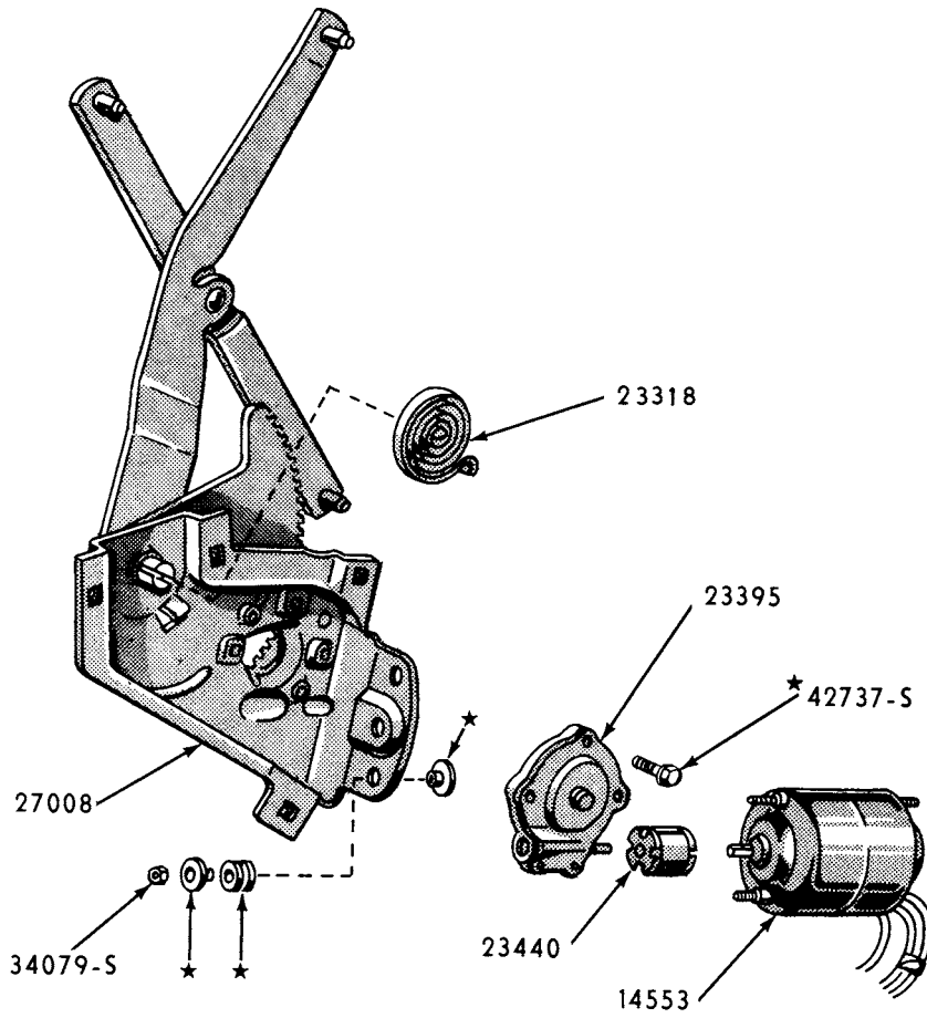
1954 REAR DOOR & QUARTER POWER-LIFT WINDOW REGULATOR
