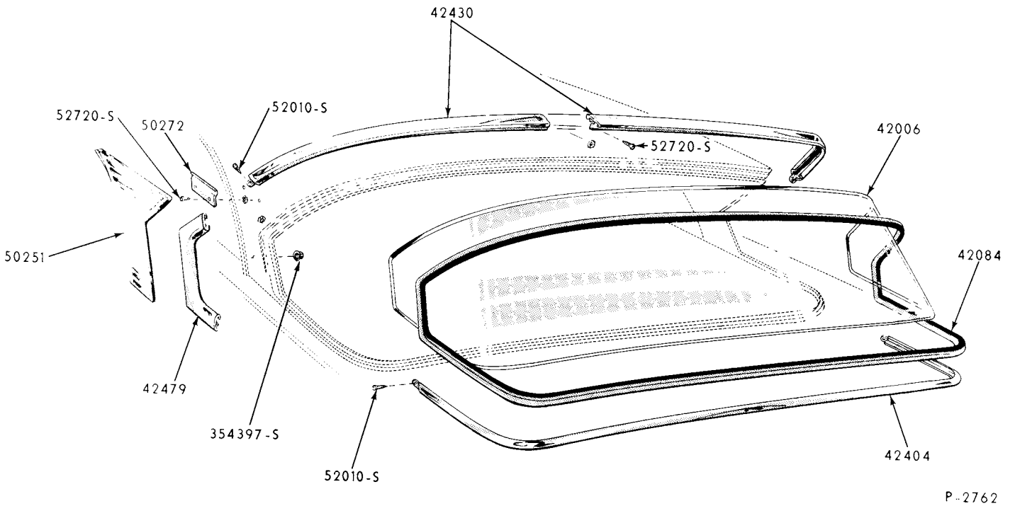
1957/59 BACK WINDOW & RELATED PARTS (BODY TYPE 66)
