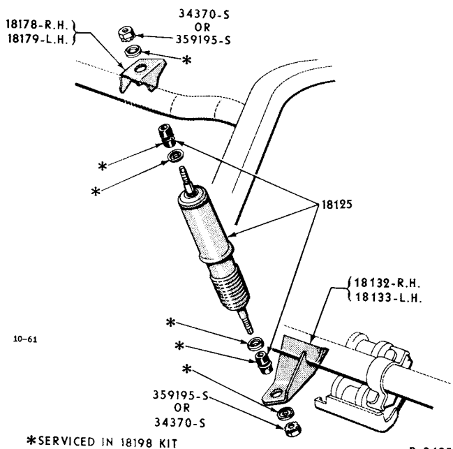
REAR (MODELS 57, 58, 63, 64, 76)
