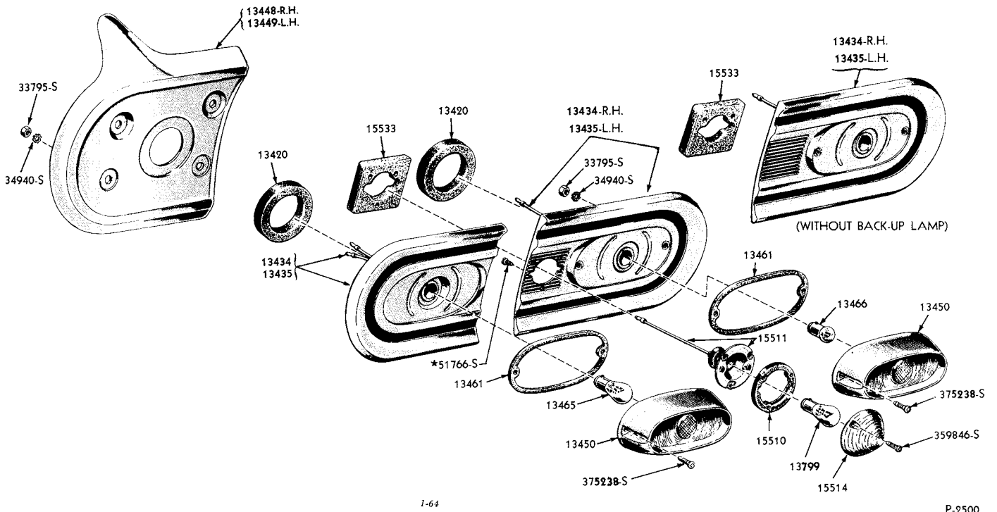
1958 REAR LAMP & BACK-UP LAMP (STATION WAGON)
