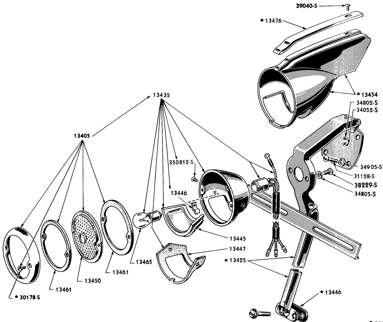
1949/51 REAR LAMP (STATION WAGON)
