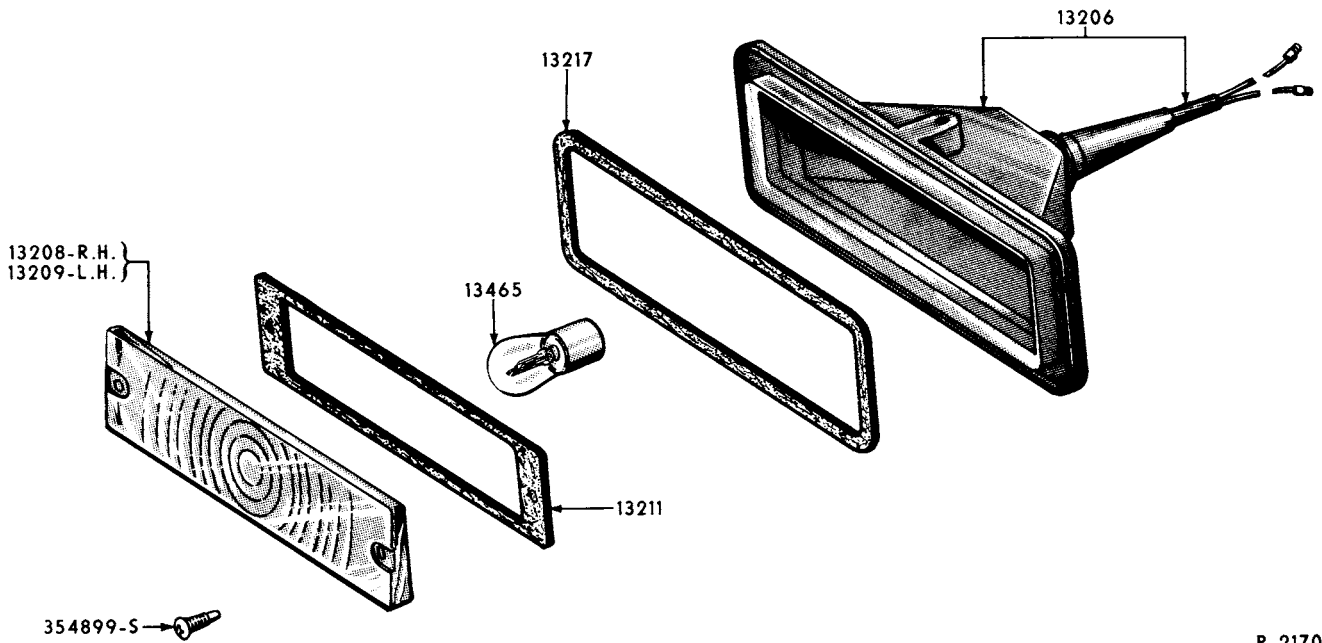
1957 PARKING LAMP (THUNDERBIRD)
