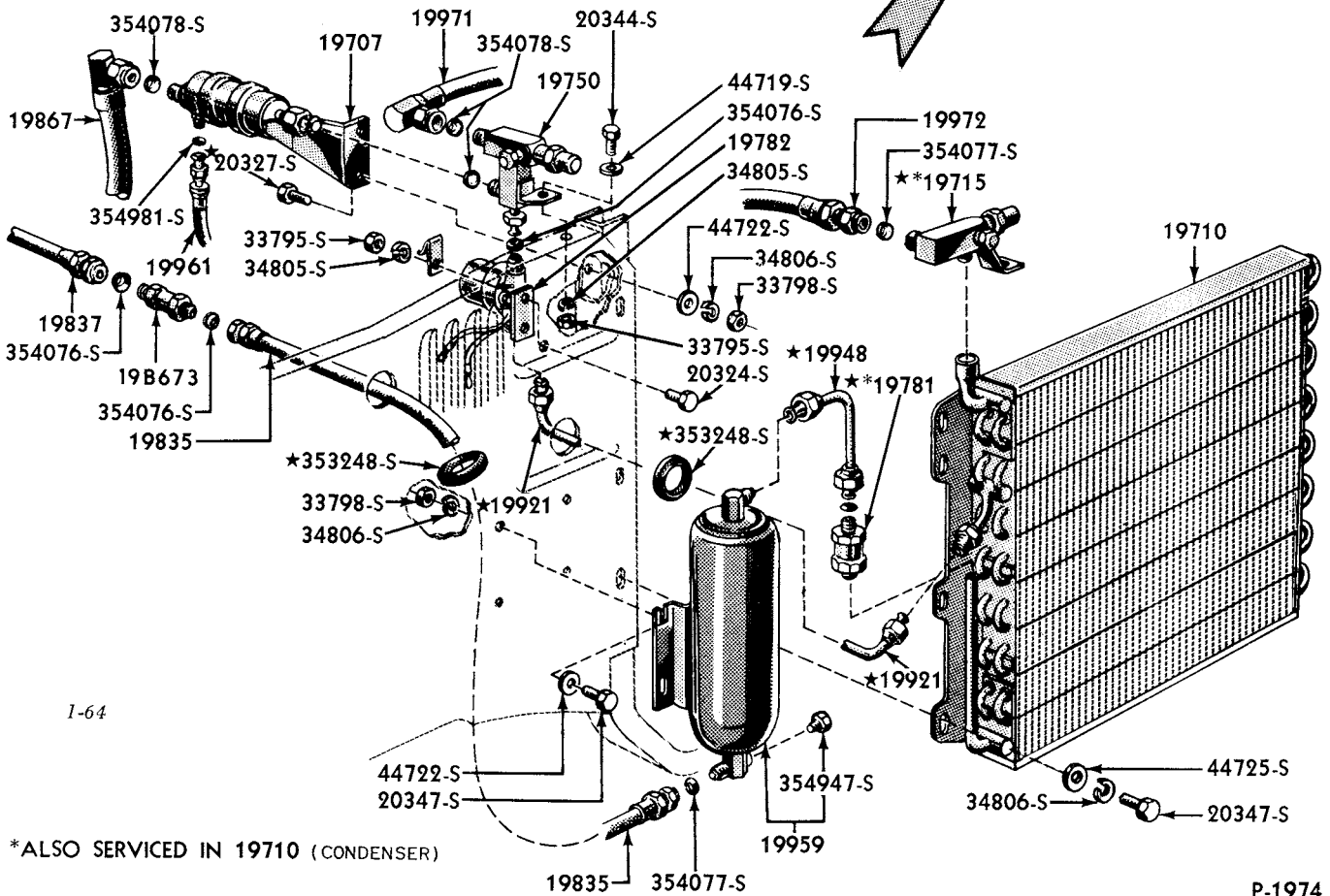
1956 FORD SELECT AIRE CONDITIONER CONDENSER, DEHYDRATOR & RELATED PARTS
