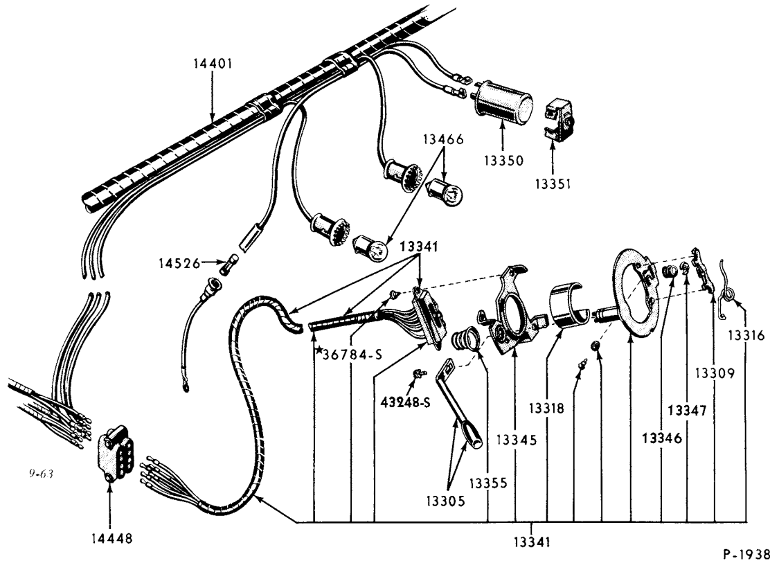
1956/58 TURN INDICATOR (FORD)
