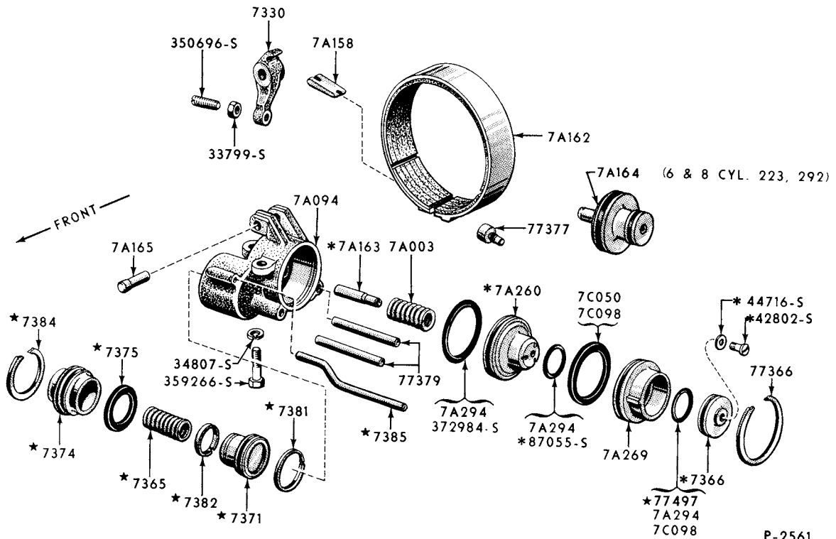
1956/59 8 CYLINDER 312, 332, 352 FRONT SERVO & BAND (FORDOMATIC TRANSMISSION)-TYPICAL
