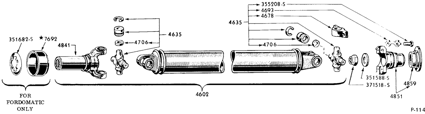
1951 DRIVE SHAFT
