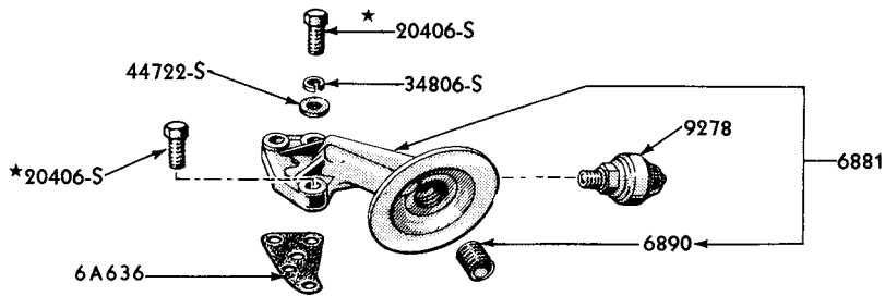
1958/ OIL PUMP & RELATED PARTS (8 CYLINDER 332, 352 ENGINES)-TYPICAL
