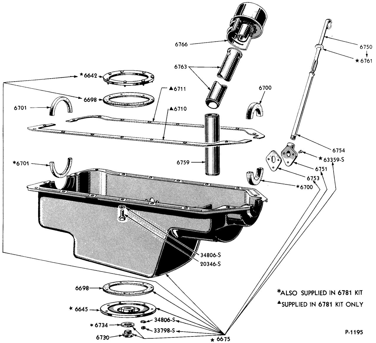
1949/53 OIL PAN AND RELATED PARTS (8 CYLINDER 239 "L" HEAD ENGINE)
