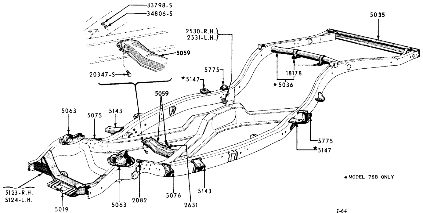
"X" TYPE 1957/59 FRAME (FORD)
