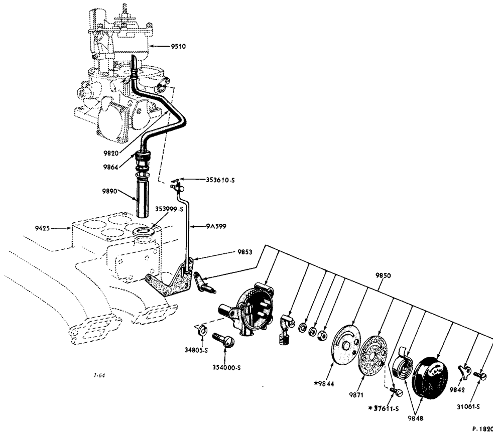
1955 THERMOSTATIC CHOKE AND RELATED PARTS (8 CYLINDER ENGINE)
