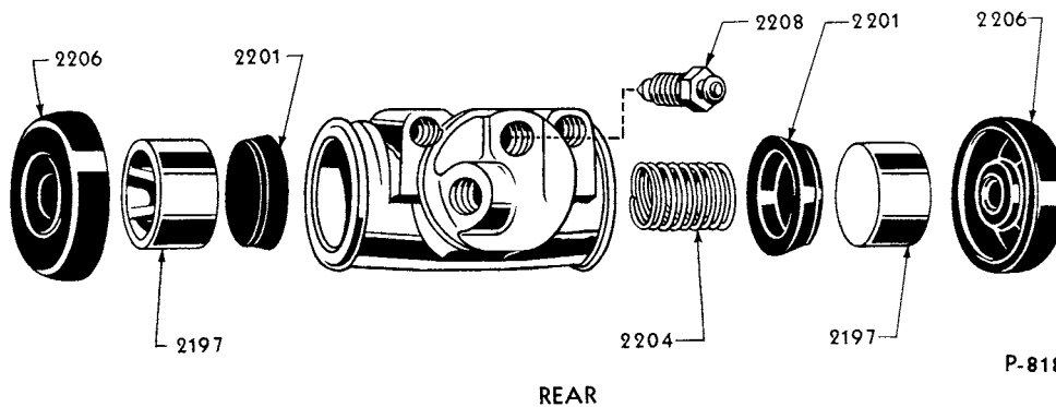
1949/56 FRONT & REAR BRAKE CYLINDERS
