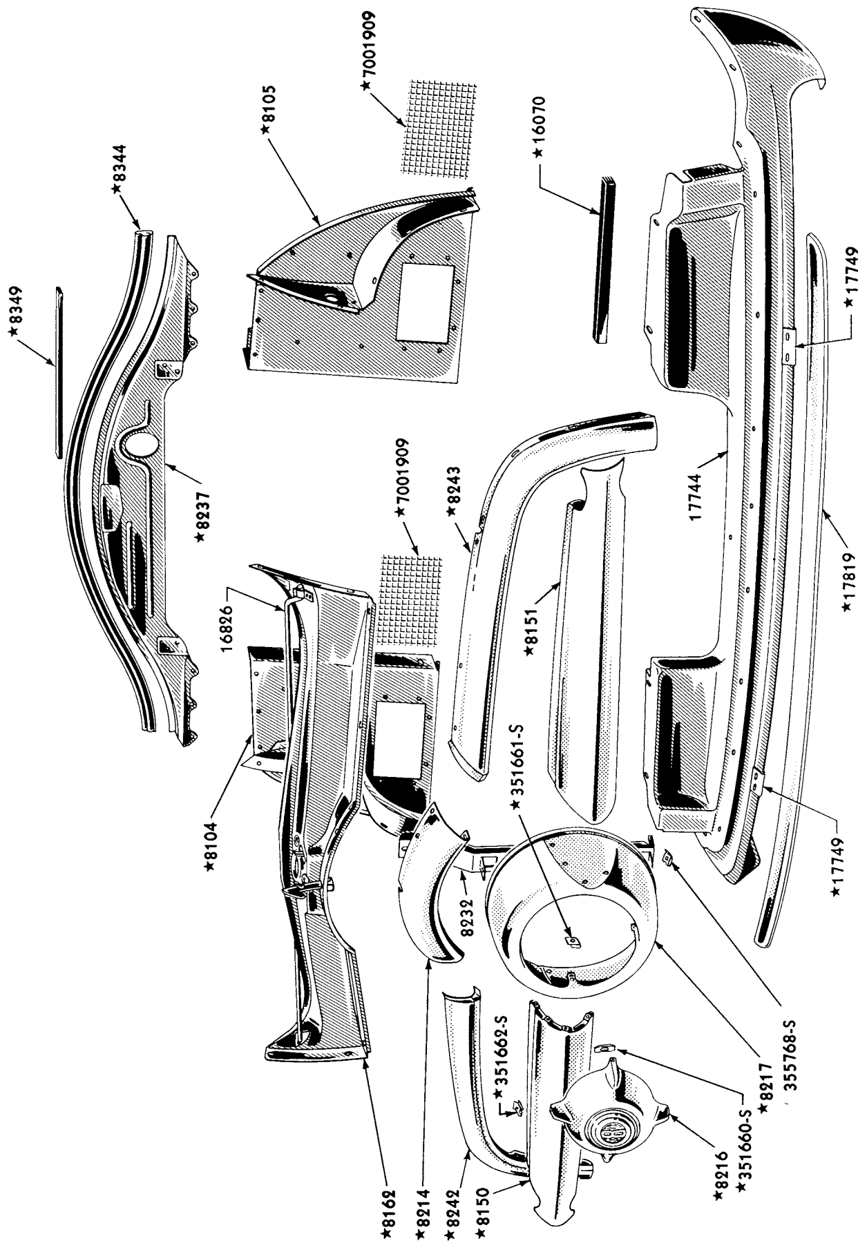
1949 RADIATOR GRILLE AND RELATED PARTS
