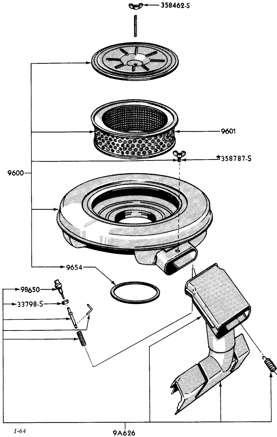
1959/ "TYPICAL" CARBURETOR AIR CLEANER & RELATED PARTS (THUNDERBIRD 430 ENGINE)
