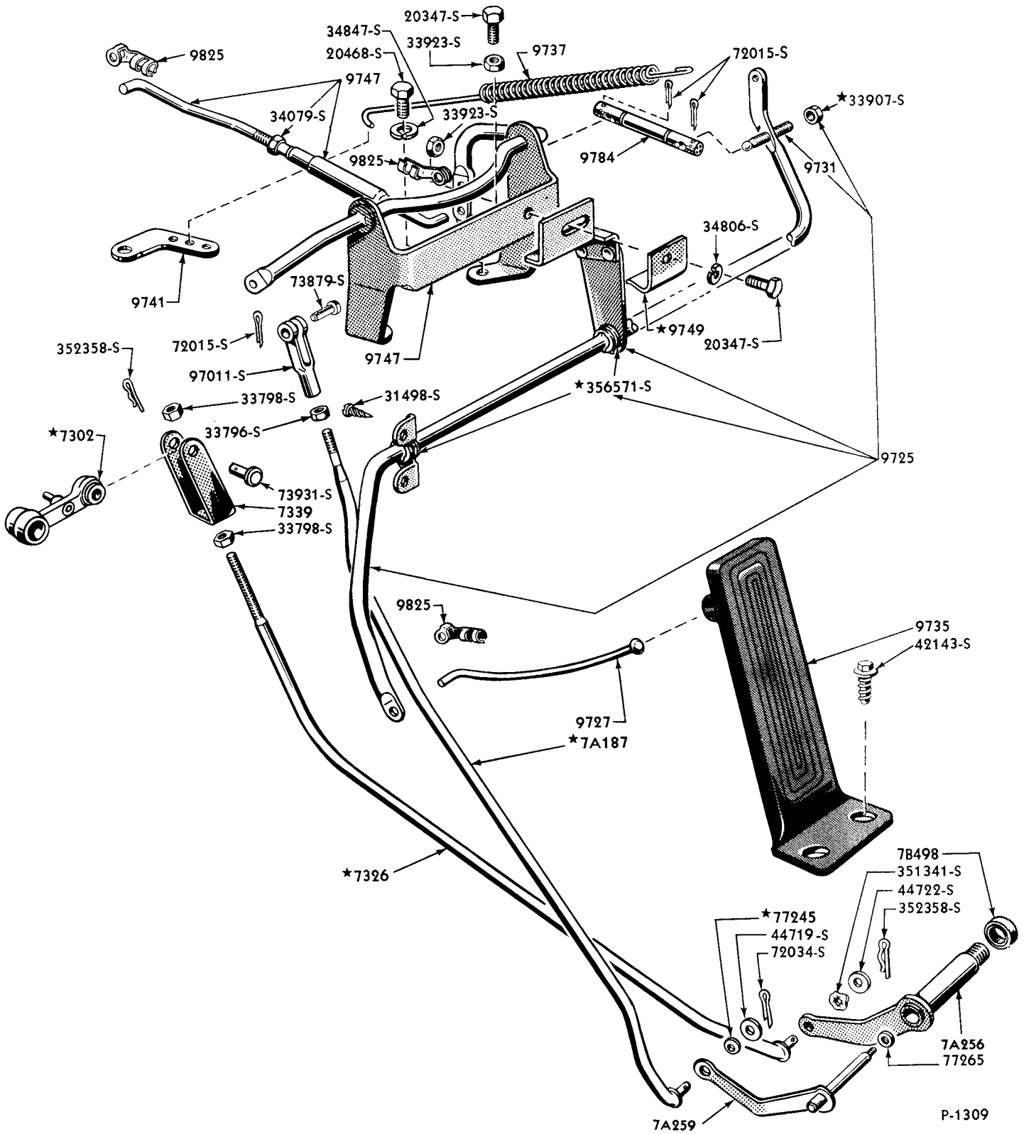
1952/53 ACCELERATOR LINKAGE (8 CYLINDER 239 ENGINE)(WITH FORDOMATIC)
