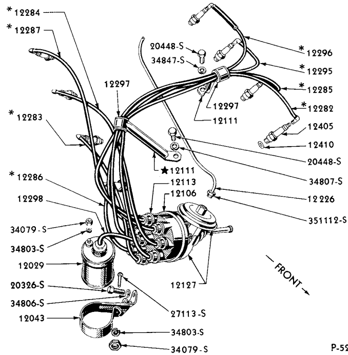
1949/53 IGNITION WIRING (8 CYLINDER 239 ENGINE)
