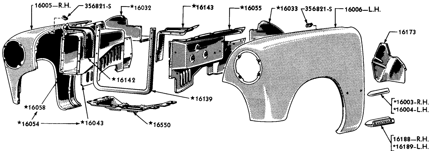
1949 FENDER AND RELATED PARTS
