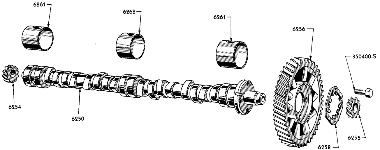
1949/53 CAMSHAFT, GEAR, BEARINGS, ETC. (8 CYLINDER 239 "L" HEAD ENGINE)
