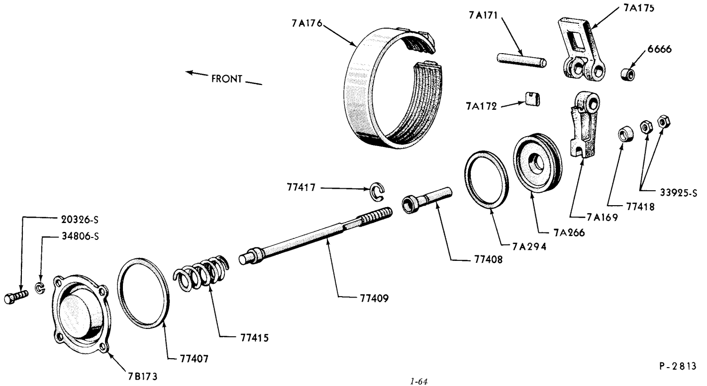
"TYPICAL" REAR SERVO AND BAND(1959/F/M/2 TRANSMISSION)
