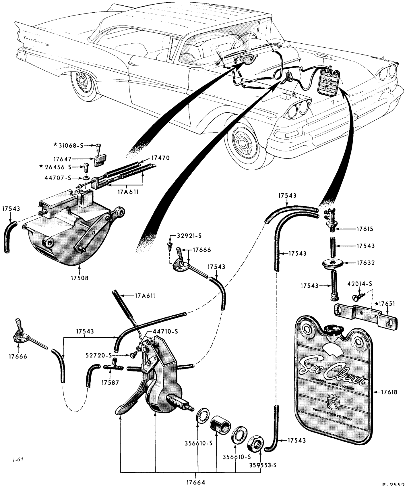
1958 WINDSHIELD WASHER (FORD)
