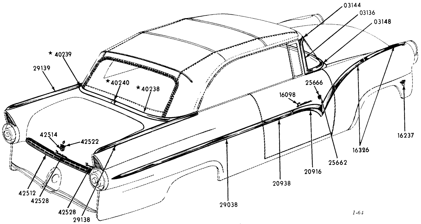
1955 FAIRLANE CONVERTIBLE COUPE (BODY TYPE 76B)
