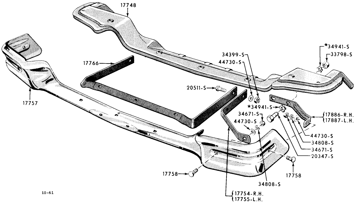
1958 FRONT BUMPER (FORD)
