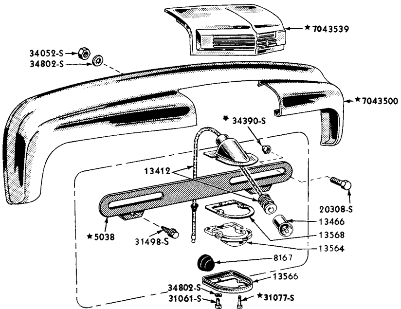
1950 LICENSE PLATE LAMP
