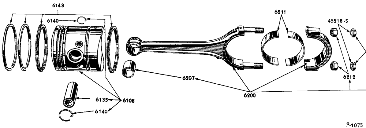
1949/53 PISTON AND CONNECTING ROD (8 CYLINDER 239 "L" HEAD ENGINE)
