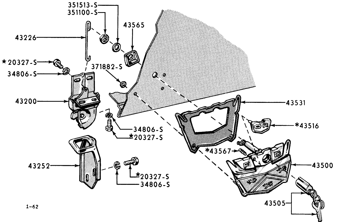
1958/ THUNDERBIRD LUGGAGE COMPARTMENT DOOR LOCK AND RELATED PARTS BODY TYPE S(63A)
