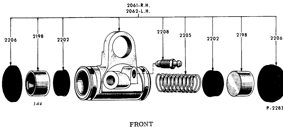
1949/56 FRONT & REAR BRAKE CYLINDERS
