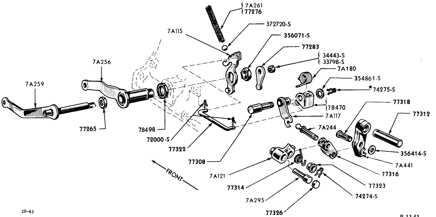
1951/59 "TYPICAL" PARKING PAWL LINKAGE, THROTTLE AND MANUAL CONTROL LEVERS (FORDOMATIC TRANSMISSION)
