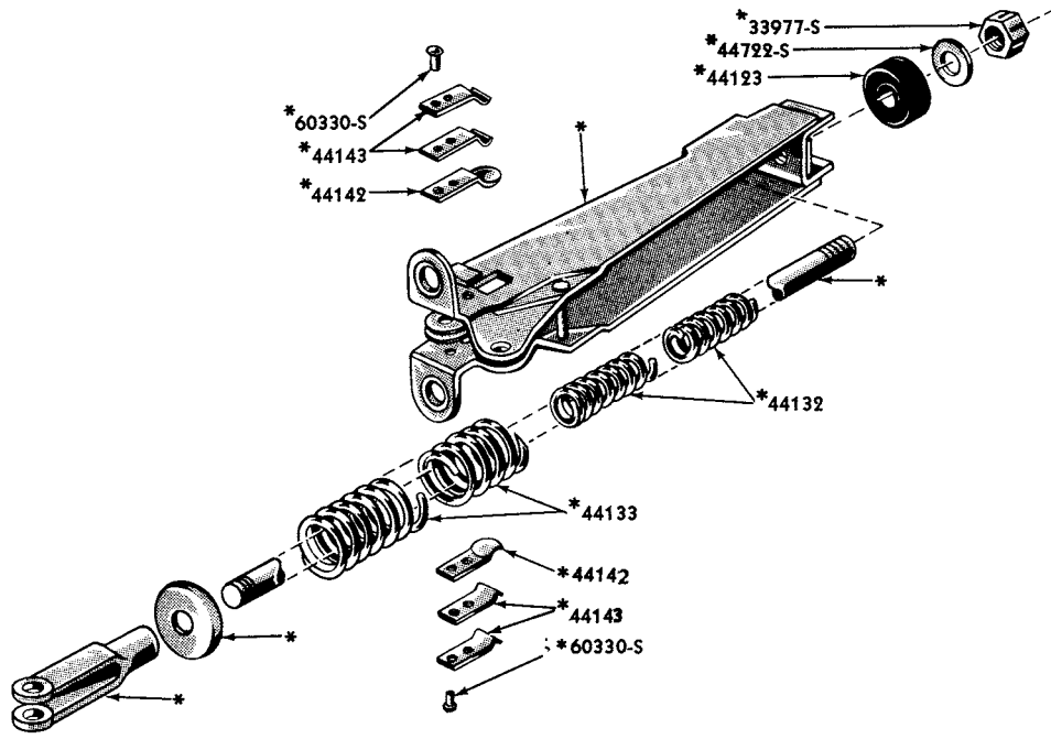
1953 REAR DOOR CHECK ARM ASS'Y. (BODY TYPE 78)
