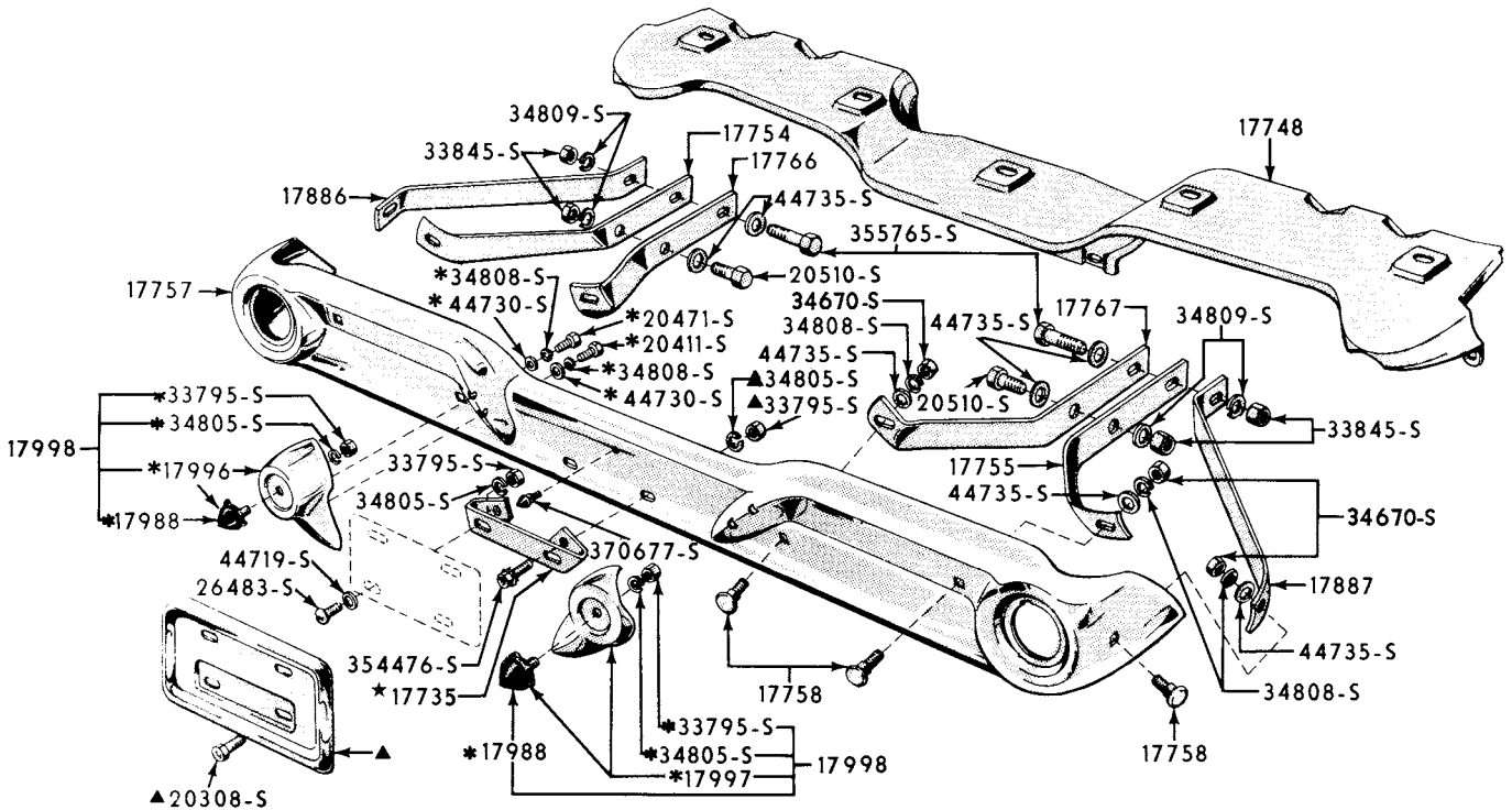
1958/ FRONT BUMPER (THUNDERBIRD)
