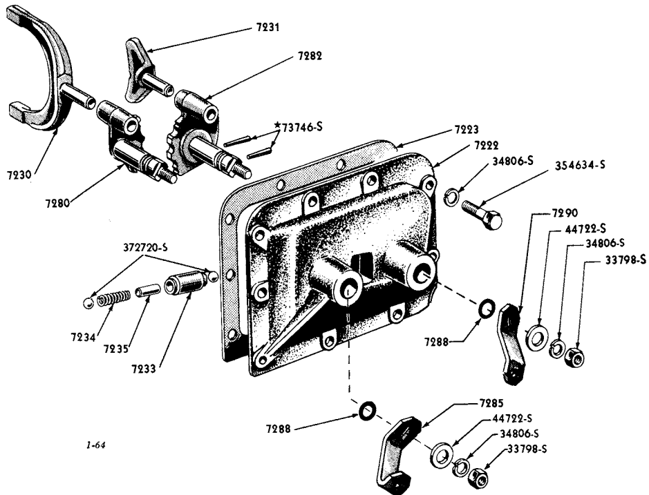
1958/ "TYPICAL" GEAR SHIFT HOUSING, LEVERS, FORKS, ETC. (PASSENGER)
