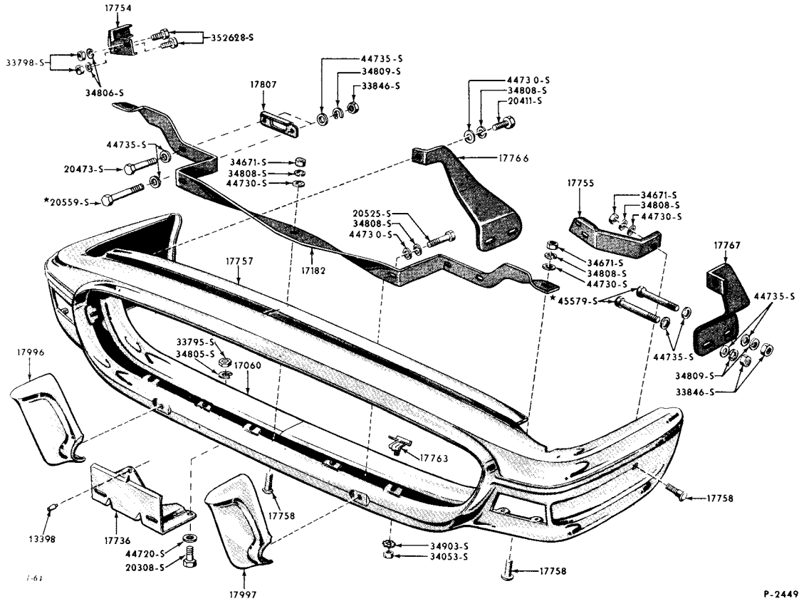
1958/ FRONT BUMPER (THUNDERBIRD)
