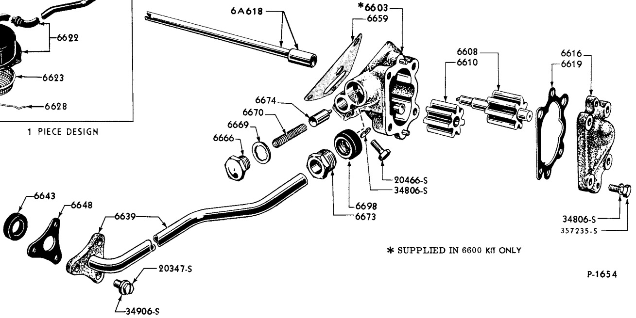
1954 OIL PUMP & RELATED PARTS (8 CYLINDER 239 "O. H. V." ENGINE)
