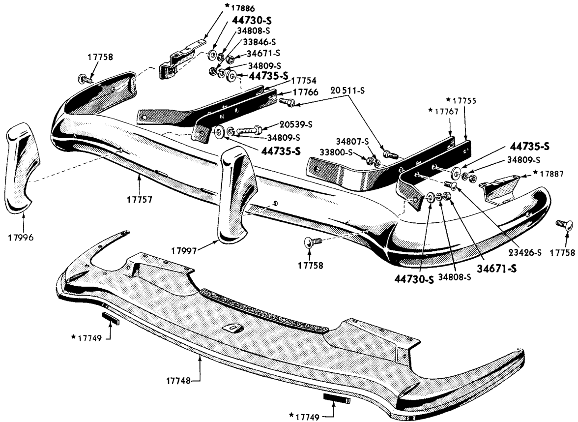
1952/53 FRONT BUMPER
