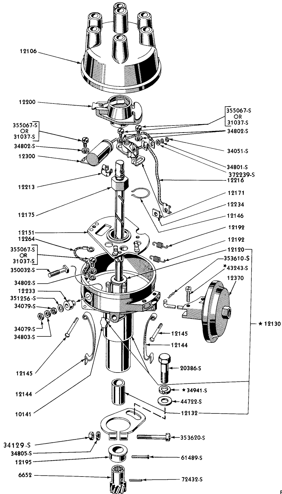
1949/51 DISTRIBUTOR (6 CYLINDER 226 ENGINE)
