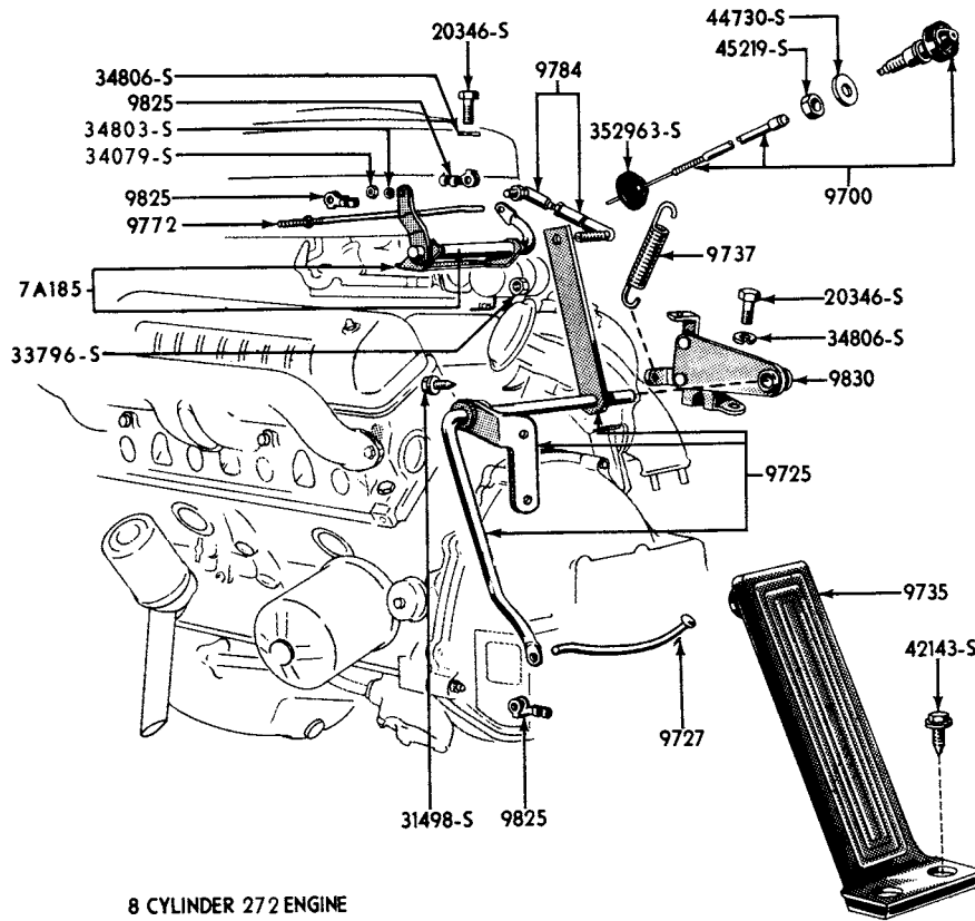
8 CYLINDER 272 ENGINE
