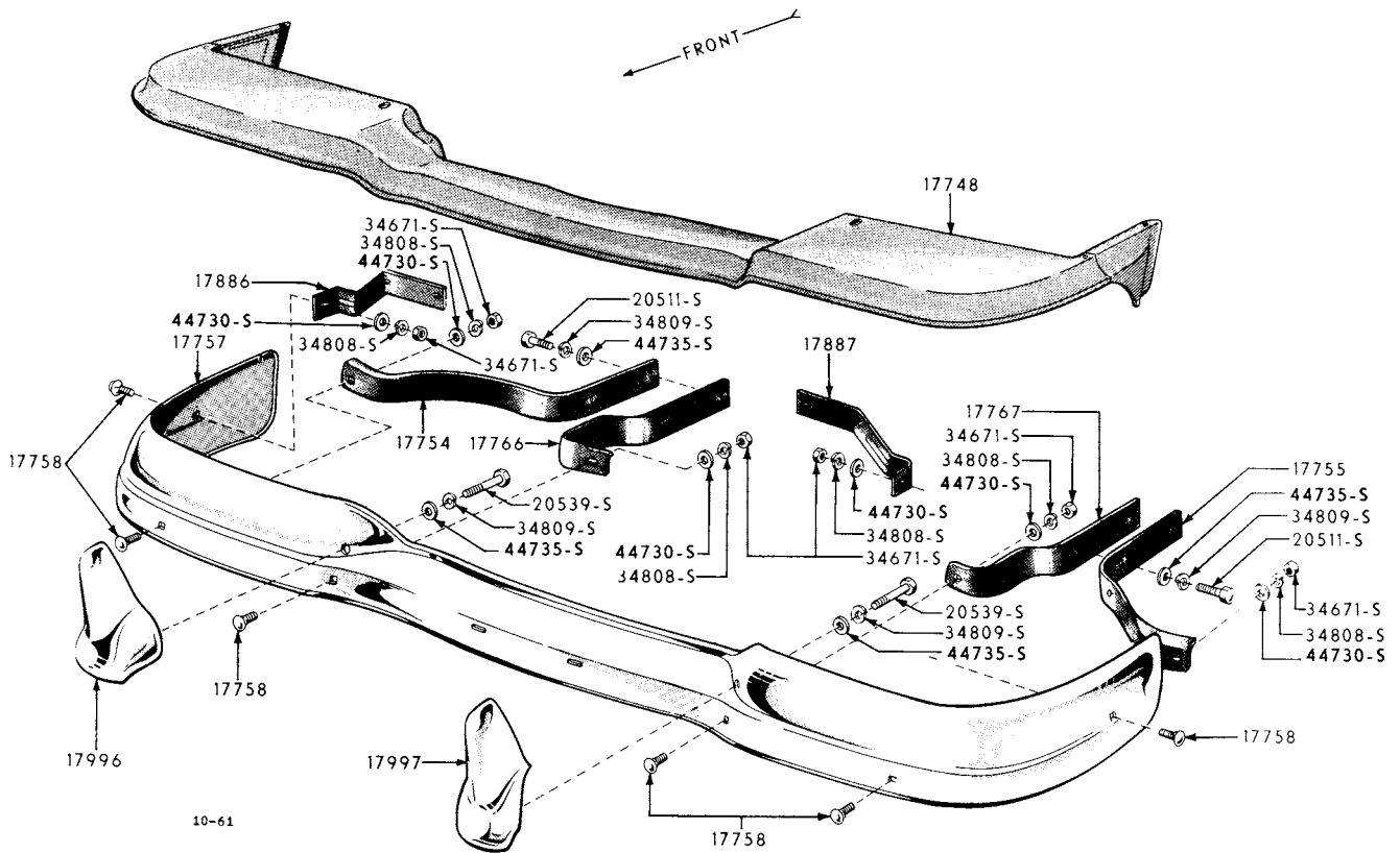
1955/56 FRONT BUMPER (FORD)
