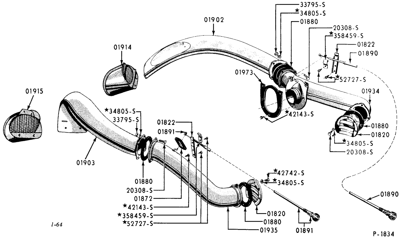
1955/57 THUNDERBIRD VENTILATING SYSTEM WITHOUT HEATER
