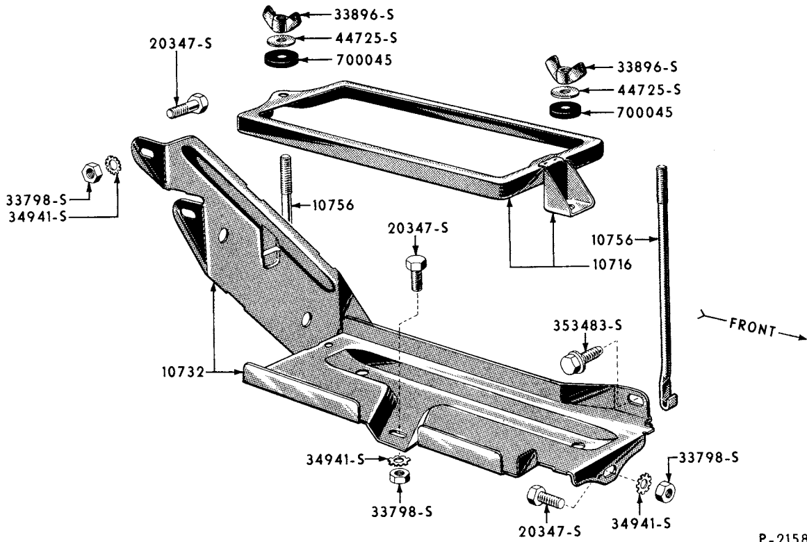
1957/58 BATTERY CARRIER AND RELATED PARTS (FORD)
