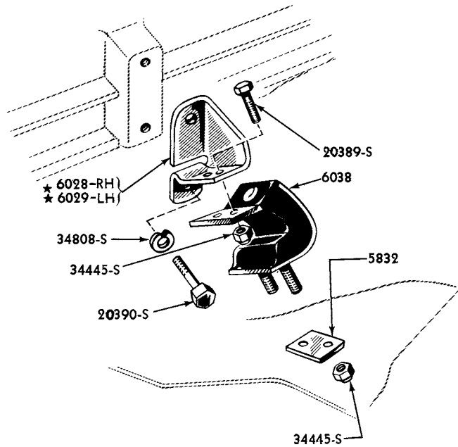
1949/53 ENGINE FRONT SUPPORT 6 CYLINDER 226 ENGINE 8 CYLINDER 239 ENGINE
