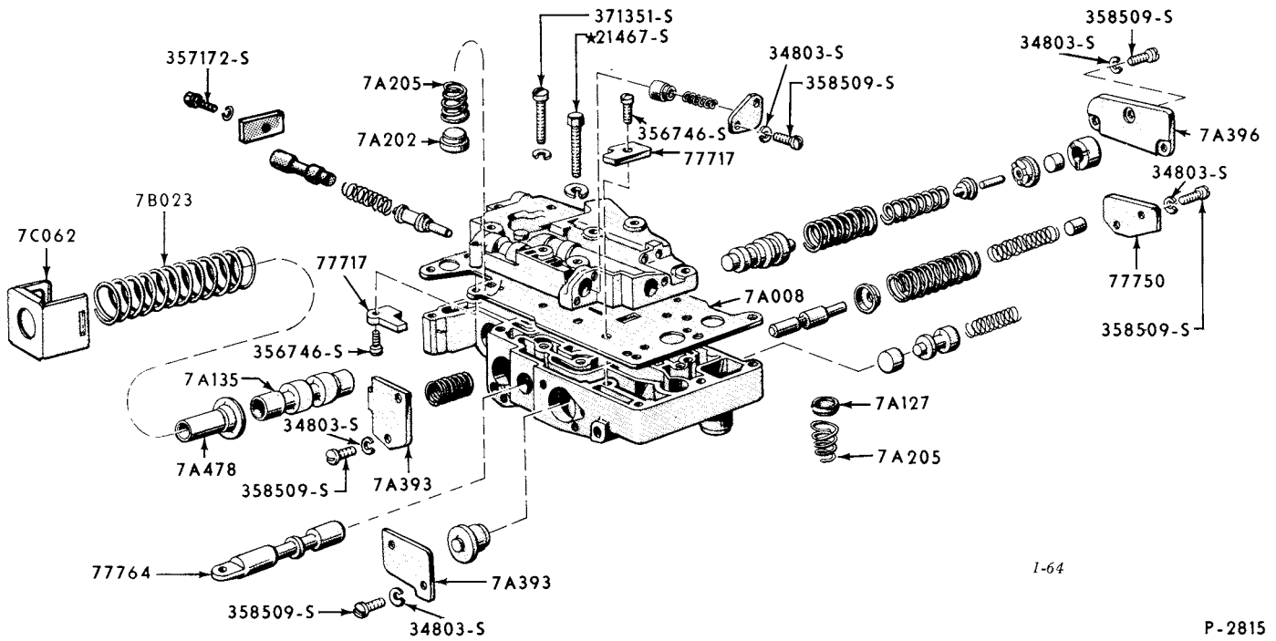
"TYPICAL" MAIN CONTROL (1959/ F/M/2 TRANSMISSION)
