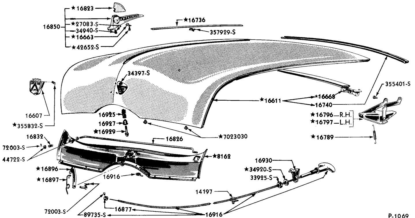
1949 HOOD AND RELATED PARTS
