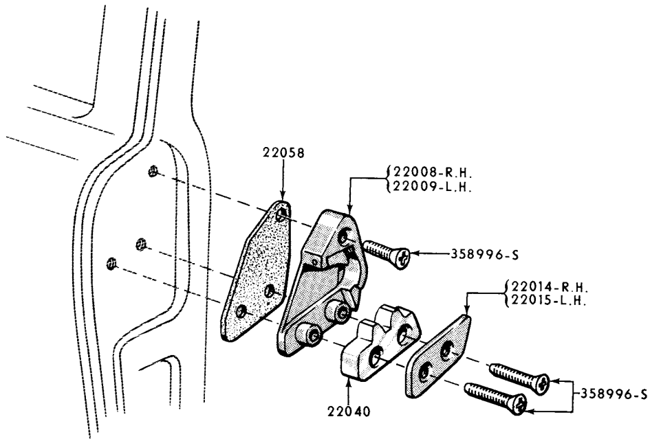
1957/58 DOOR STRIKER PLATE AND RELATED PARTS
