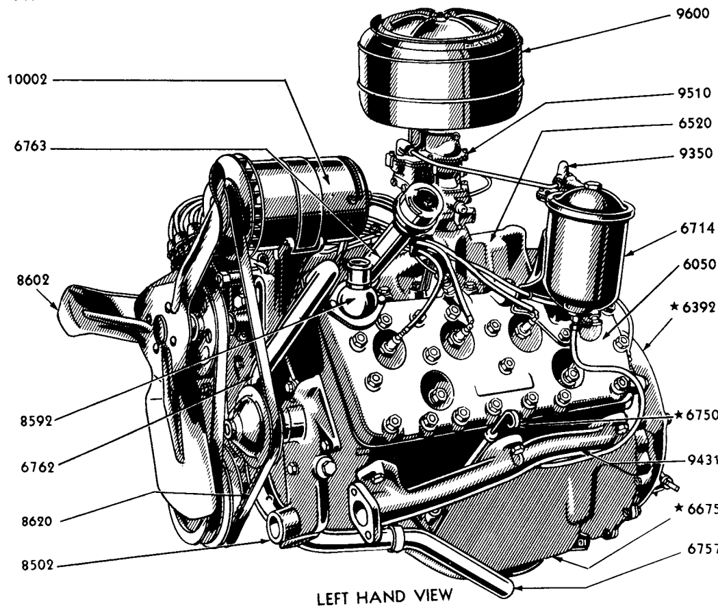
1949/53 (8 CYLINDER 239 ENGINE)-TYPICAL
