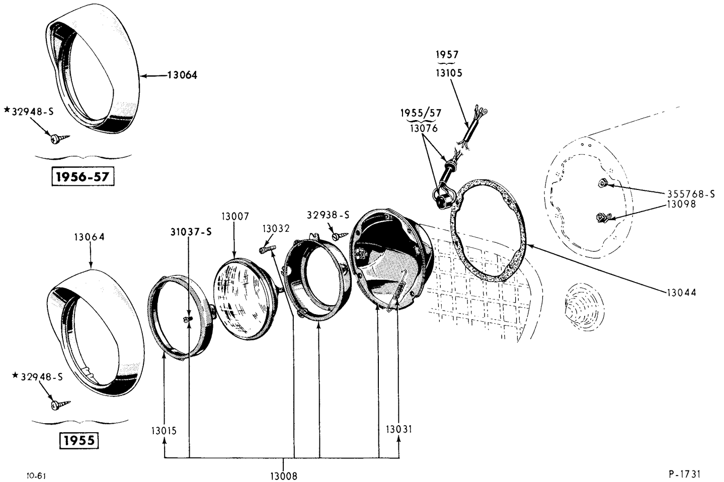
1955/57 HEADLAMP (THUNDERBIRD)
