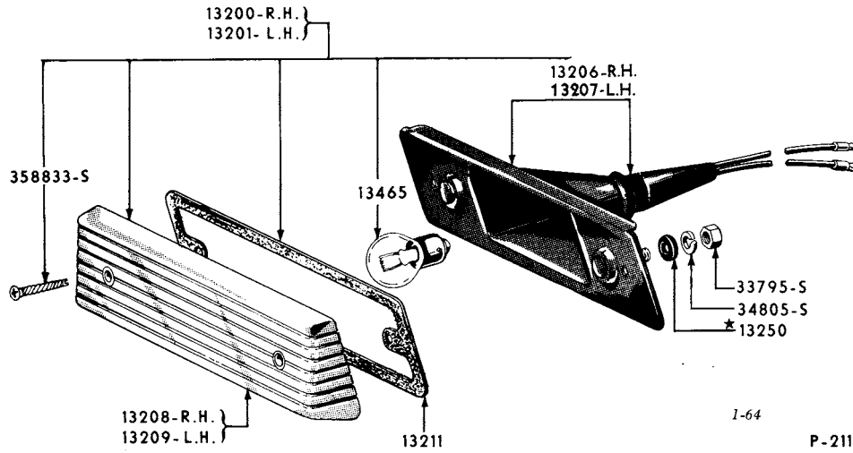
1957 PARKING LAMP (FORD)
