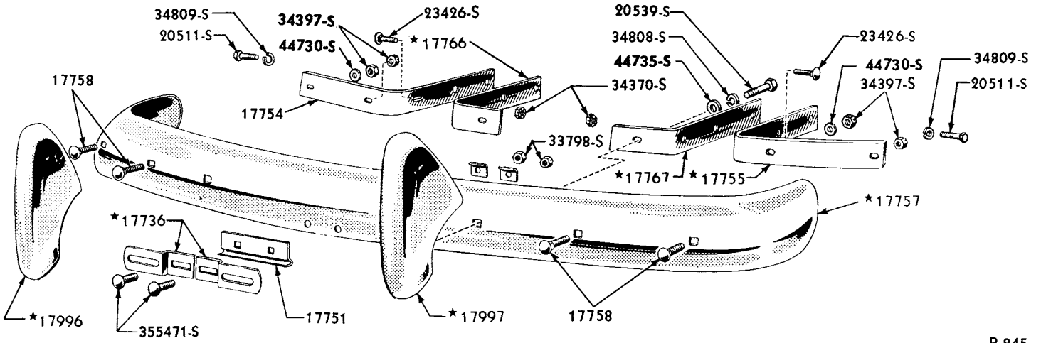
1949 FRONT BUMPER
