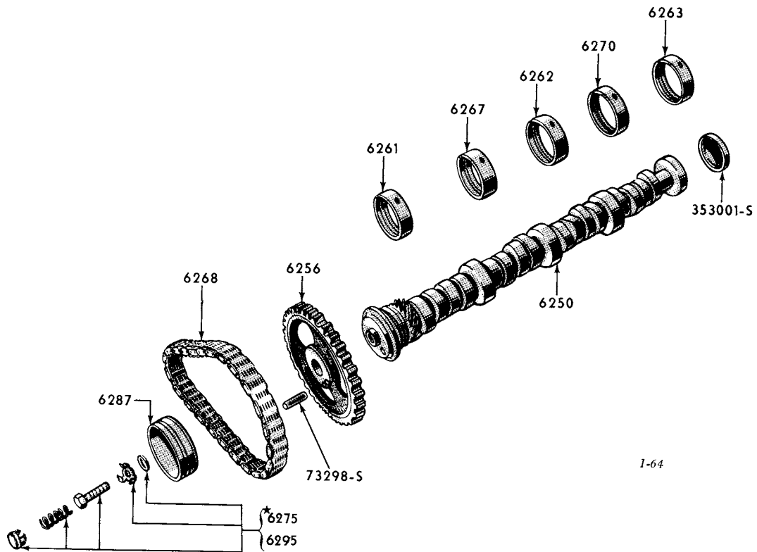
1958/ CAMSHAFT, GEAR, BEARINGS, ETC. (8 CYLINDER 332, 352 ENGINES)-TYPICAL
