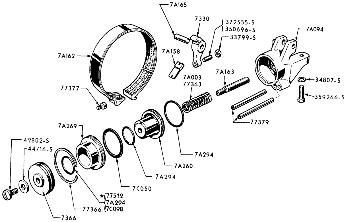
1956/59 8 CYLINDER 312, 332, 352 FRONT SERVO & BAND (FORDOMATIC TRANSMISSION)-TYPICAL
