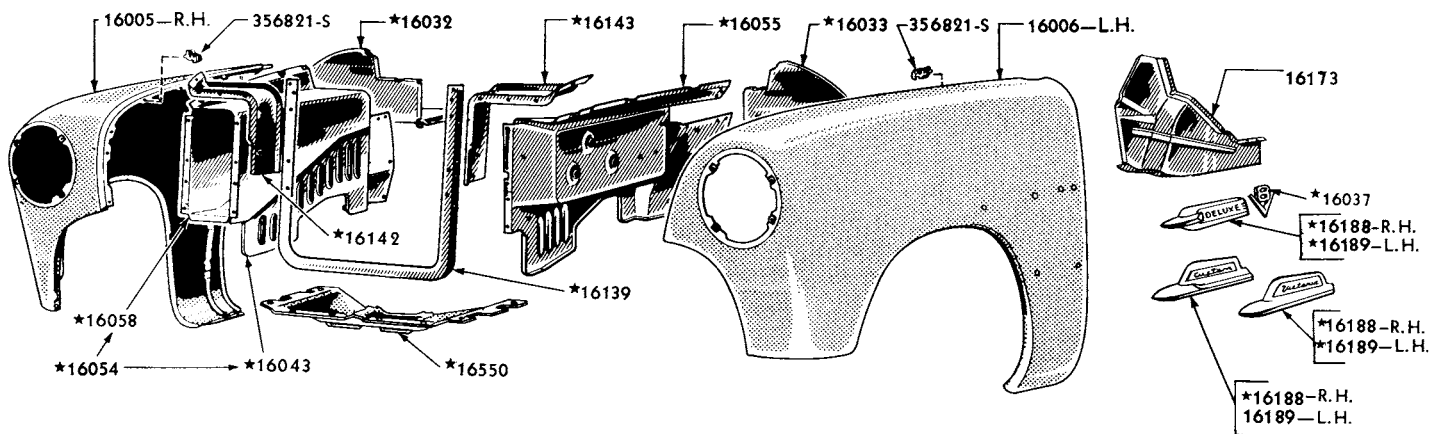
1951 FENDER AND RELATED PARTS
