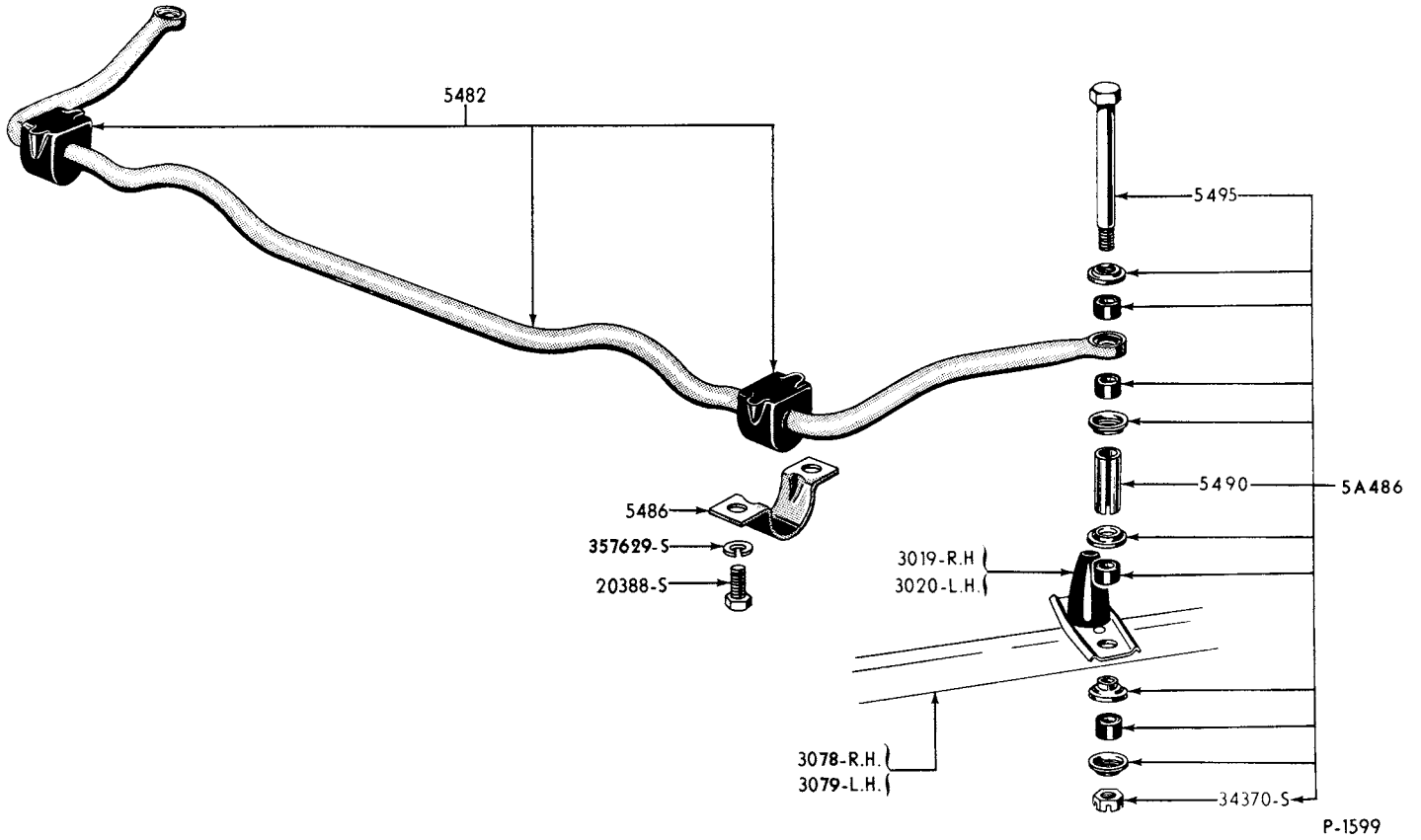
STABILIZER (1954/56 FORD) (1955/57 THUNDERBIRD)
