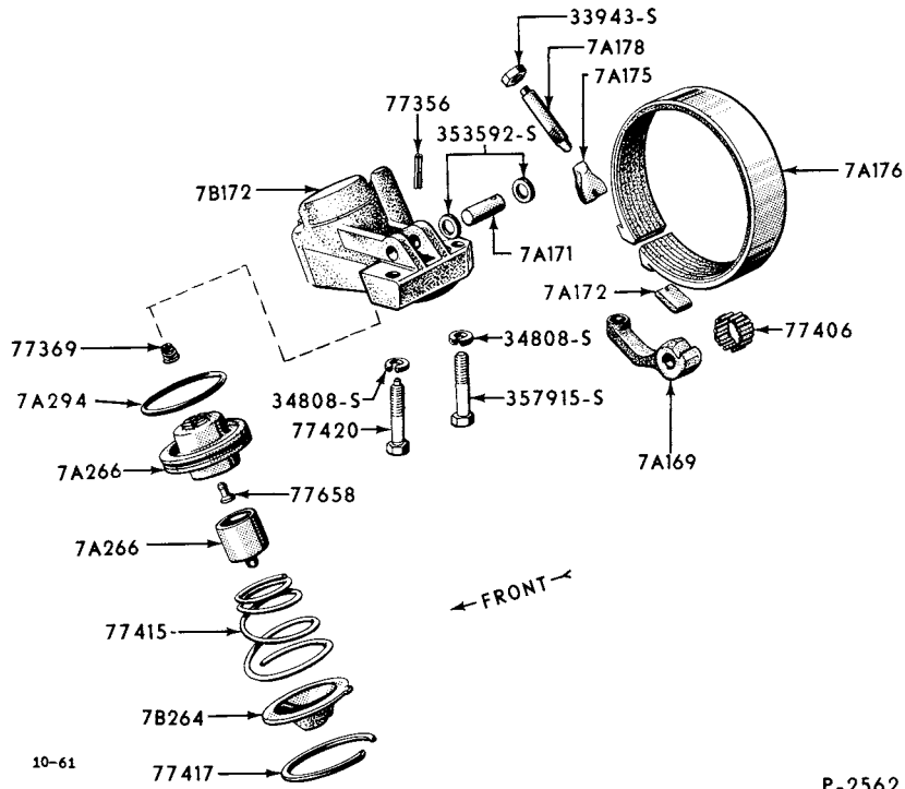
"TYPICAL" REAR SERVO AND BAND (1958 FORDOMATIC TRANSMISSION) (1958/ CRUISE-O-MATIC TRANSMISSION)
