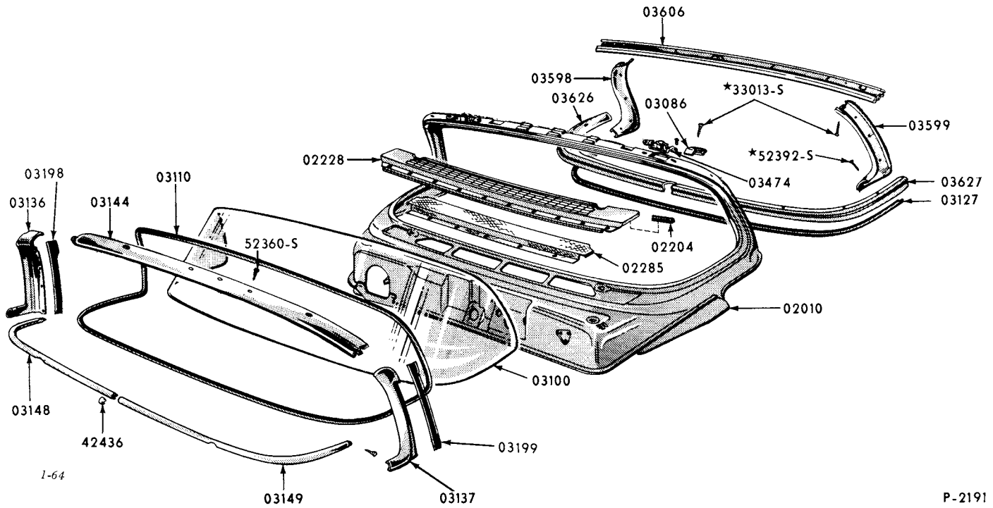
1957/58 WINDSHIELD PARTS (BODY TYPE 51A, 76)
