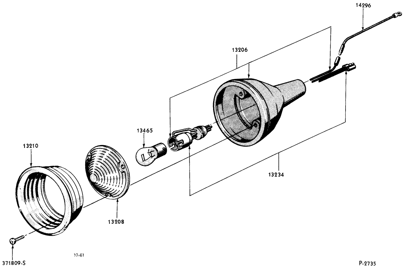
1959 PARKING LAMP (FORD)
