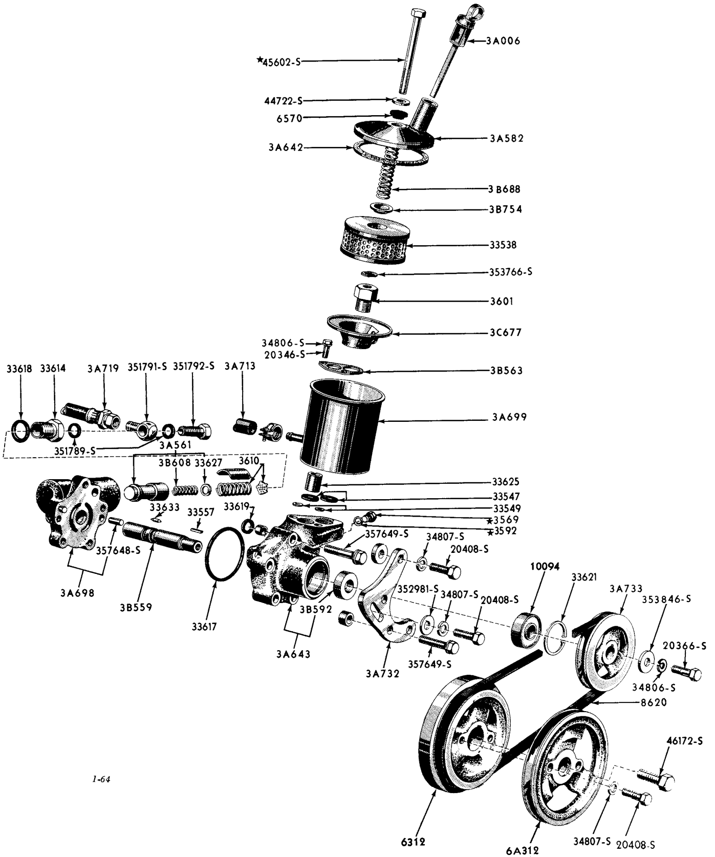
1954/56 "TYPICAL" POWER STEERING PUMP, BRACKET AND RESERVOIR (FORD - 6 CYL.)
