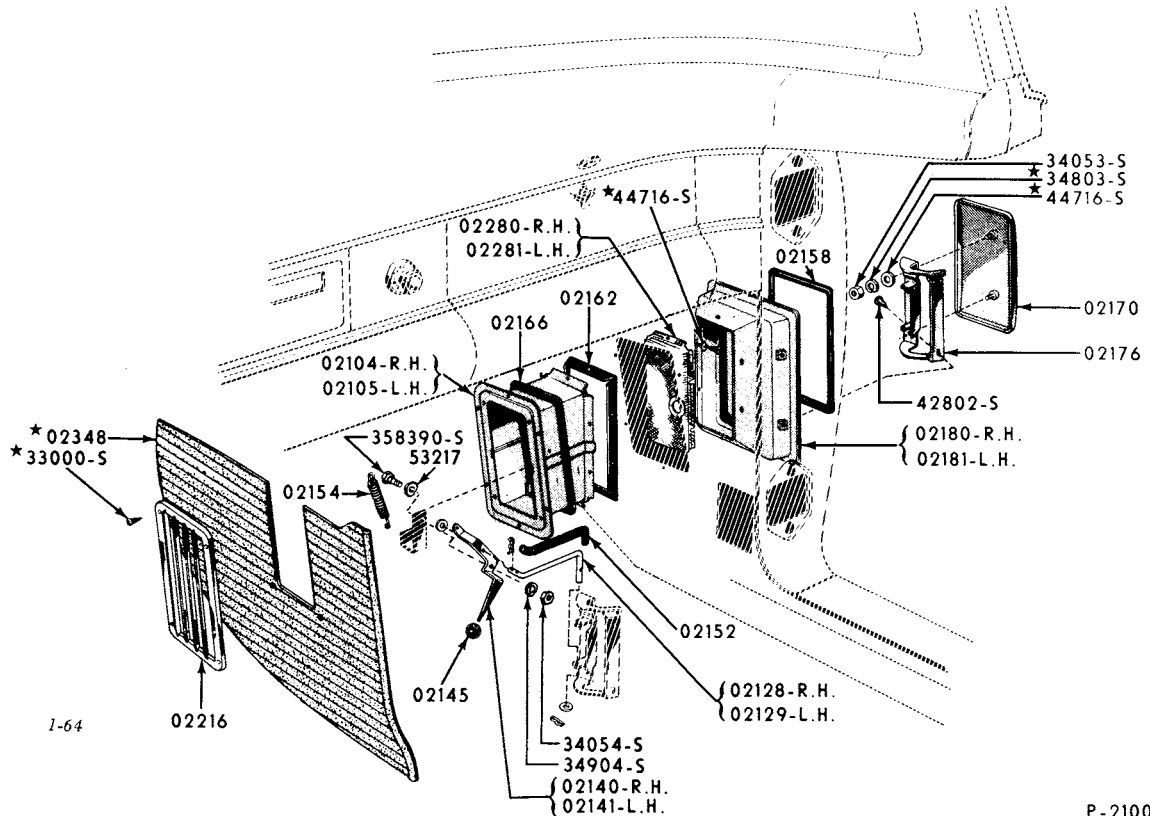
1956/57 THUNDERBIRD COWL SIDE VENTILATOR & RELATED PARTS
