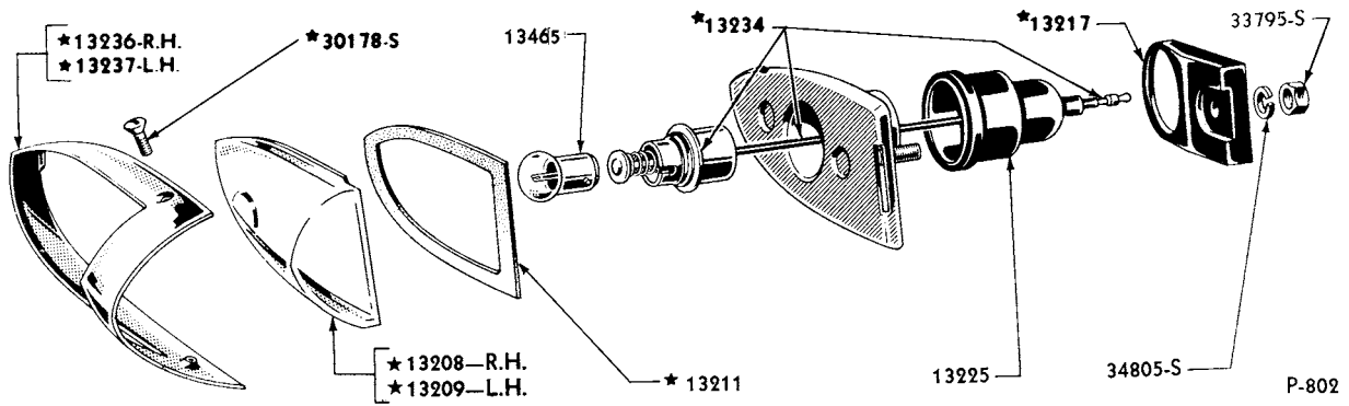
1949 PARKING LAMP
