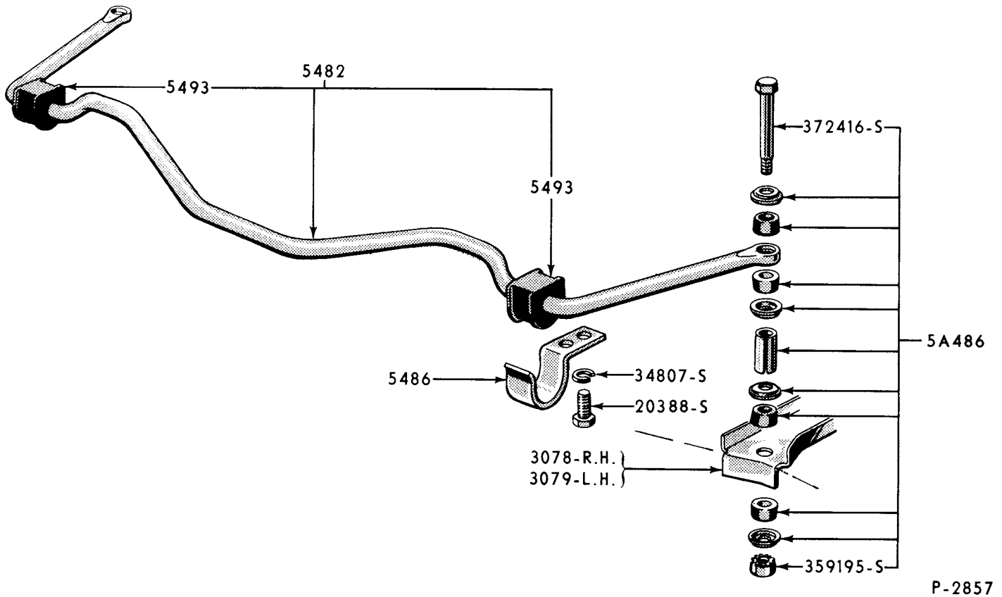
1959 PASSENGER STABILIZER
