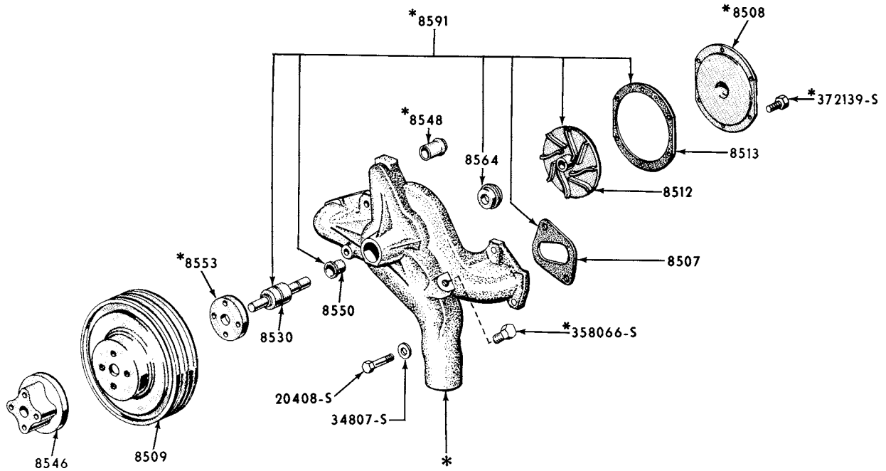
1958/ WATER PUMP (8 CYLINDER 332, 352 ENGINES)
