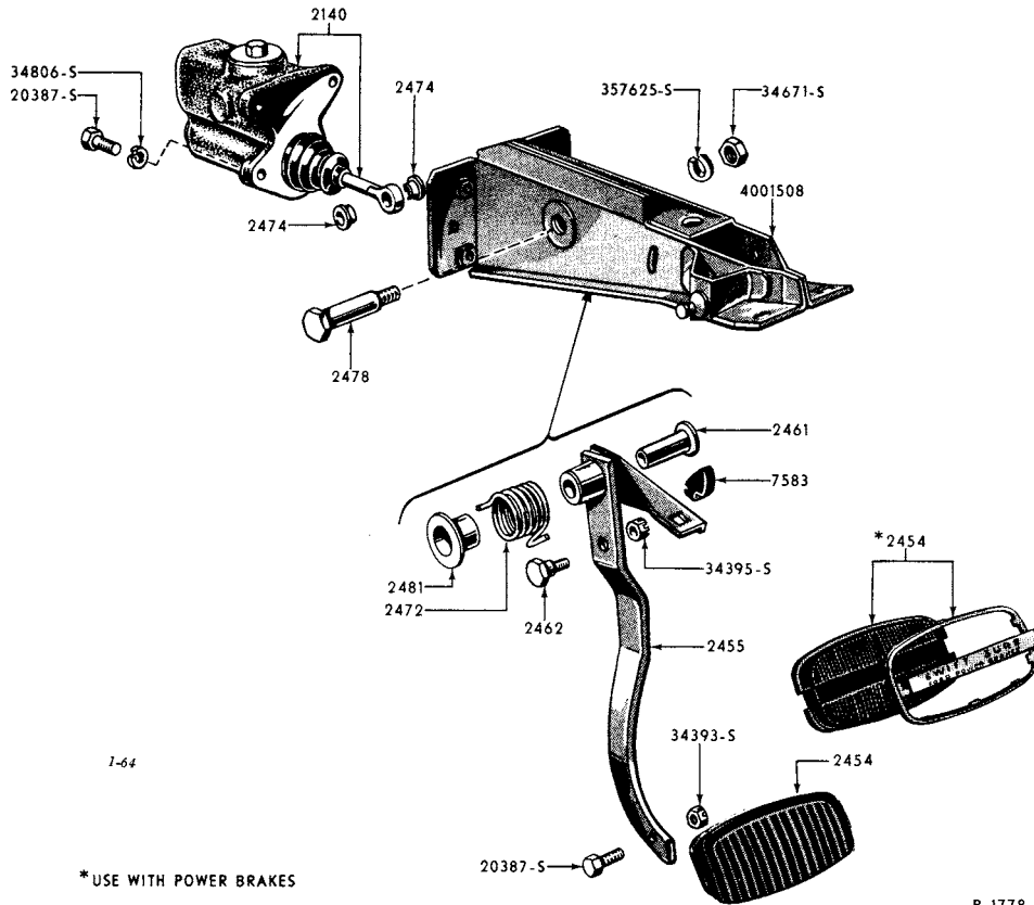
1955/59 BRAKE PEDAL & RELATED PARTS (FORDOMATIC)(THUNDERBIRD)
