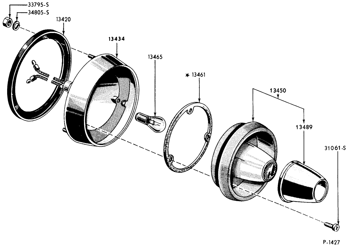
1953 REAR LAMP
