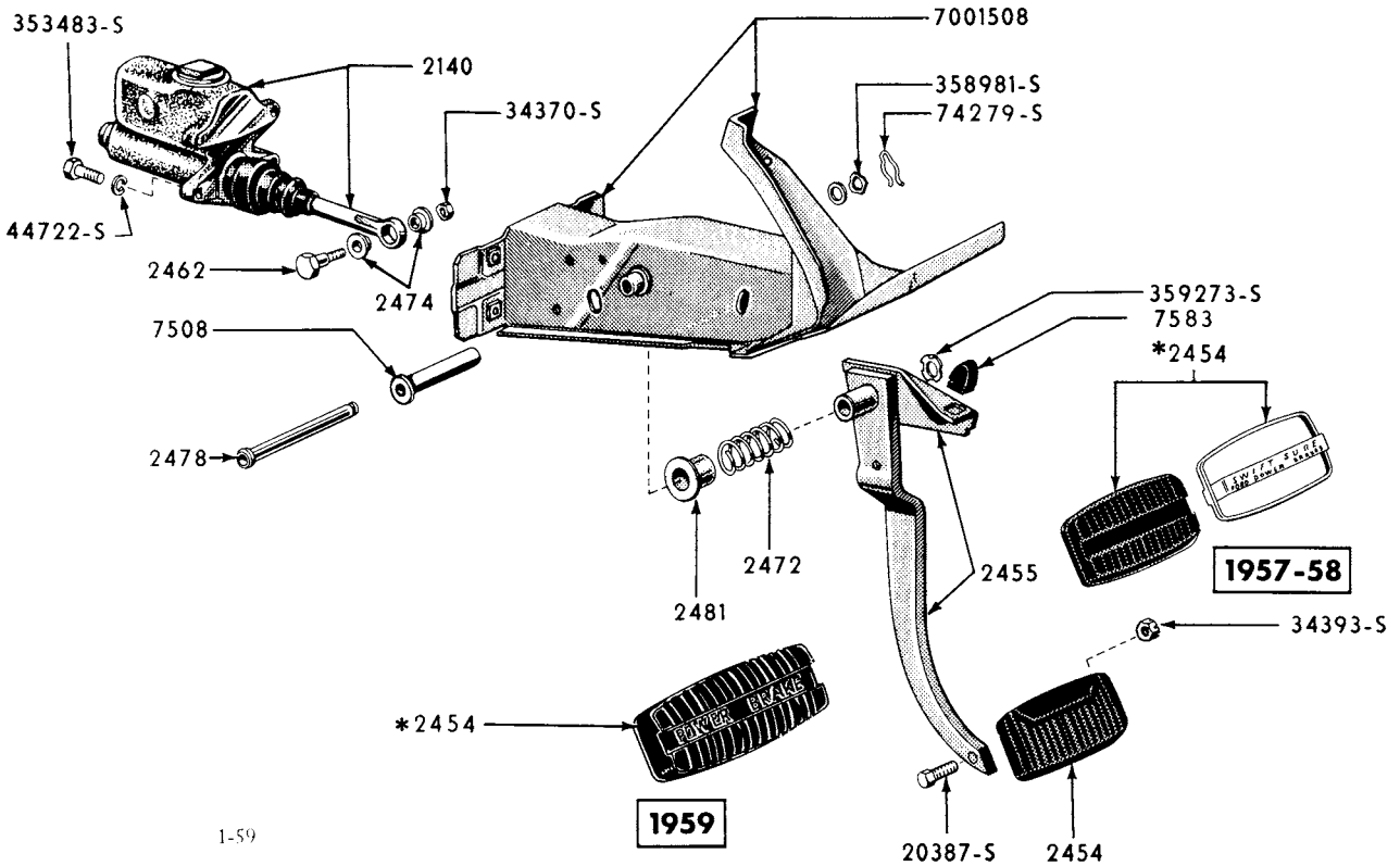
1957/59 BRAKE PEDAL AND RELATED PARTS (FORDOMATIC) (FORD)
