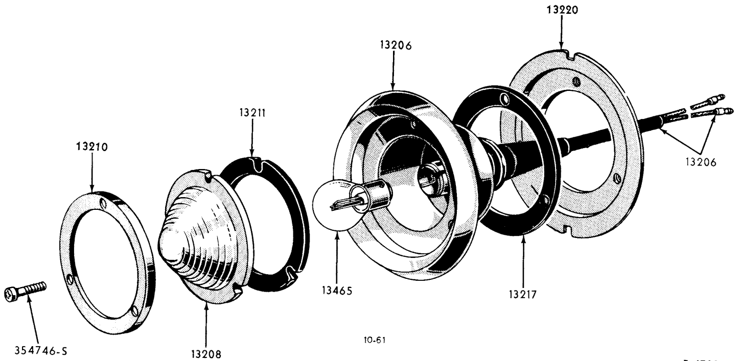
1955/56 PARKING LAMP (THUNDERBIRD)
