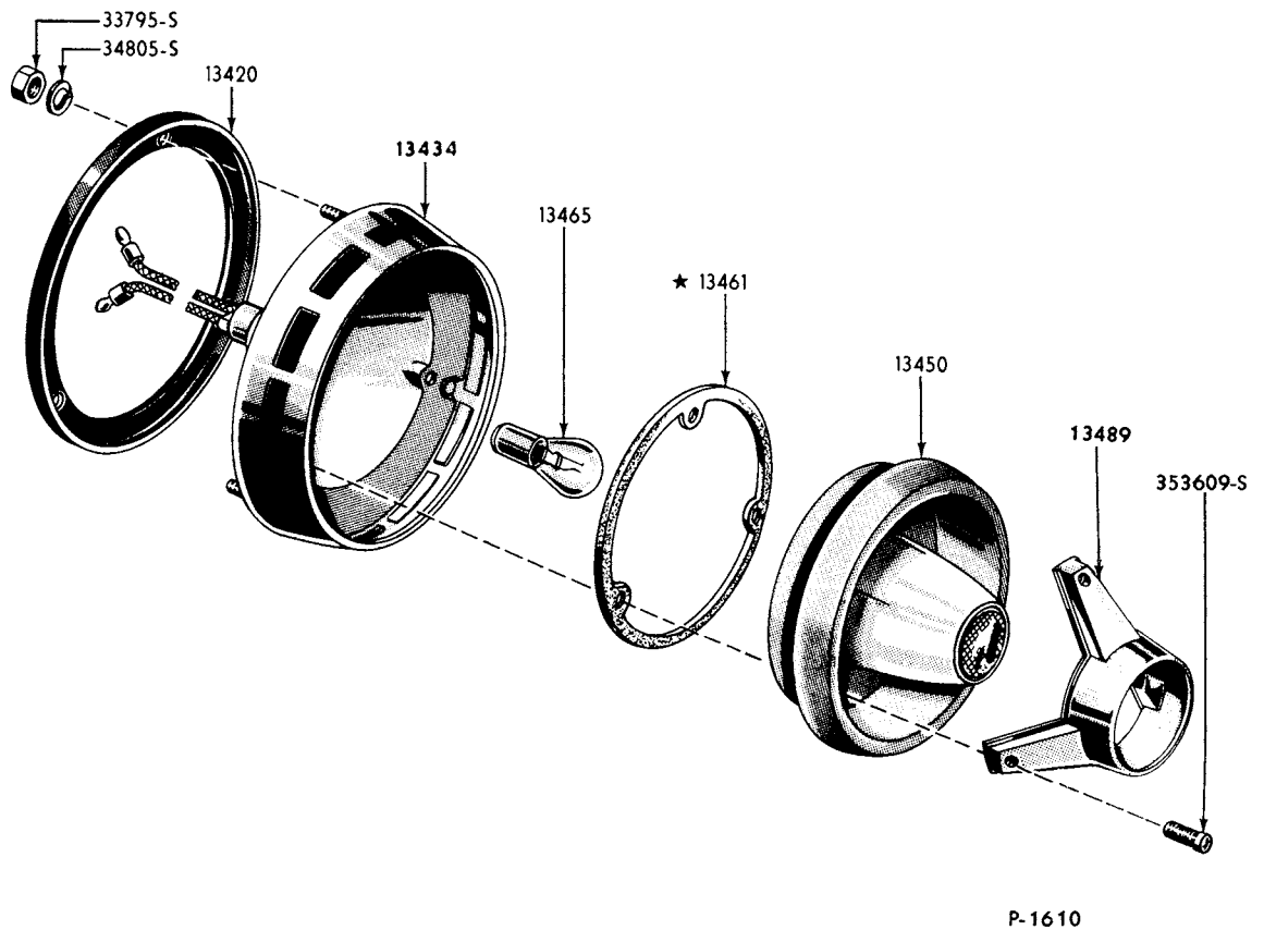
1954 REAR LAMP
