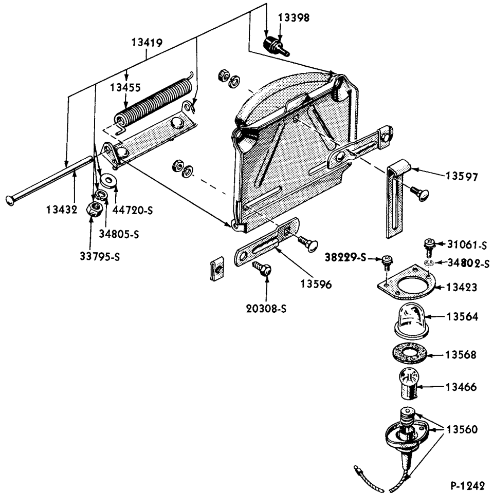
1952/54 LICENSE PLATE LAMP
