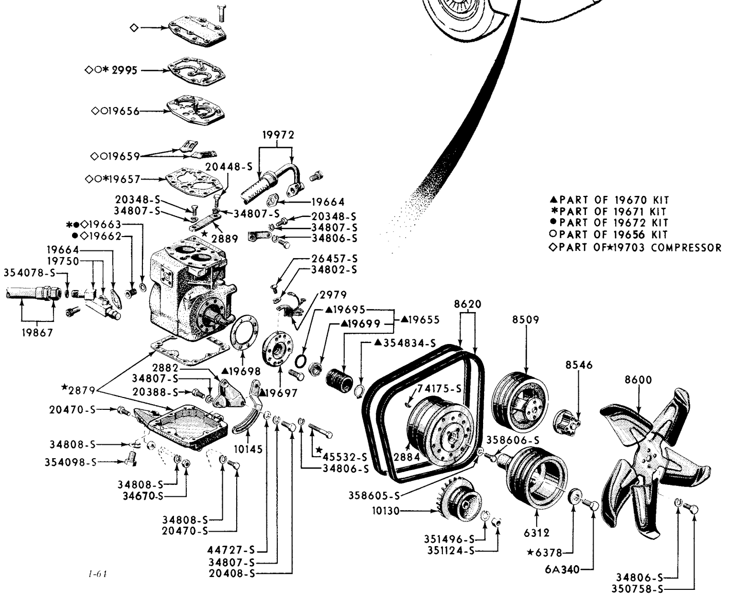
1957 FORD SELECT AIRE & POLAR AIRE CONDITIONER COMPRESSOR, PULLEYS & RELATED PARTS-TYPICAL
