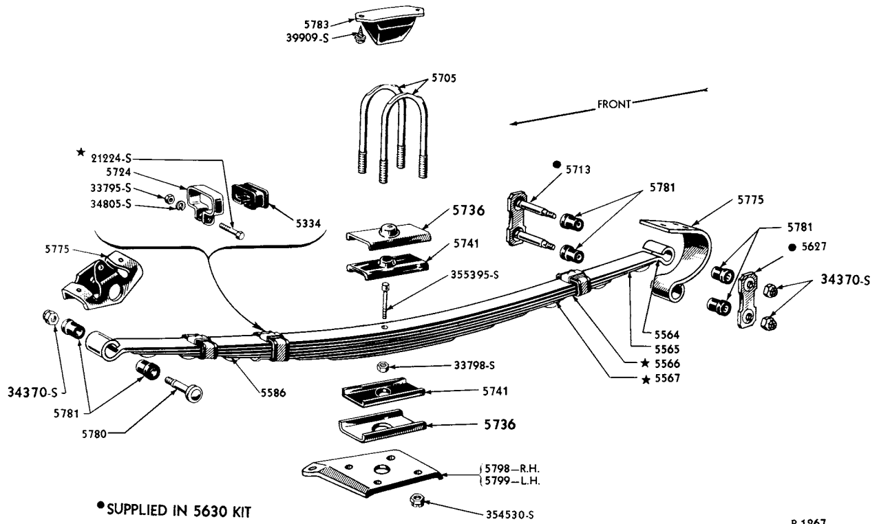
1952/54 REAR SPRING
