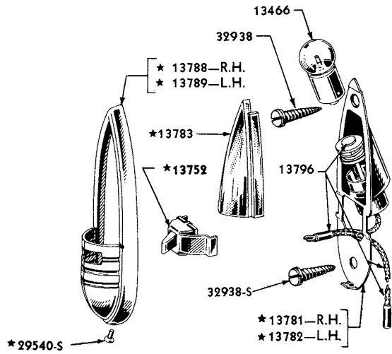
1949 FORDOR SEDAN PILLAR LAMP
