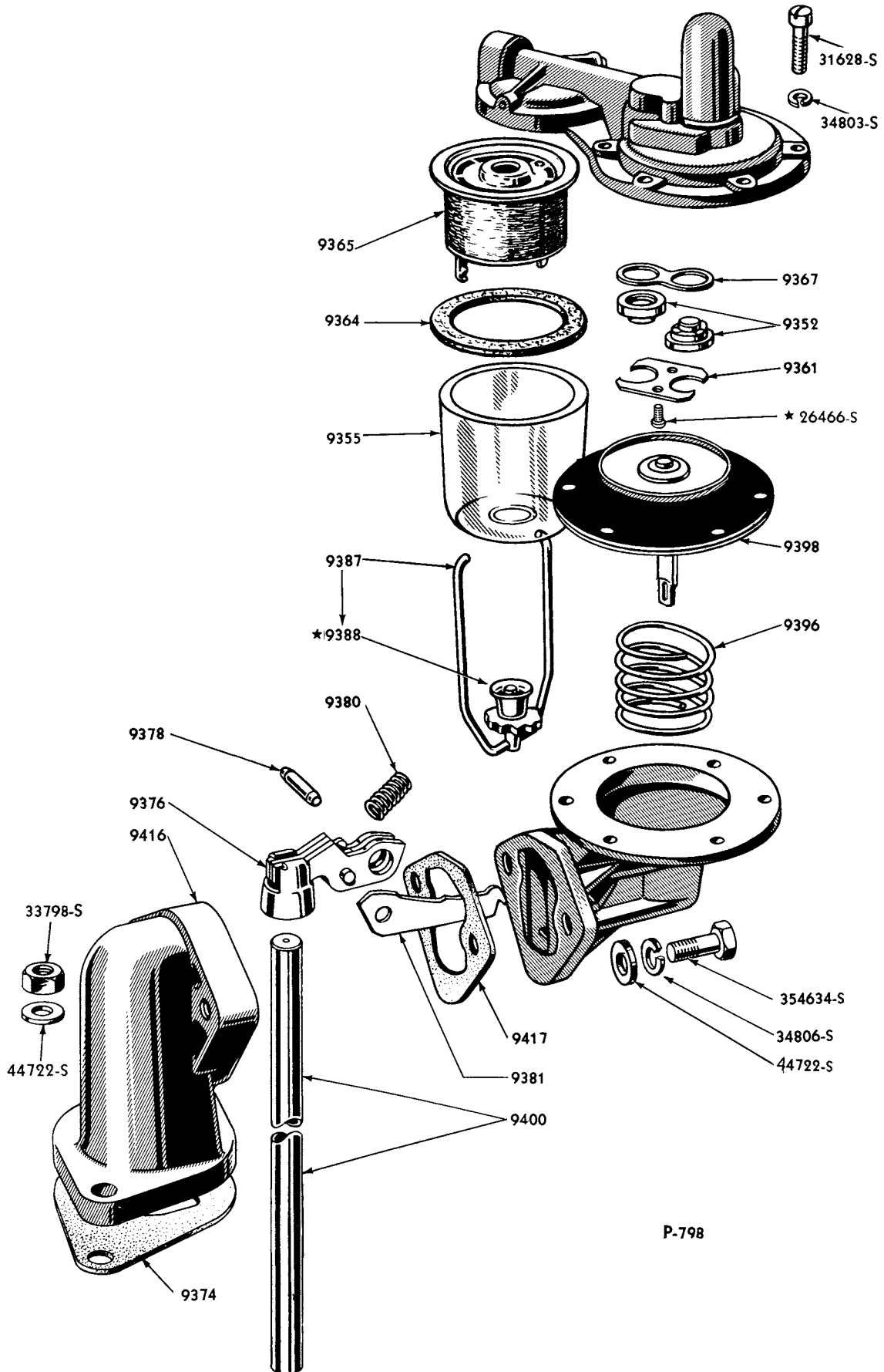
1949/53 FUEL PUMP (8 CYLINDER 239 ENGINE)
