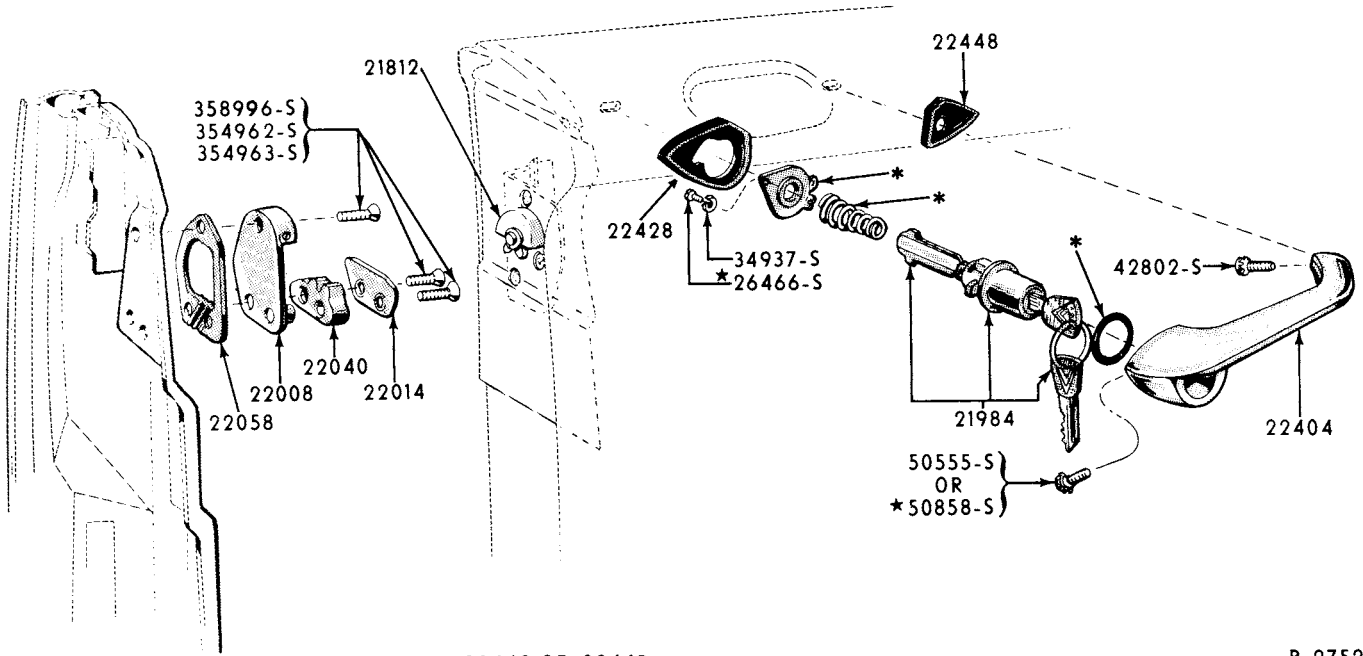
1959 FRONT DOOR OUTSIDE HANDLE & RELATED PARTS
