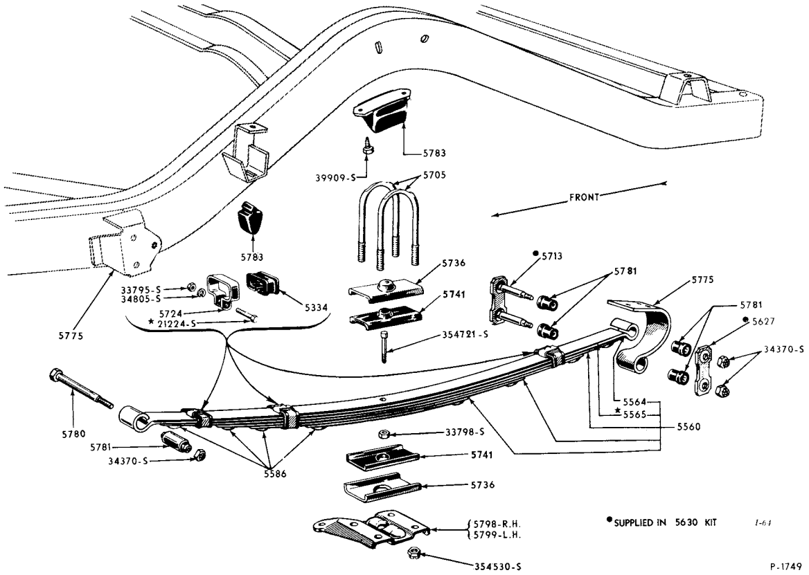
1955/57 REAR SUSPENSION (THUNDERBIRD)
