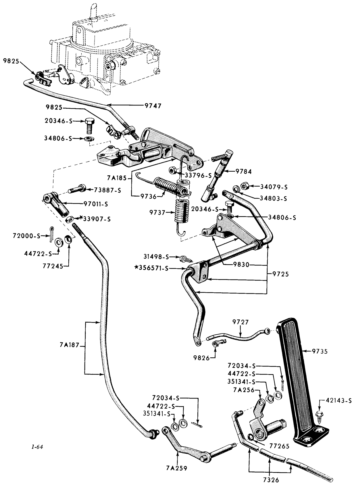
1957 ACCELERATOR LINKAGE - WITH 4 BARREL CARBURETOR - FORDOMATIC (THUNDERBIRD)
