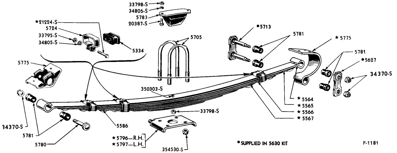
1951 REAR SUSPENSION
