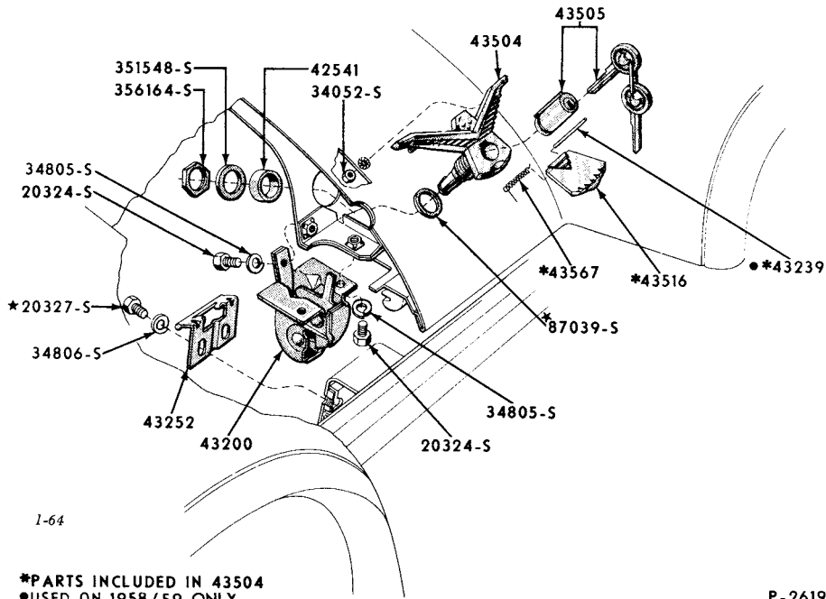
1958/ THUNDERBIRD LUGGAGE COMPARTMENT DOOR LOCK AND RELATED PARTS BODY TYPE S(63A)
