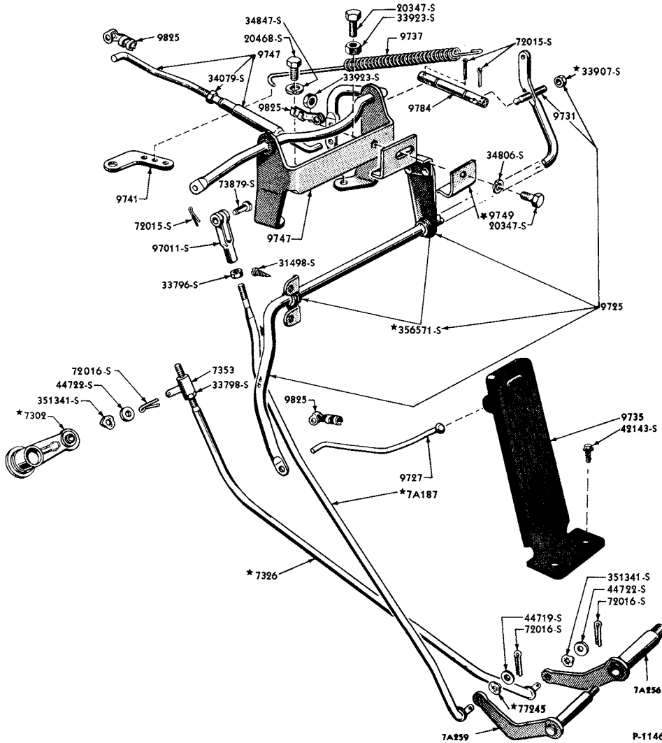
1951 ACCELERATOR LINKAGE (FORDOMATIC)
