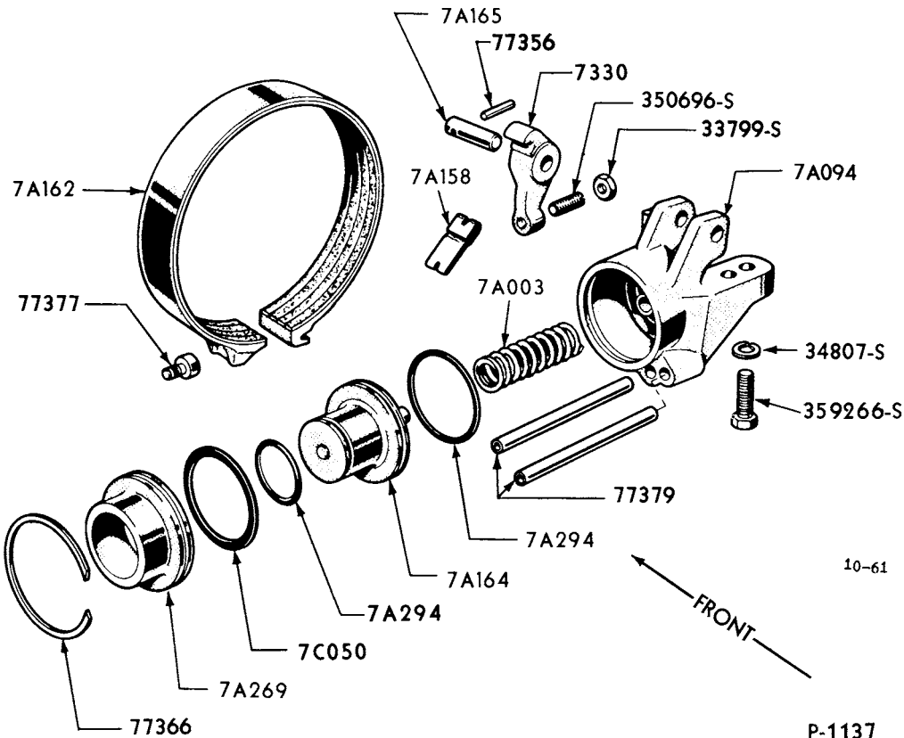
1951/59 "TYPICAL" 6 & 8 CYLINDER 215, 223, 239, 272, 292 FRONT SERVO & BAND (FORDOMATIC TRANSMISSION)
