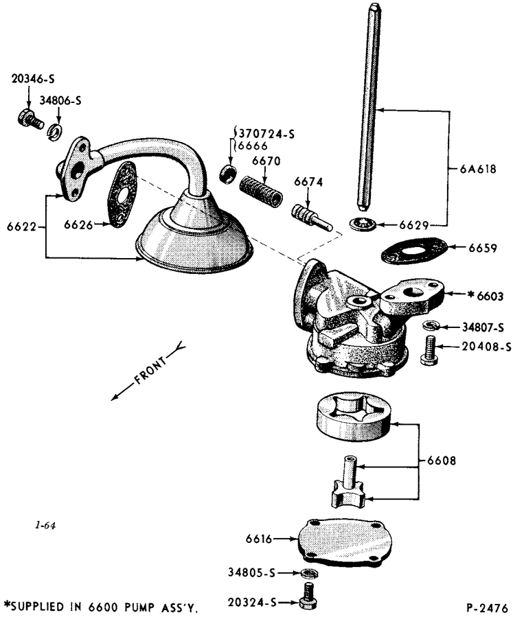
1958/ OIL PUMP & RELATED PARTS (8 CYLINDER 332, 352 ENGINES)-TYPICAL
