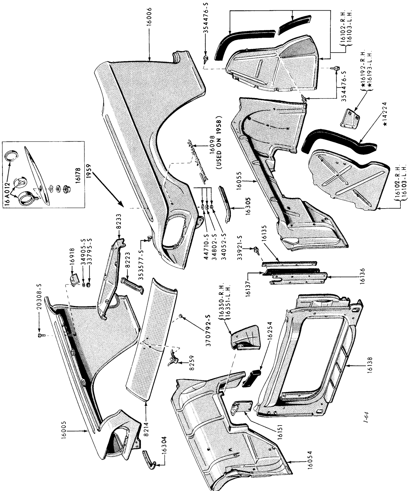
1958/ FENDERS & RELATED PARTS (THUNDERBIRD)
