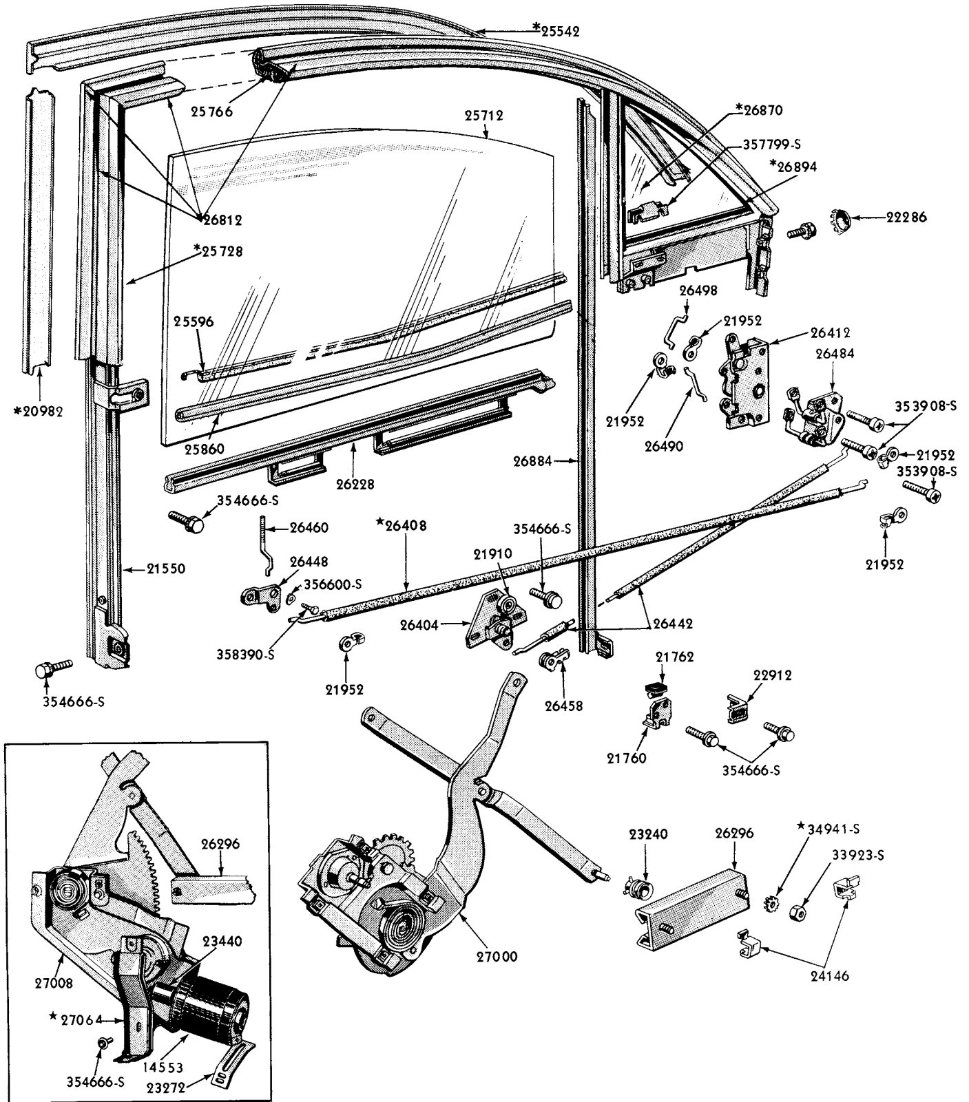
ELECTRIC REGULATOR
