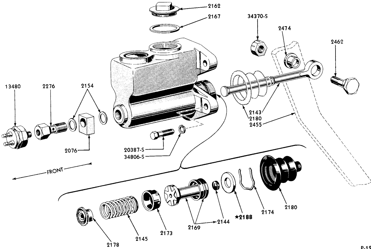
1952/54 BRAKE MASTER CYLINDER
