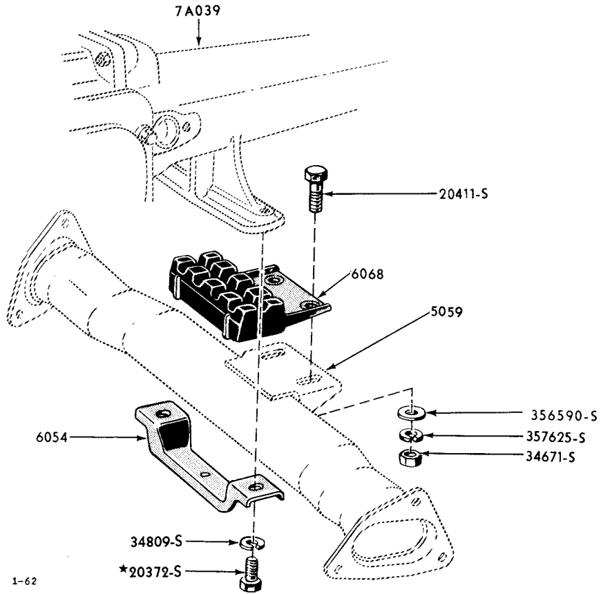
1957/59 ENGINE SUPPORT-REAR
