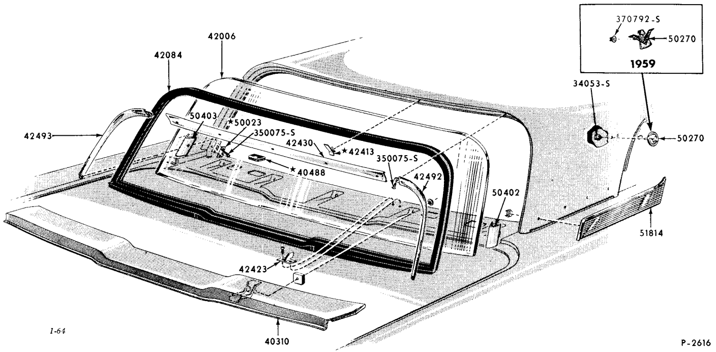
1958/ THUNDERBIRD BACK WINDOW & RELATED PARTS-BODY TYPE S(63A)
