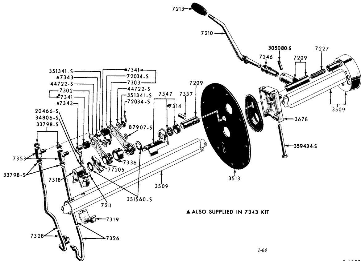
1956 GEAR SHIFT COLUMN (FORD - 6 & 8 CYLINDER ENGINES)
