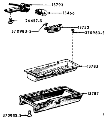
1954/56 DOME LAMP (FORD)
