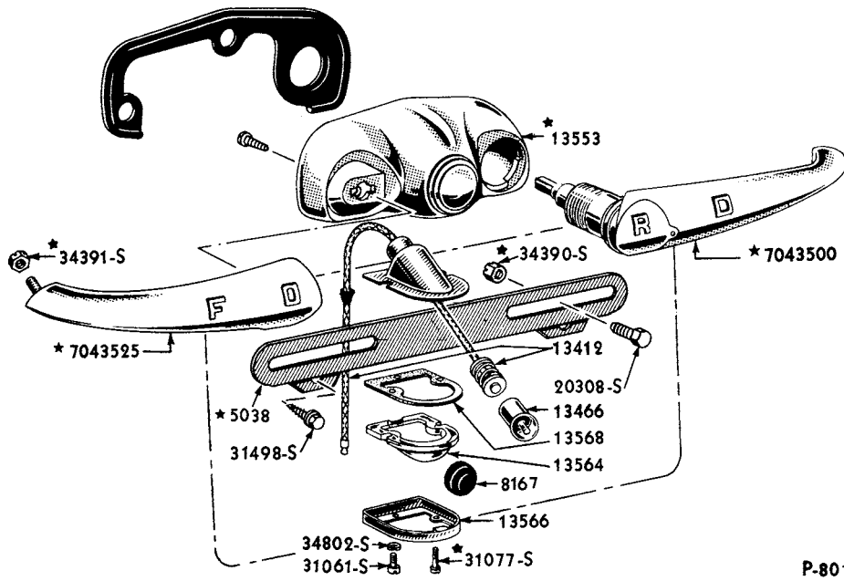
1949 LICENSE PLATE LAMP
