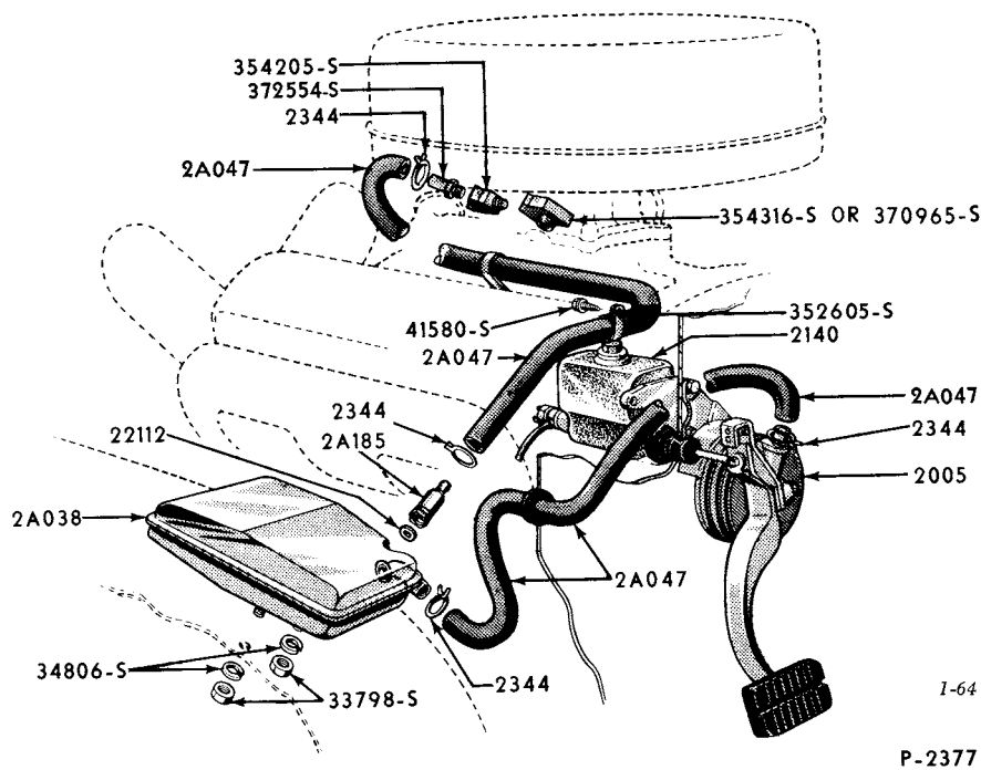
1957/59 POWER BRAKE BOOSTER INSTALLATION (FORD) 1957 THUNDERBIRD
