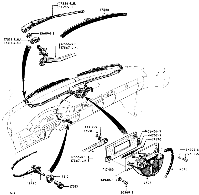
1958 WINDSHIELD WIPER (FORD)
