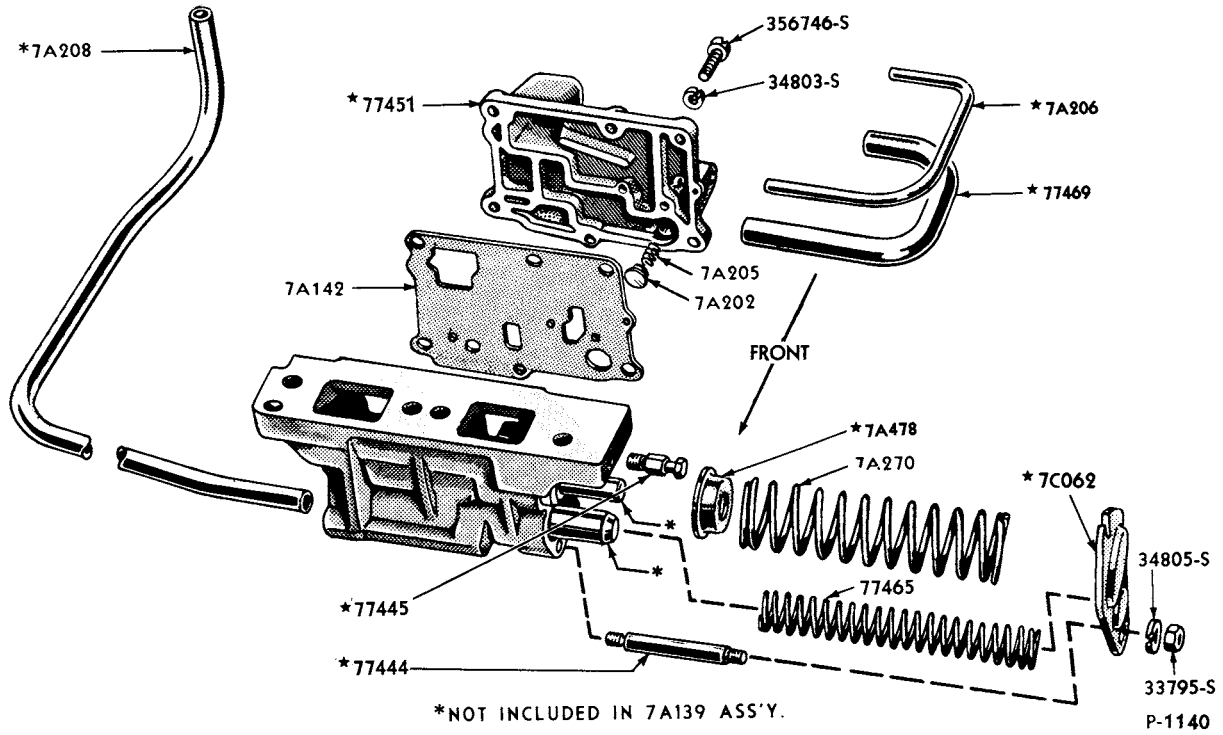
1951/54 OIL PRESSURE REGULATOR (FORDOMATIC TRANSMISSION)
