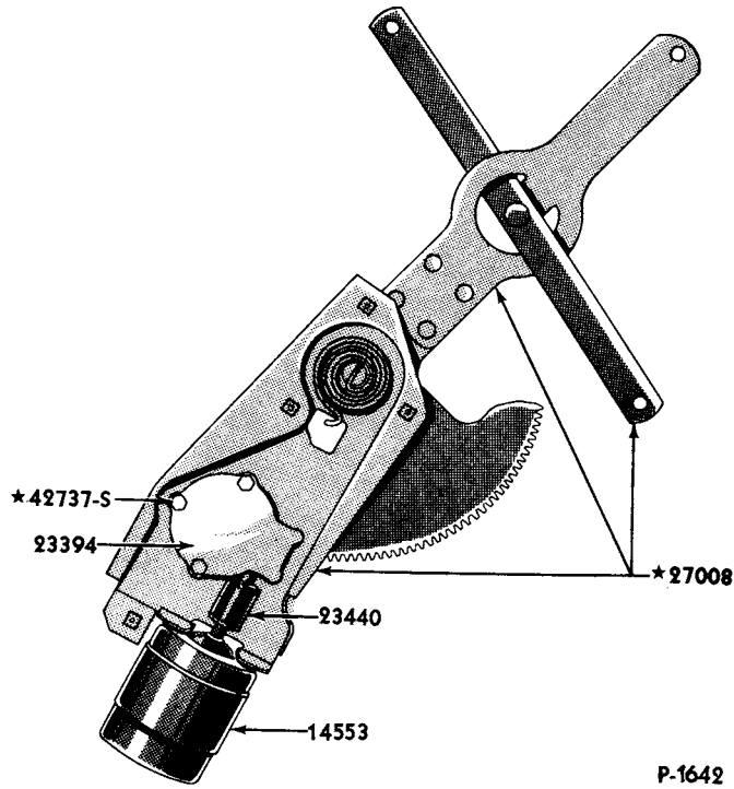
1954 REAR DOOR & QUARTER POWER-LIFT WINDOW REGULATOR
