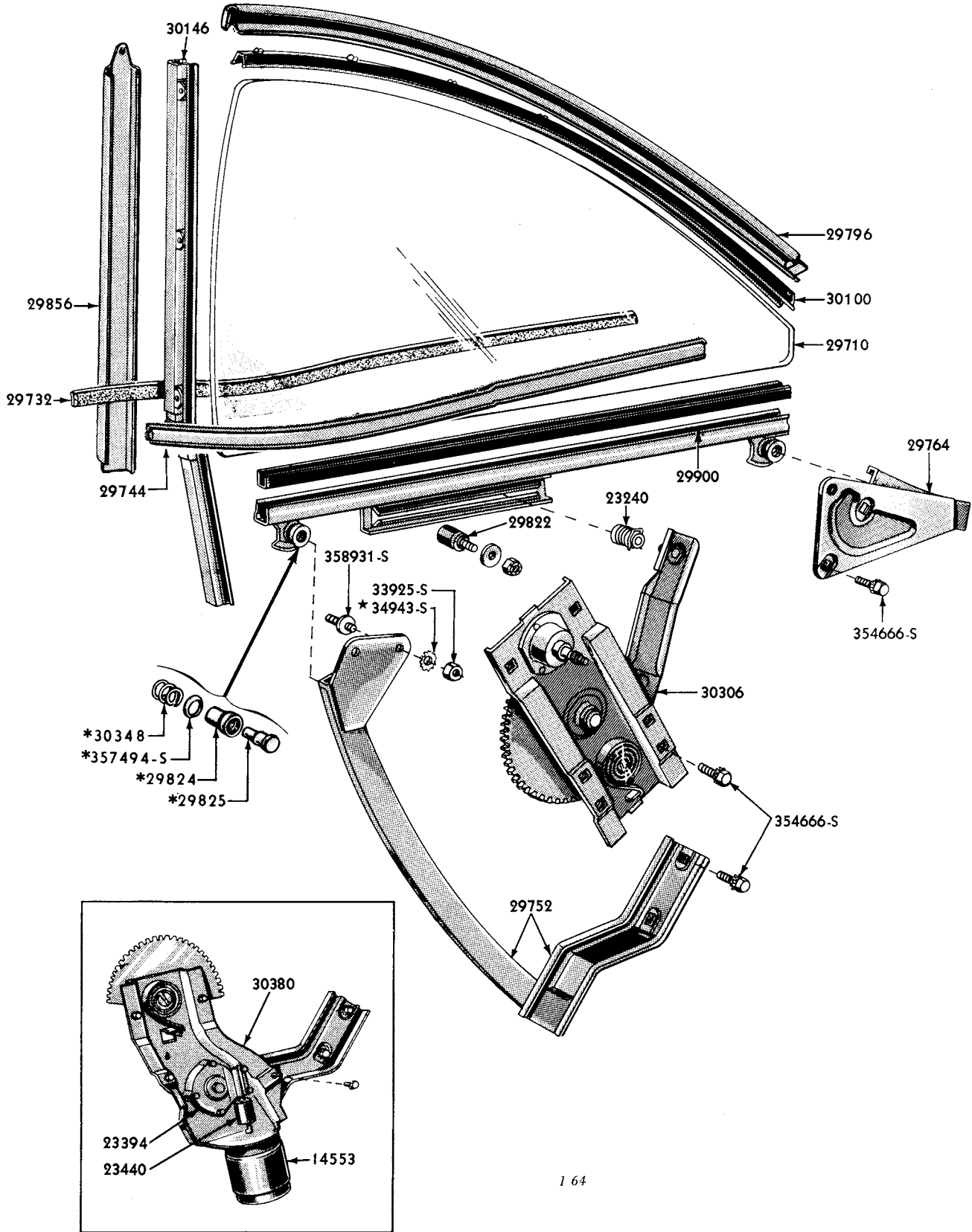
ELECTRIC REGULATOR
