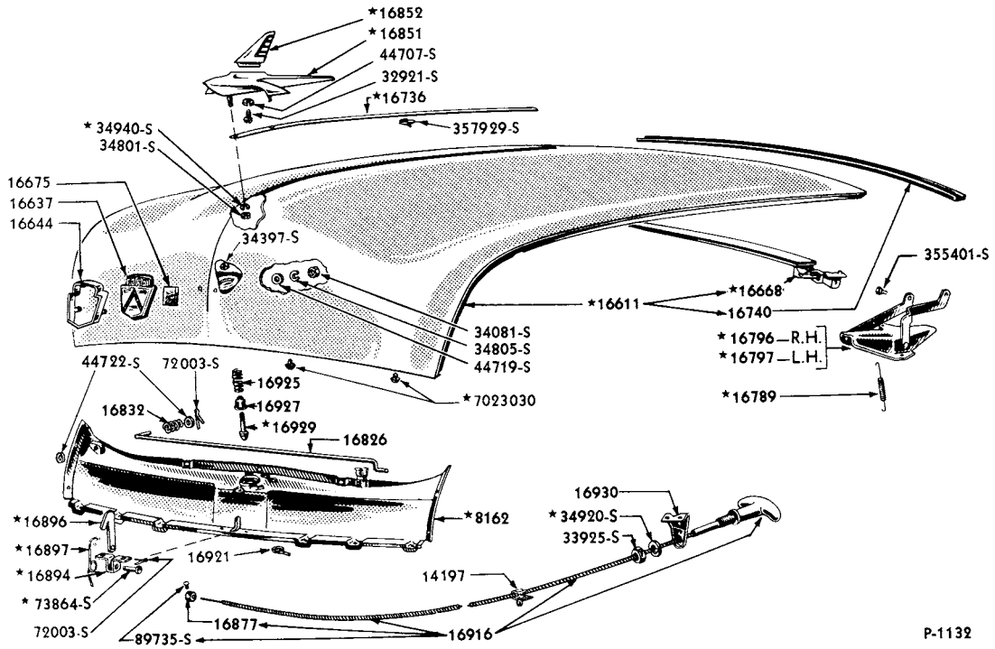
1951 HOOD AND RELATED PARTS
