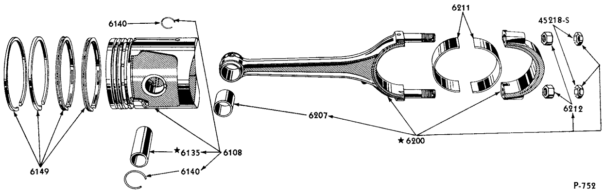
PISTON AND CONNECTING ROD (6 CYLINDER 226 ENGINE)
