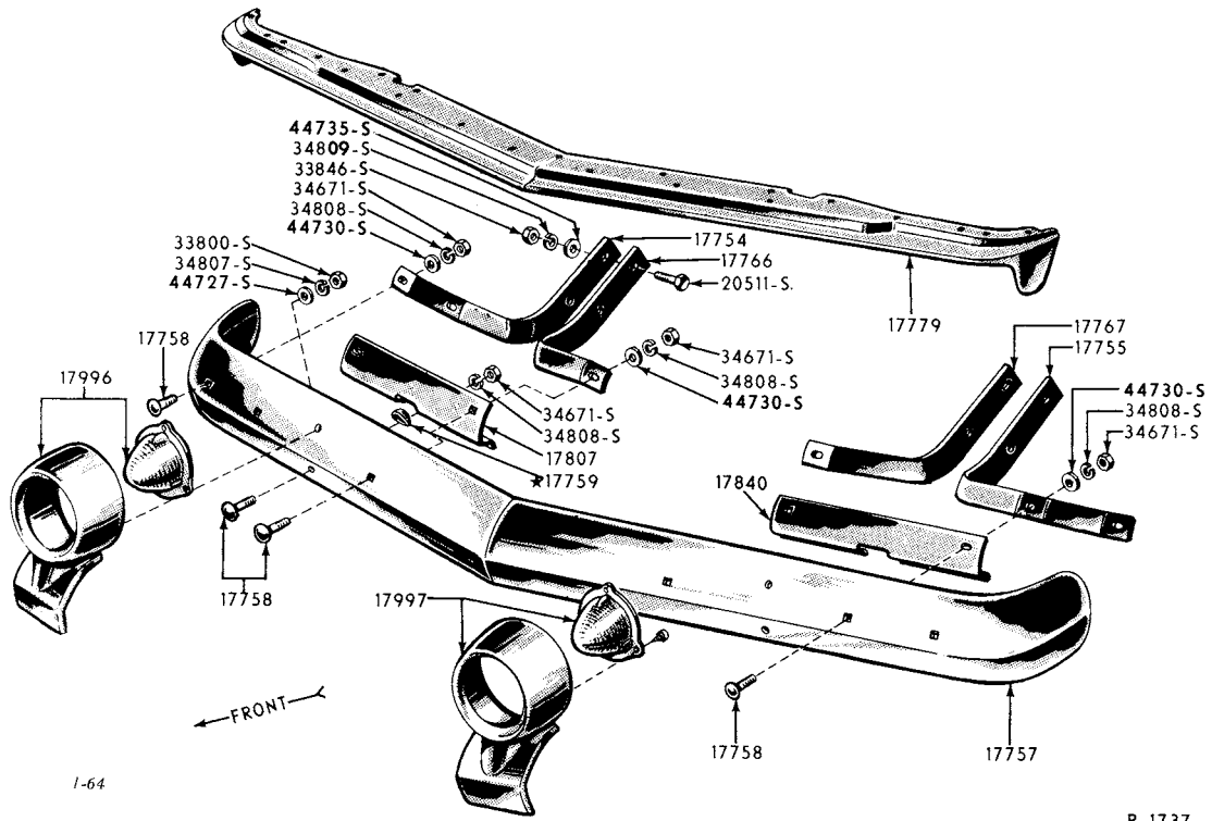
1955/56 FRONT BUMPER (THUNDERBIRD)
