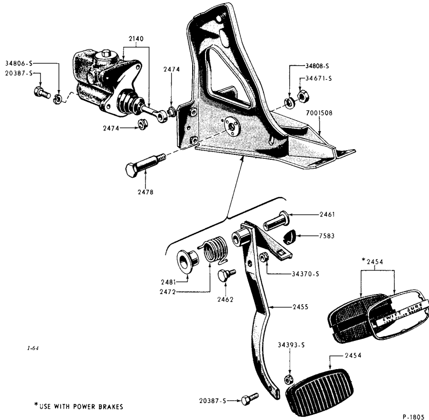
1955/56 BRAKE PEDAL & RELATED PARTS (FORDOMATIC)(FORD)
