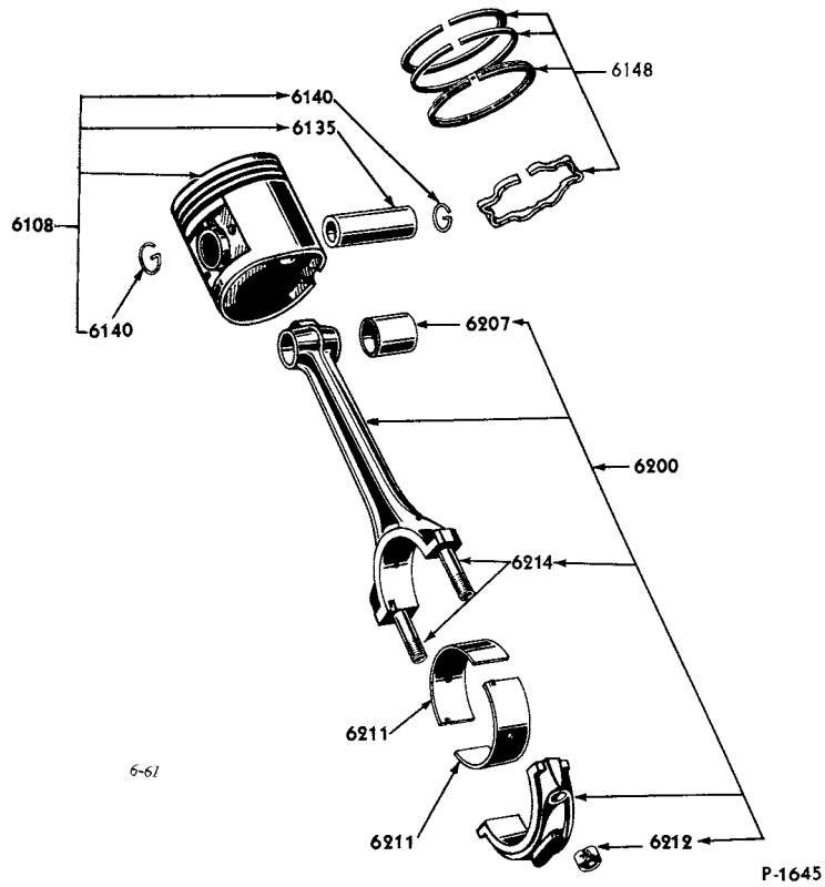
PISTON AND CONNECTING ROD (6 & 8 CYLINDER 215, 223, 239, 272, 292, 312 "O. H. V." ENGINES)-TYPICAL
