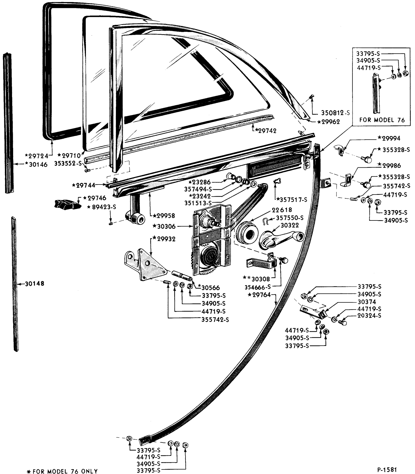
1953/54 QUARTER WINDOW PARTS WITH MANUAL REGULATOR - (BODY TYPES 60, 76)
