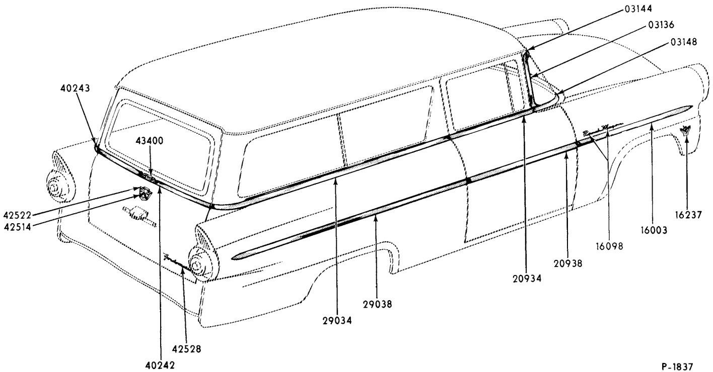
1955 CUSTOMLINE RANCH WAGON (BODY TYPE 59B)
