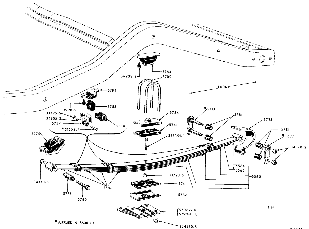
1955/56 REAR SUSPENSION (FORD)
