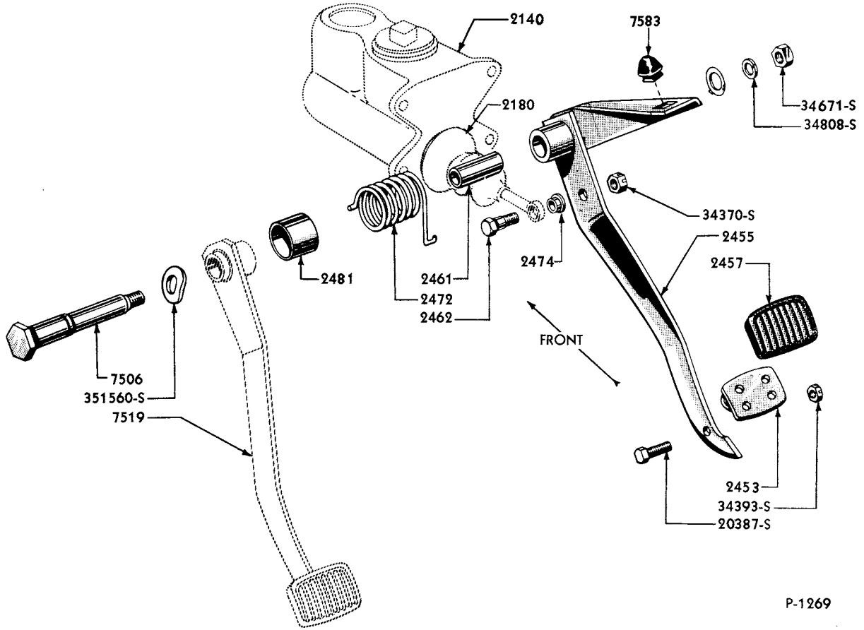
1952/54 BRAKE PEDAL AND RELATED PARTS (MANUAL GEAR SHIFT)
