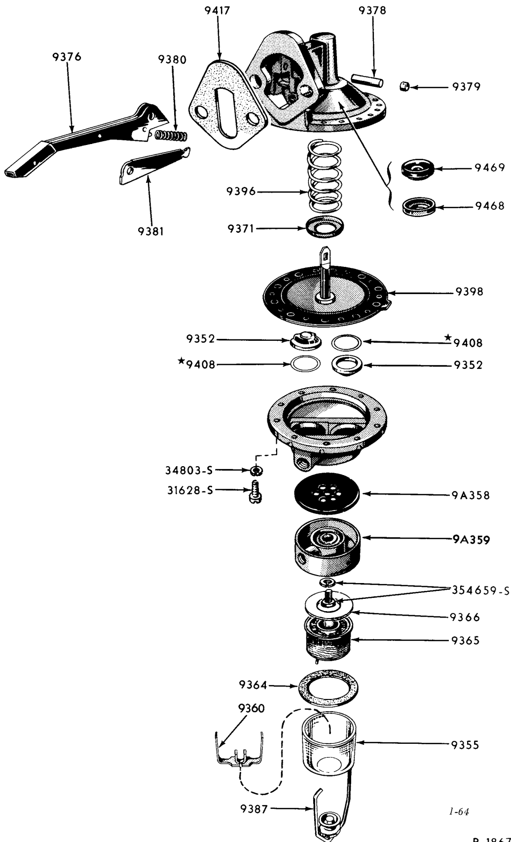
"TYPICAL" FUEL PUMP 1955/ FORD & 1958/ THUNDERBIRD (6 & 8 CYLINDER ENGINES)
