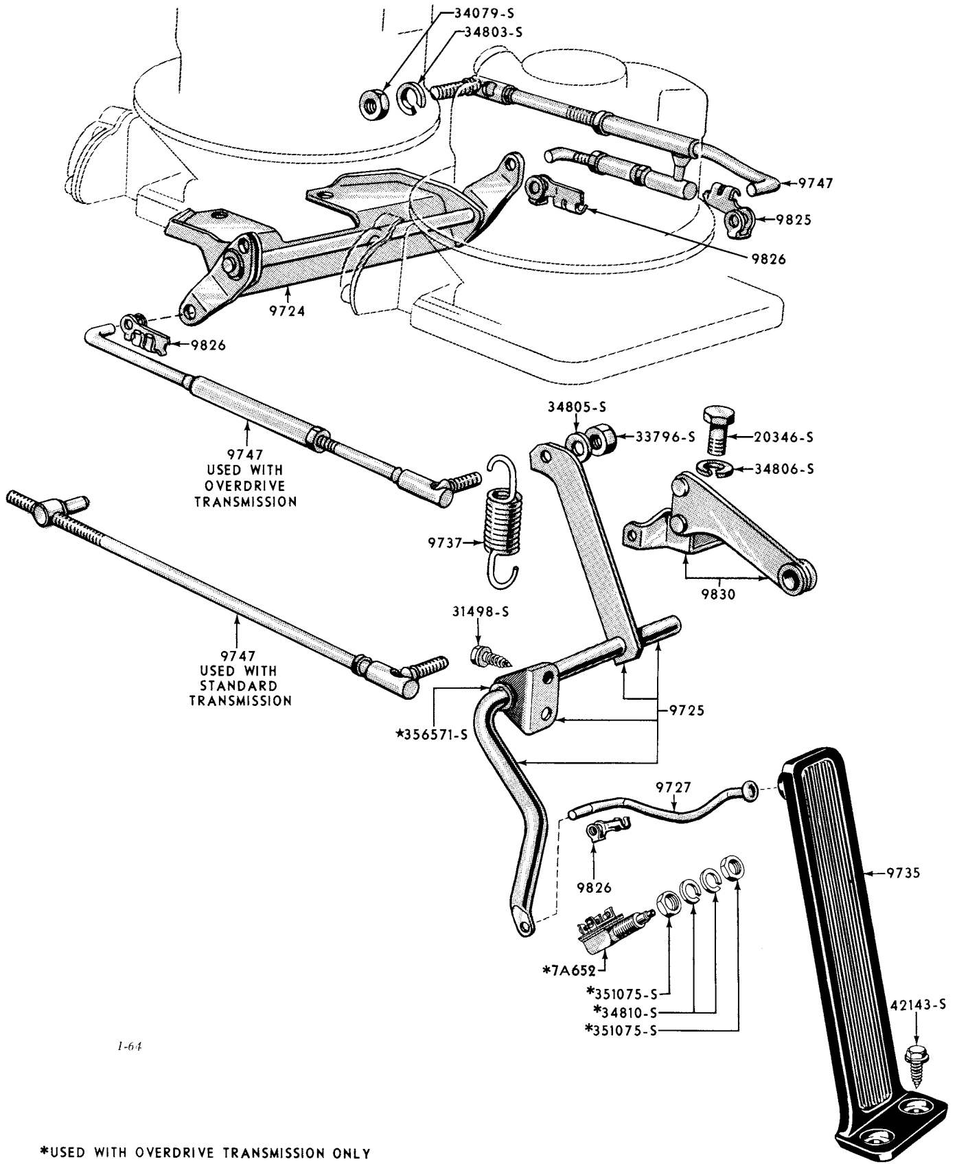
1957 ACCELERATOR LINKAGE - WITH DUAL 4 BARREL CARBURETOR - STANDARD & OVERDRIVE TRANSMISSION (THUNDERBIRD)
