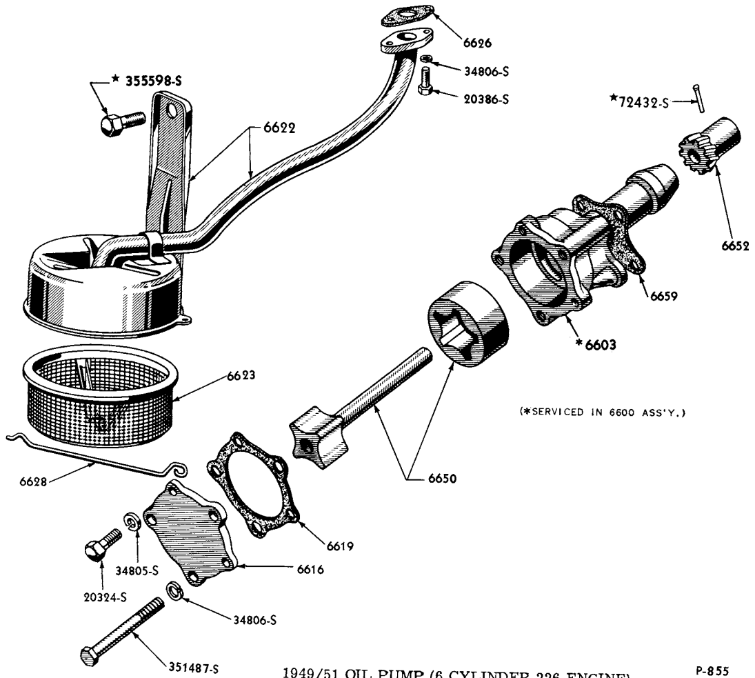
1949/51 OIL PUMP (6 CYLINDER 226 ENGINE)
