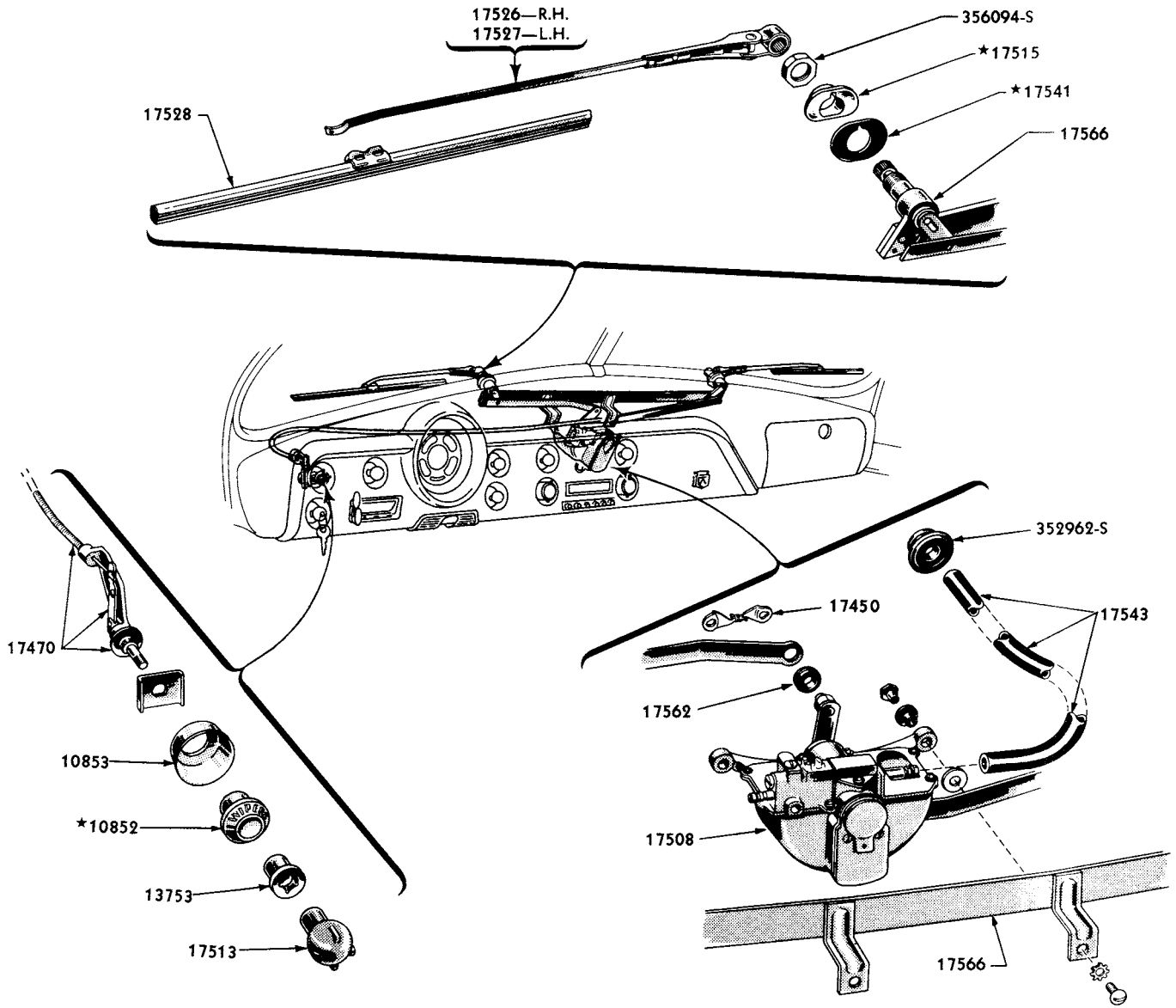
1951 WINDSHIELD WIPER
