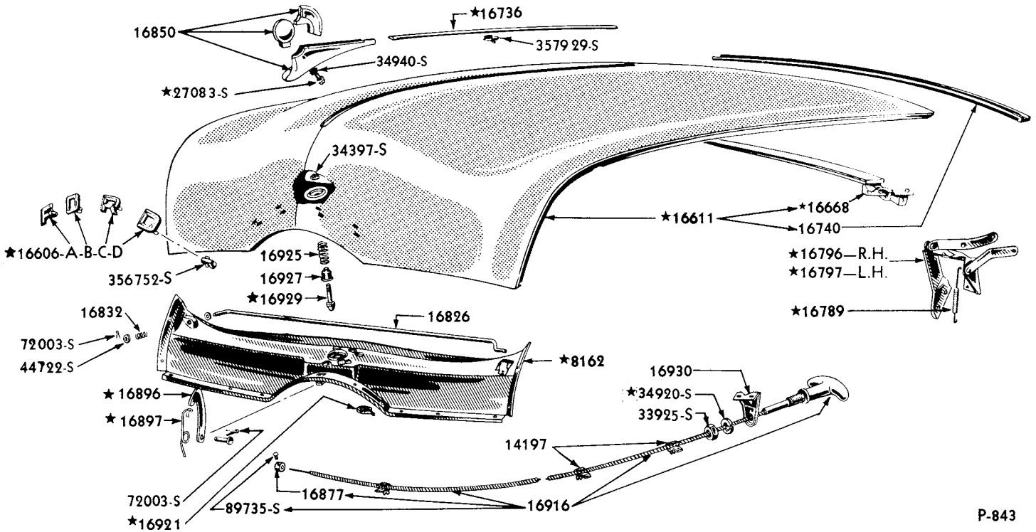
1949 HOOD AND RELATED PARTS
