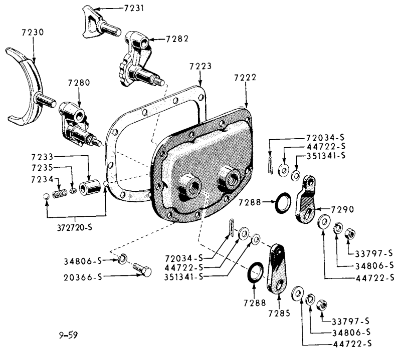
1952/54 GEAR SHIFT HOUSING, LEVERS, FORKS, ETC.
