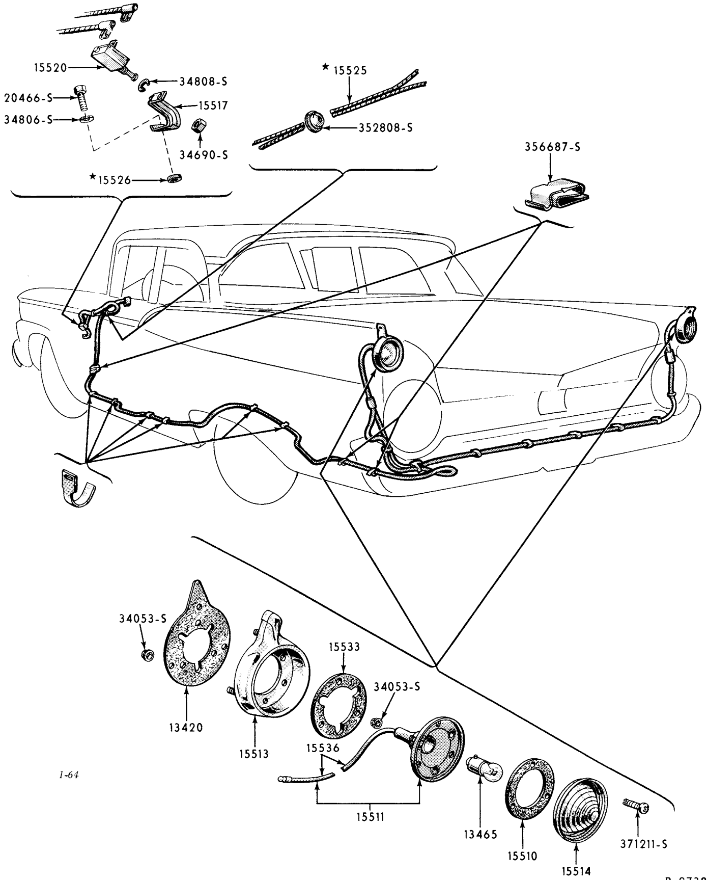
1959 BACK UP LAMP (FORD)
