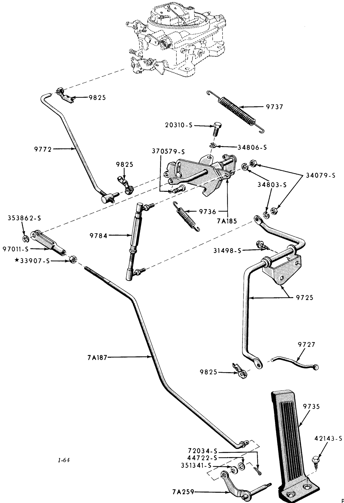
1959/ ACCELERATOR LINKAGE (THUNDERBIRD) (8 CYLINDER 352 & 430 ENGINES) (WITH CRUISE-O-MATIC TRANSMISSION)
