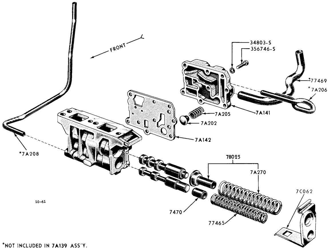
1951/54 OIL PRESSURE REGULATOR (FORDOMATIC TRANSMISSION)
