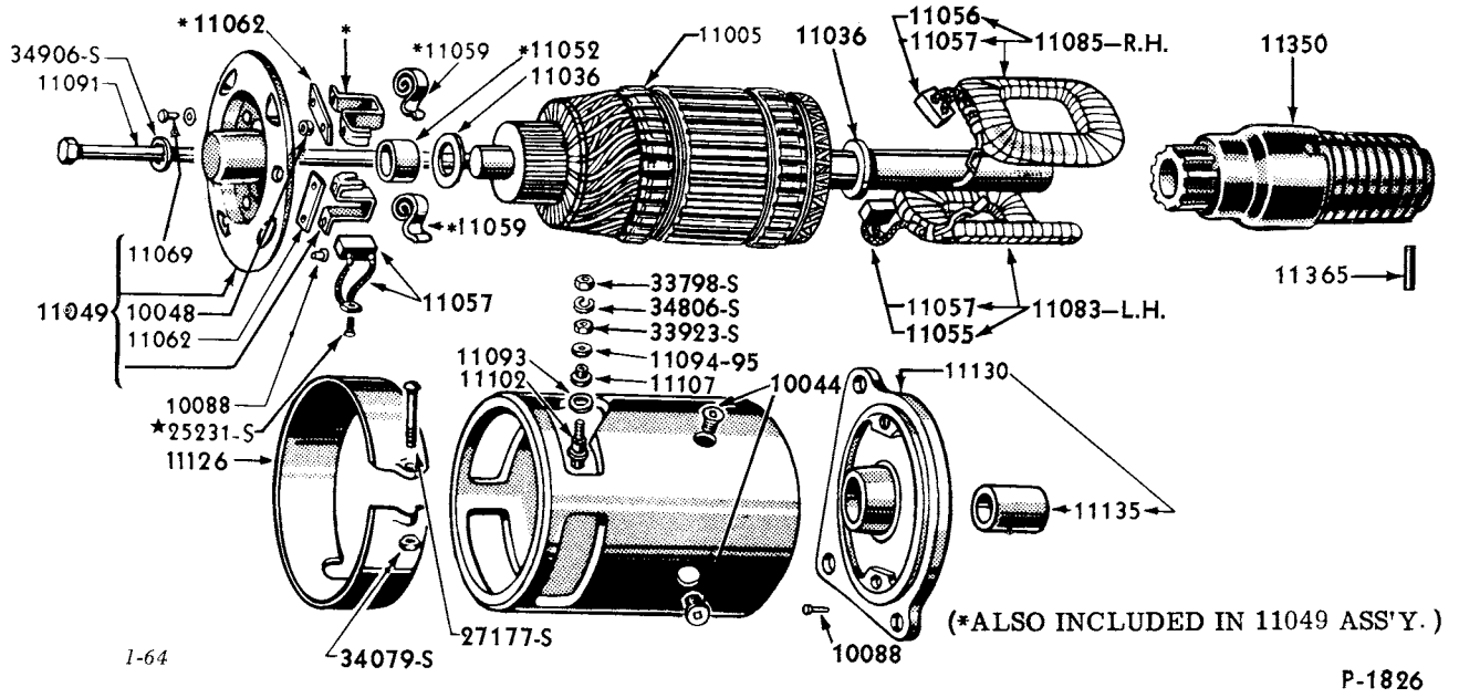
"TYPICAL" STARTER AND STARTER DRIVE (6 VOLT)
