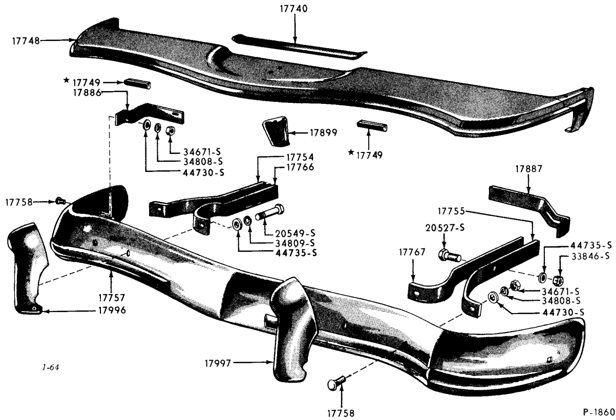
1955/56 FRONT BUMPER (FORD)
