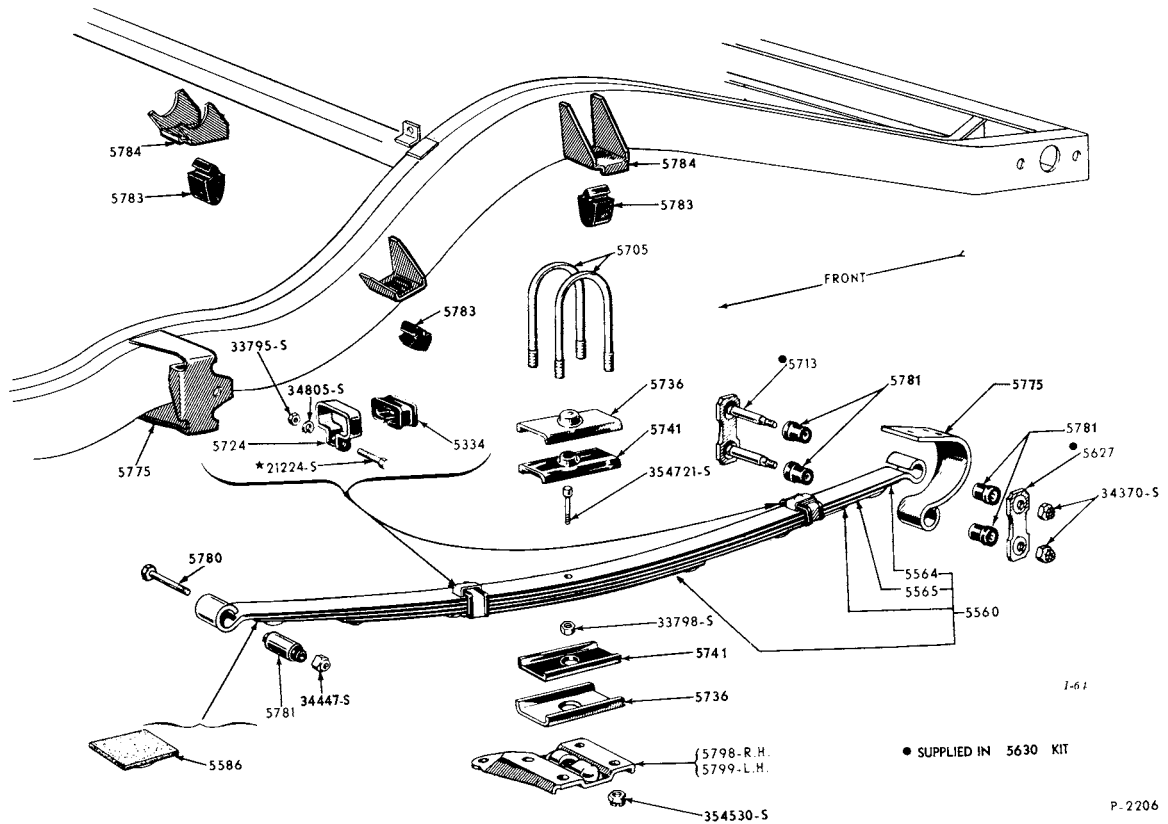
1957/59 REAR SUSPENSION (FORD)
