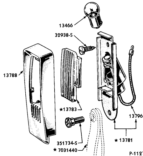
1951 PILLAR LAMP (EXCEPT VICTORIA)
