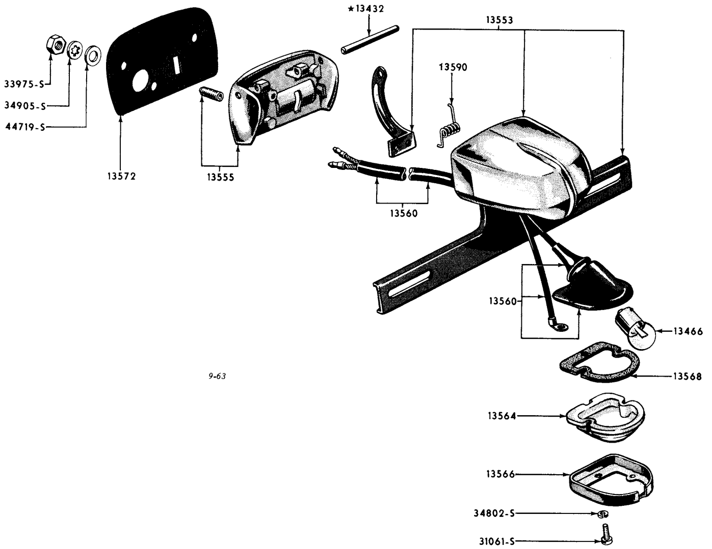
1955/56 STATION WAGON & SEDAN DELIVERY LICENSE PLATE LAMP
