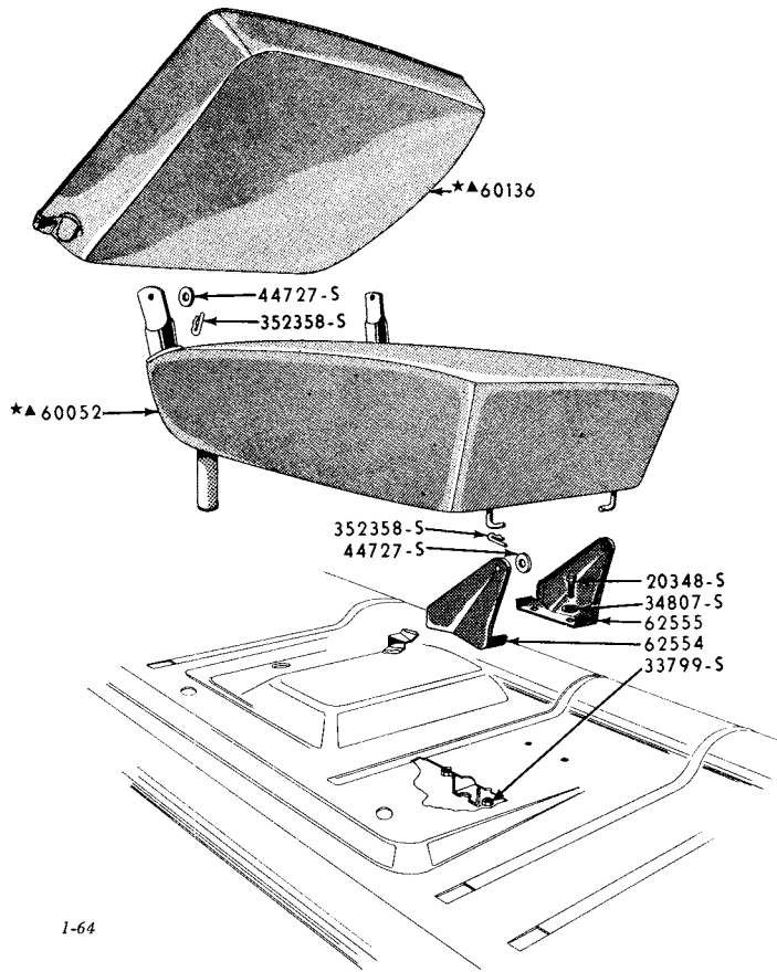
1953/58 TYPICAL PASSENGER'S SEAT (BODY TYPE 78)
