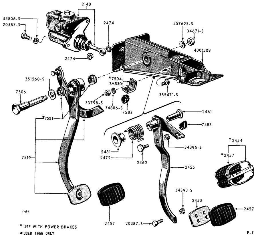
1955/57 BRAKE PEDAL & RELATED PARTS (MANUAL GEAR SHIFT)(THUNDERBIRD)
