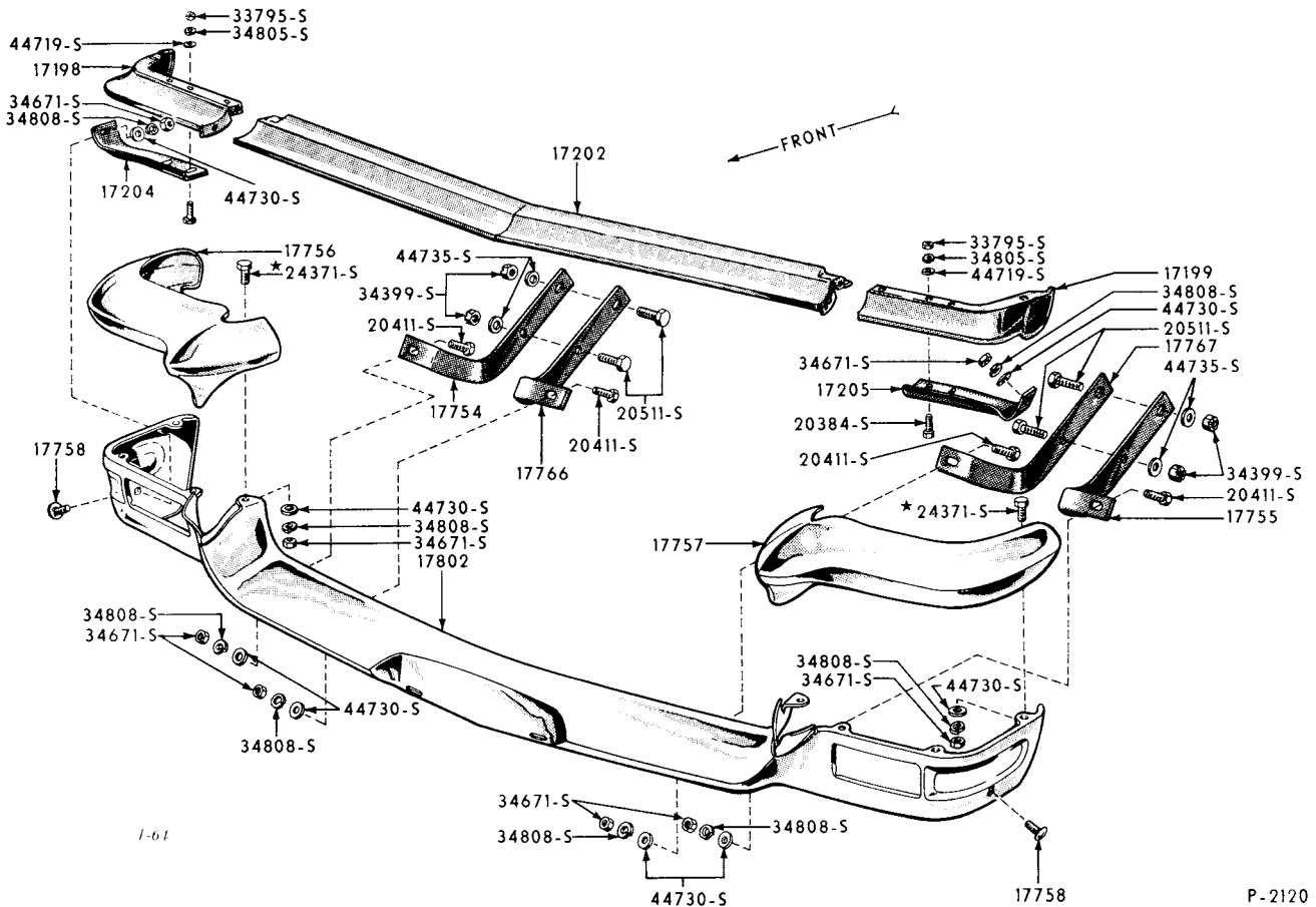
1957 FRONT BUMPER (THUNDERBIRD)
