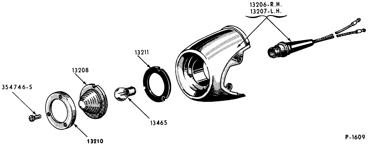
1954 PARKING LAMP
