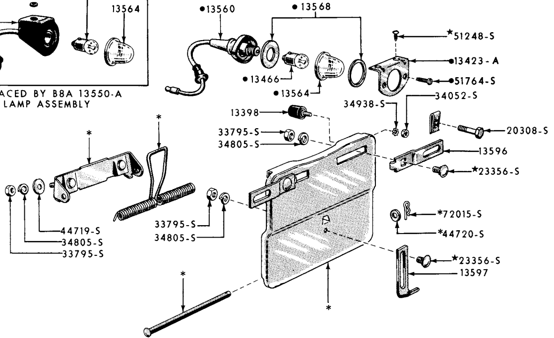
1957/58 LICENSE PLATE LAMP AND SUPPORT (FORD)
