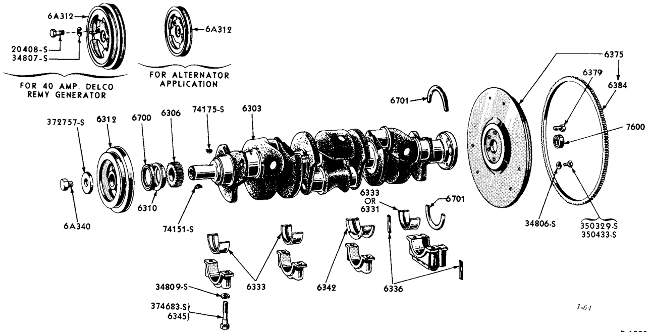
1952/ "TYPICAL" CRANKSHAFT, FLYWHEEL AND RELATED PARTS (6 CYLINDER 215, 223 ENGINES)
