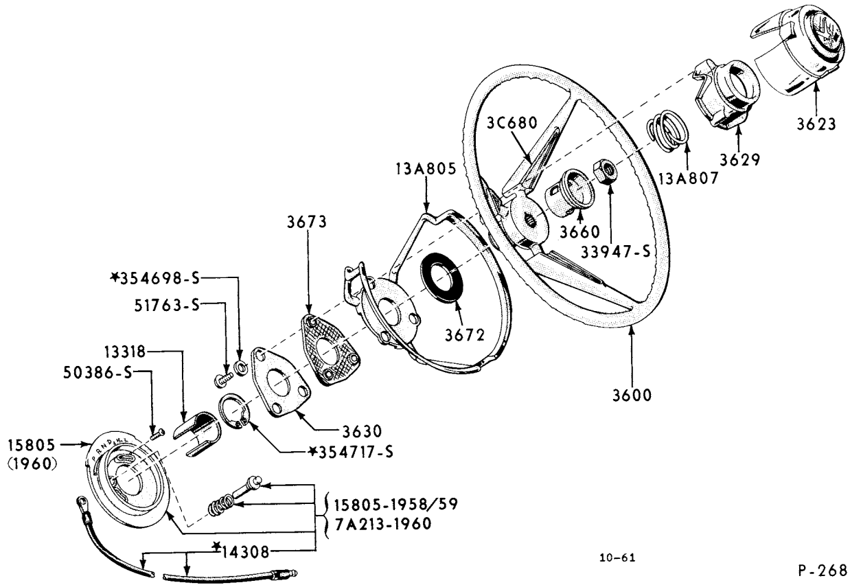
1958/ THUNDERBIRD STEERING WHEEL & HORN RING
