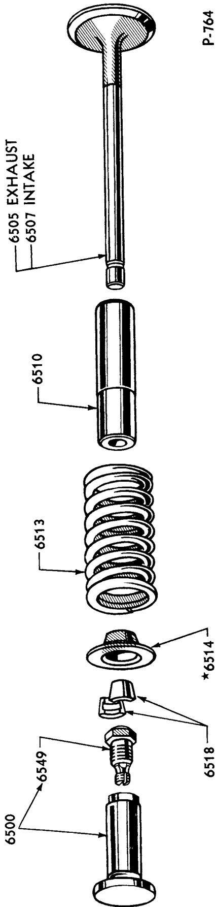
1949/51 VALVE AND RELATED PARTS (6 CYLINDER 226 ENGINE)
