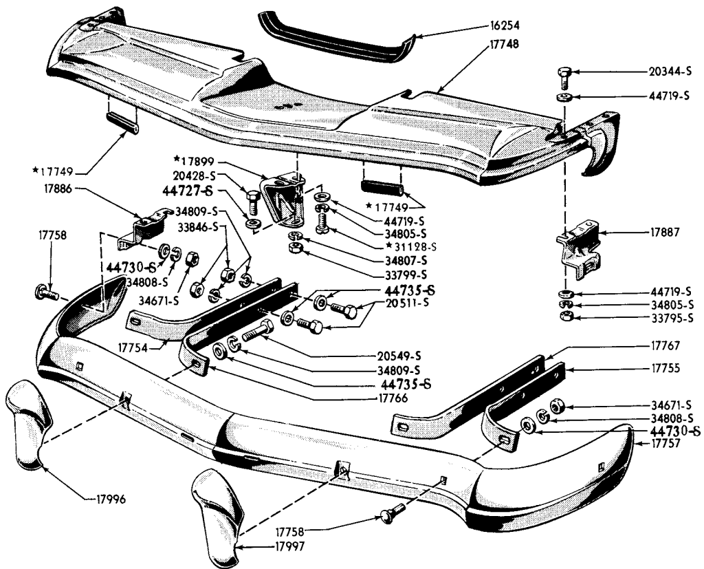
1954 FRONT BUMPER
