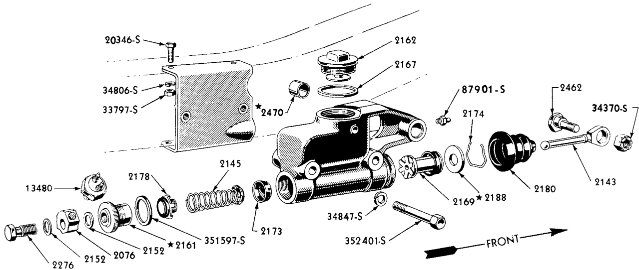
1949/51 BRAKE MASTER CYLINDER
