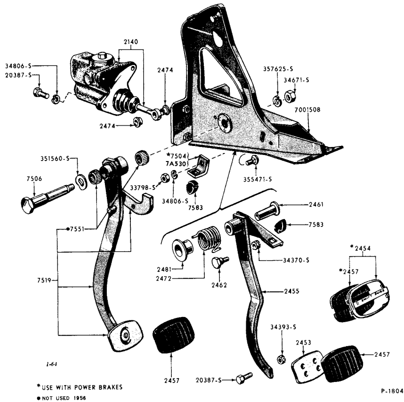
1955/56 BRAKE PEDAL AND RELATED PARTS(MANUAL GEAR SHIFT)(FORD)
