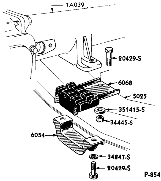
1949/50 6 AND 8 CYLINDER ENGINE REAR SUPPORT
