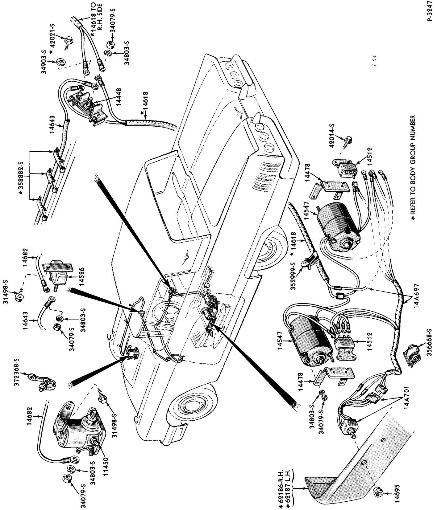
1958/ 4 WAY ELECTRIC SEAT REGULATOR & RELATED PARTS (THUNDERBIRD)
