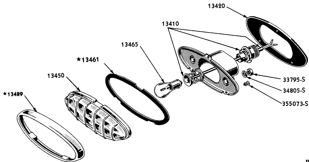
1949/50 REAR LAMP (EXCEPT STATION WAGON)
