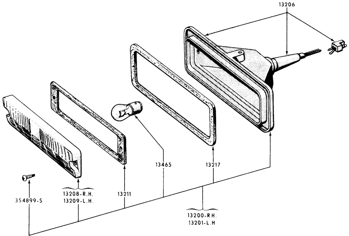
1958/ PARKING LAMP (THUNDERBIRD)
