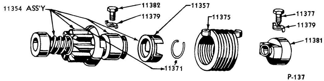
STARTER DRIVE (B 11350)
