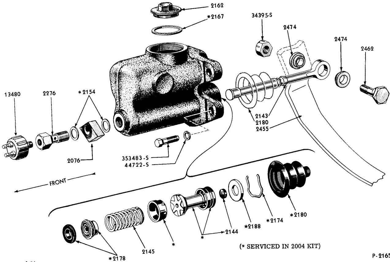
1955/59 BRAKE MASTER CYLINDER ( FORD )
