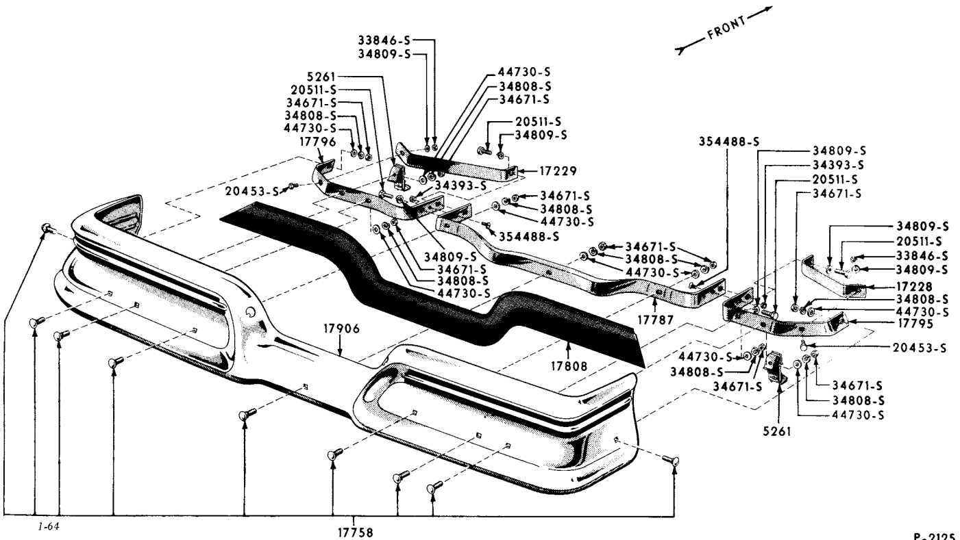
1957 REAR BUMPER (FORD-FAIRLANE-FAIRLANE "500")
