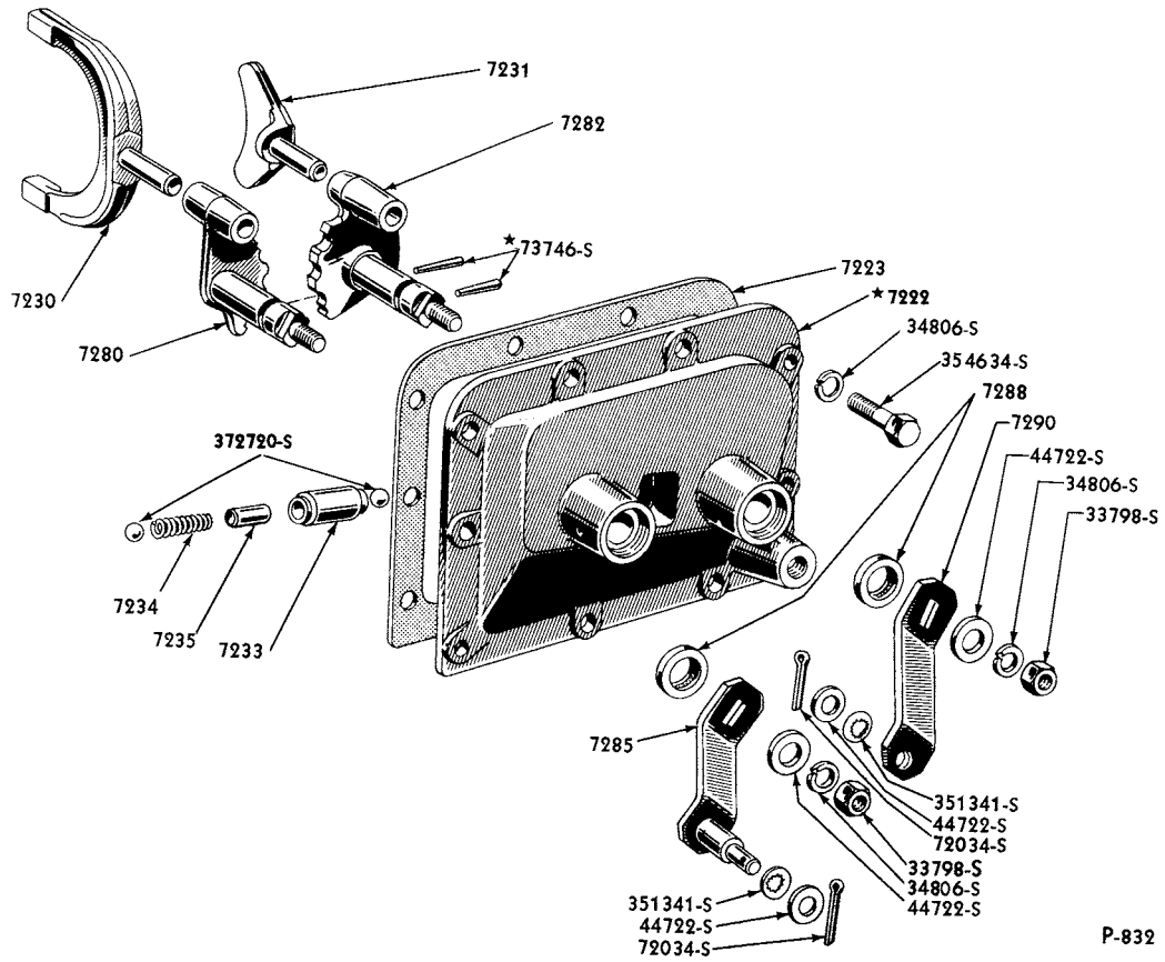
1949/50 GEAR SHIFT HOUSING, LEVERS, FORKS, ETC.
