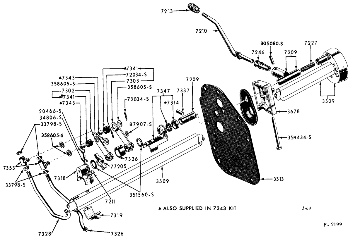
1957 GEAR SHIFT COLUMN (FORD - 6 & 8 CYLINDER ENGINES)
