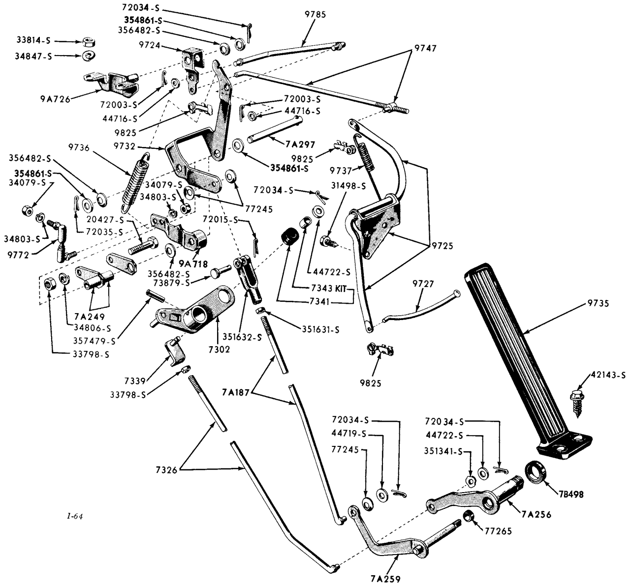
1955/56 "TYPICAL" ACCELERATOR LINKAGE (6 CYLINDER 223 ENGINE)-FORDOMATIC
