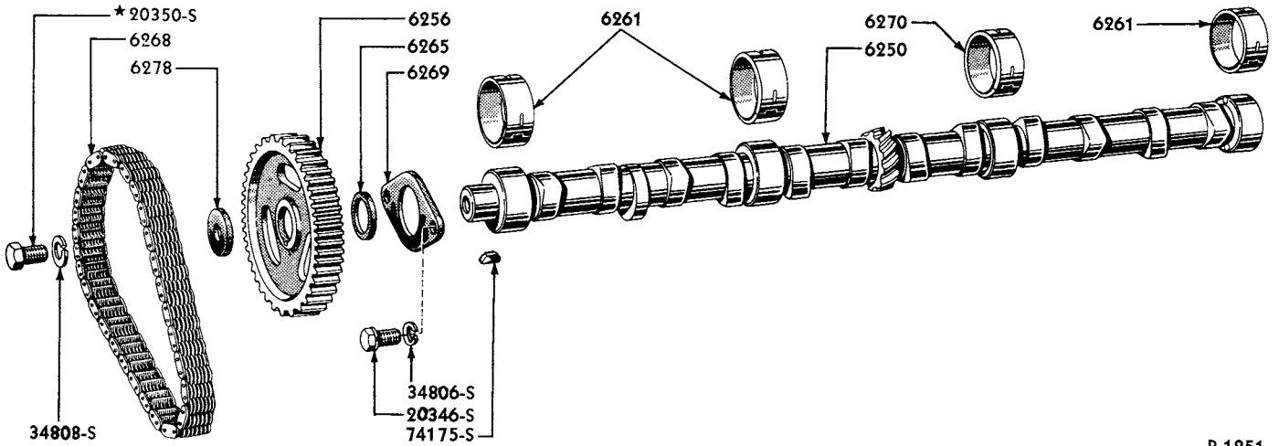
1952/53 CAMSHAFT, GEAR, BEARINGS, ETC. (6 CYLINDER 215 ENGINE)
