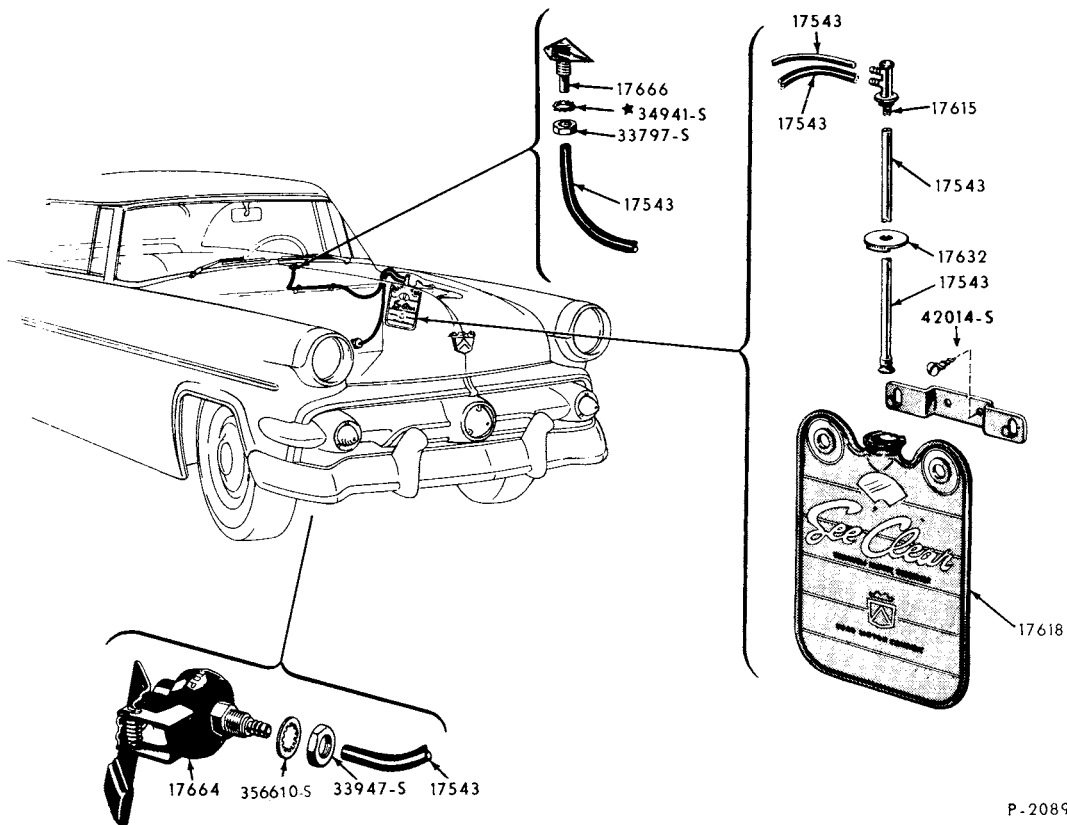
1954 WINDSHIELD WASHER
