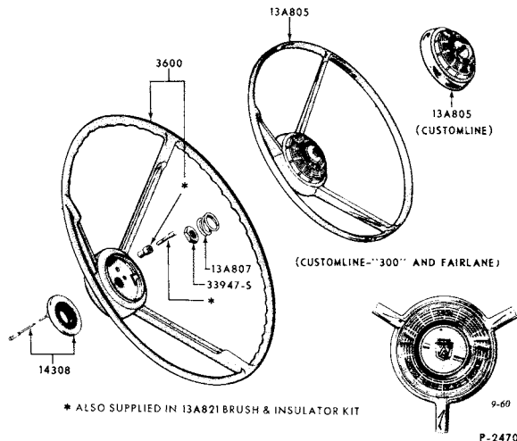
1958 STEERING WHEEL AND HORN RING (FORD)
