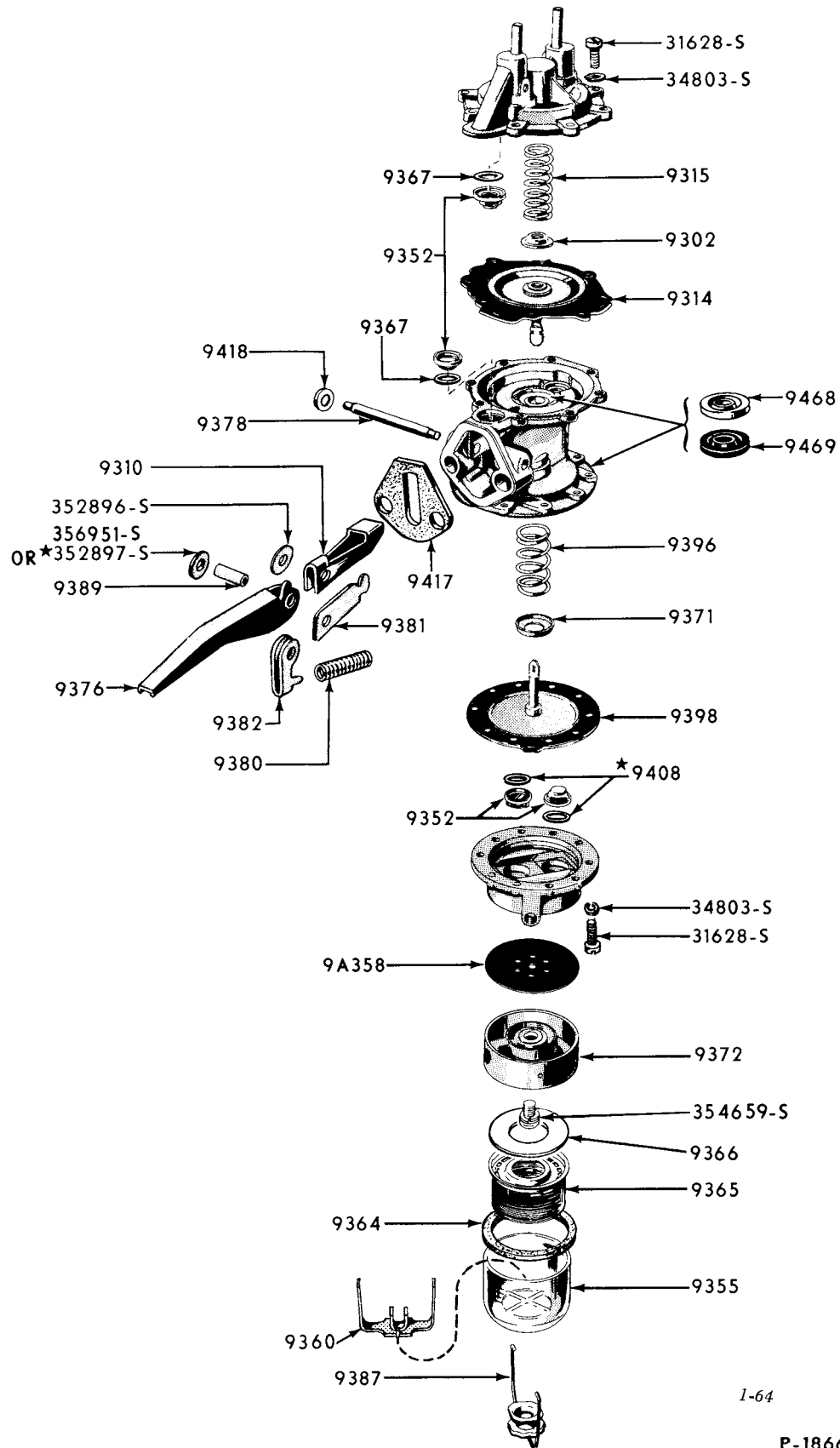
"TYPICAL" FUEL AND VACUUM PUMP 1955/ FORD & 1958/ THUNDERBIRD (6 & 8 CYLINDER ENGINES)
