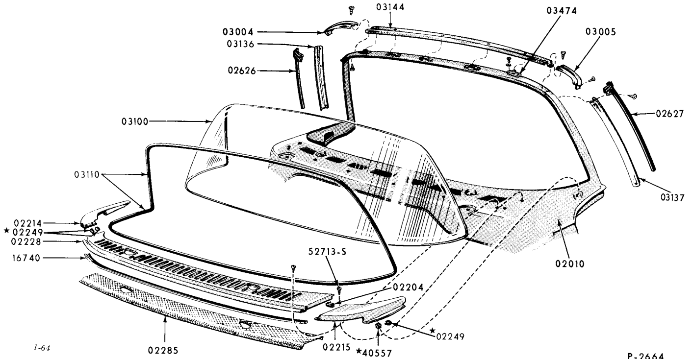
1958/ THUNDERBIRD CONVERTIBLE WINDSHIELD & RELATED PARTS - BODY TYPE S(76A)
