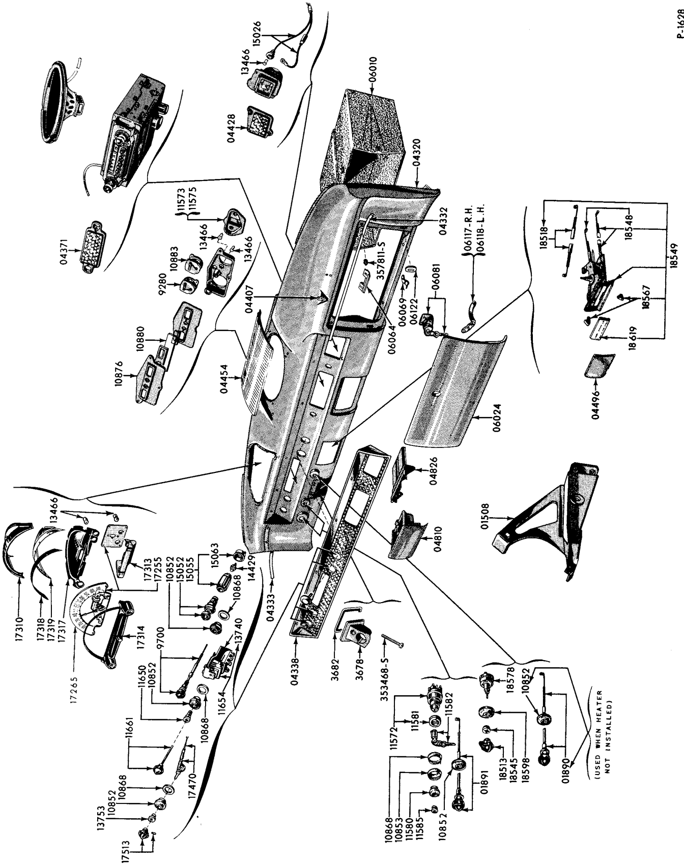
1954 INSTRUMENT PANEL AND RELATED PARTS
