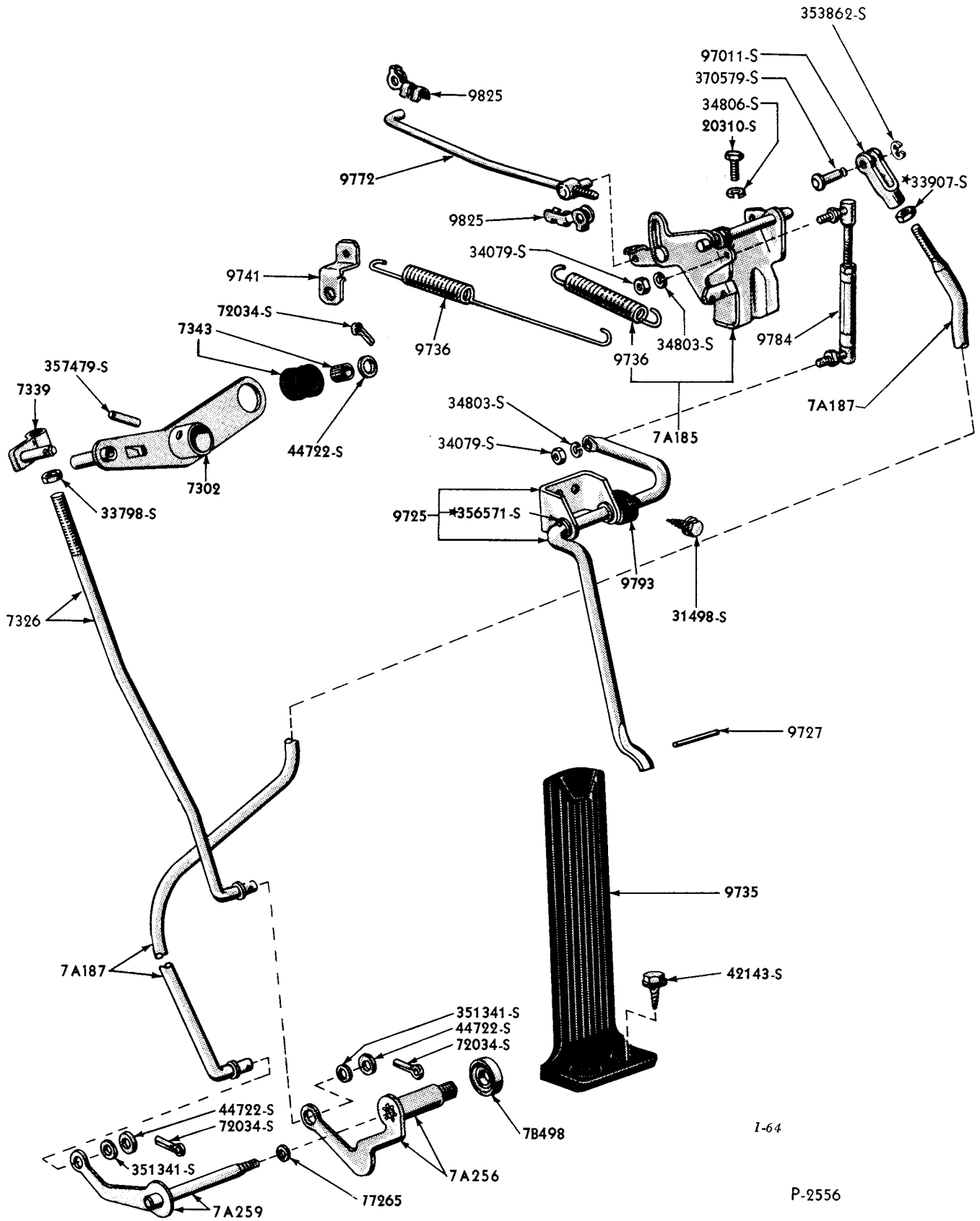
1958 ACCELERATOR LINKAGE (8 CYLINDER 332 & 352 ENGINES)- FORDOMATIC & CRUISE-O-MATIC TRANSMISSION - (FORD)
