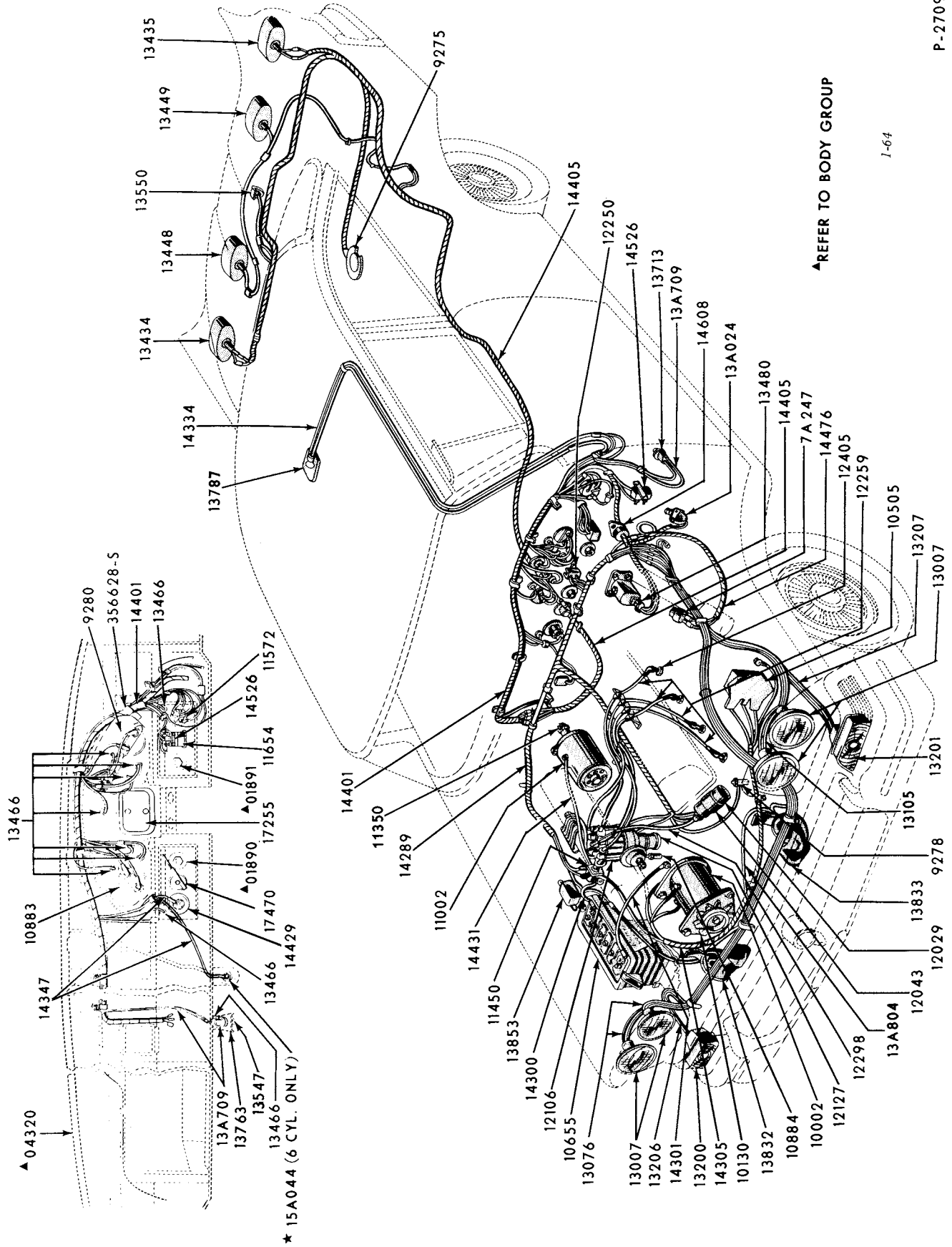
1958 WIRING SYSTEM (FORD)
