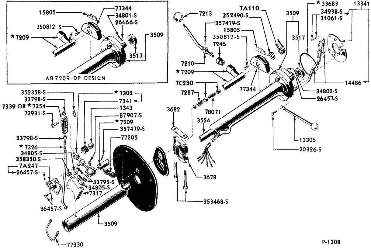
1952/53 GEAR SHIFT COLUMN (FORDOMATIC)
