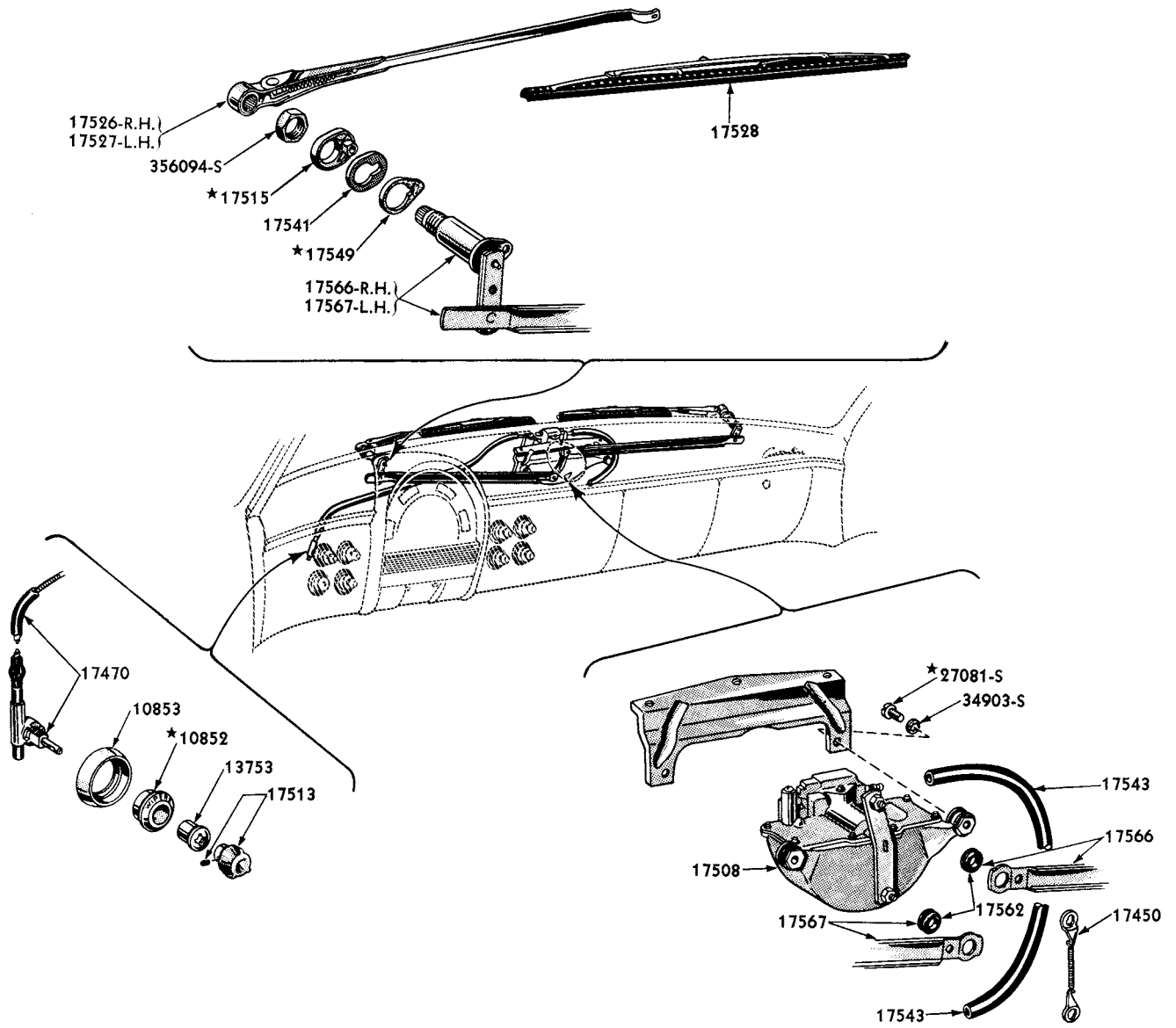
1952/54 WINDSHIELD WIPER
