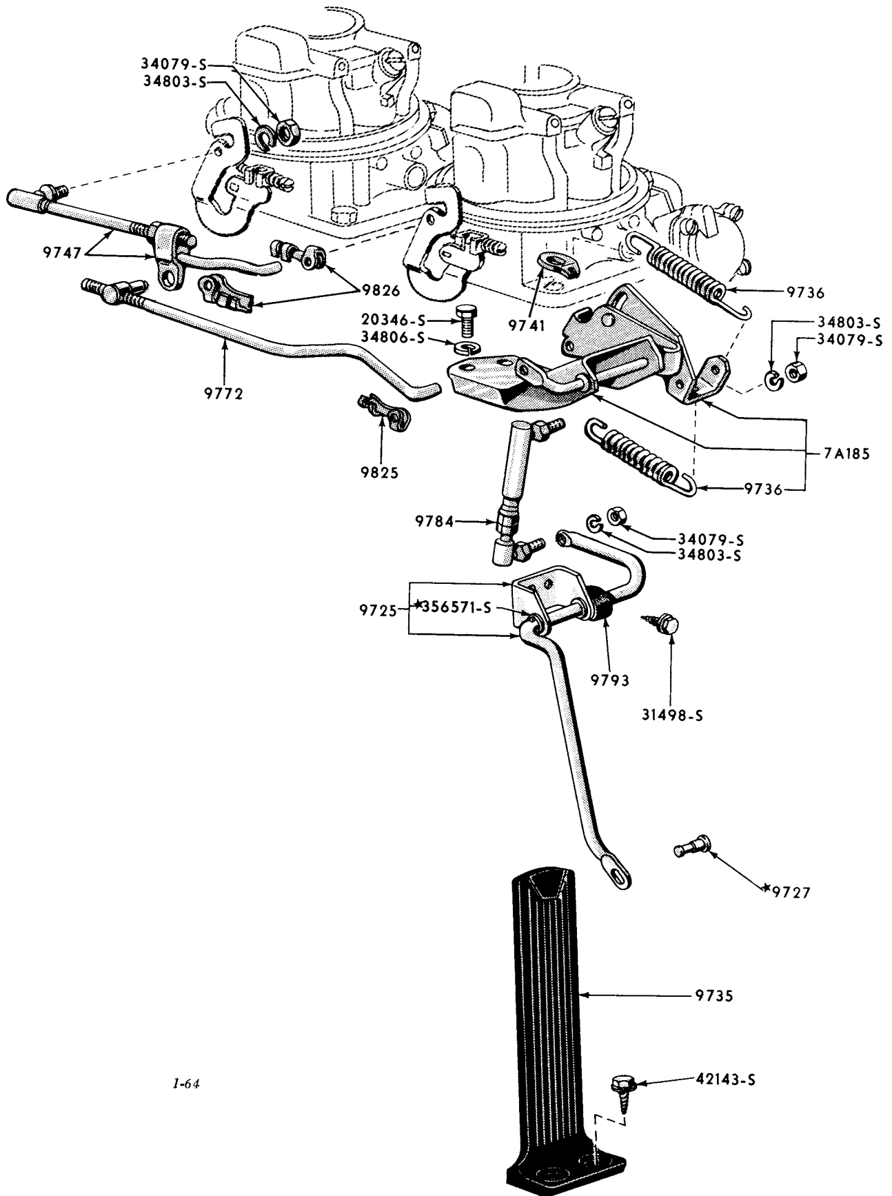
1957 ACCELERATOR LINKAGE - WITH DUAL 4 BARREL CARBURETOR - FORDOMATIC (FORD)
