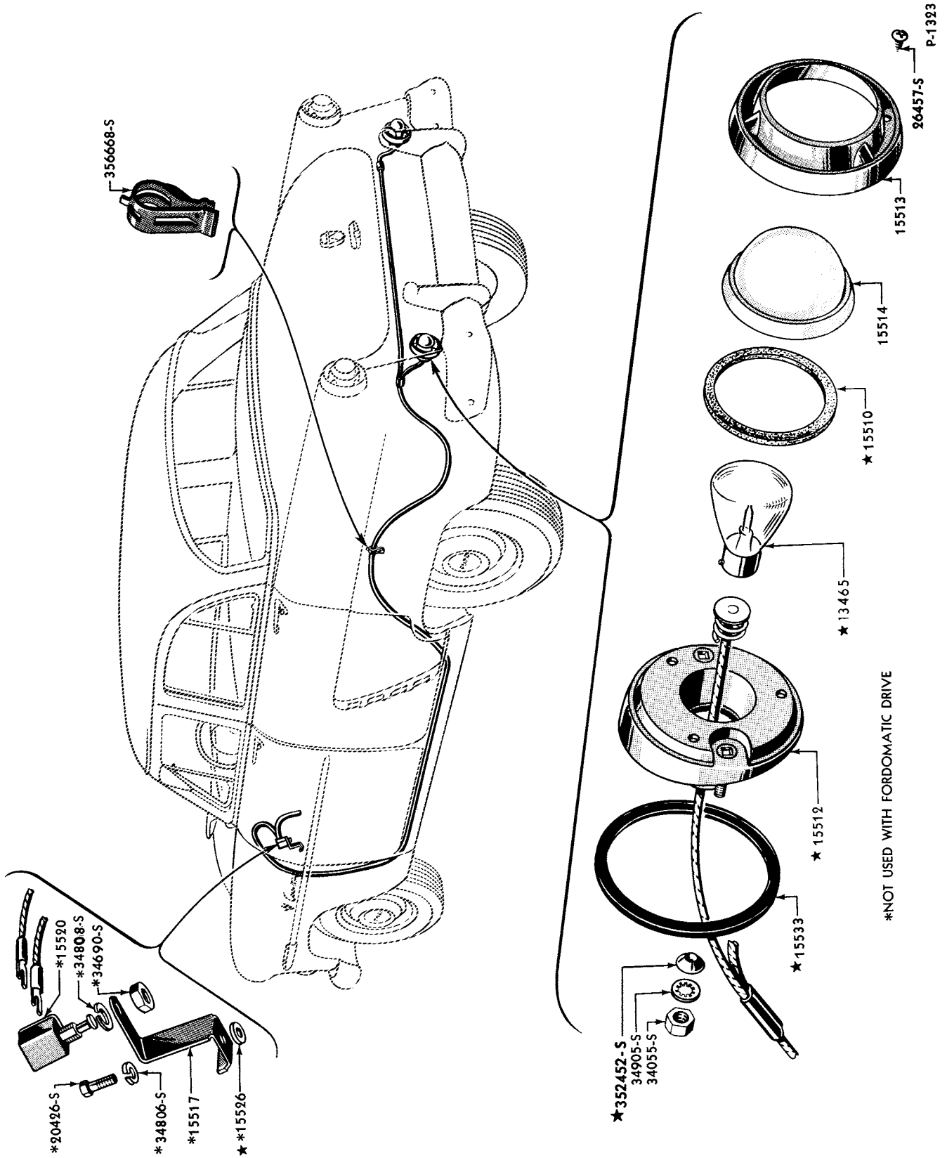
1952/54 BACK UP LAMP (FORD)
