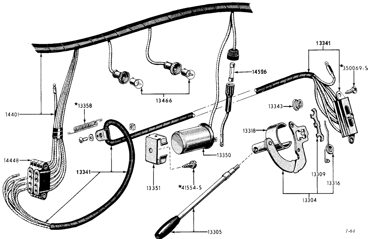
1955/57 "TYPICAL" TURN INDICATOR (THUNDERBIRD)
