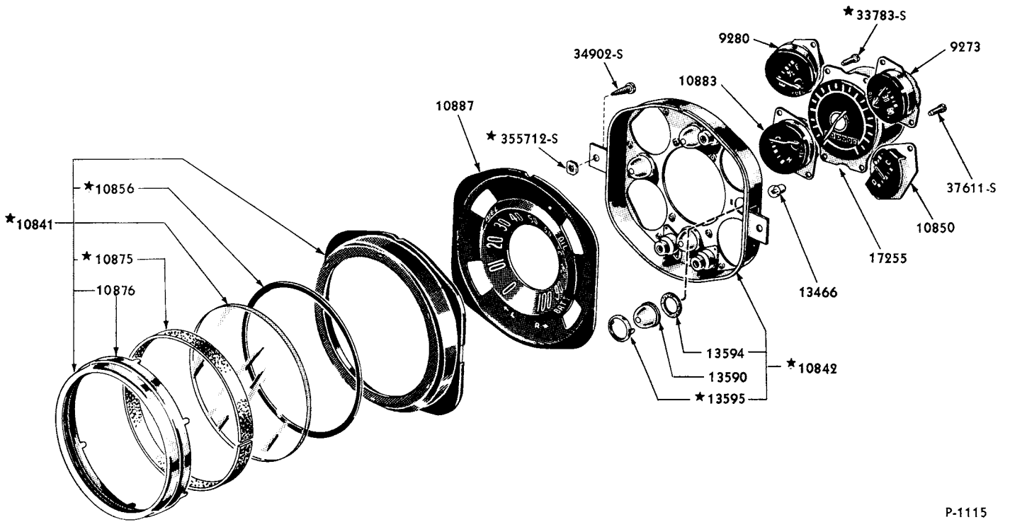
1950 INSTRUMENT PANEL CLUSTER
