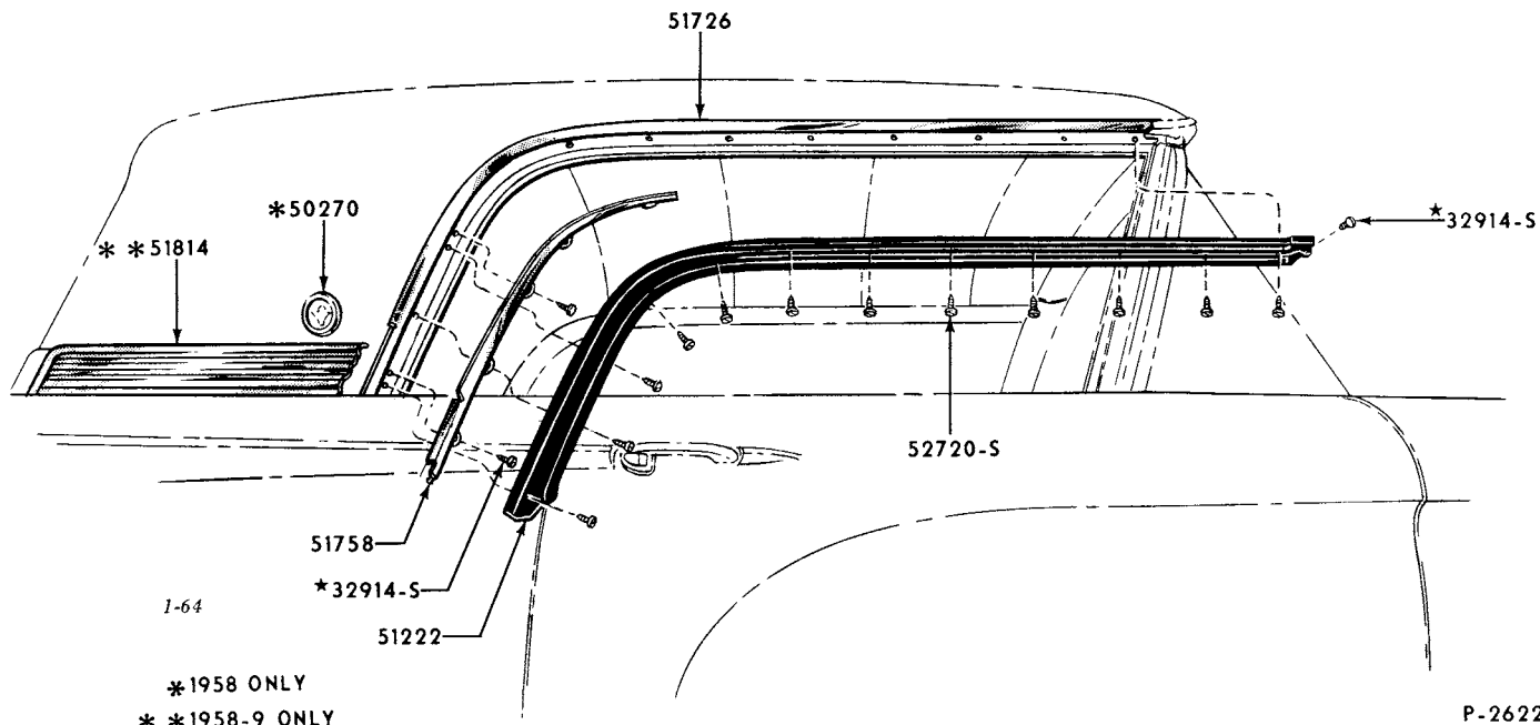
1958/ THUNDERBIRD ROOF SIDE RAIL WEATHERSTRIP & RELATED PARTS-BODY TYPE S(63A)
