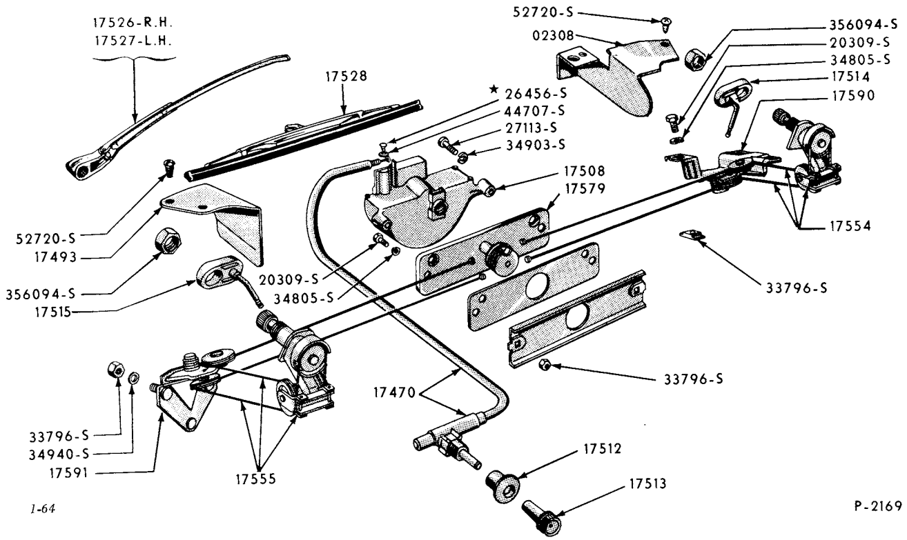
1957 WINDSHIELD WIPER (FORD)
