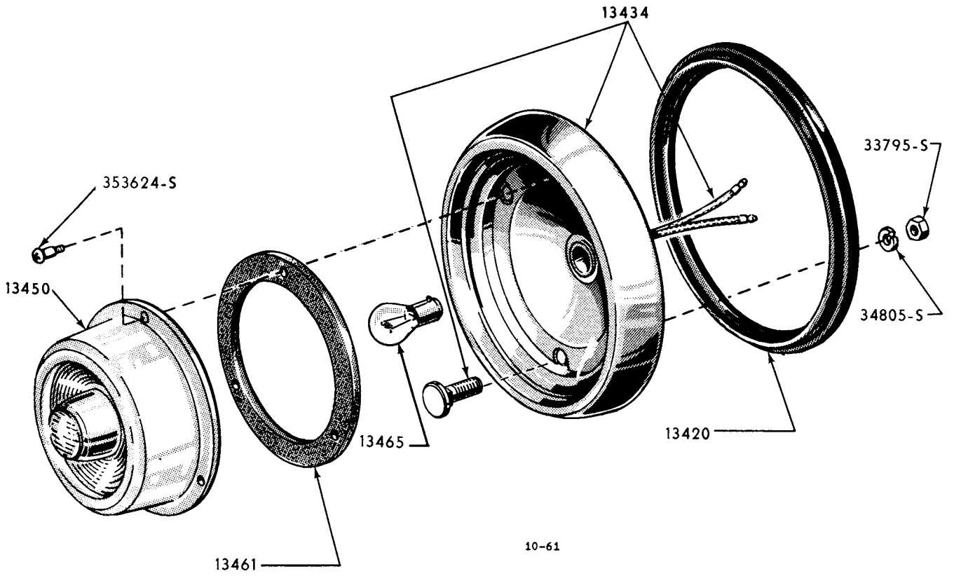
1955 REAR LAMP (FORD)
