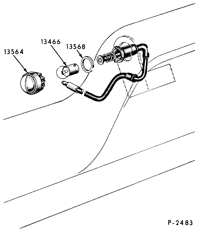
1958 LICENSE PLATE LAMP (51A)
