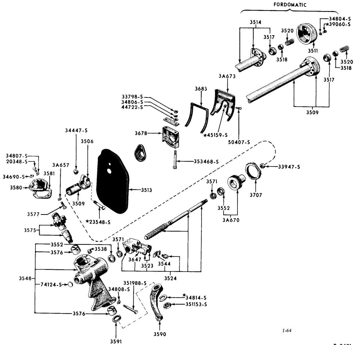
1958 STEERING GEAR (FORD)
