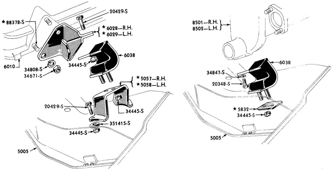
1949/53 ENGINE FRONT SUPPORT 6 CYLINDER 226 ENGINE 8 CYLINDER 239 ENGINE
