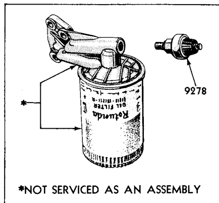
1959/ OIL FILTER AND RELATED PARTS (THUNDERBIRD-8 CYLINDER 430 ENGINE)-TYPICAL
