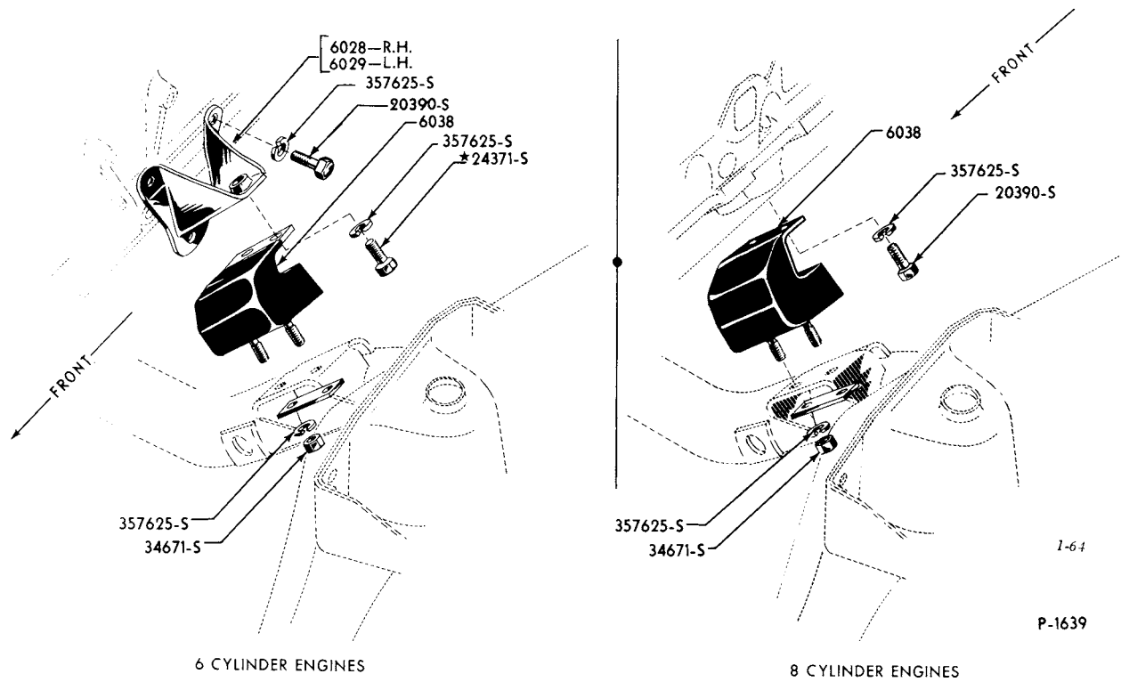
1954/ ENGINE FRONT SUPPORT 6 CYLINDER 223 ENGINE 8 CYLINDER ENGINES - FORD
