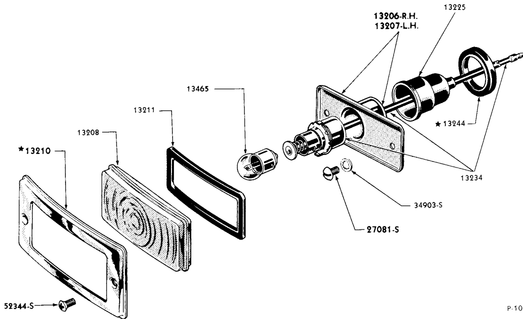
1950 PARKING LAMP
