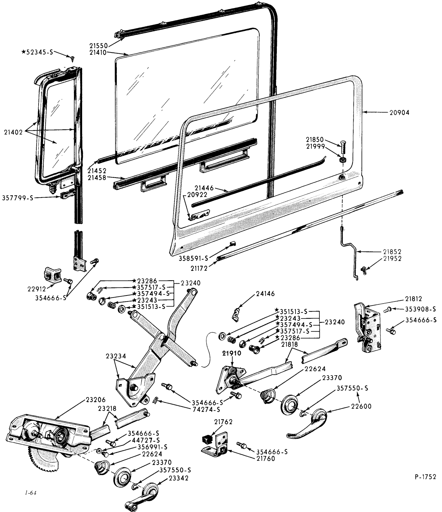
1955/56 TYPICAL FRONT DOOR PARTS (BODY TYPES 59, 70, 73, 78, 79)
