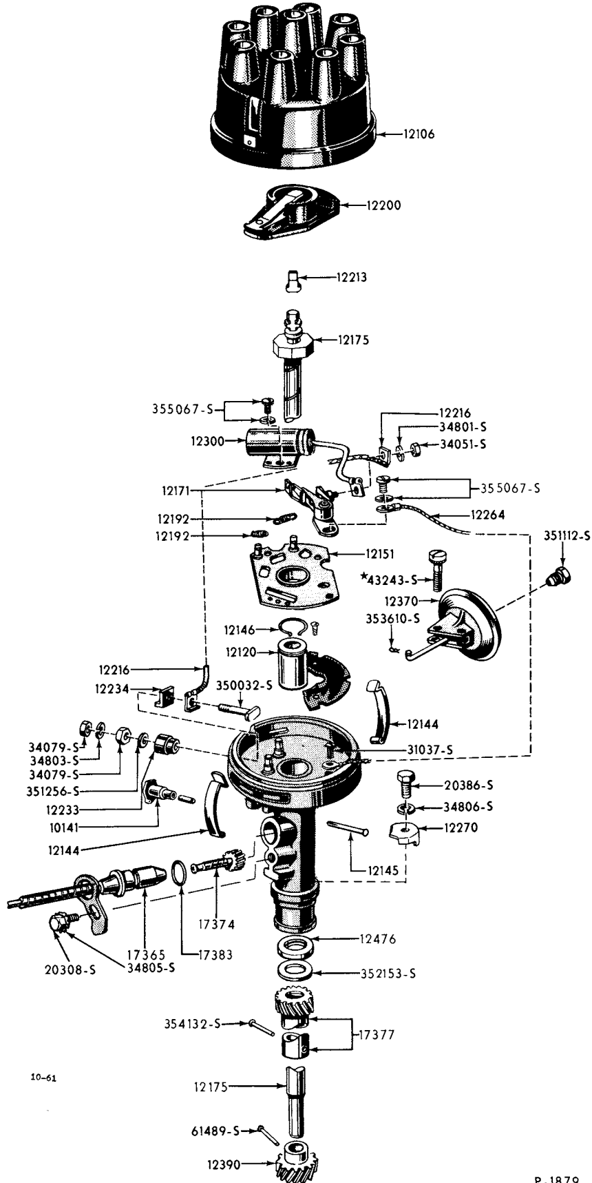
1955/56 "TYPICAL" DISTRIBUTOR (8 CYLINDER ENGINE)-THUNDERBIRD
