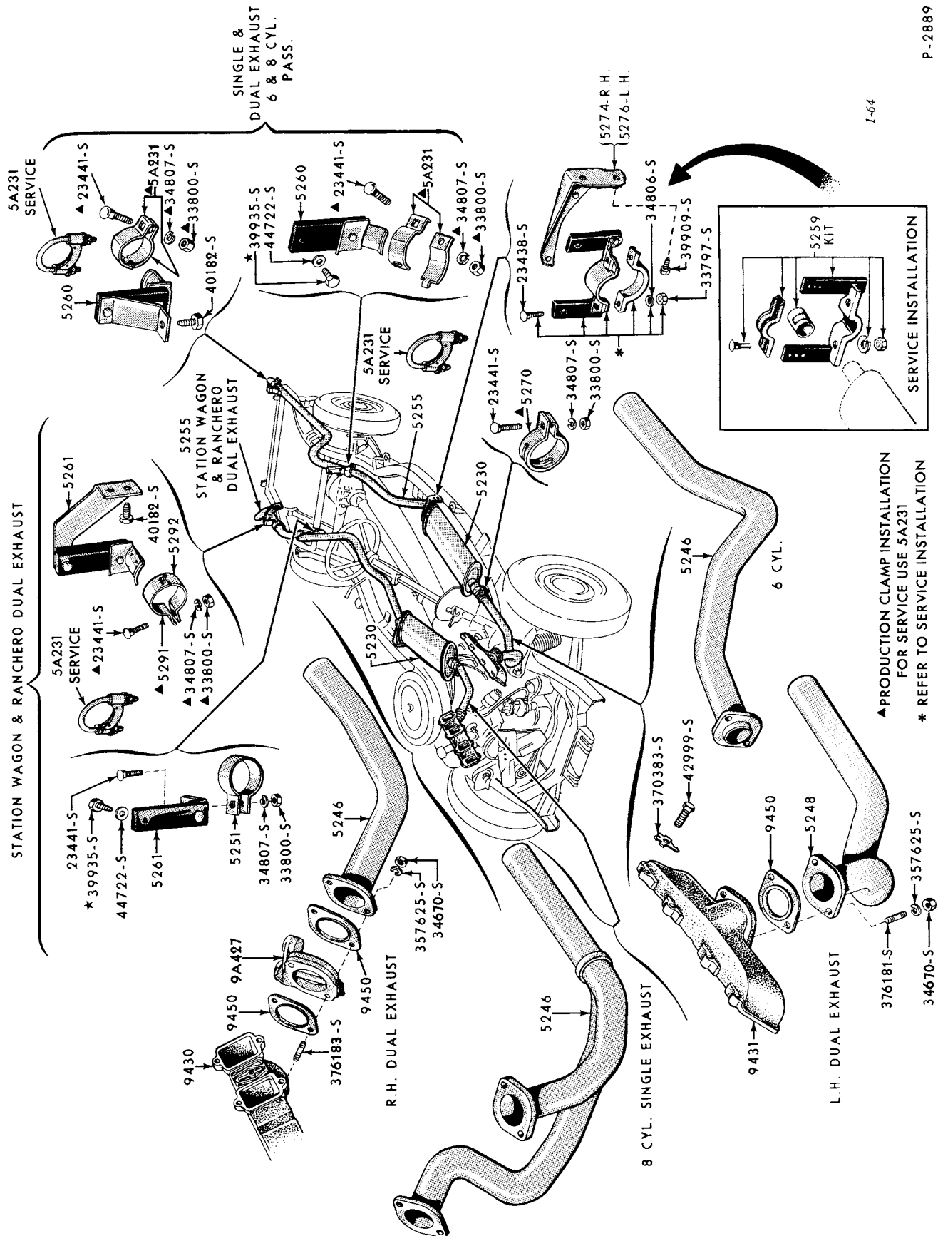
1959 EXHAUST SYSTEM (FORD)-BOX TYPE FRAME
