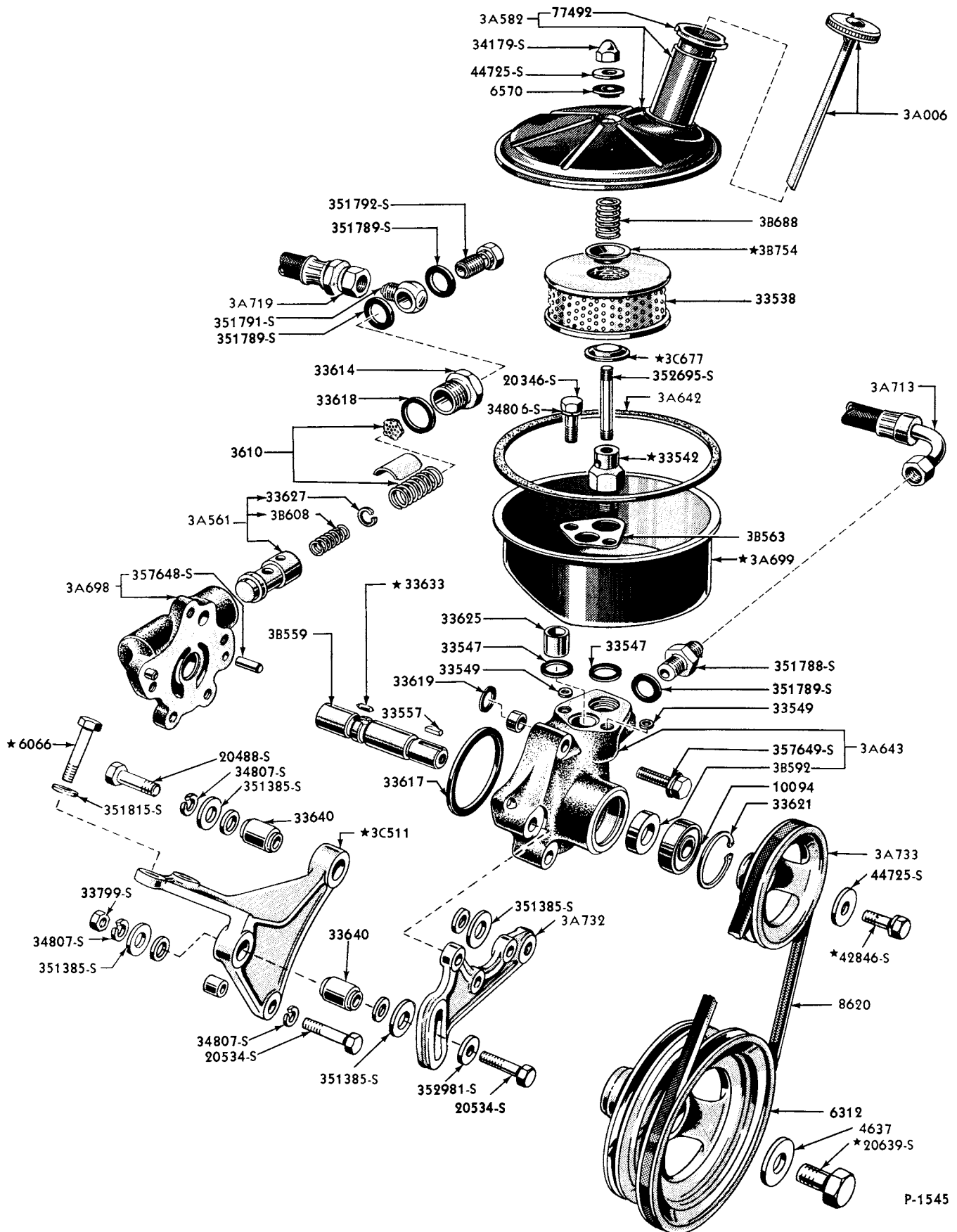
1953 POWER STEERING PUMP, BRACKETS AND RESERVOIR
