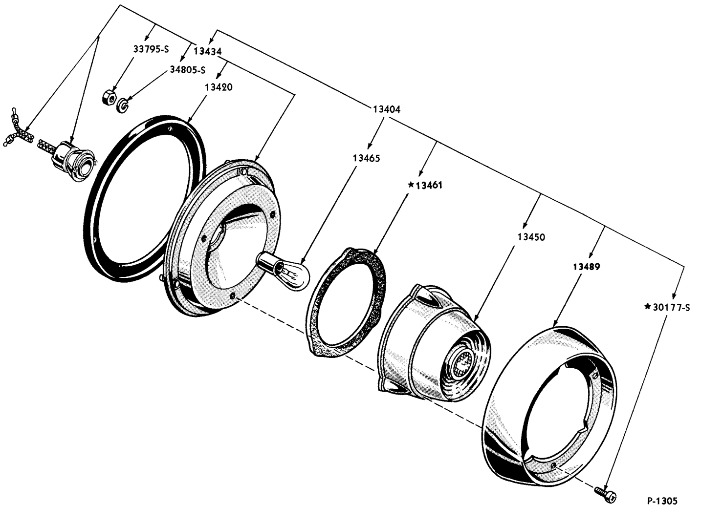
1952 REAR LAMP
