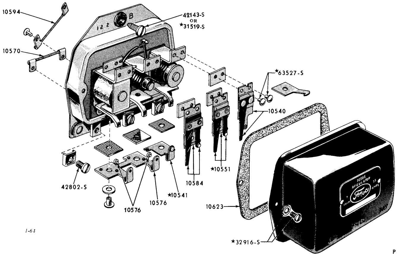
"TYPICAL" VOLTAGE REGULATOR
