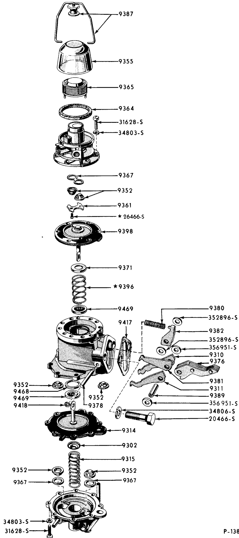
1952/54 FUEL AND VACUUM PUMP (6 CYLINDER 215 AND 223 ENGINES) 1954 FUEL AND VACUUM PUMP (8 CYLINDER 239 ENGINE)
