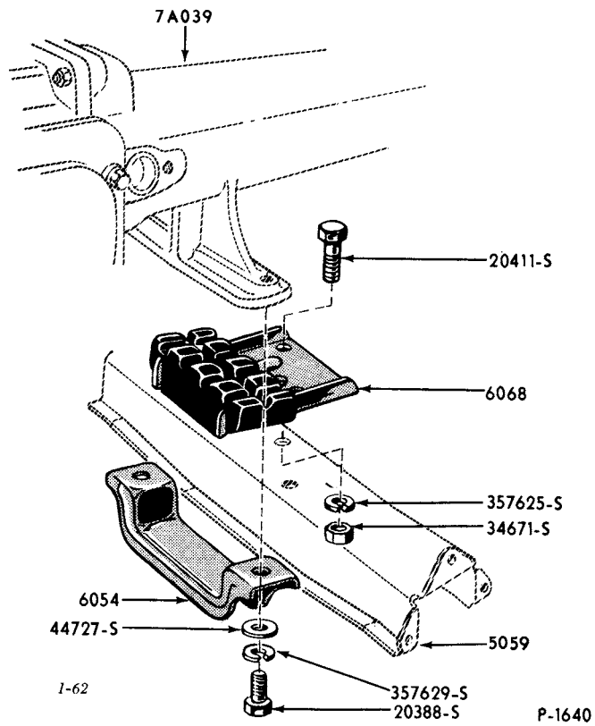
1954/56 ENGINE SUPPORT REAR ("O. H. V" ENGINES)-TYPICAL
