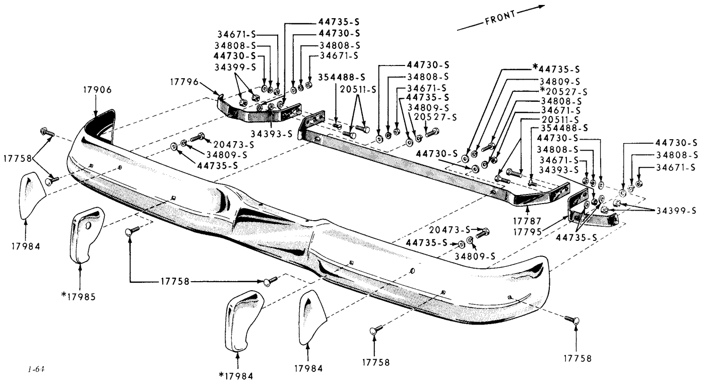
1957 REAR BUMPER (FORD - CUSTOM & CUSTOM "300")
