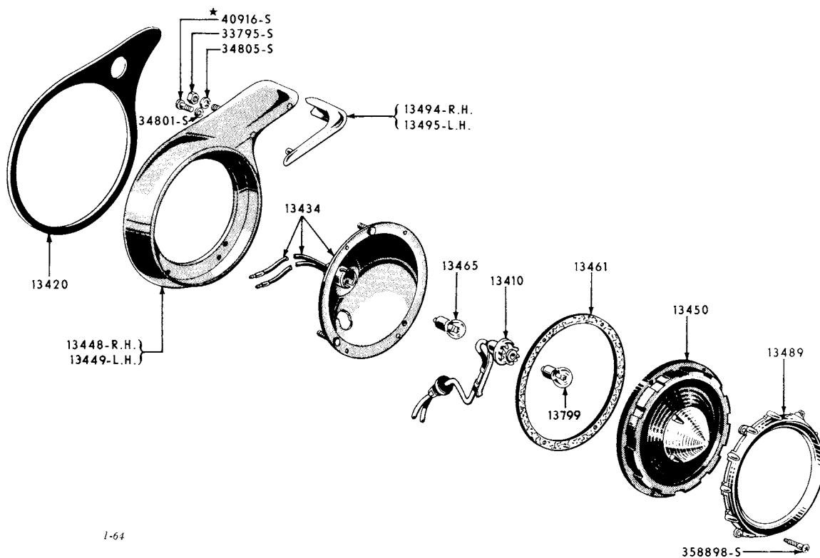
1957 REAR LAMP (FORD - CUSTOM AND CUSTOM "300")
