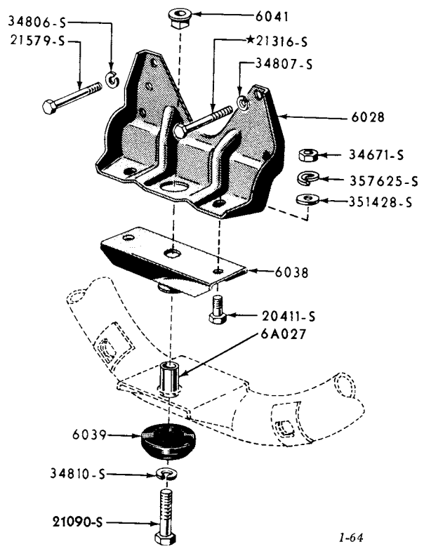
1954/ ENGINE FRONT SUPPORT 6 CYLINDER 223 ENGINE 8 CYLINDER ENGINES - FORD
