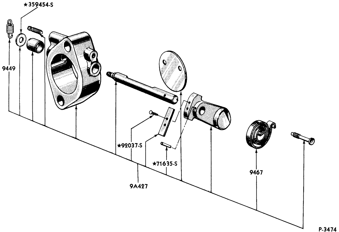
"TYPICAL" VALVE ASSY. -(EXHAUST THERMOSTAT CONTROL)
