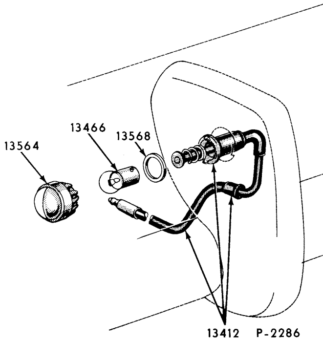
1957 STATION WAGON, SEDAN DELIVERY & 51A MODEL LICENSE PLATE LAMP
