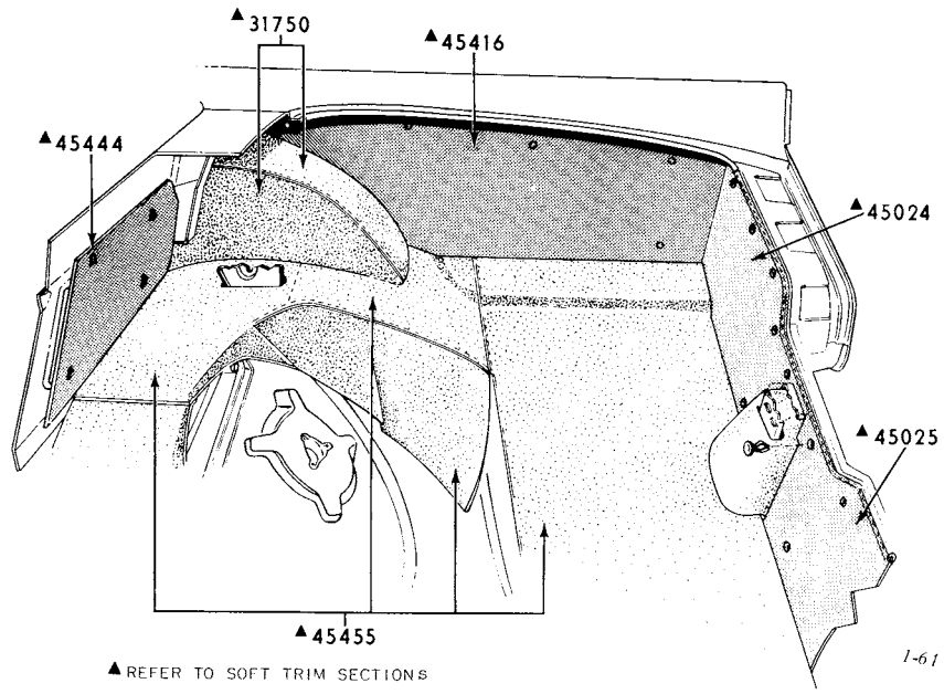
1958/ THUNDERBIRD LUGGAGE COMPARTMENT TRIM - TYPICAL
