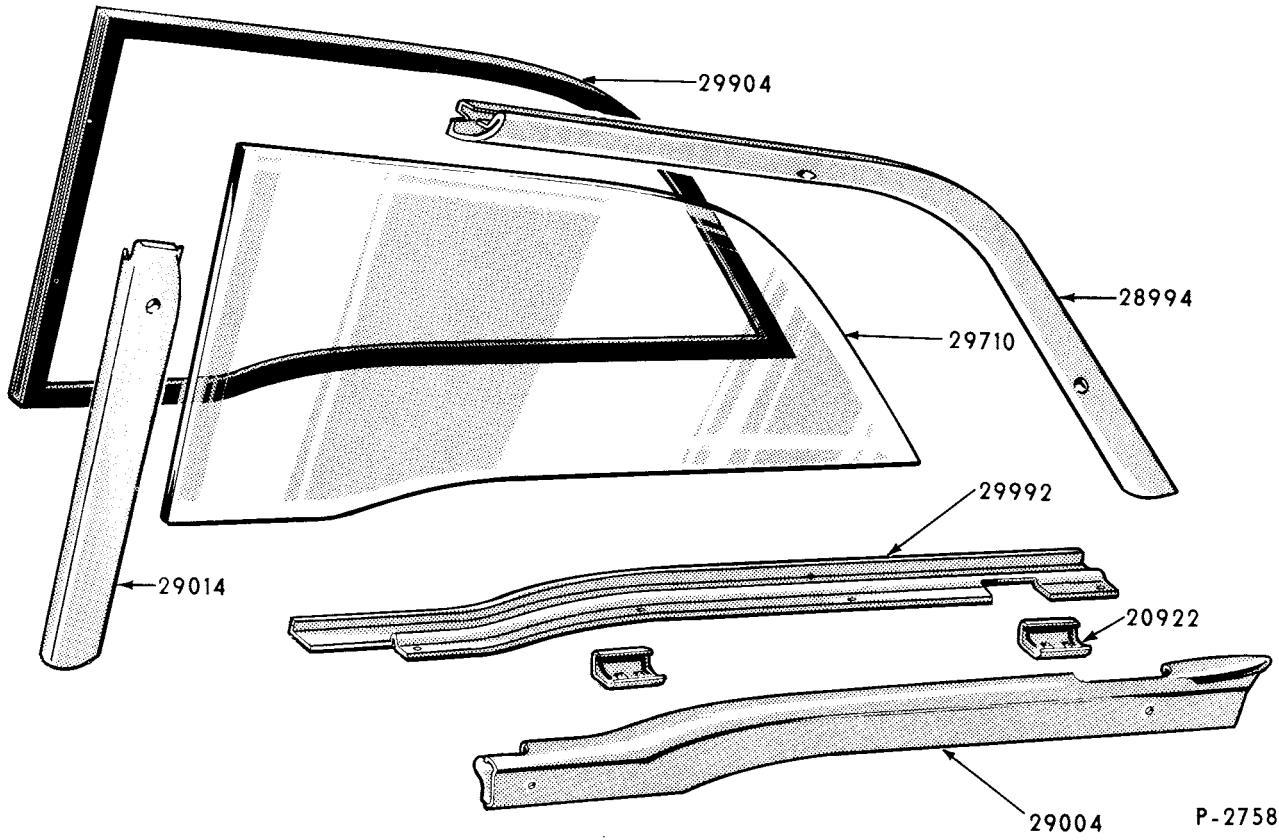
1959 QUARTER WINDOW PARTS (BODY TYPES 59E, 64G)
