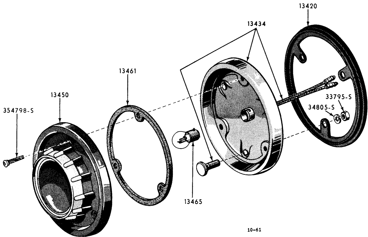
1956 REAR LAMP (FORD AND THUNDERBIRD)
