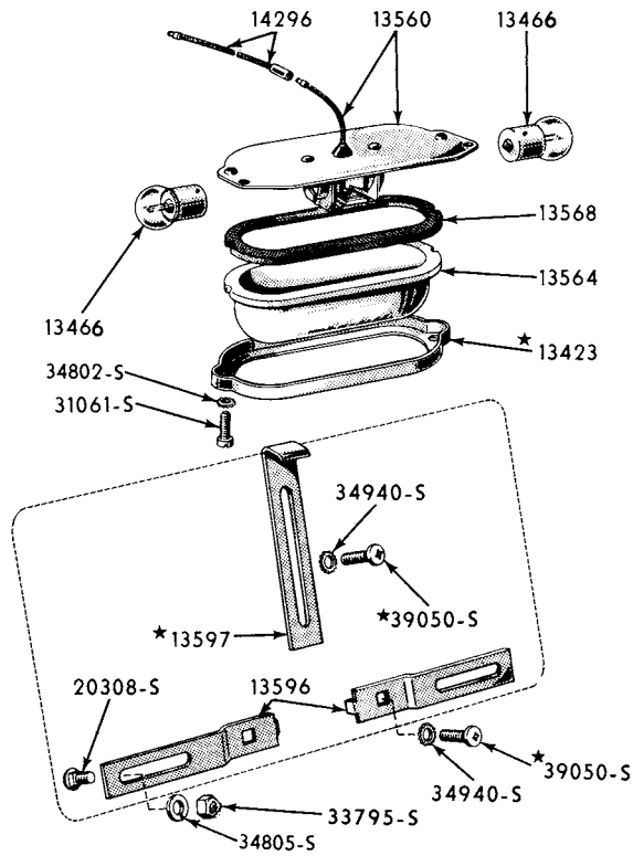
1955/56 LICENSE PLATE LAMP (THUNDERBIRD)
