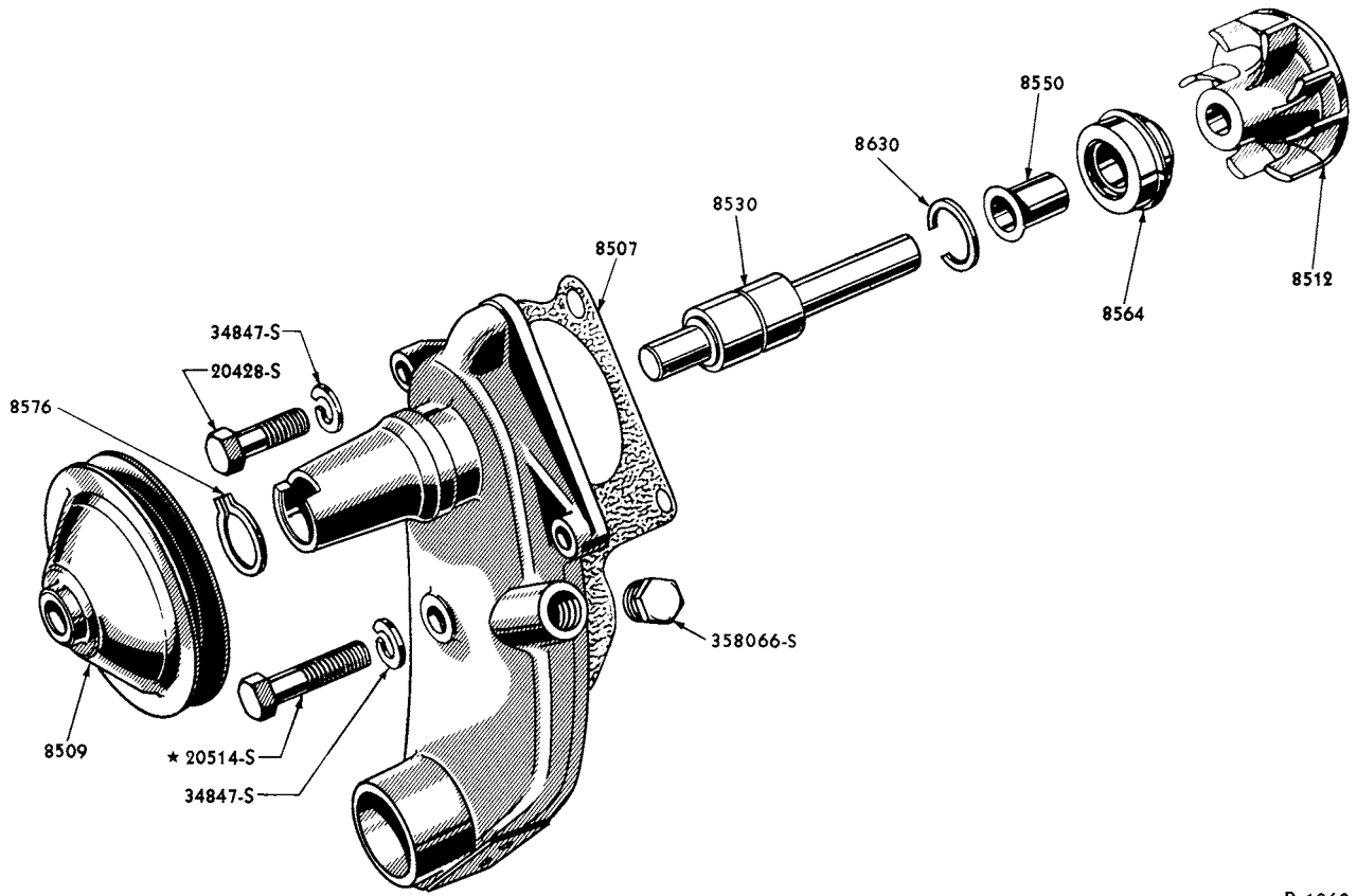
1949/53 WATER PUMP (8 CYLINDER 239 ENGINE)
