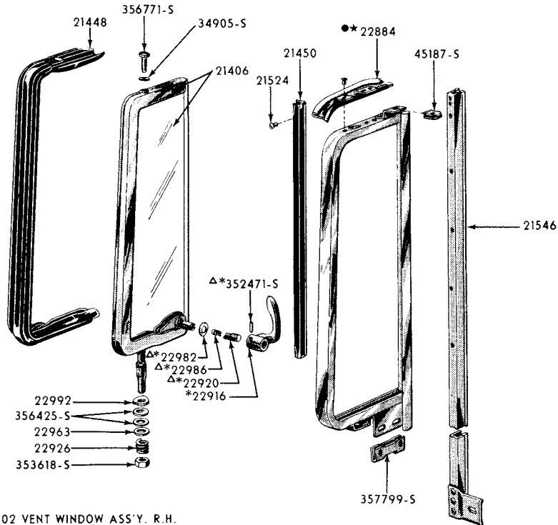
21402 VENT WINDOW ASS'Y. R.H. (INCLUDES ALL PARTS SHOWN) *THESE PARTS INCLUDED IN 21406 ● 1955 ONLY △ INCLUDED WITH 22916-7
