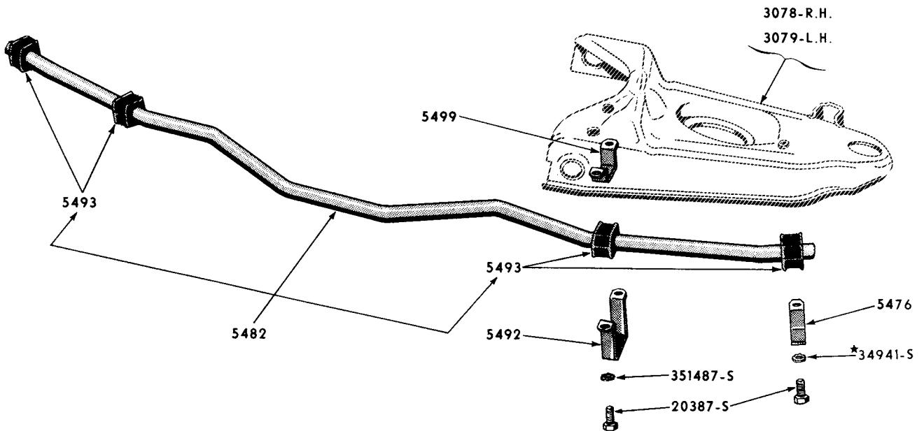
STABILIZER (1954/56 FORD) (1955/57 THUNDERBIRD)
