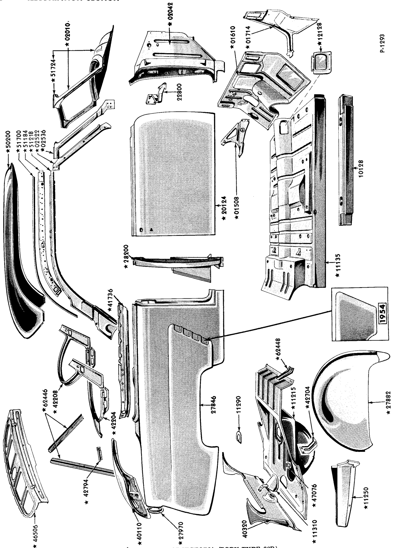
1953/54 CRESTLINE VICTORIA (BODY TYPE 60B)
