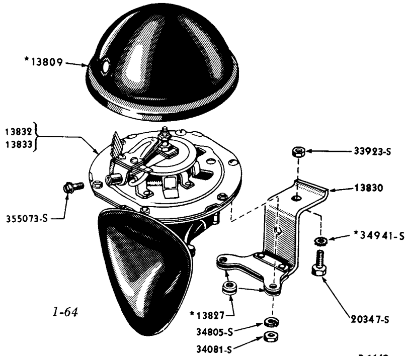
1949/50 HORN
