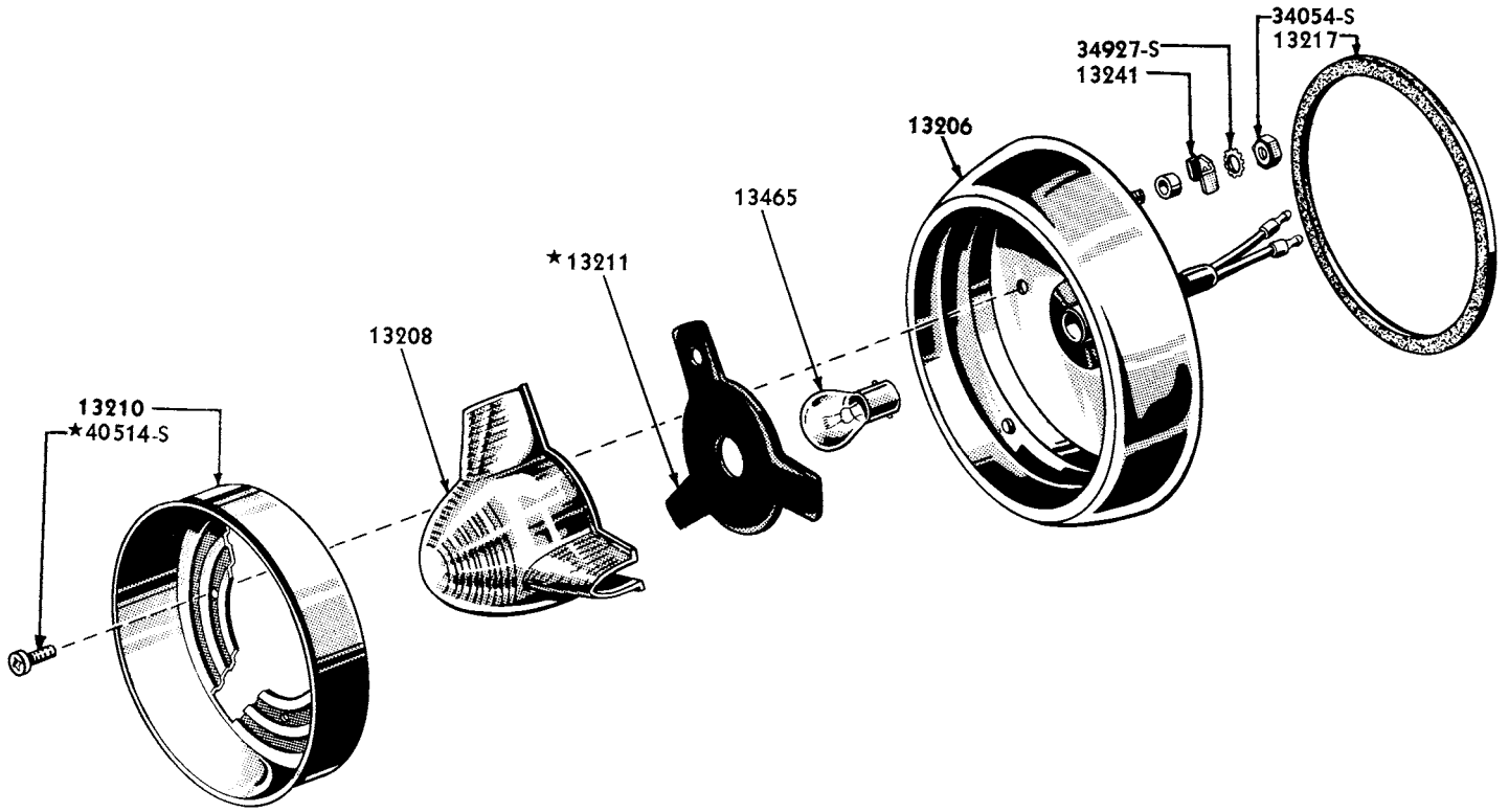
1952 PARKING LAMP
