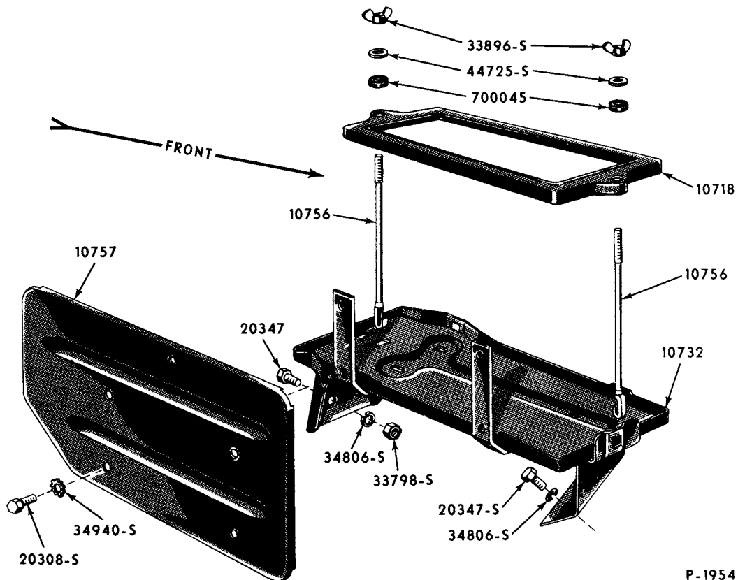
1956/57 "TYPICAL" BATTERY CARRIER AND RELATED PARTS (THUNDERBIRD)
