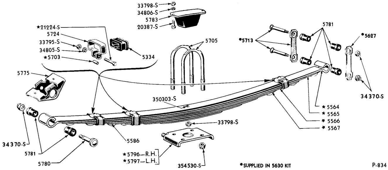
1949/50 REAR SUSPENSION
