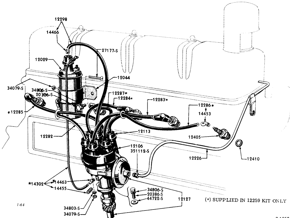
1952/54 IGNITION WIRING (6 CYLINDER 215 & 223 ENGINES)
