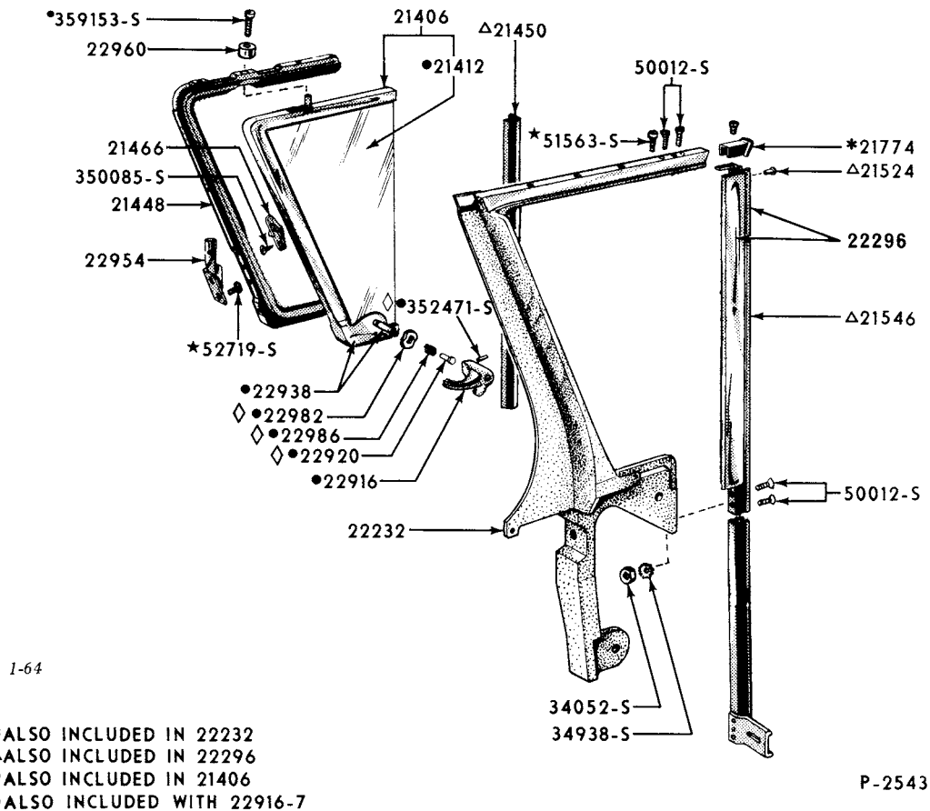
1957/58 DOOR VENT WINDOW PARTS (BODY TYPES 51A, 57, 63, 76)
