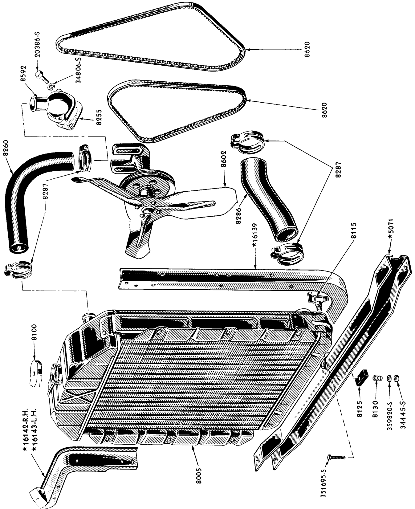
1949/53 "TYPICAL" COOLING SYSTEM (8 CYLINDER 239)
