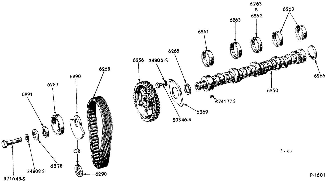
1954/ CAMSHAFT, GEAR, BEARING, ETC. (8 CYLINDER 239, 272, 292, 312 "O. H. V." ENGINES)-TYPICAL
