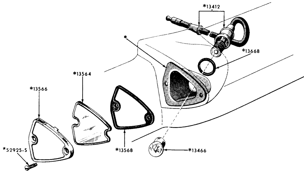
1958 LICENSE PLATE LAMP (RANCHERO, SEDAN DELIVERY AND STATION WAGON)
