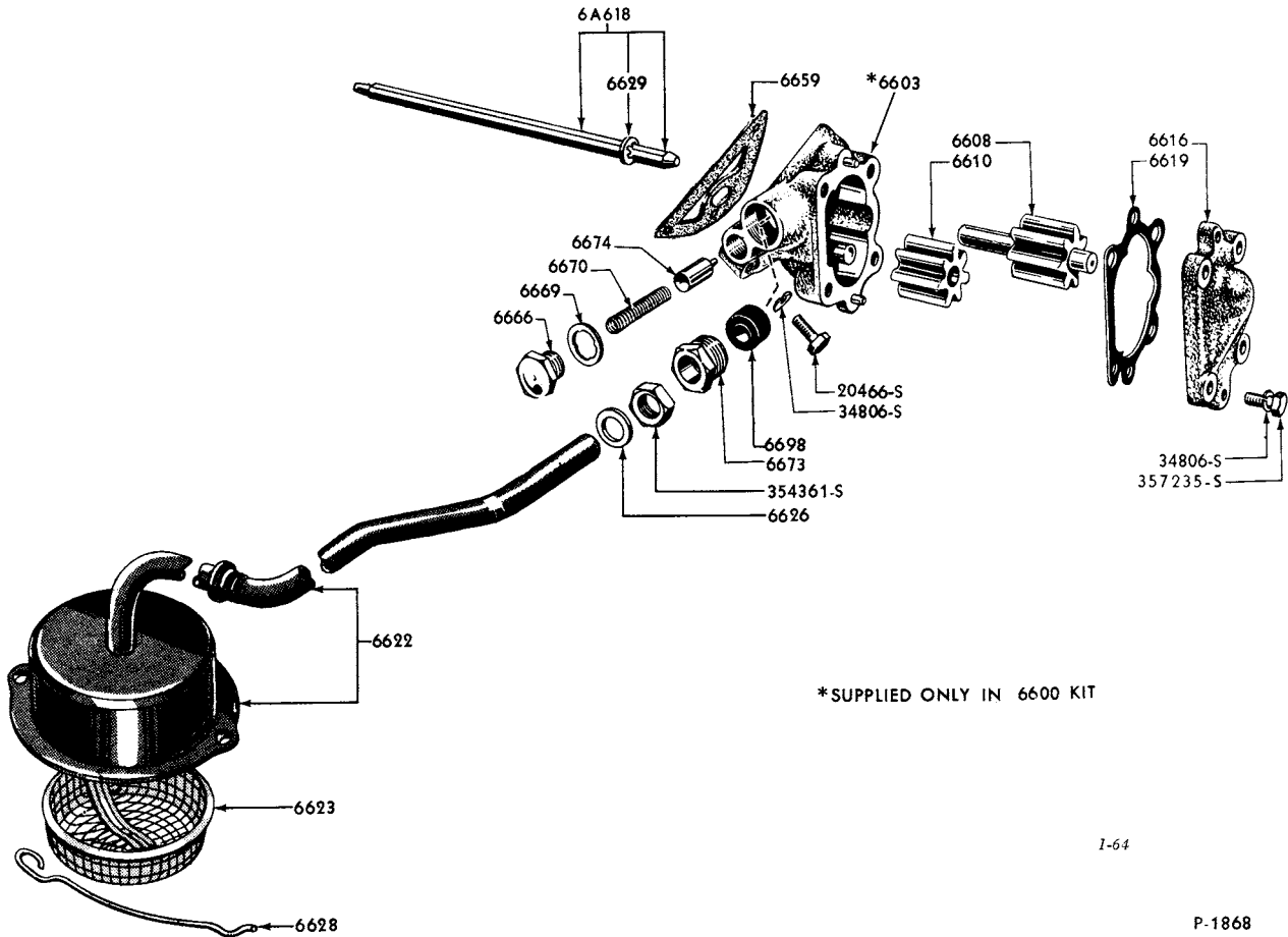
1954/ OIL PUMP & RELATED PARTS (GEAR TYPE) (8 CYLINDER "O. H. V." ENGINES)-TYPICAL
