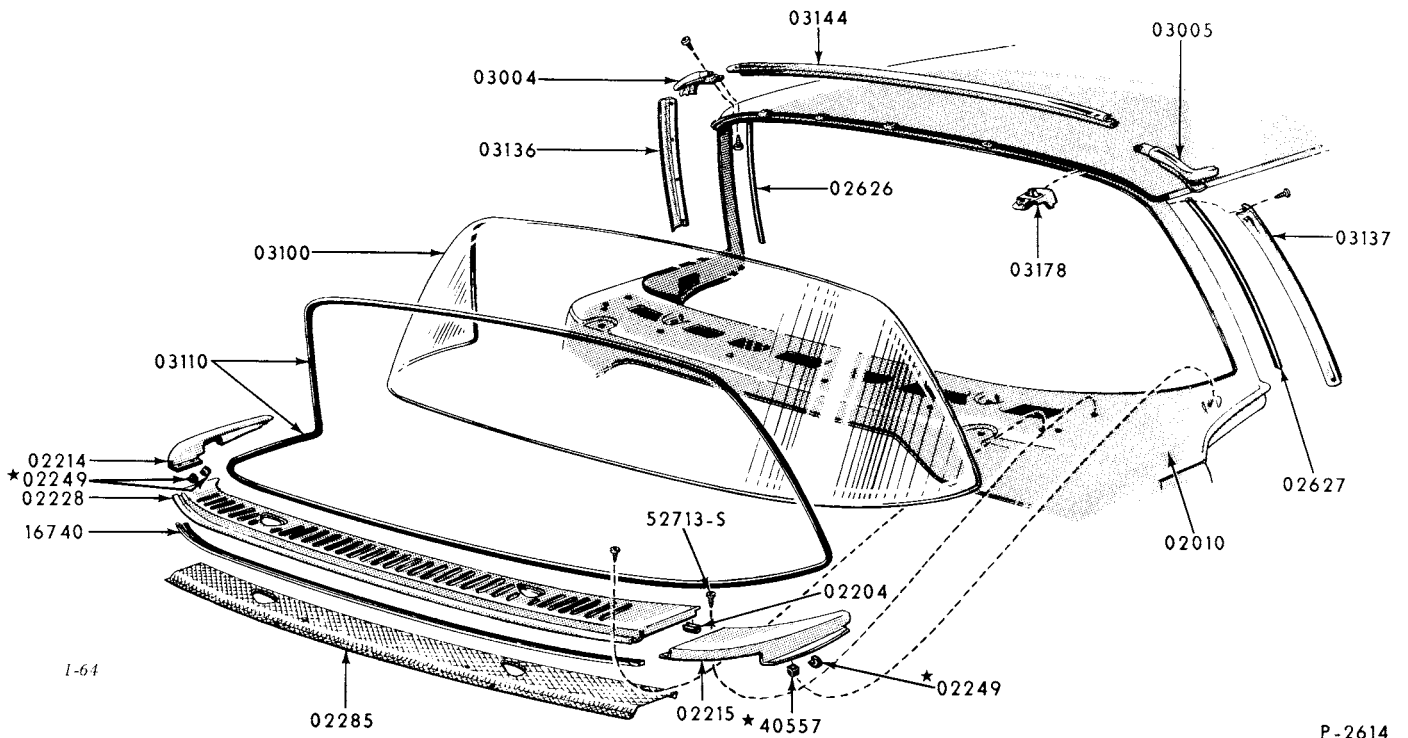
1958/ THUNDERBIRD WINDSHIELD PARTS - BODY TYPE S (63A)
