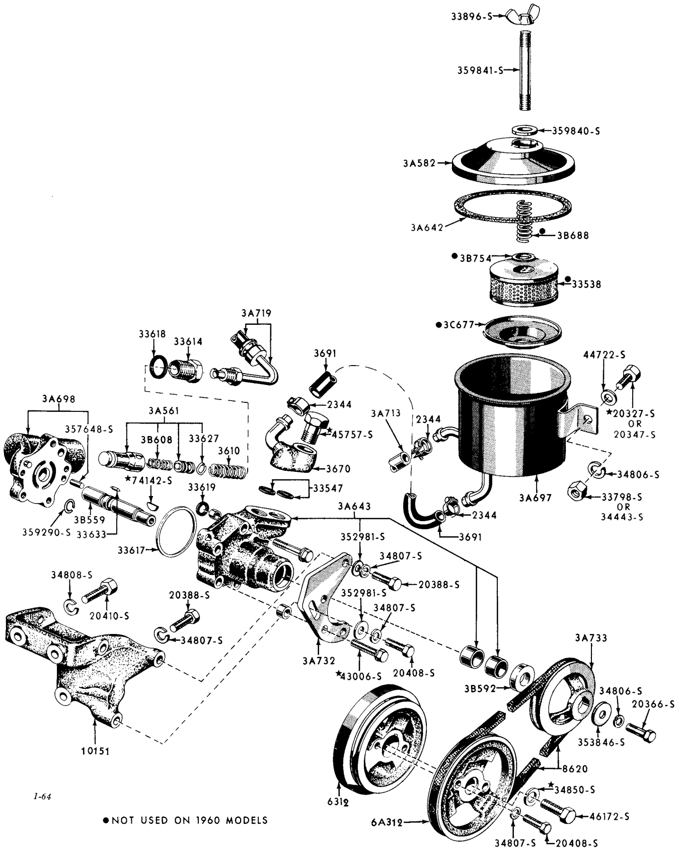
1957/ "TYPICAL" POWER STEERING PUMP, RESERVOIR AND RELATED PARTS (FORD - 6 CYL.)
