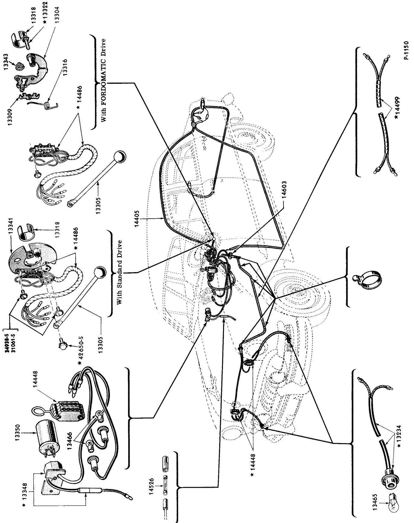
1951 TURN INDICATOR
