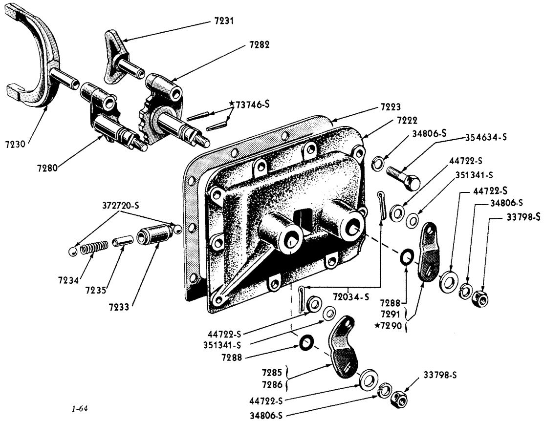
1955/57 "TYPICAL" GEAR SHIFT HOUSING, LEVERS, FORKS, ETC. (THUNDERBIRD 8 CYLINDER 292)
