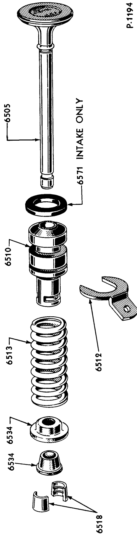
1949/53 VALVE AND RELATED PARTS (8 CYLINDER 239 "L" HEAD ENGINE)
