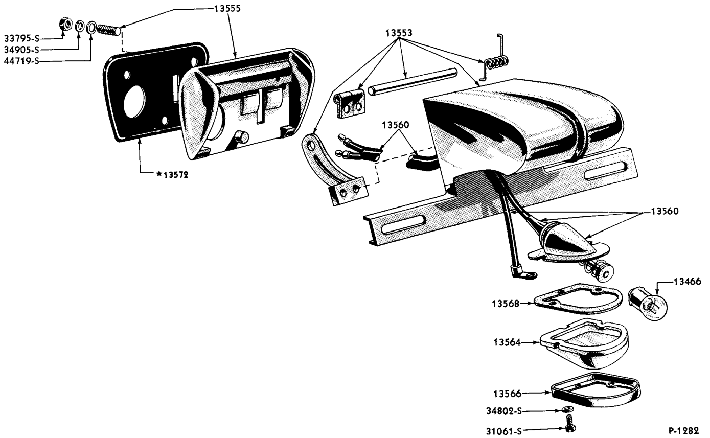
1952/54 LICENSE PLATE LAMP (STATION WAGON AND SEDAN DELIVERY)
