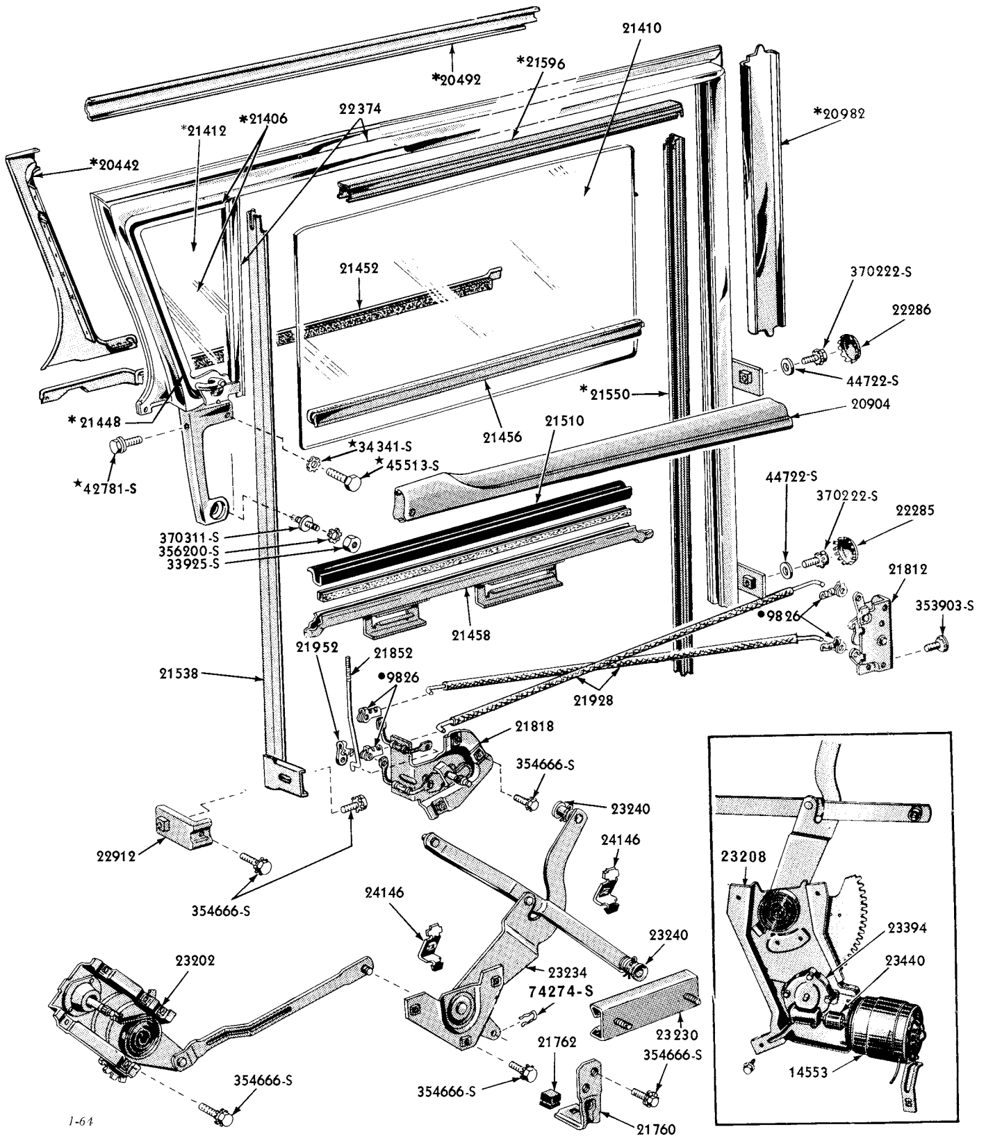
ELECTRIC REGULATOR
