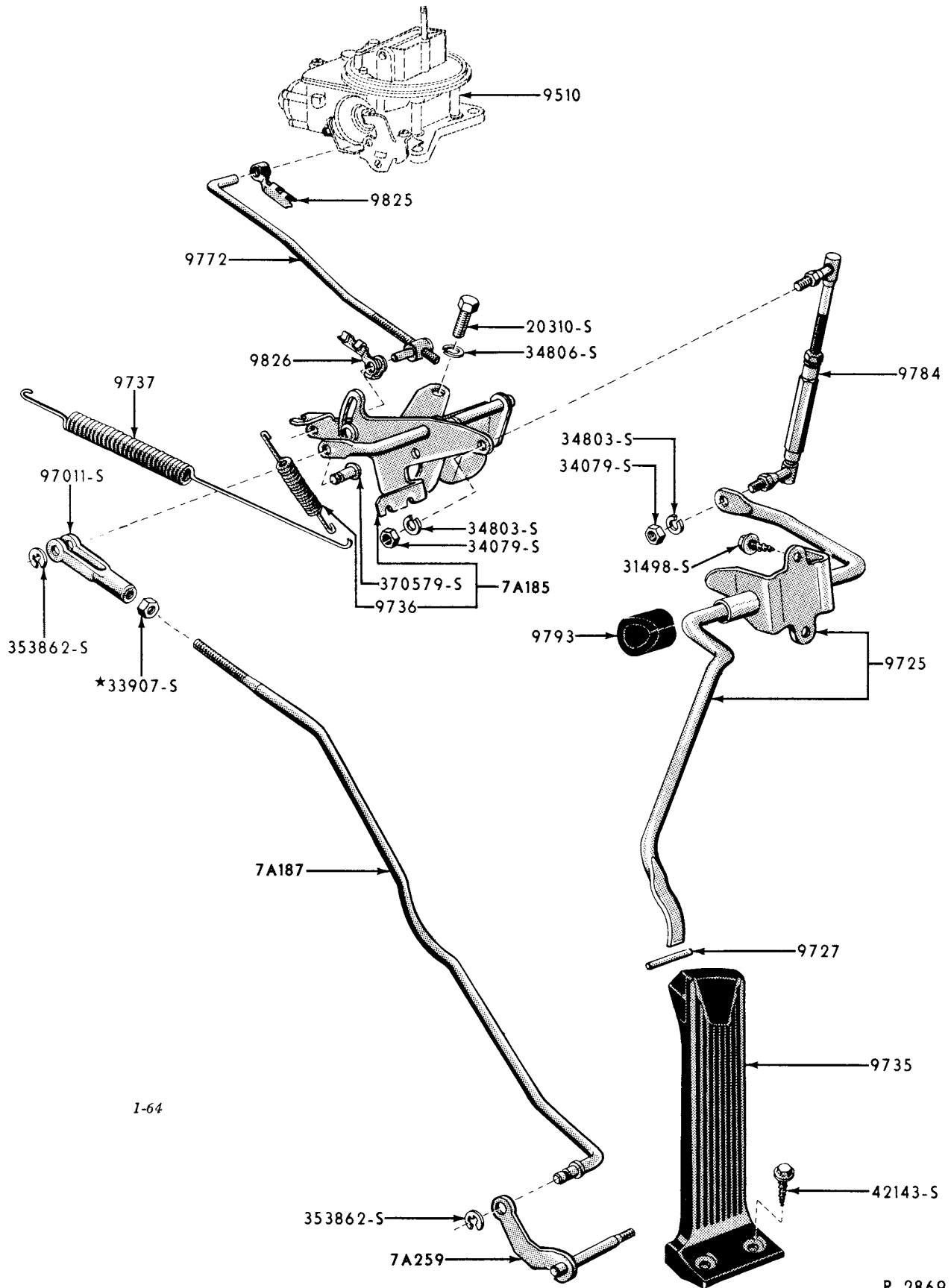
1959 ACCELERATOR LINKAGE - FORD (8 CYLINDER)-WITH CRUISE-O-MATIC TRANSMISSION
