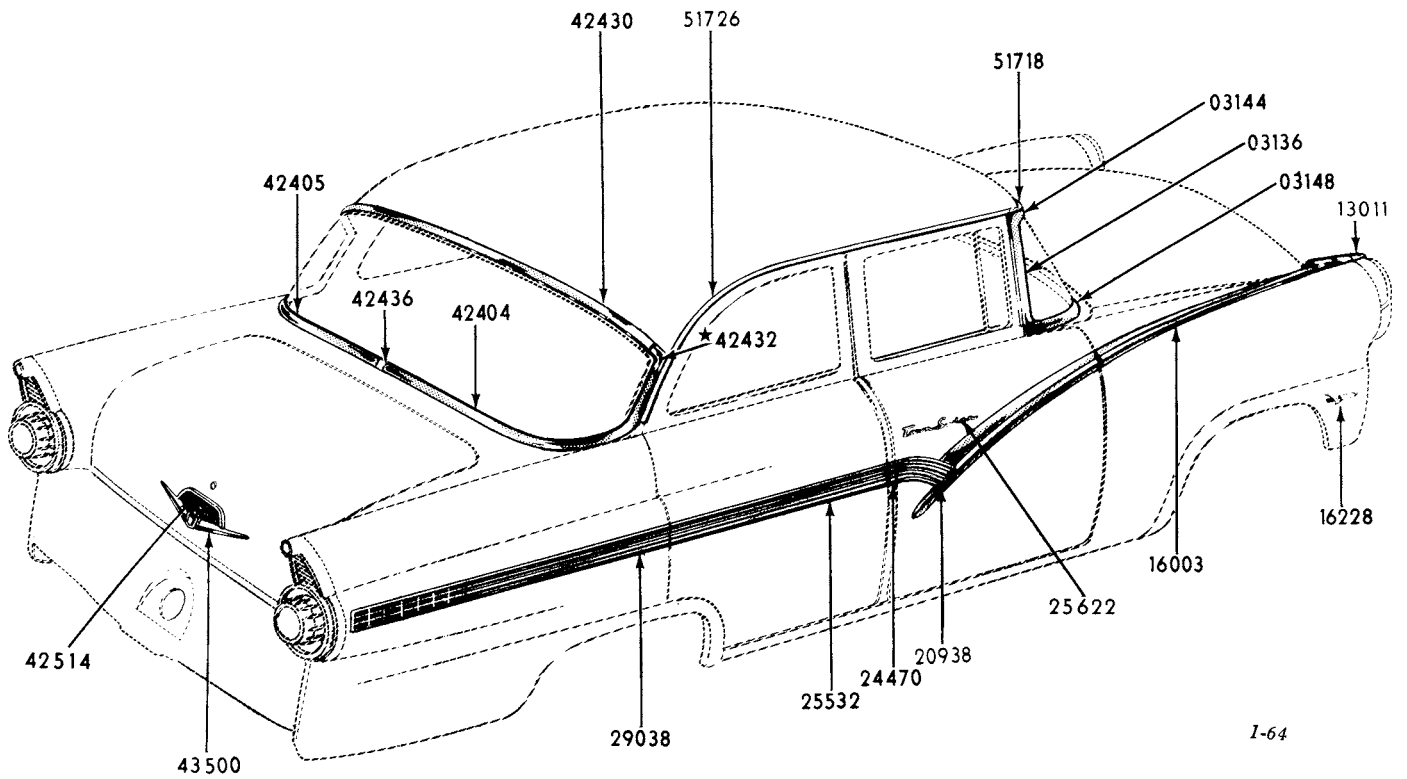
1956 FAIRLANE FORDOR SEDAN (BODY TYPE 73C)
