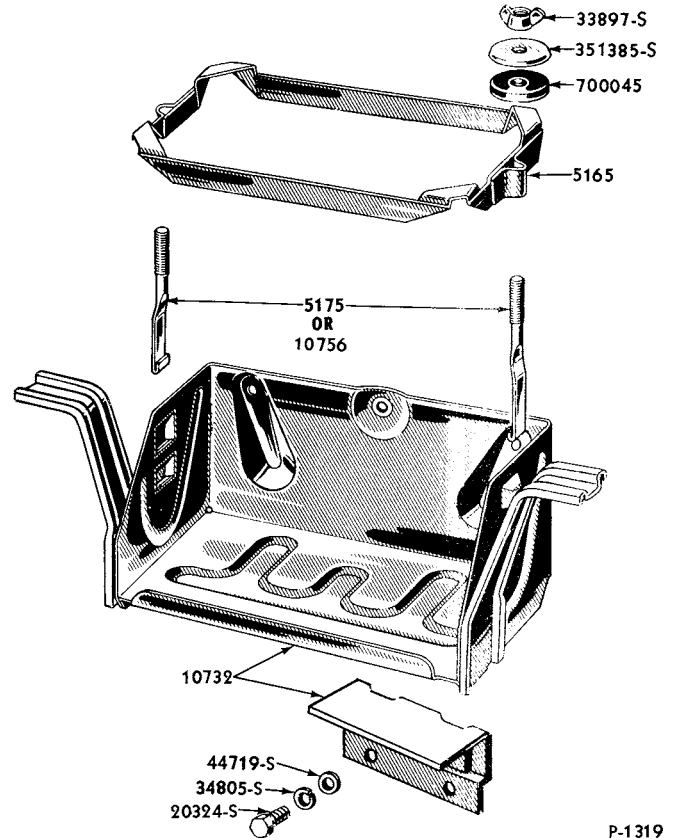
1952/53 BATTERY CARRIER AND RELATED PARTS
