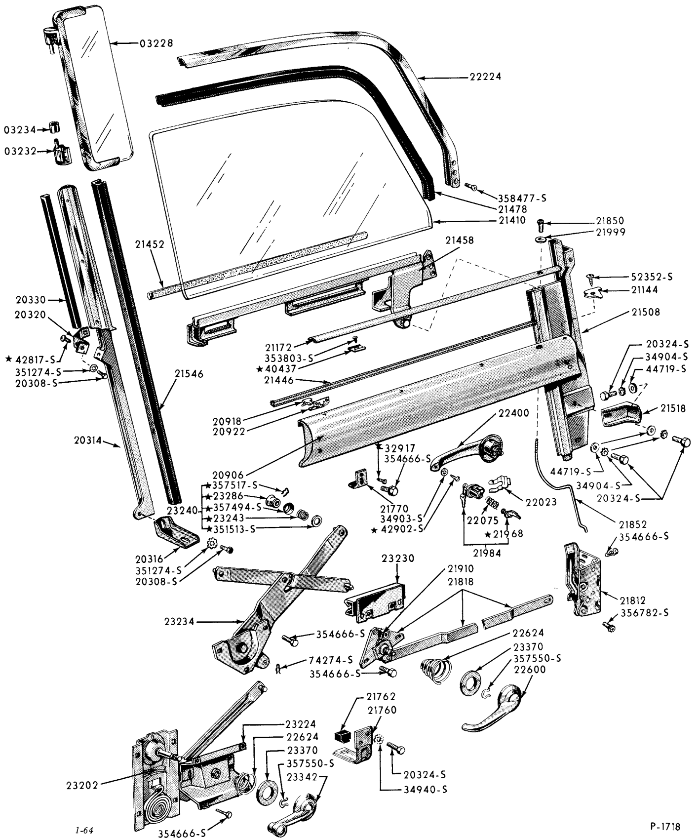
1955/57 THUNDERBIRD DOOR PARTS WITH MANUAL WINDOW REGULATOR
