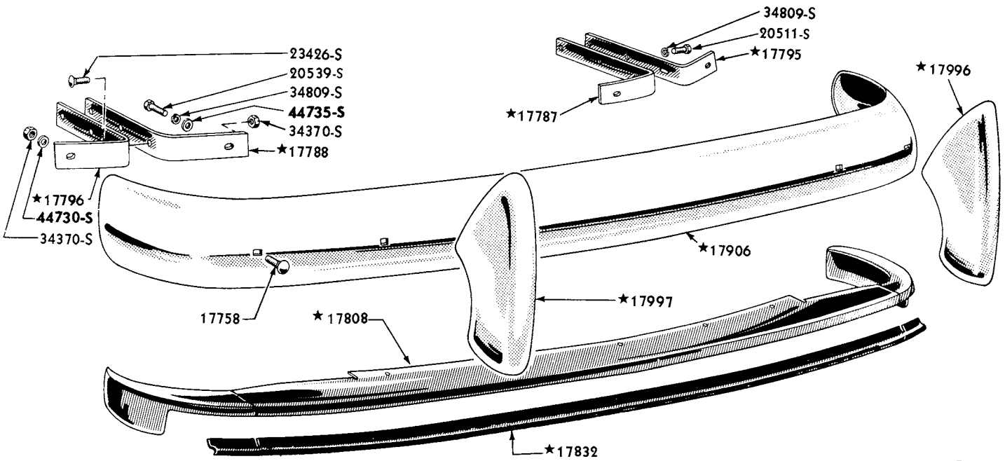
1949 REAR BUMPER AND STONE DEFLECTOR
