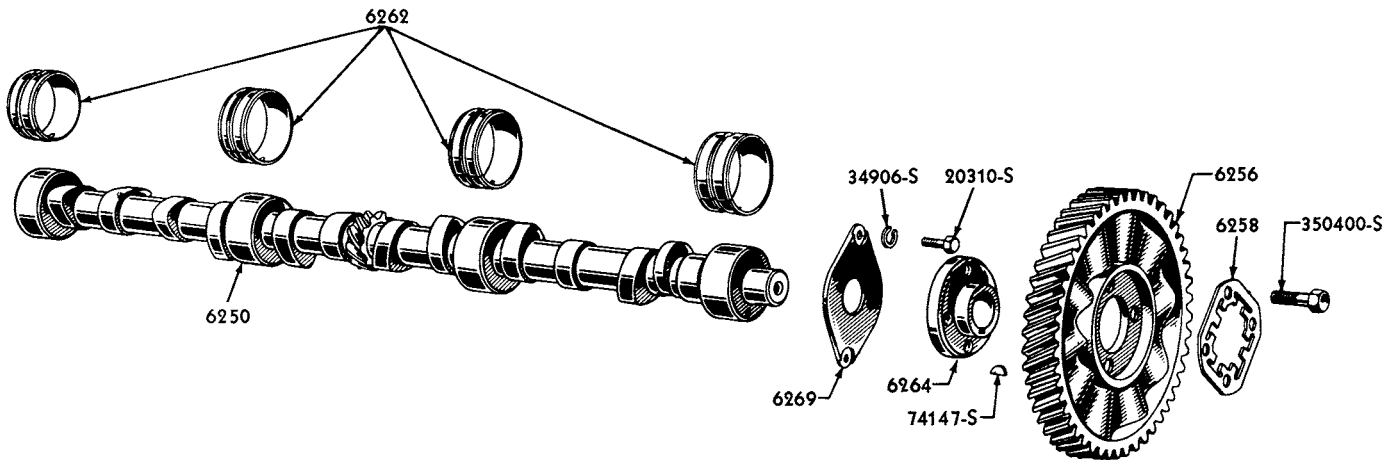
1954/ CAMSHAFT, GEAR, BEARINGS, ETC. (6 CYLINDER 223 ENGINE)
