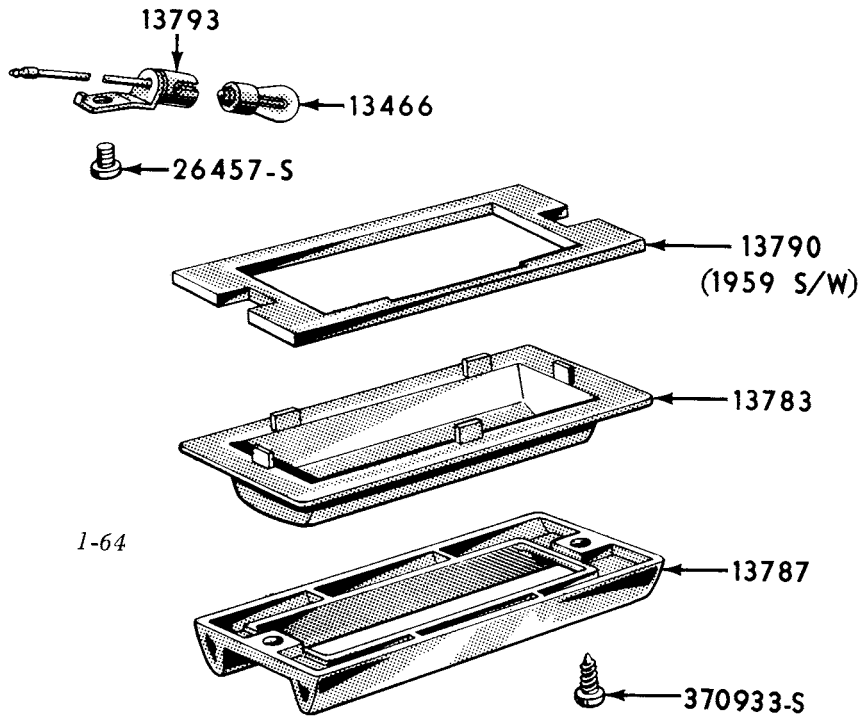
1958/ THUNDERBIRD & 1959 FORD DOME LAMP
