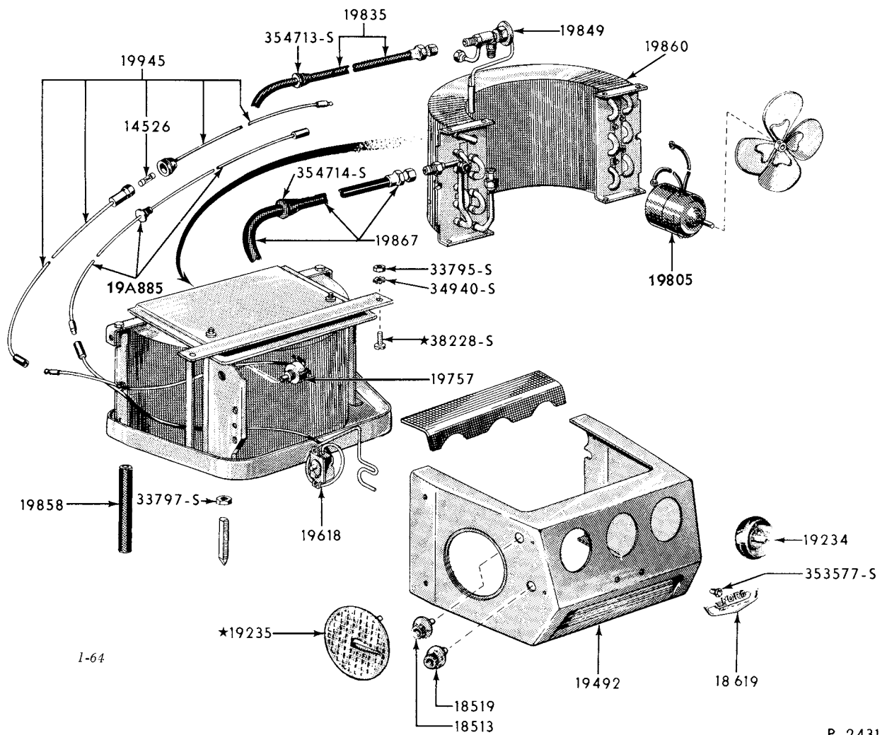
1957/58 FORD POLAR AIRE CONDITIONER EVAPORATOR & CONTROLS
