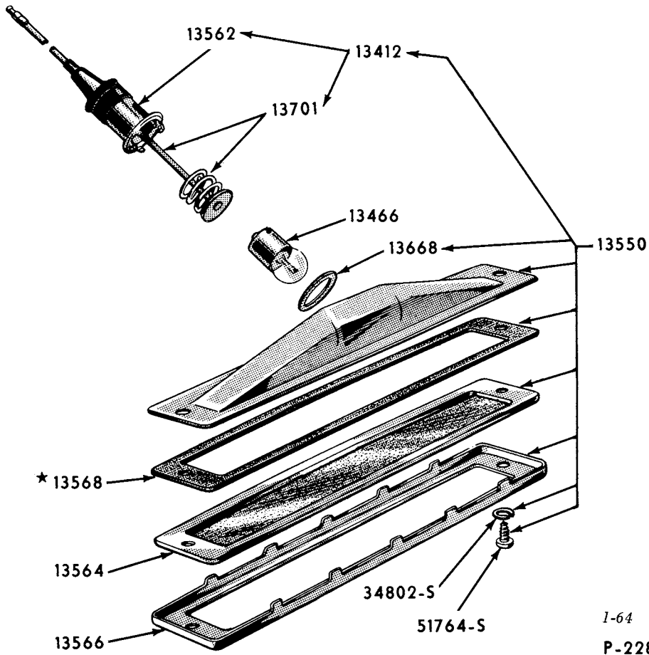
1957 LICENSE PLATE LAMP (THUNDERBIRD)
