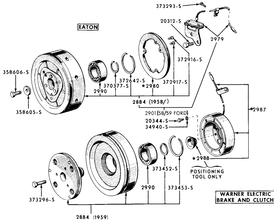
1958/59 FORD & THUNDERBIRD AIR CONDITIONER COMPRESSOR, PULLEYS & RELATED PARTS (SIDE MOUNTED HOSES)
