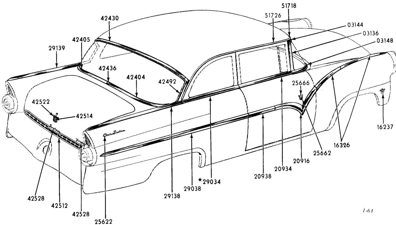
1955 CUSTOMLINE TUDOR SEDAN (BODY TYPE 70B)
