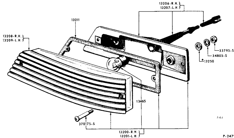
1958 PARKING LAMP (FORD)
