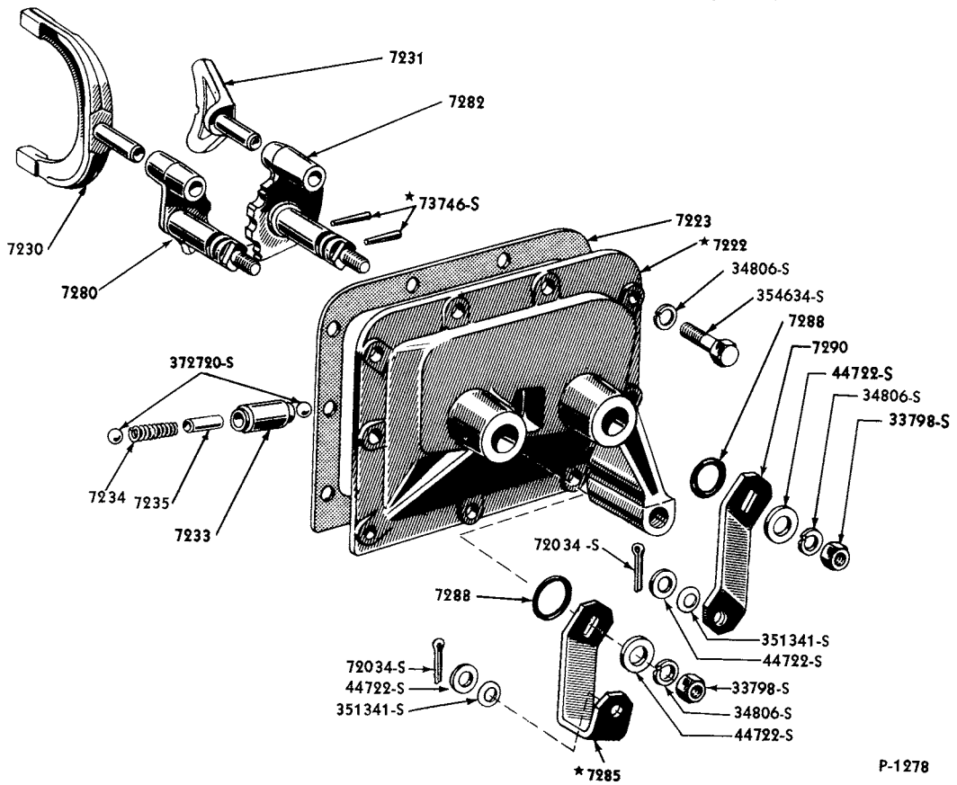
1951 GEAR SHIFT HOUSING, LEVERS, FORKS, ETC.
