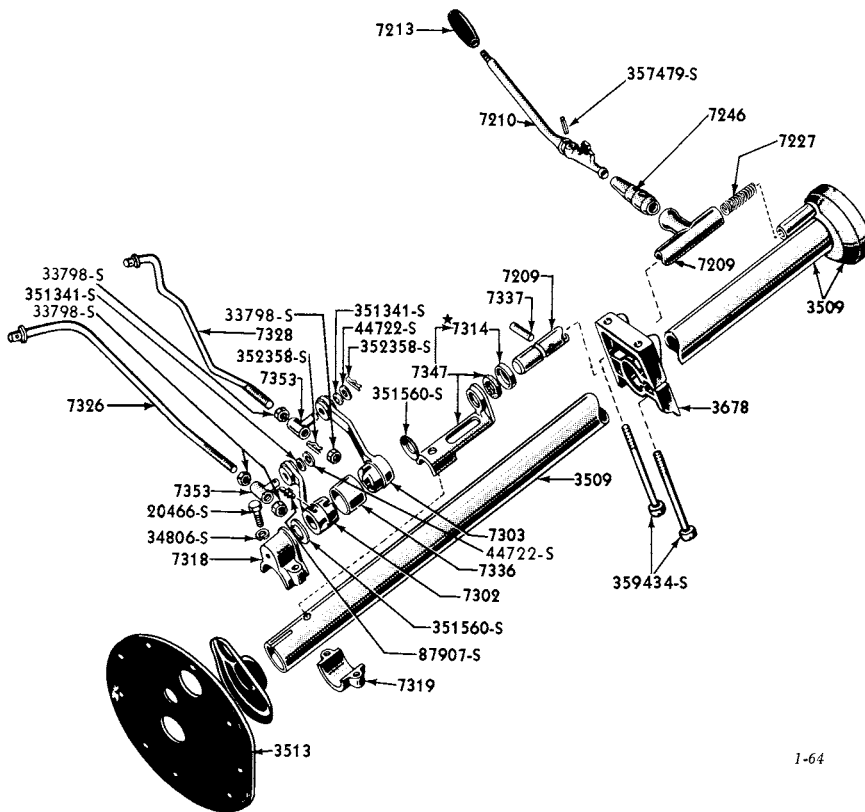
1955 GEAR SHIFT COLUMN (FORD - 6 & 8 CYLINDER ENGINES)
