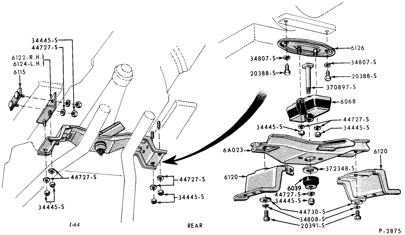
1959/ ENGINE SUPPORTS-FRONT & REAR (THUNDERBIRD-8 CYLINDER 430)-TYPICAL
