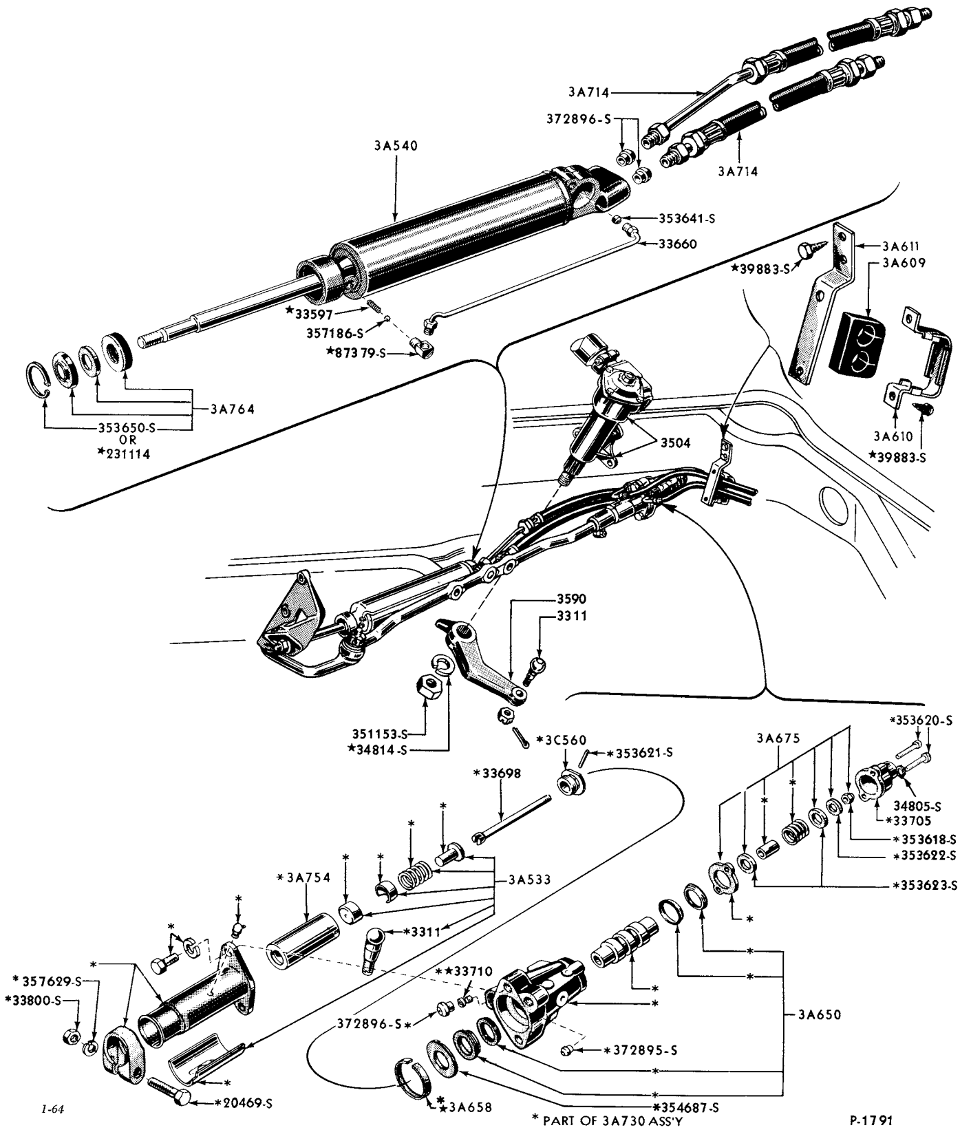
1955/56 "TYPICAL" POWER STEERING VALVE AND CYLINDER (THUNDERBIRD)
