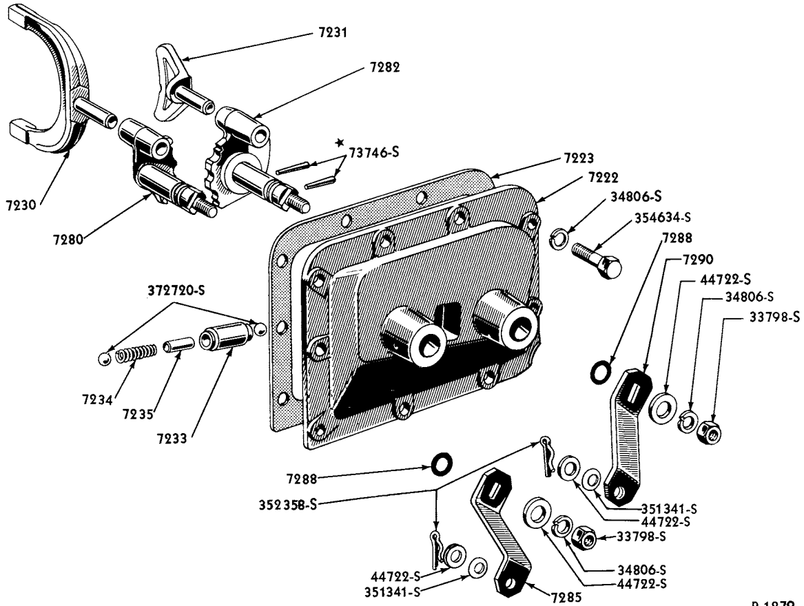
1952/54 GEAR SHIFT HOUSING, LEVERS, FORKS, ETC.
