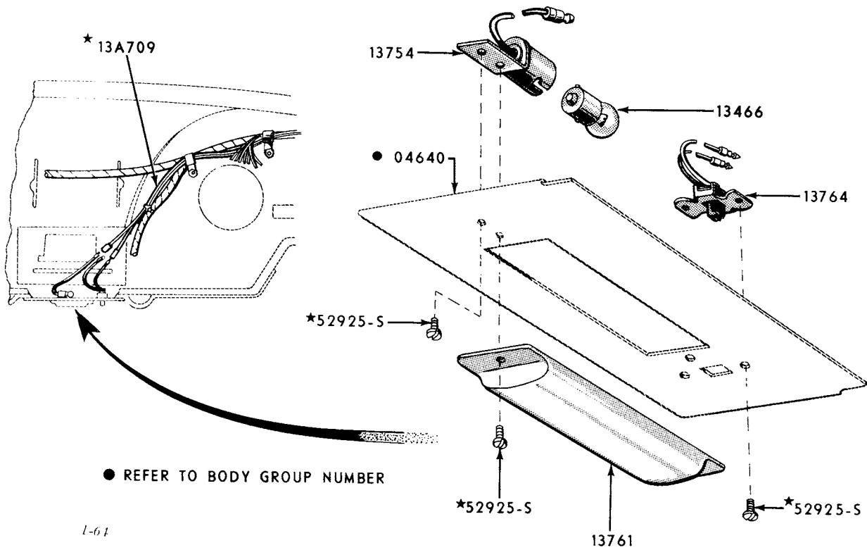
1958/ THUNDERBIRD & 1959 FORD DOME LAMP
