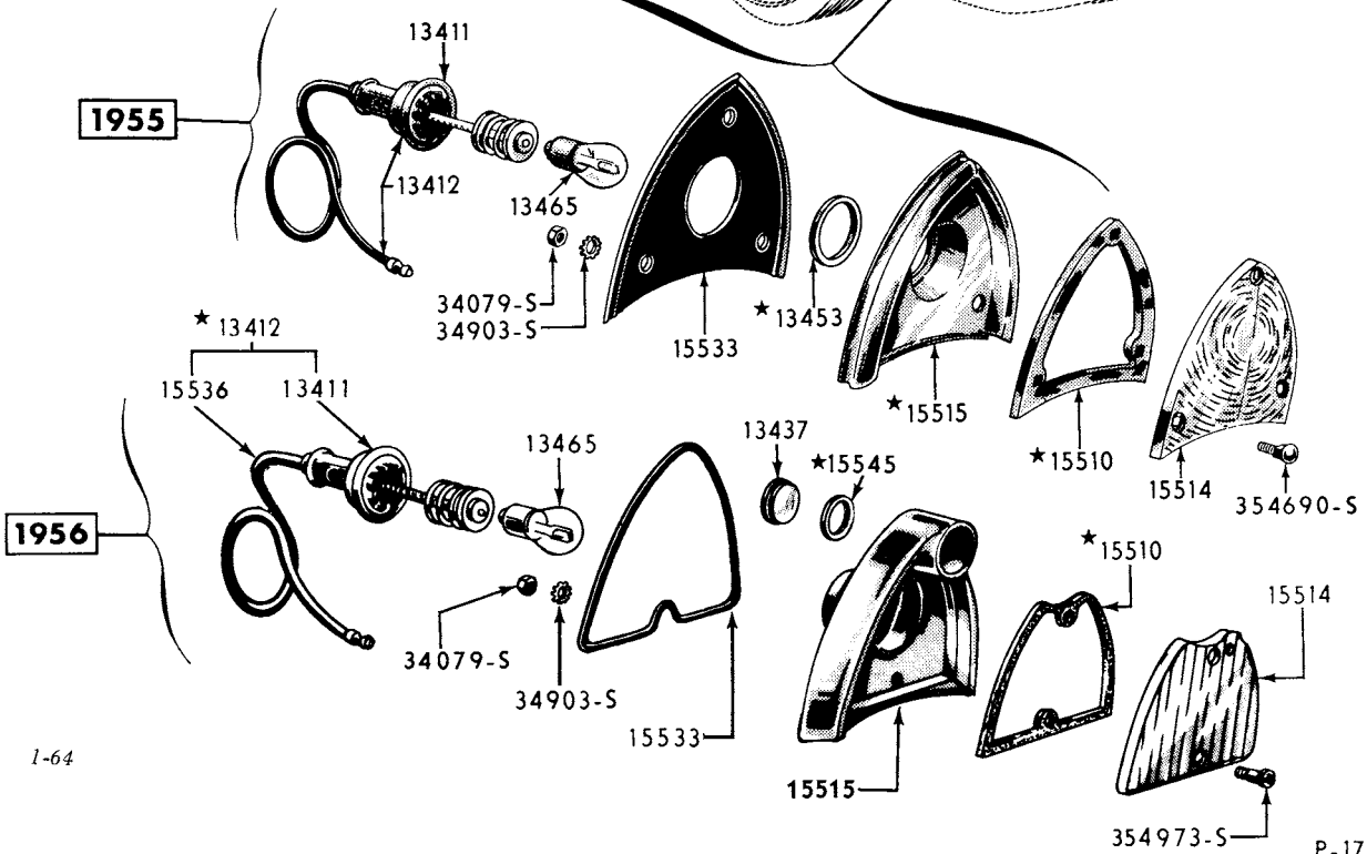
1955/56 BACK UP LAMP (THUNDERBIRD)
