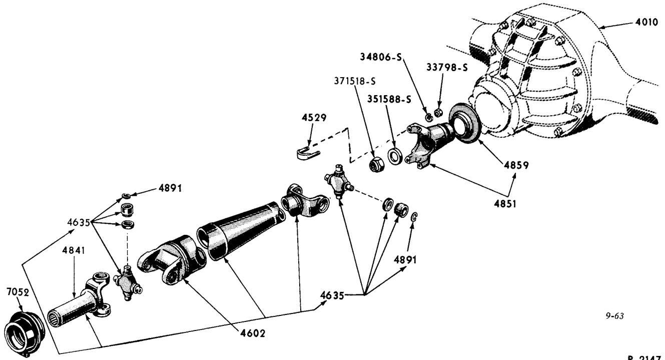
1957/59 "TYPICAL" DRIVE SHAFT
