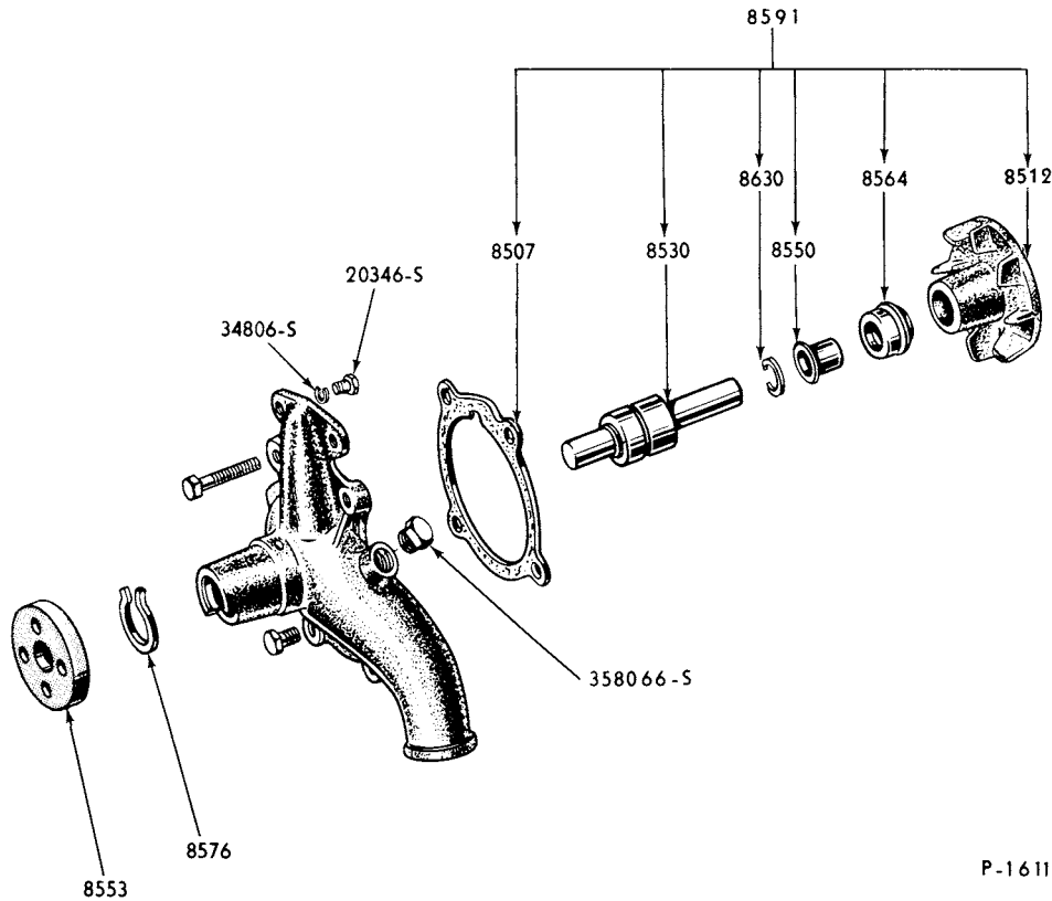
1954/57 "TYPICAL" WATER PUMP (8 CYLINDER "O. H. V." ENGINES)
