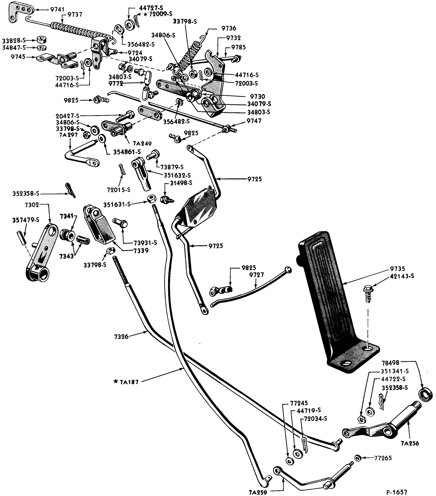
1954 ACCELERATOR LINKAGE (6 CYLINDER 223 ENGINE)-FORDOMATIC
