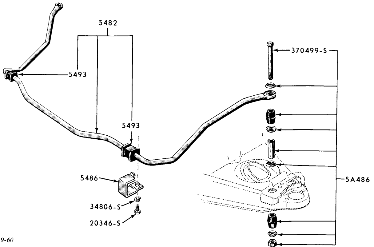
1959 PASSENGER STABILIZER
