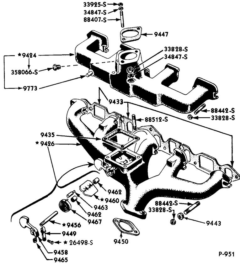
1949/51 MANIFOLD AND RELATED PARTS (6 CYLINDER 226 ENGINE)
