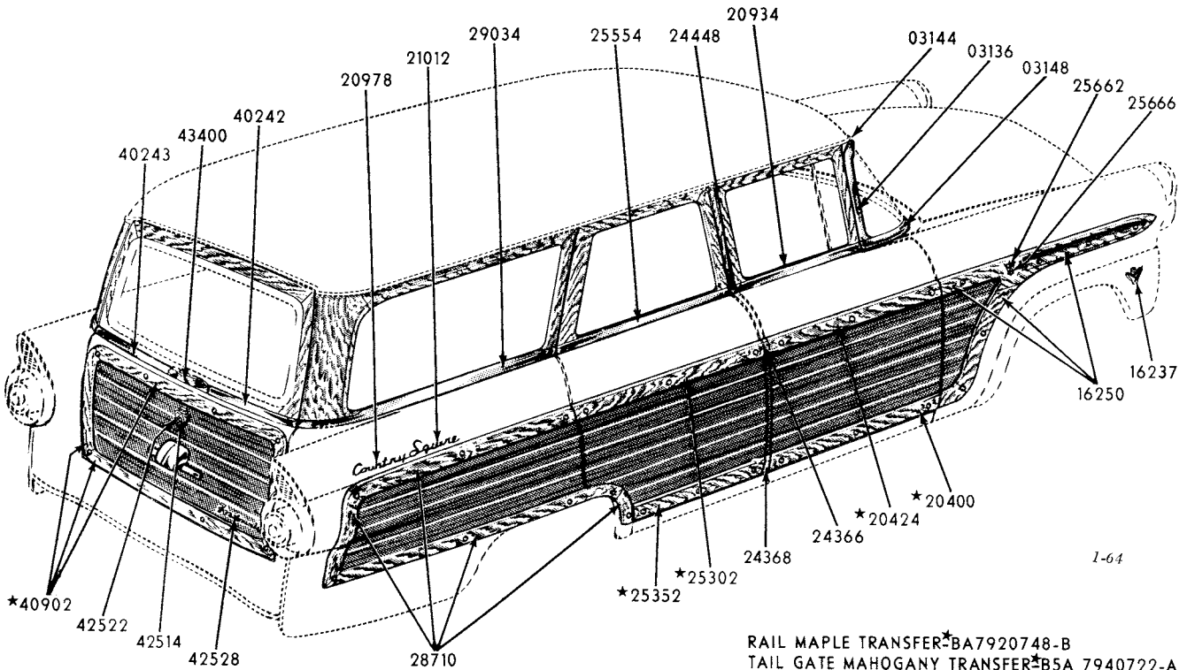
1955 FAIRLANE STATION WAGON "COUNTRY SEDAN"-(BODY TYPE 79B)
