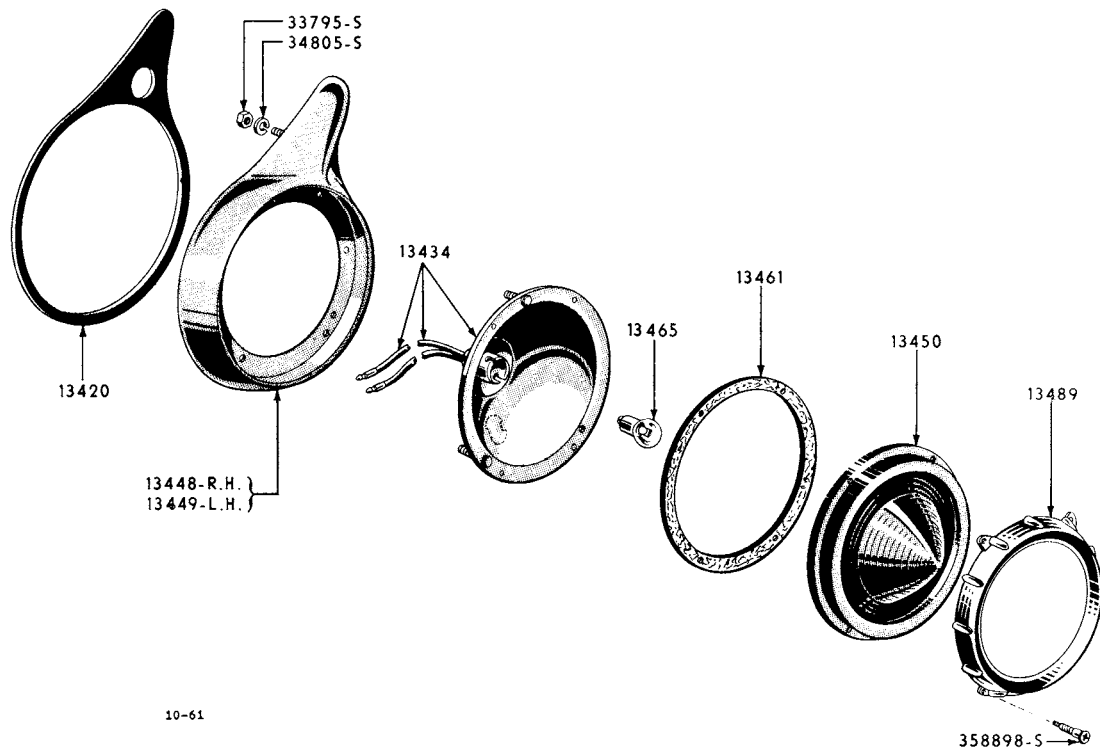
1957 REAR LAMP (FORD - CUSTOM AND CUSTOM "300")
