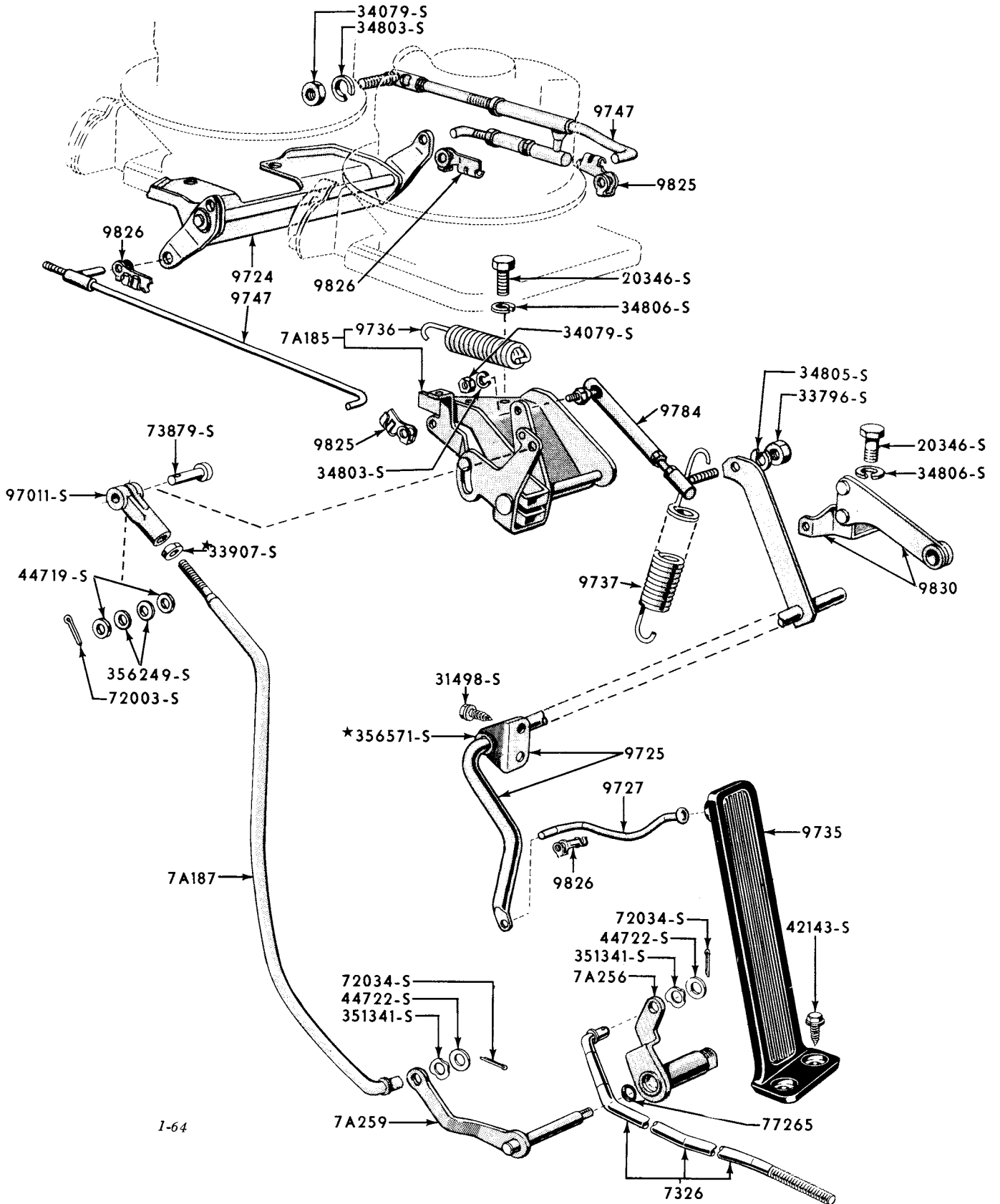
1957 ACCELERATOR LINKAGE - WITH DUAL 4 BARREL CARBURETOR - FORDOMATIC (THUNDERBIRD)
