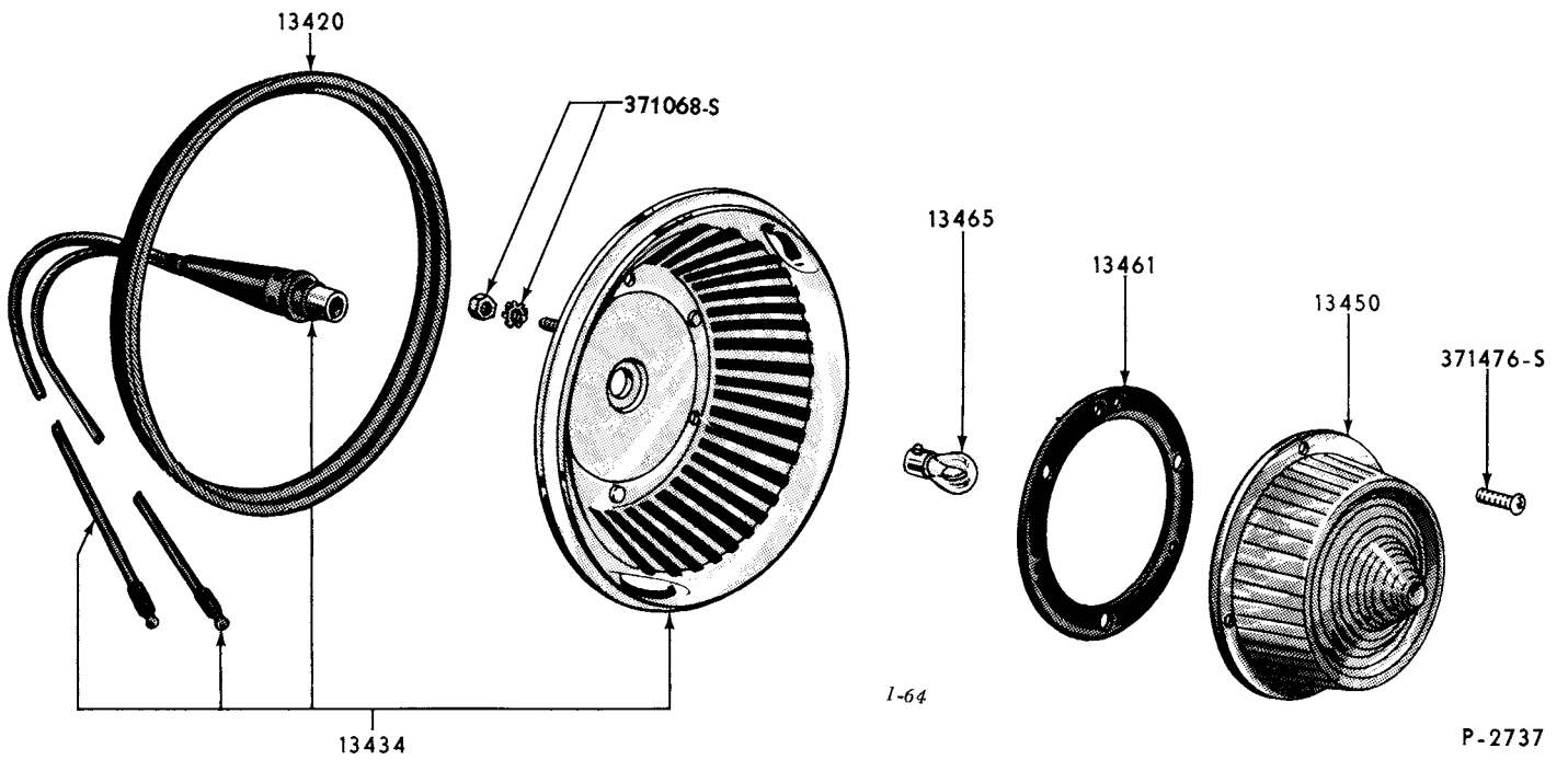
1959 REAR LAMP (FORD)
