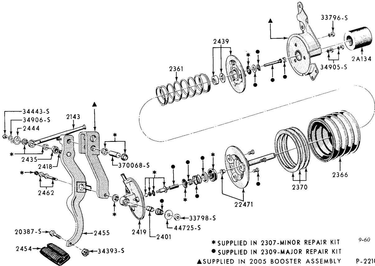
1957/59 POWER BRAKE BOOSTER (FORD) 1957 THUNDERBIRD
