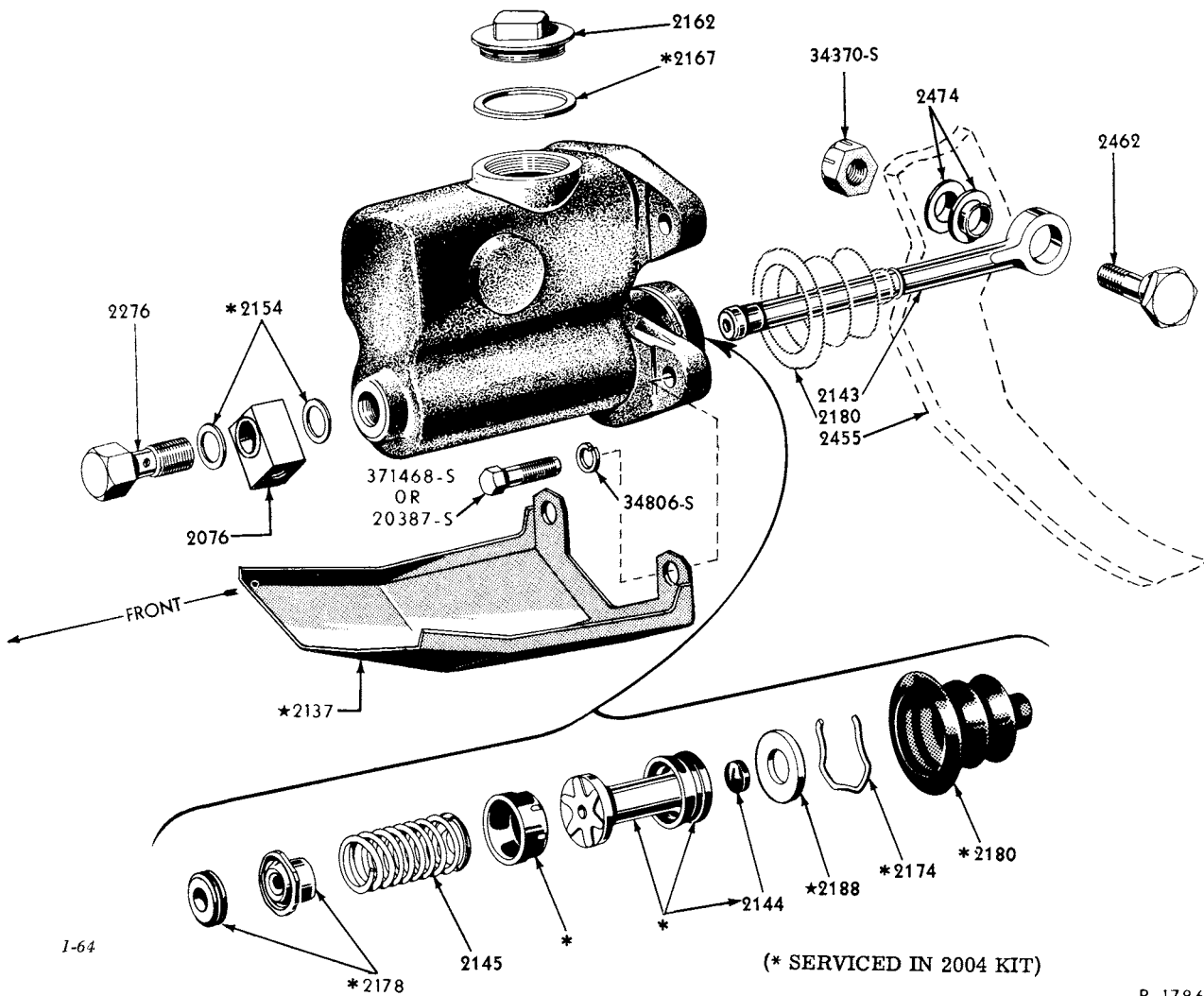
1955/ BRAKE MASTER CYLINDER (THUNDERBIRD)
