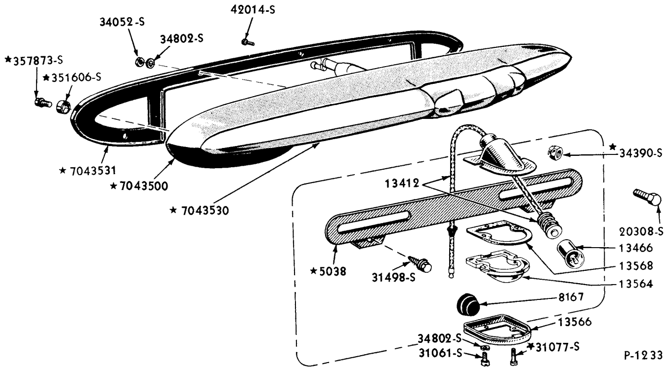
1951 LICENSE PLATE LAMP
