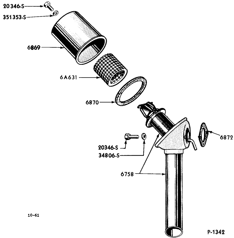
1954/57 CRANKCASE VENT SYSTEM (FORD-8 CYLINDER)-TYPICAL
