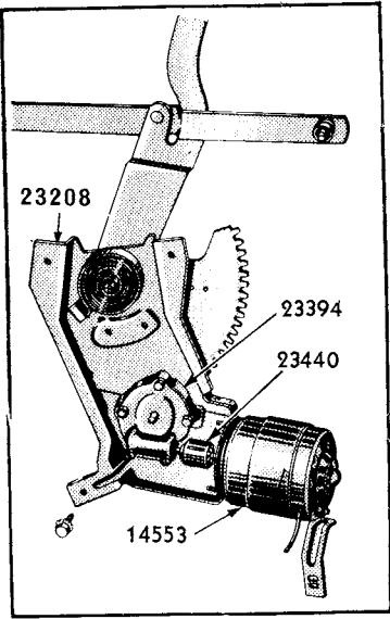
ELECTRIC REGULATOR
