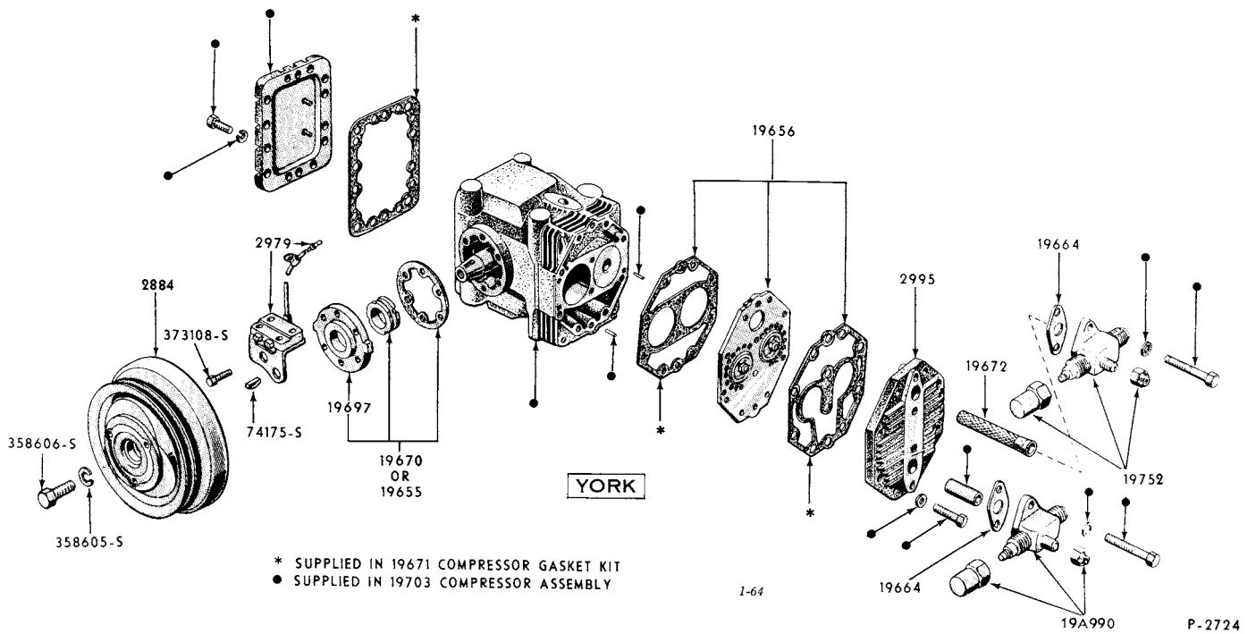
1958/59 FORD & THUNDERBIRD AIR CONDITIONER COMPRESSOR, PULLEYS & RELATED PARTS (SIDE MOUNTED HOSES)
