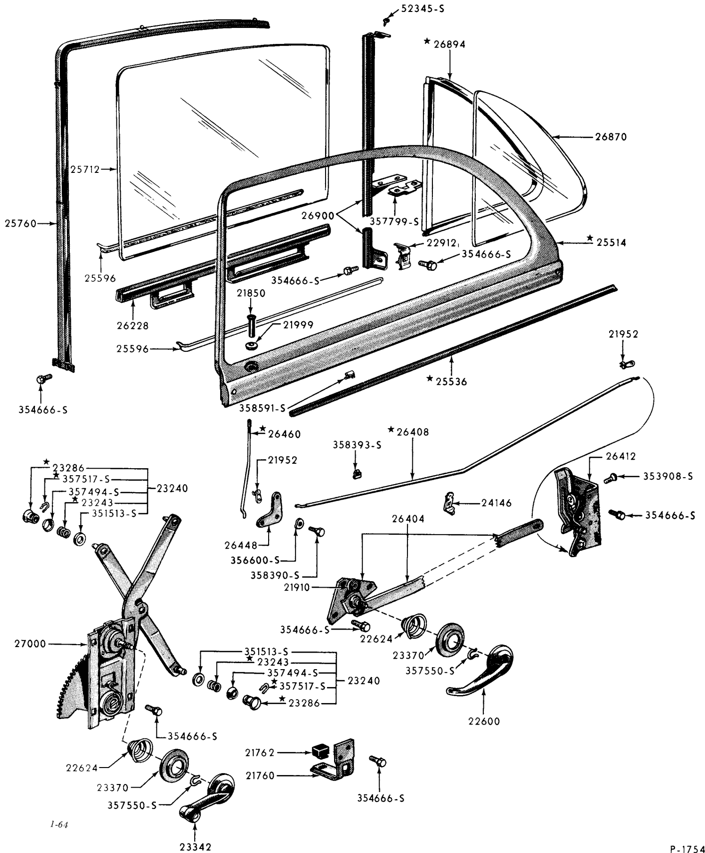
1955/56 TYPICAL REAR DOOR PARTS WITH MANUAL REGULATOR (BODY TYPES 73, 79)
