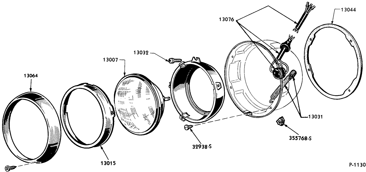
1951 HEADLAMP
