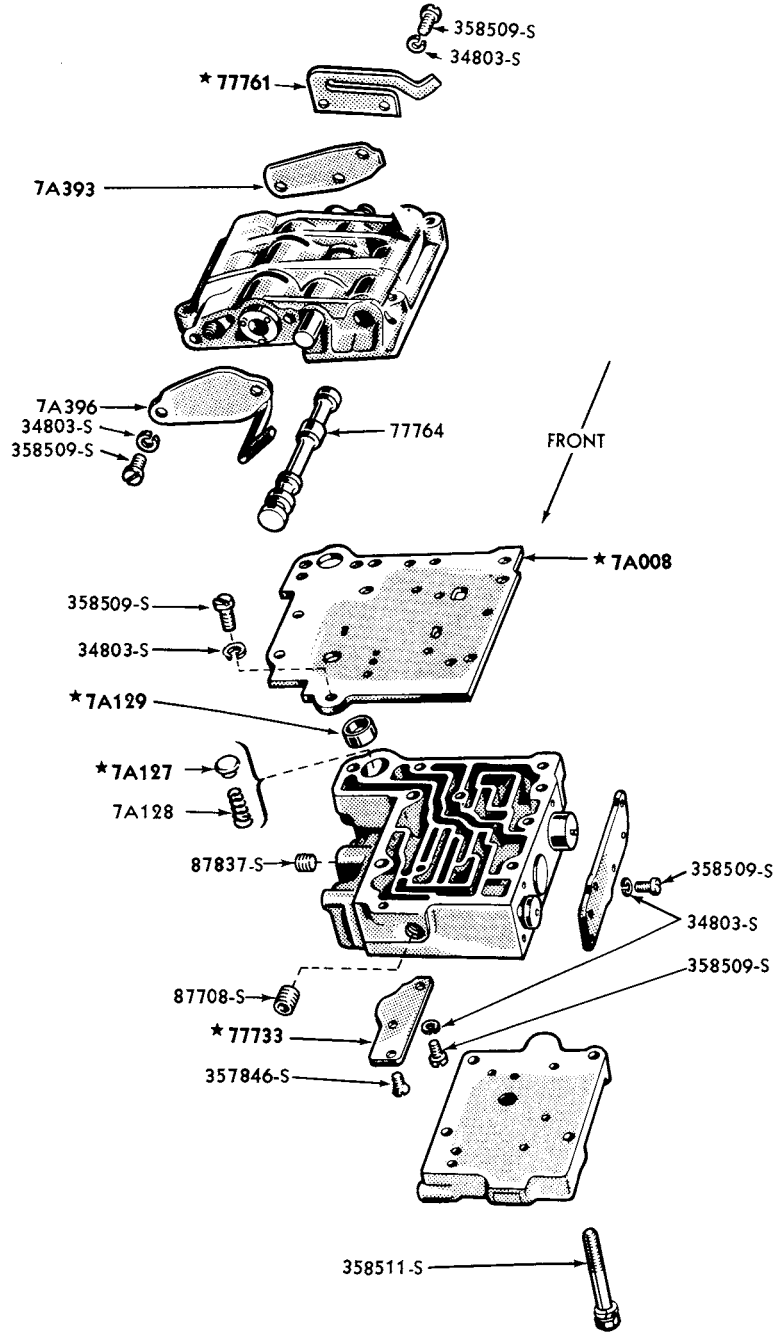
1951/54 MAIN CONTROL (FORDOMATIC TRANSMISSION)
