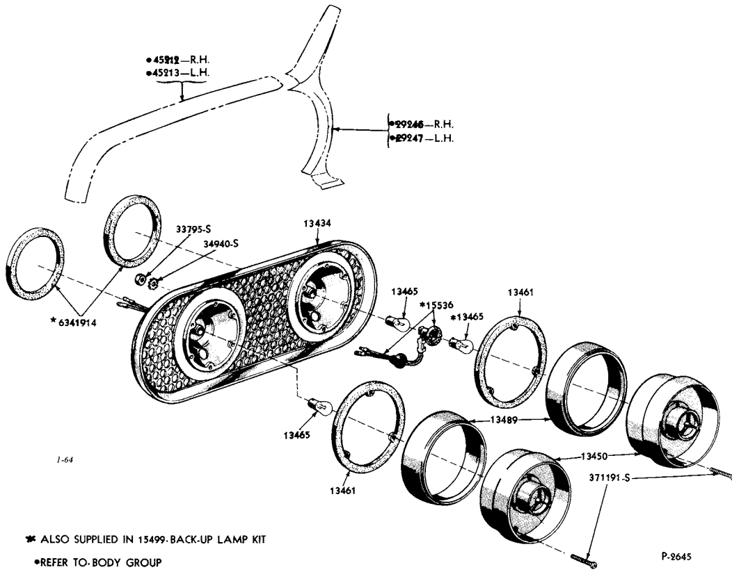
1958 REAR LAMP & BACK-UP LAMP (THUNDERBIRD)
