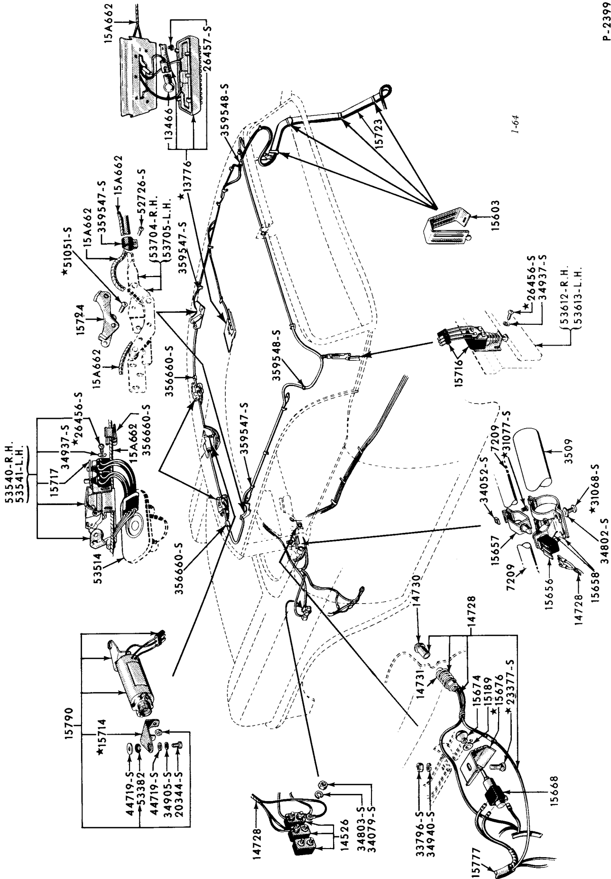
1957/59 ELECTRICAL SYSTEM (RETRACTABLE HARDTOP ROOF SECTION)
