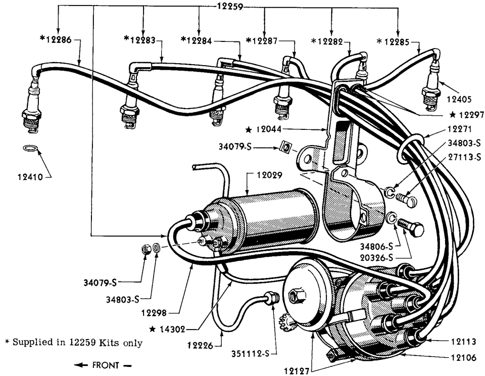
1949/51 IGNITION WIRING (6 CYLINDER 226 ENGINE)
