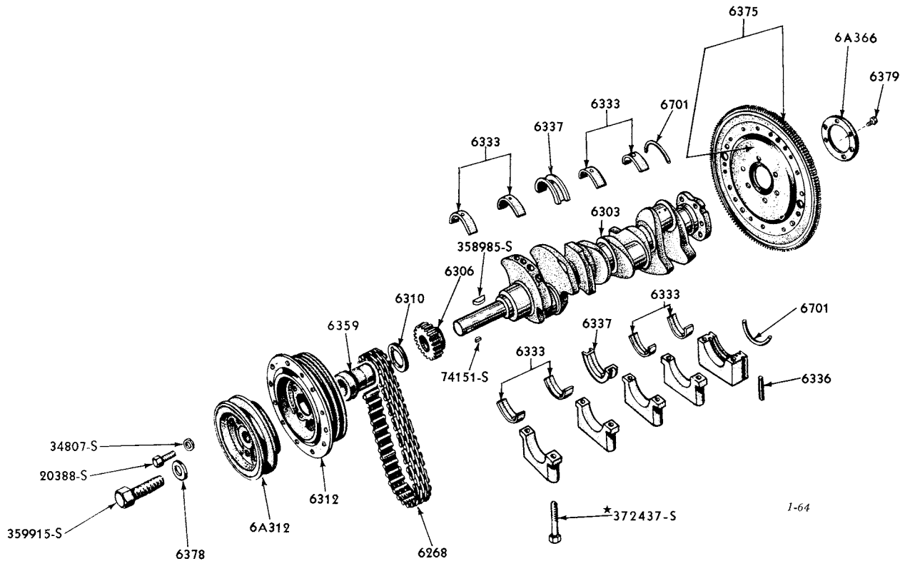
1959/ CRANKSHAFT, FLYWHEEL & RELATED PARTS (8 CYLINDER 430 ENGINE)(THUNDERBIRD)-TYPICAL
