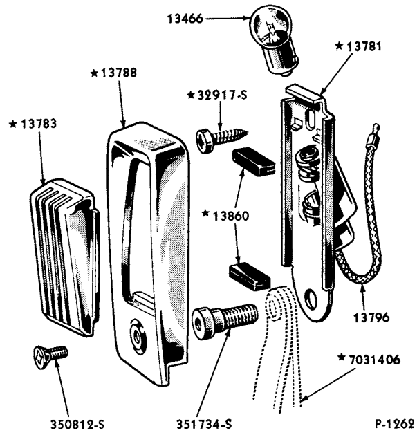
1952/53 PILLAR LAMP (EXCEPT VICTORIA)
