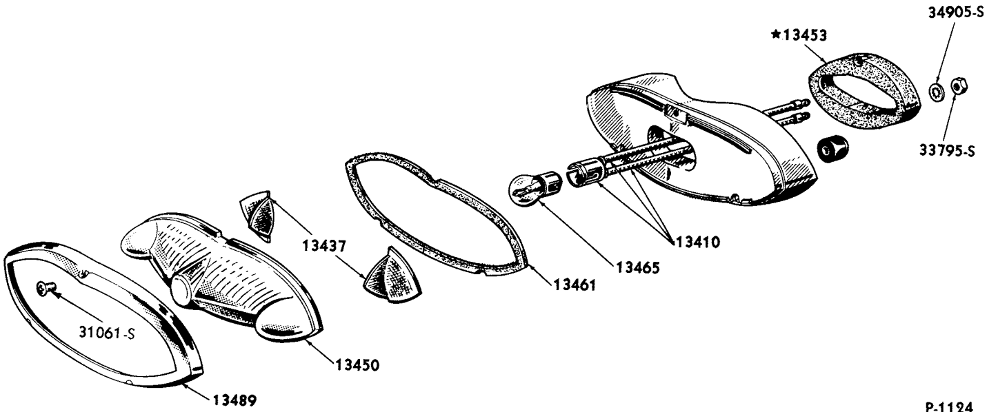
1951 REAR LAMP (EXCEPT STATION WAGON)
