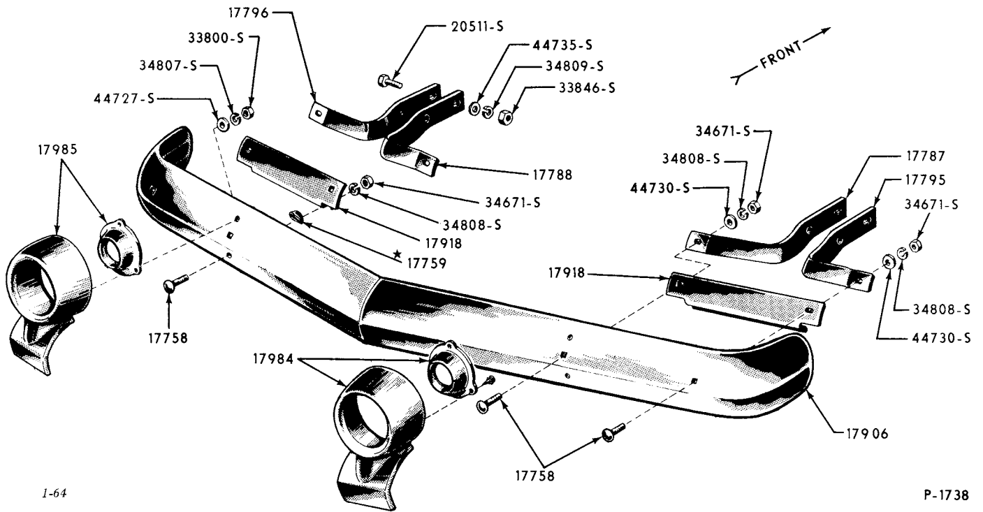
1955 REAR BUMPER (THUNDERBIRD)
