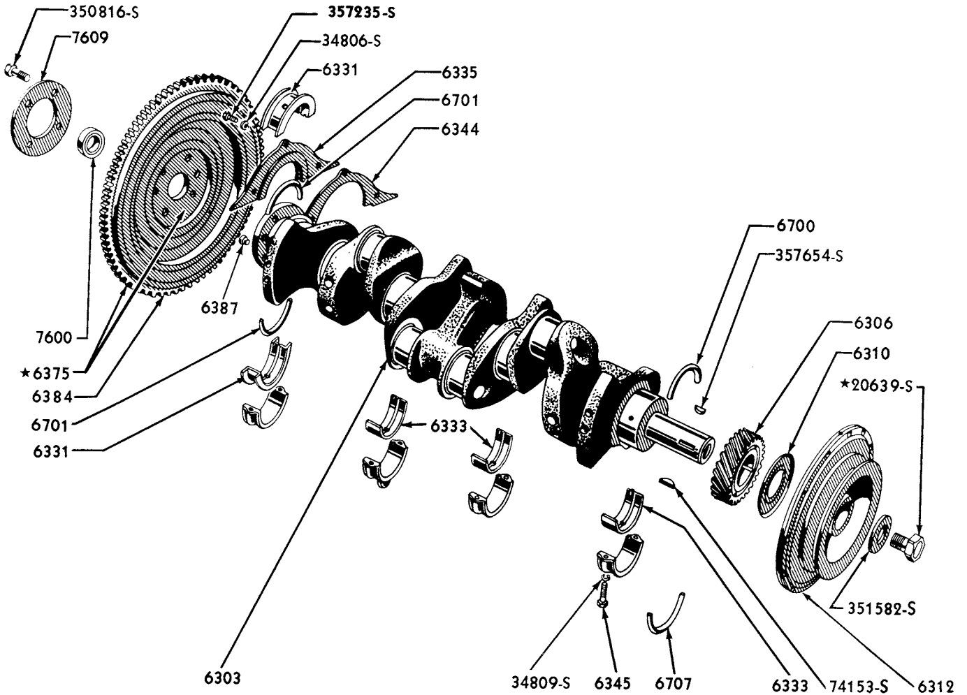
1952/ "TYPICAL" CRANKSHAFT, FLYWHEEL AND RELATED PARTS (6 CYLINDER 215, 223 ENGINES)
