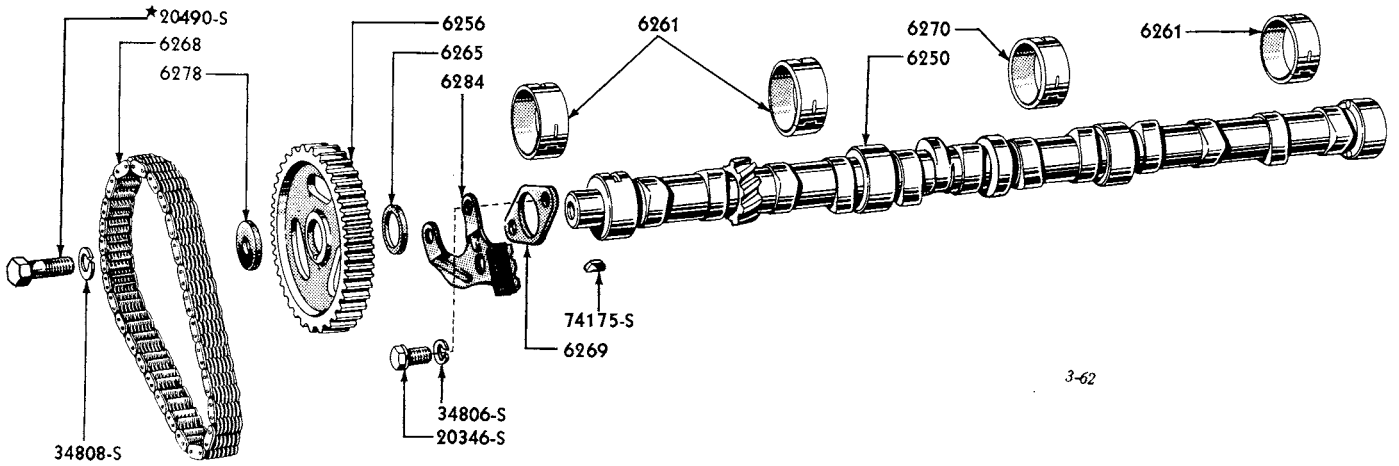
1954/ CAMSHAFT, GEAR, BEARINGS, ETC. (6 CYLINDER 223 ENGINE)
