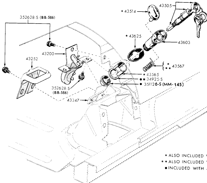
1962/63 FAIRLANE TYPICAL LUGGAGE COMPARTMENT DOOR LOCK & RELATED PARTS - BODY TYPES B (except 71)
