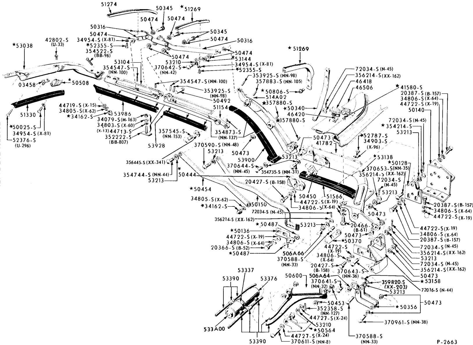
FOLDING TOP PARTS-LESS TRIM 1960 THUNDERBIRD-BODY TYPE 76
