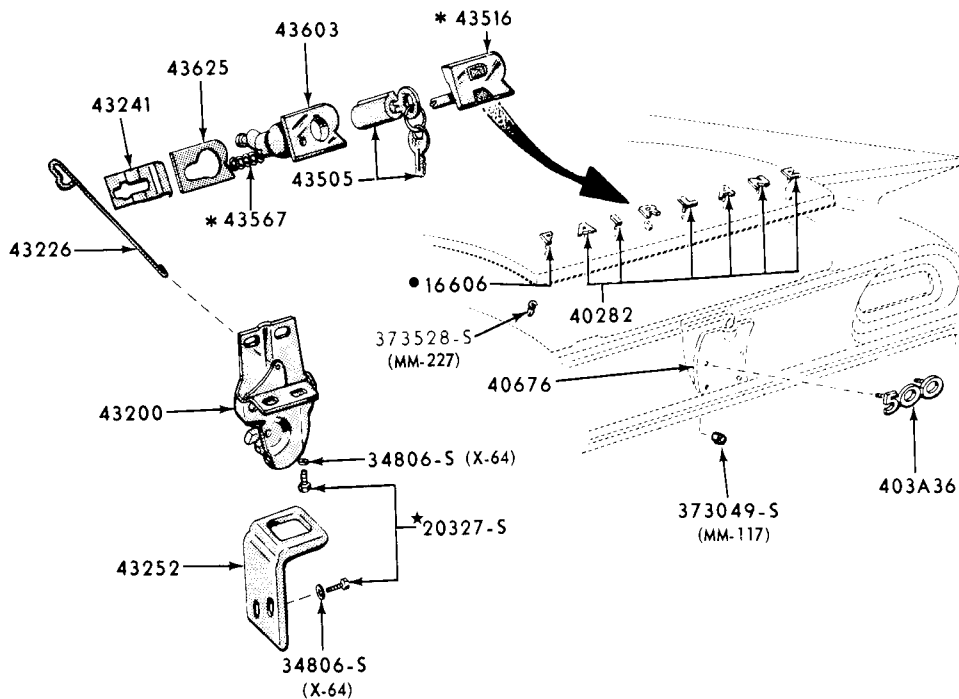
LUGGAGE COMPARTMENT DOOR LATCH and RELATED PARTS 1960 FORD - BODY TYPES 58E, 64F, G
