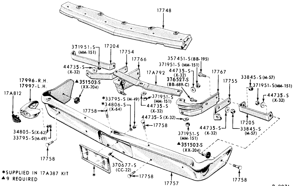
1960 FRONT BUMPER & RELATED PARTS (FORD)
