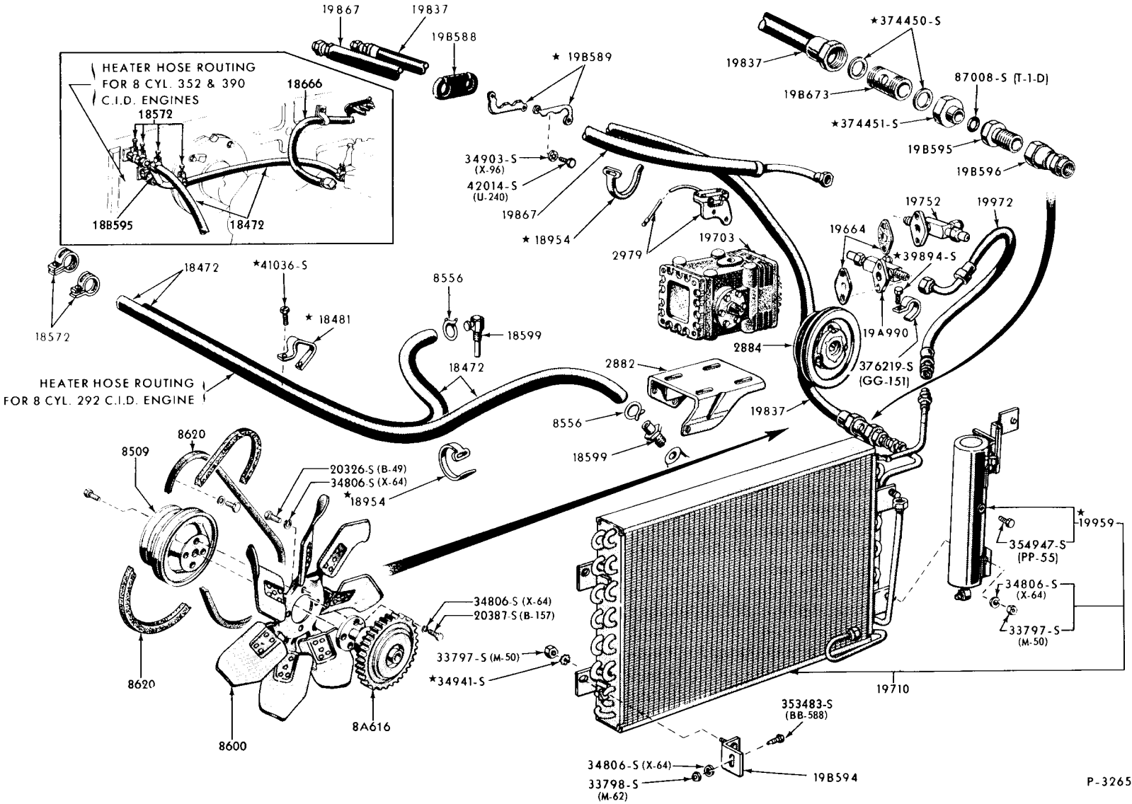
1961/62 FORD INTEGRAL & HANG-ON AIR CONDITIONER CONDENSER, DEHYDRATOR, COMPRESSOR & RELATED PARTS (8 CYLINDER)
