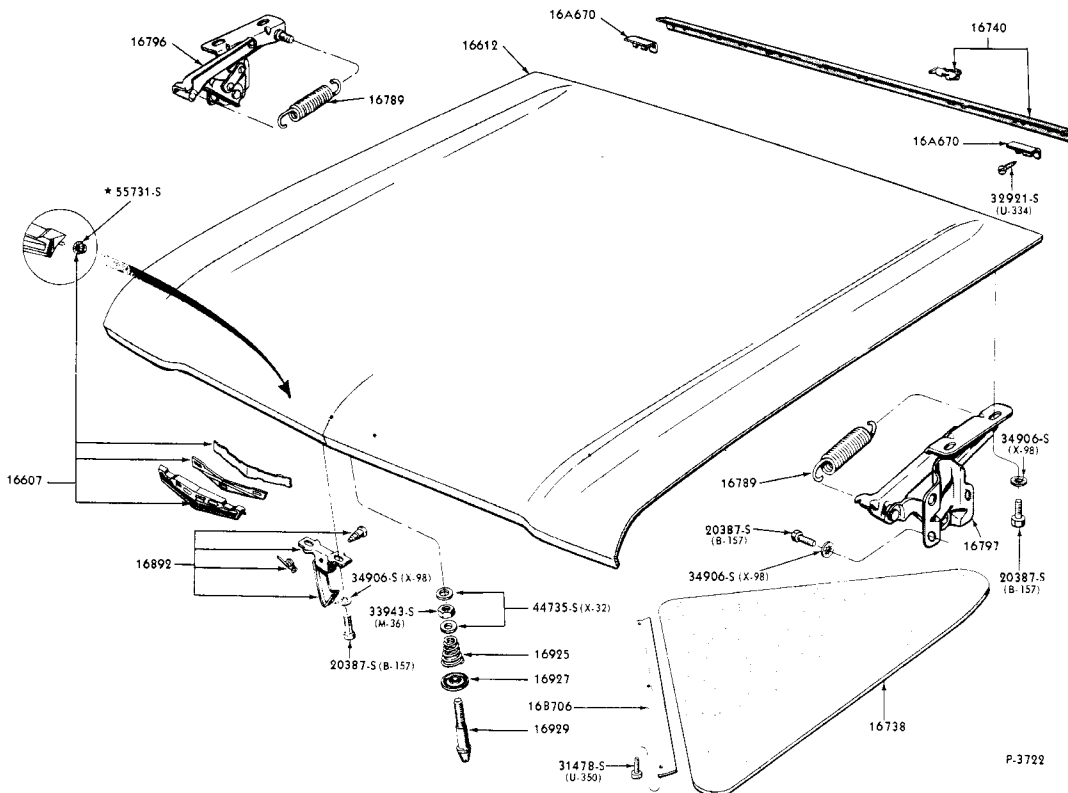
1962 HOOD and RELATED PARTS (FAIRLANE)
