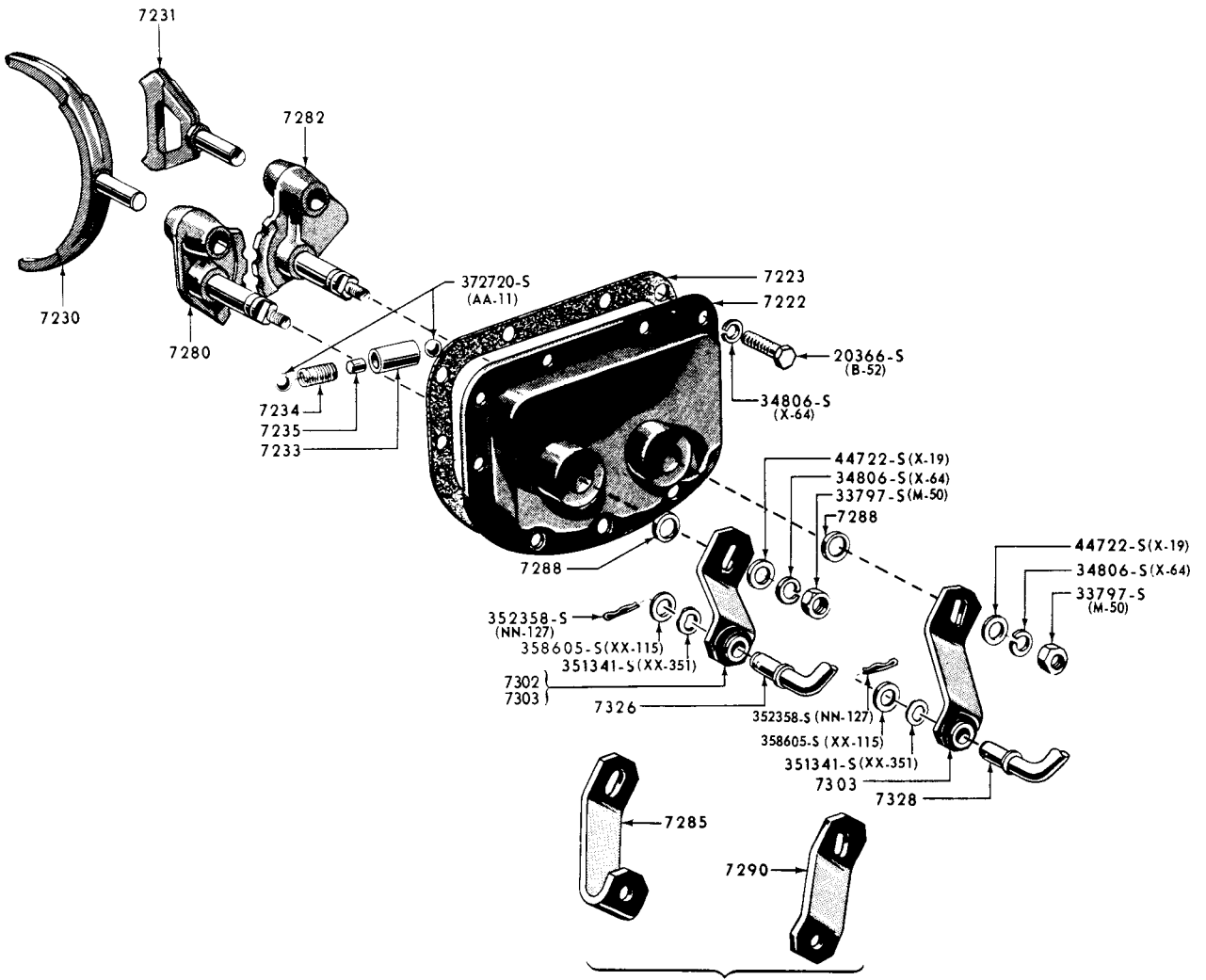
OVERDRIVE TRANSMISSION
